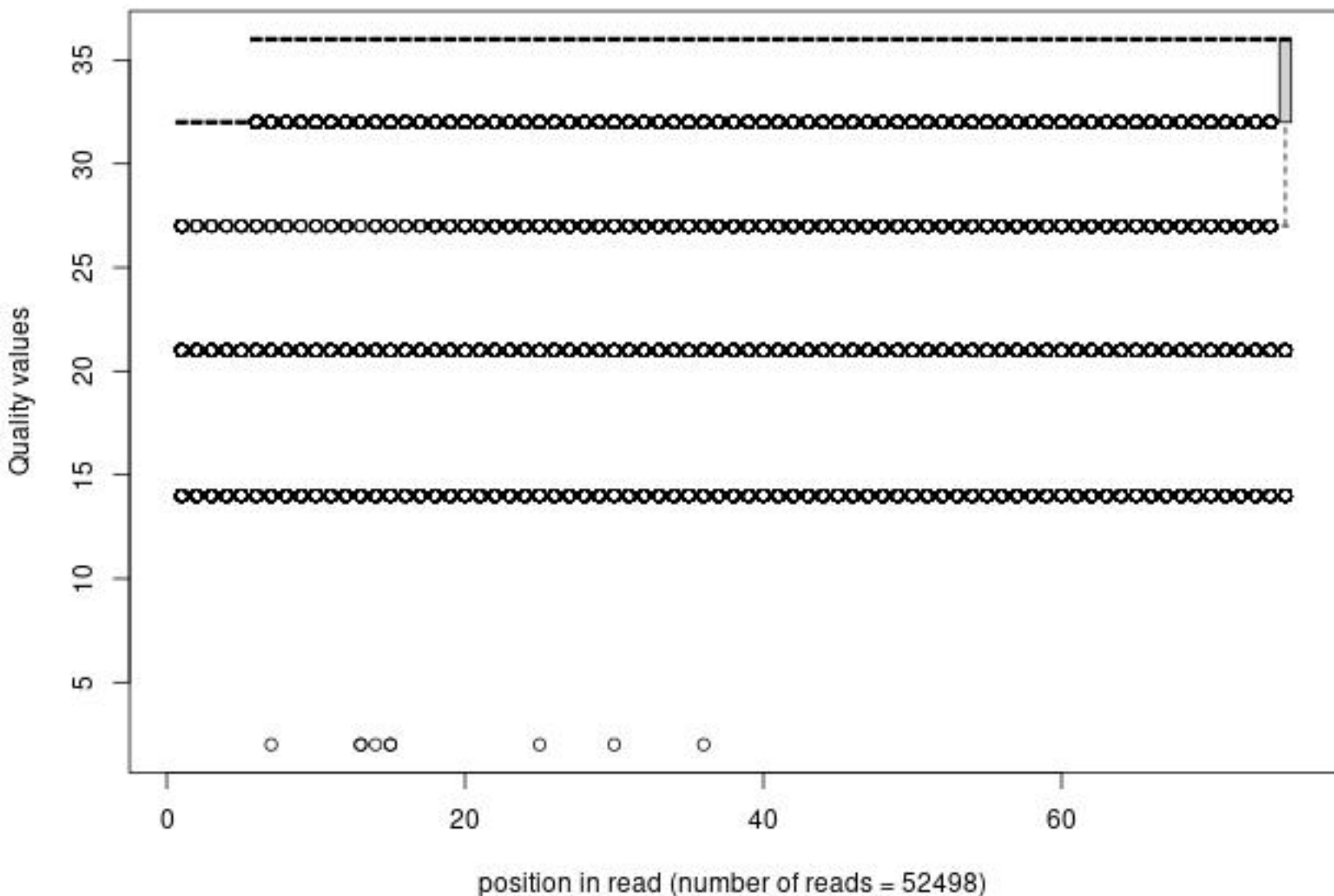
Quality distribution by position in read n2_wldtyp_xxxxx_rs053_1_frac1000
