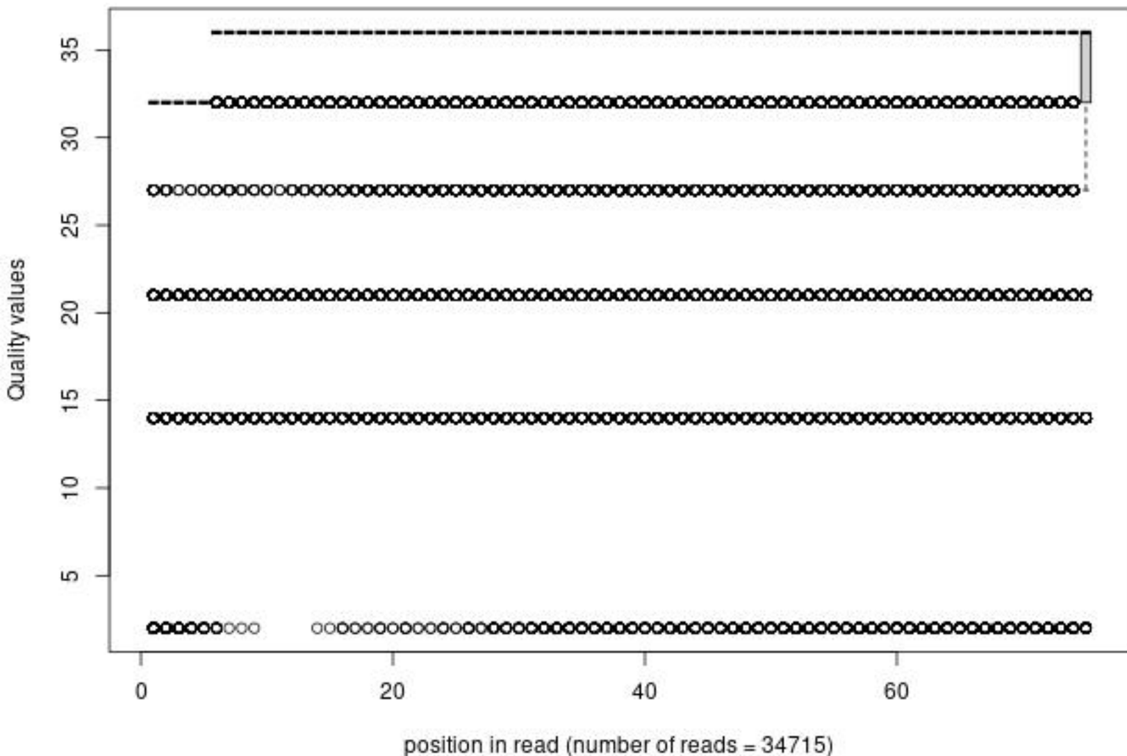
Quality distribution by position in read n2_snu66x_sz371_rs061_2_frac1000
