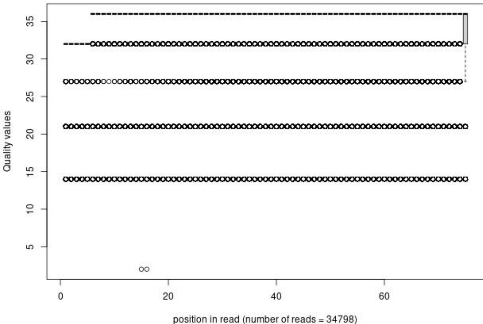
Quality distribution by position in read n2_snrp27_sz211_rs056_1_frac1000
