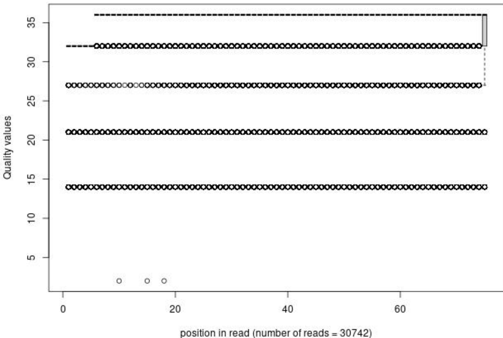
Quality distribution by position in read n2_snu66x_sz370_rs058_1_frac1000
