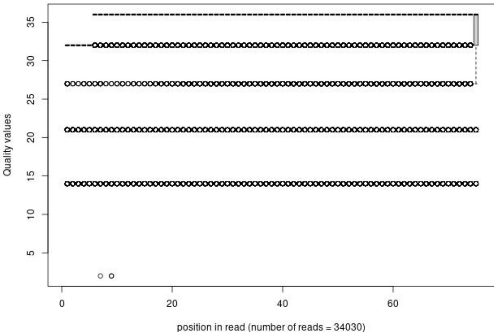
Quality distribution by position in read n2_snu66x_sz370_rs057_1_frac1000
