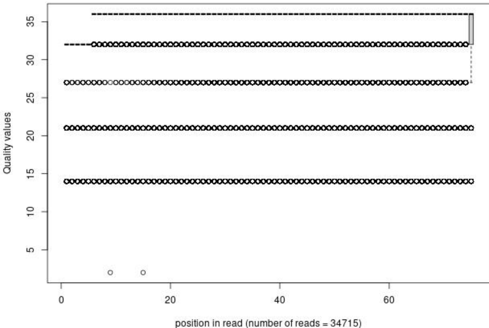
Quality distribution by position in read n2_snu66x_sz371_rs061_1_frac1000
