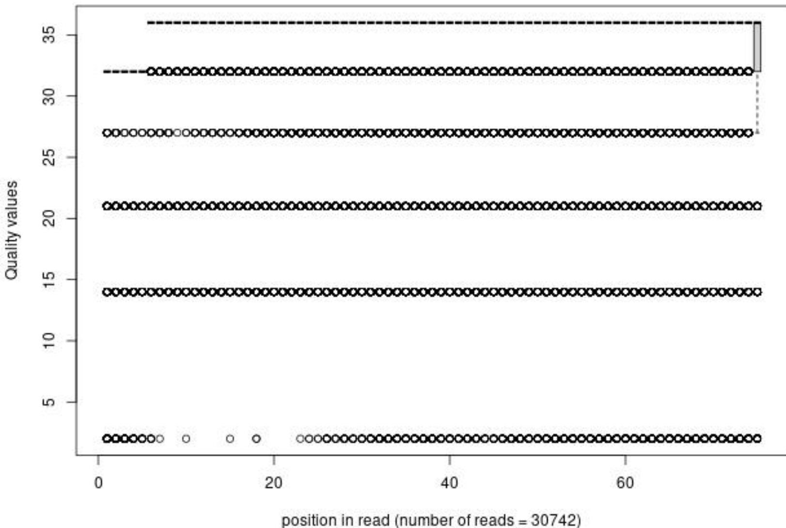
Quality distribution by position in read n2_snu66x_sz370_rs058_2_frac1000
