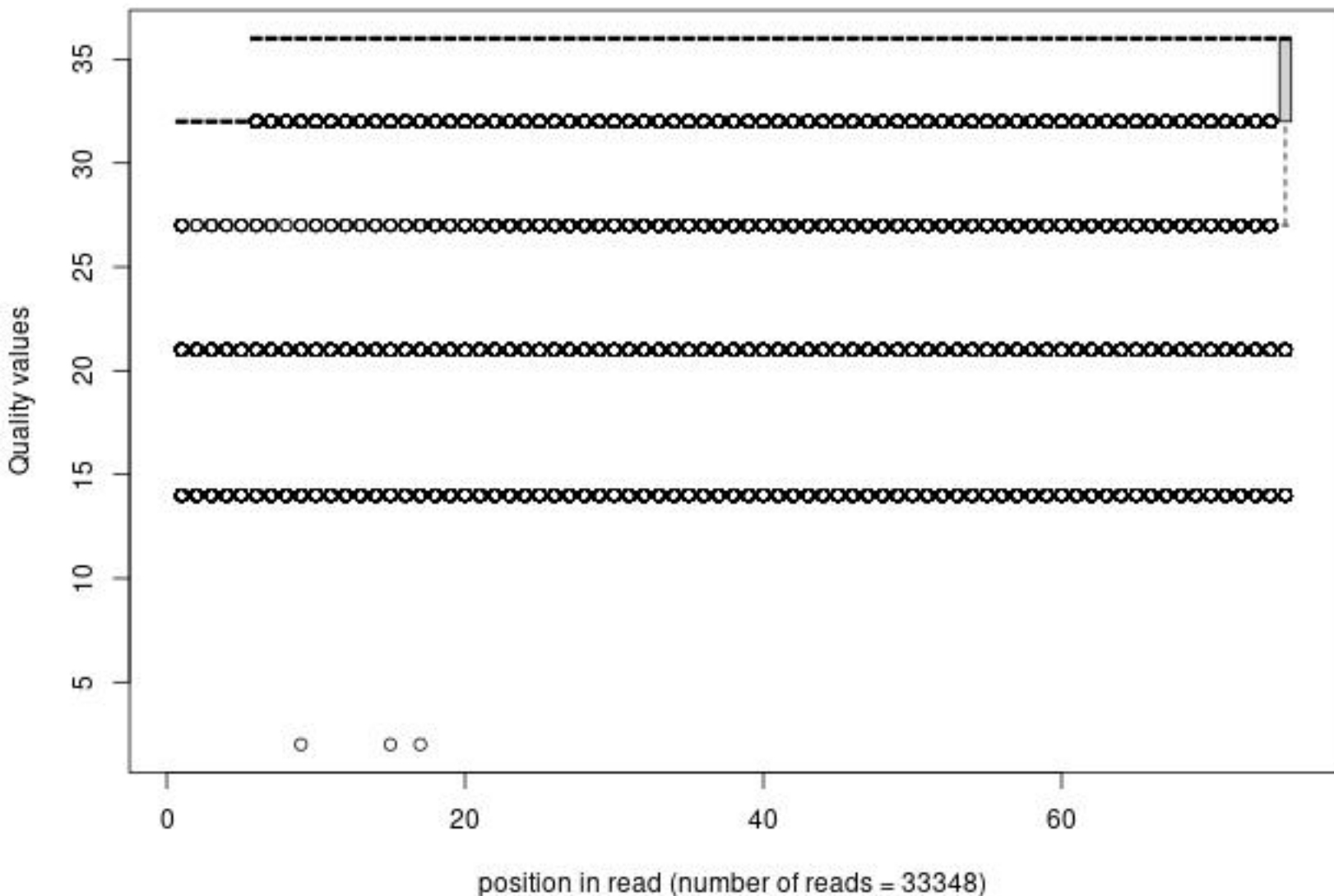
Quality distribution by position in read n2_snrp27_sz211_rs054_1_frac1000
