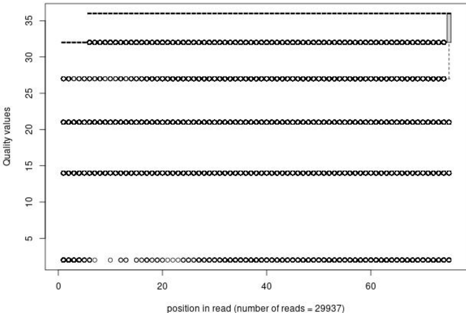
Quality distribution by position in read n2_snu66x_sz371_rs060_2_frac1000
