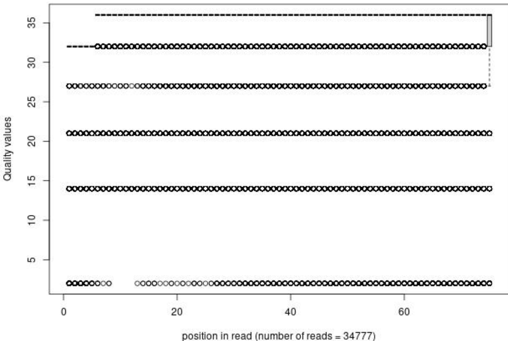
Quality distribution by position in read n2_snu66x_sz370_rs059_2_frac1000
