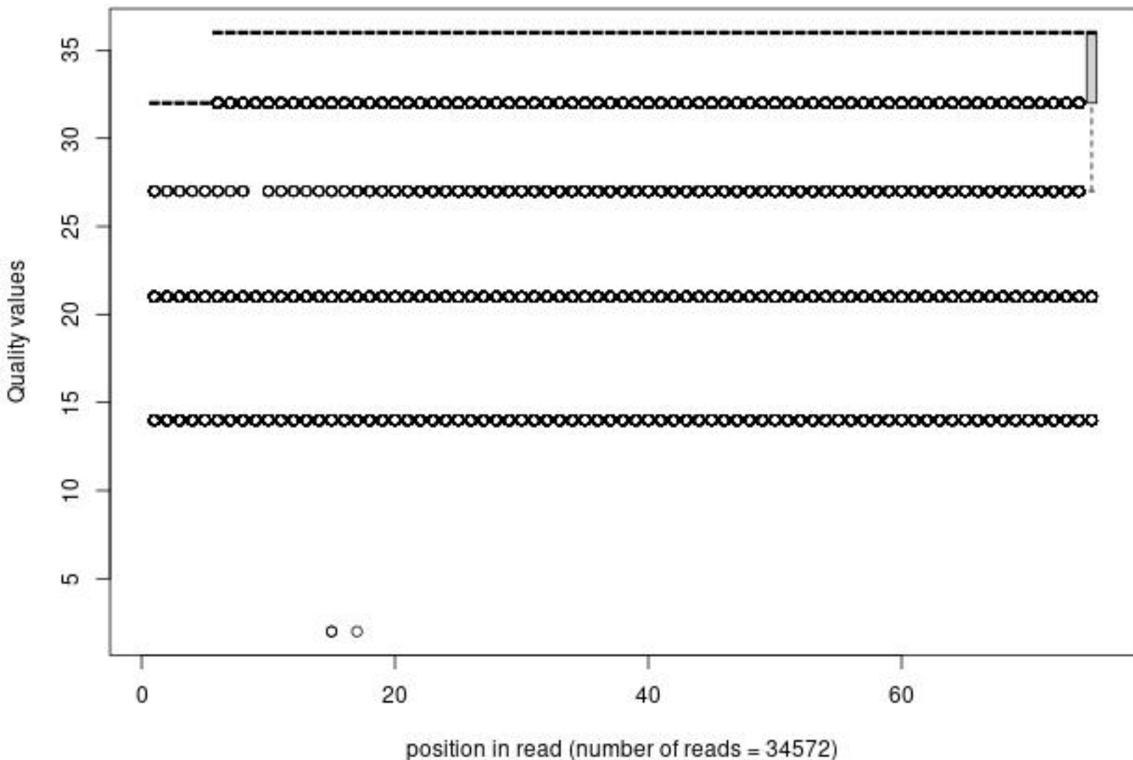
Quality distribution by position in read n2_snu66x_sz371_rs062_1_frac1000
