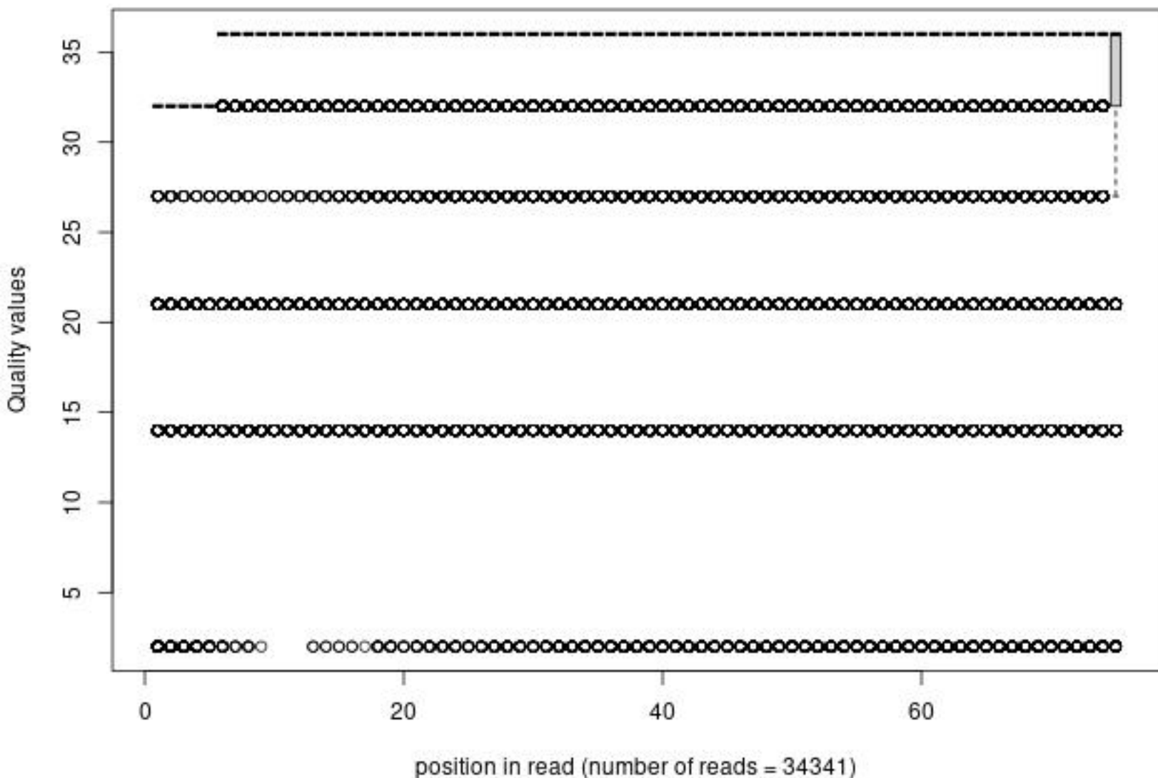
Quality distribution by position in read n2_wldtyp_xxxxx_rs052_2_frac1000
