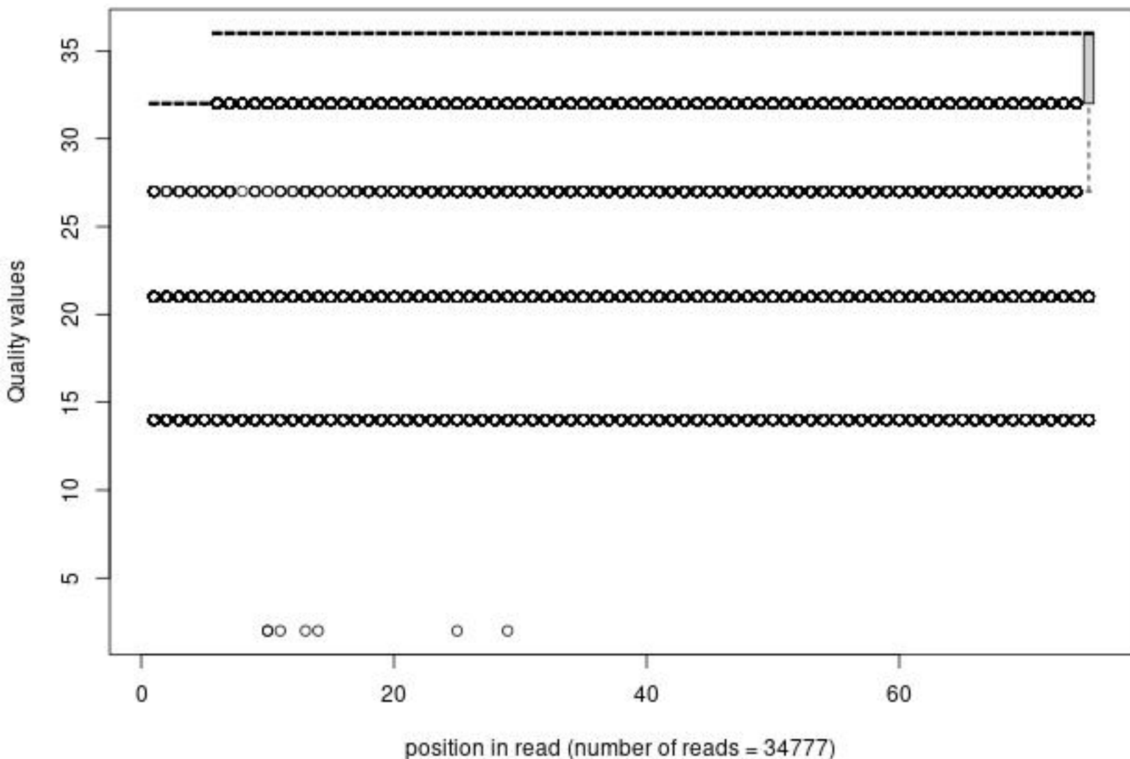
Quality distribution by position in read n2_snu66x_sz370_rs059_1_frac1000
