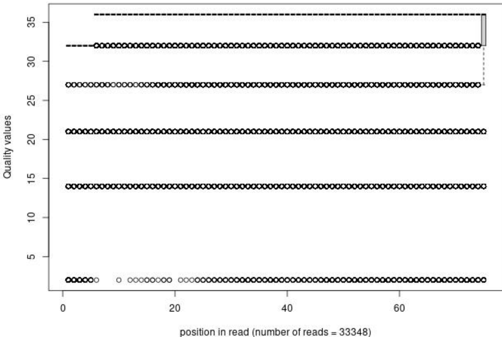
Quality distribution by position in read n2_snrp27_sz211_rs054_2_frac1000
