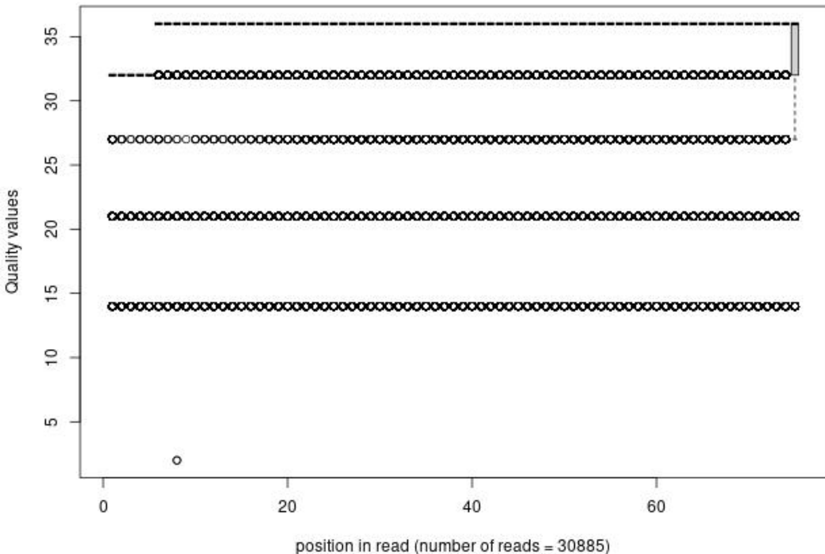
Quality distribution by position in read n2_wldtyp_xxxxx_rs051_1_frac1000
