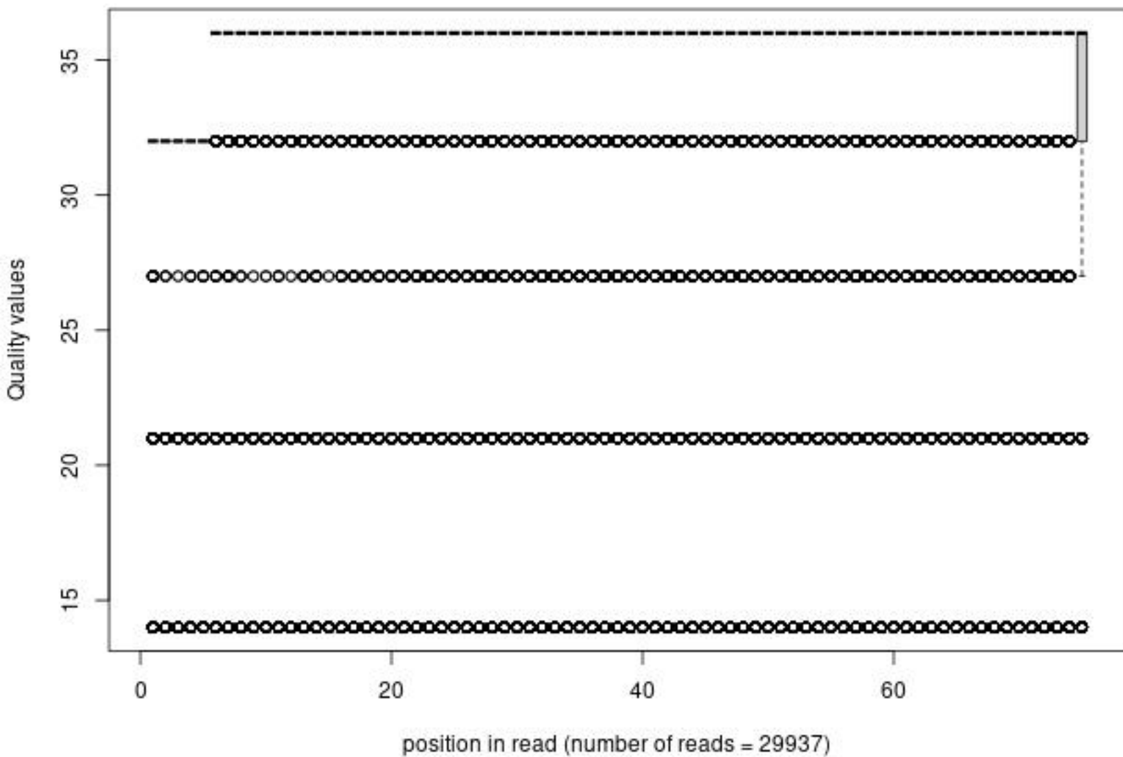
Quality distribution by position in read n2_snu66x_sz371_rs060_1_frac1000
