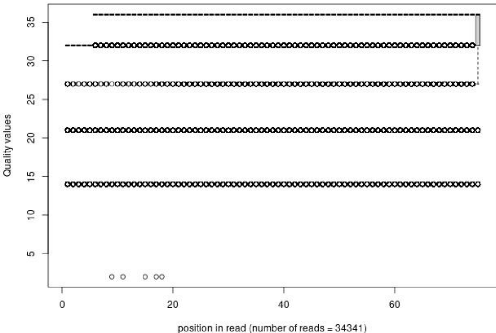
Quality distribution by position in read n2_wldtyp_xxxx_rs052_1_frac1000
