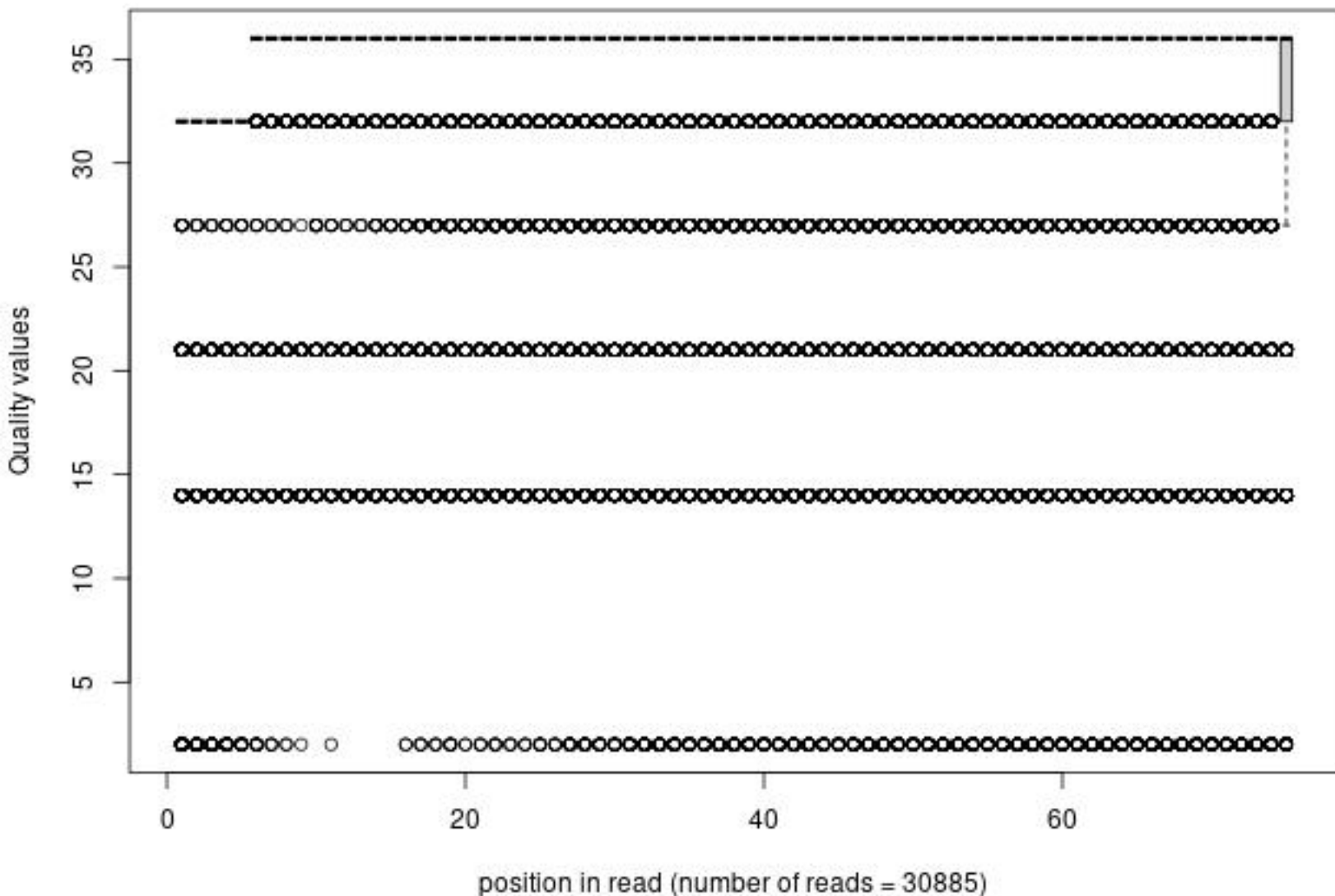
Quality distribution by position in read n2_wldtyp_xxxxx_rs051_2_frac1000
