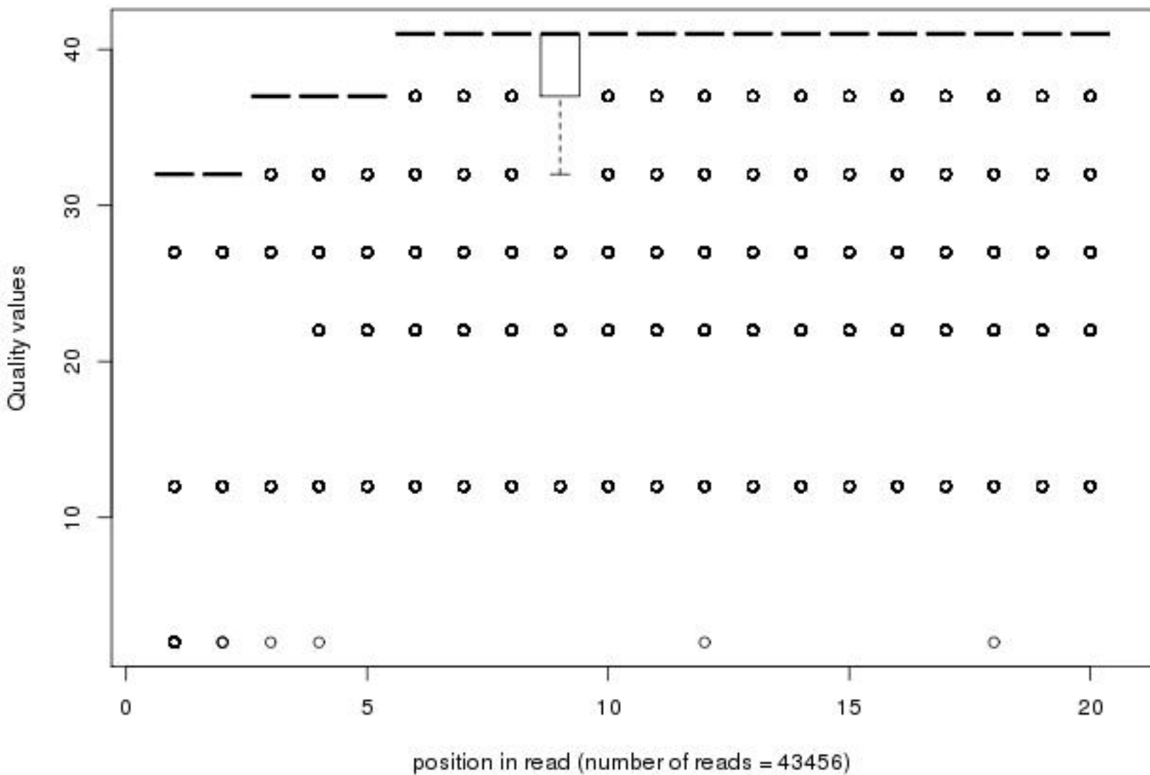
Quality distribution by position in read n2_unc73prp8ex_sy013_01of20_1_frac50_first20
