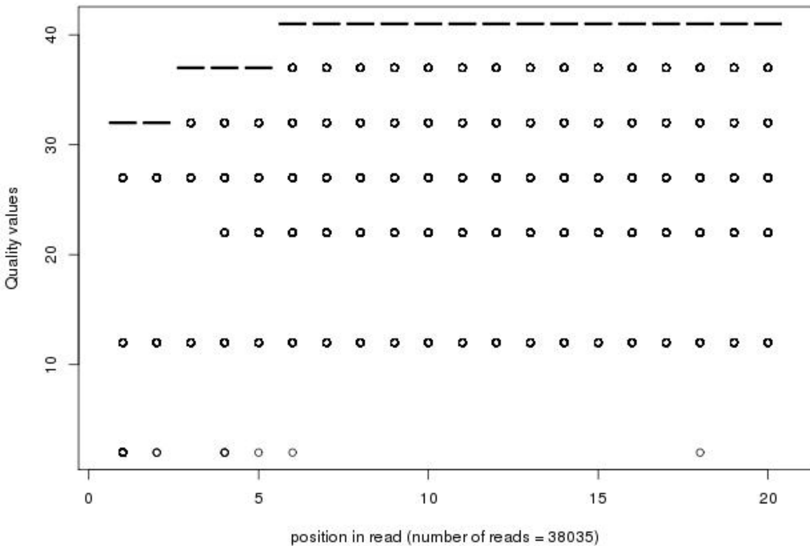
Quality distribution by position in read n2_unc73prp8dx_sy003_01of20_1_frac50_first20
