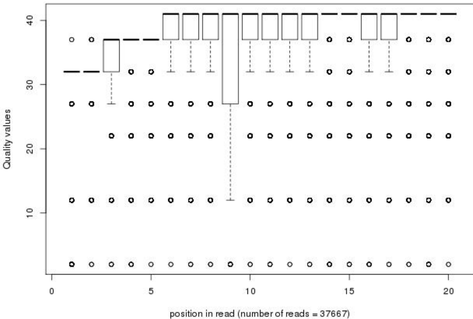
Quality distribution by position in read n2_unc73out2xx_sy016_01of20_2_frac50_first20
