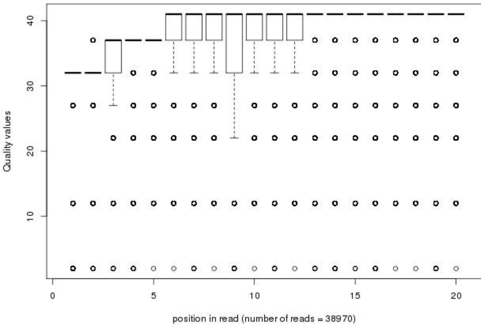
Quality distribution by position in read n2_unc73prp8fx_sy008_01of20_2_frac50_first20
