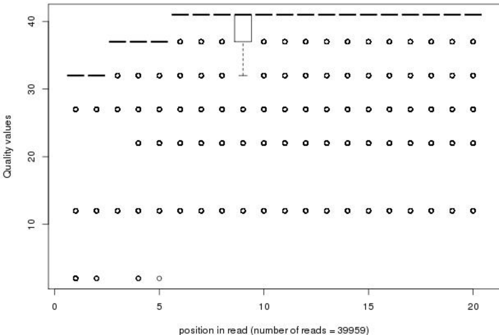
Quality distribution by position in read n2_unc73prp8eo_sy006_01of20_1_frac50_first20
