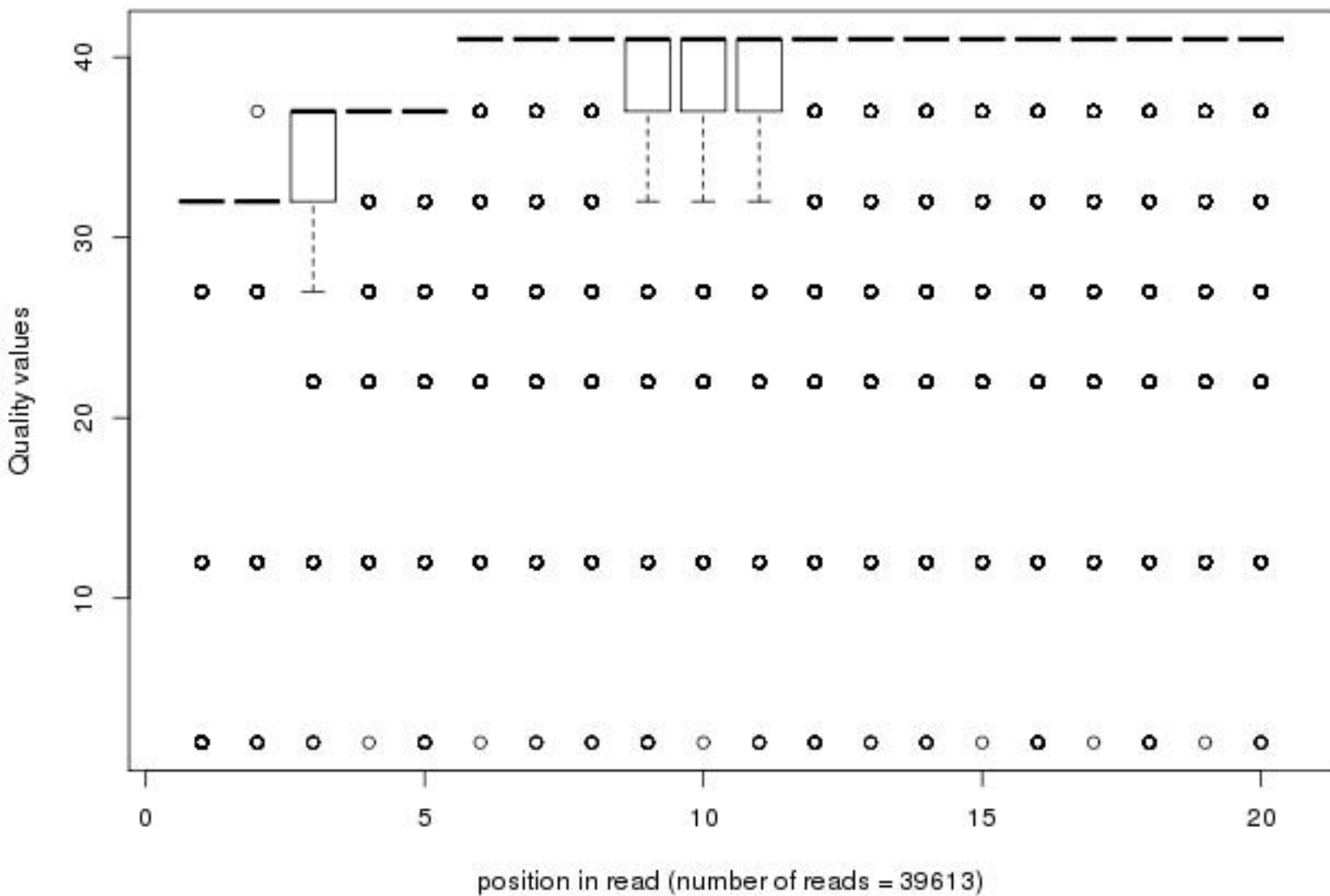
Quality distribution by position in read n2_unc73out2xx_sy015_01of20_2_frac50_first20
