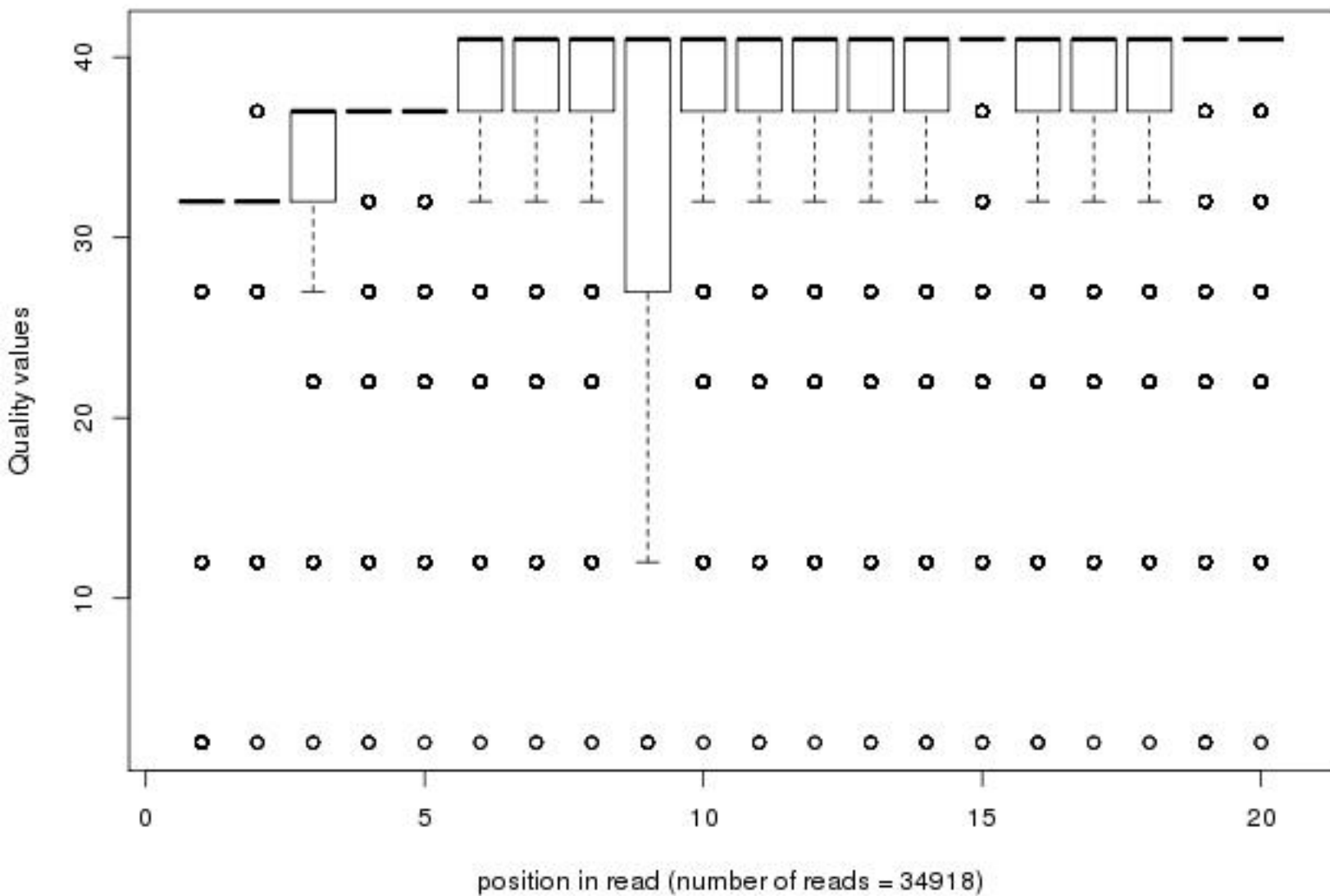
Quality distribution by position in read n2_dxbp1onlyxx_sy010_01of20_2_frac50_first20
