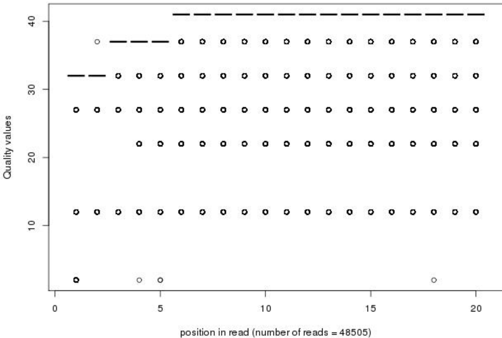
Quality distribution by position in read n2_wildtypexxx_sy001_01of20_1_frac50_first20
