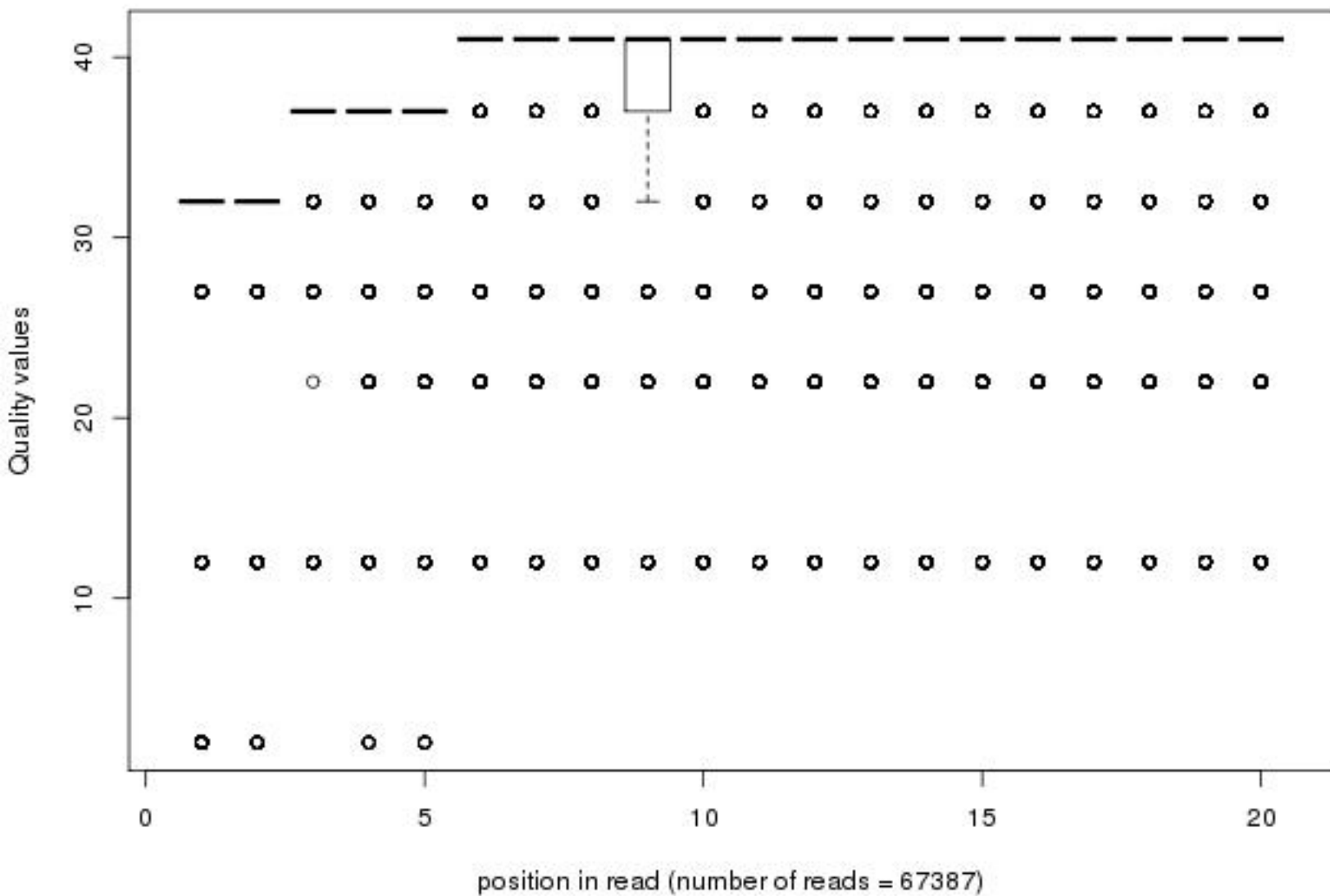
Quality distribution by position in read n2_unc73prp8ex_sy014_01of20_1_frac50_first20
