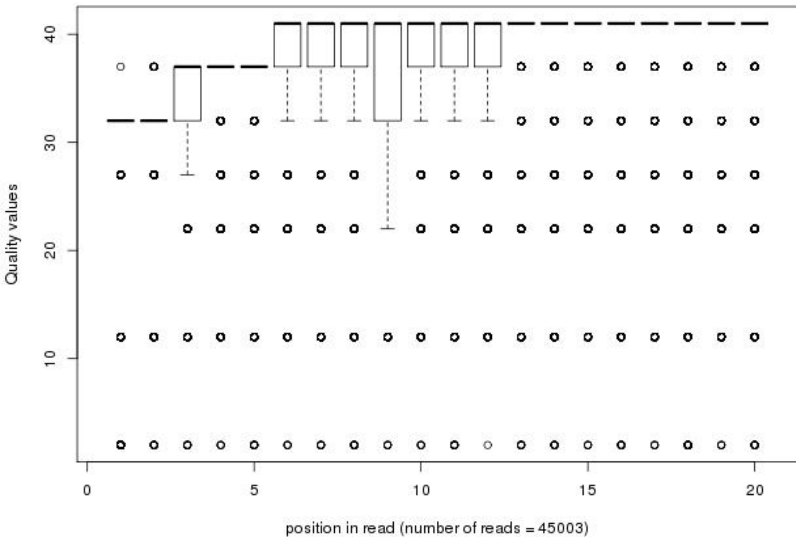
Quality distribution by position in read n2_unc73prp8eo_sy005_01of20_2_frac50_first20
