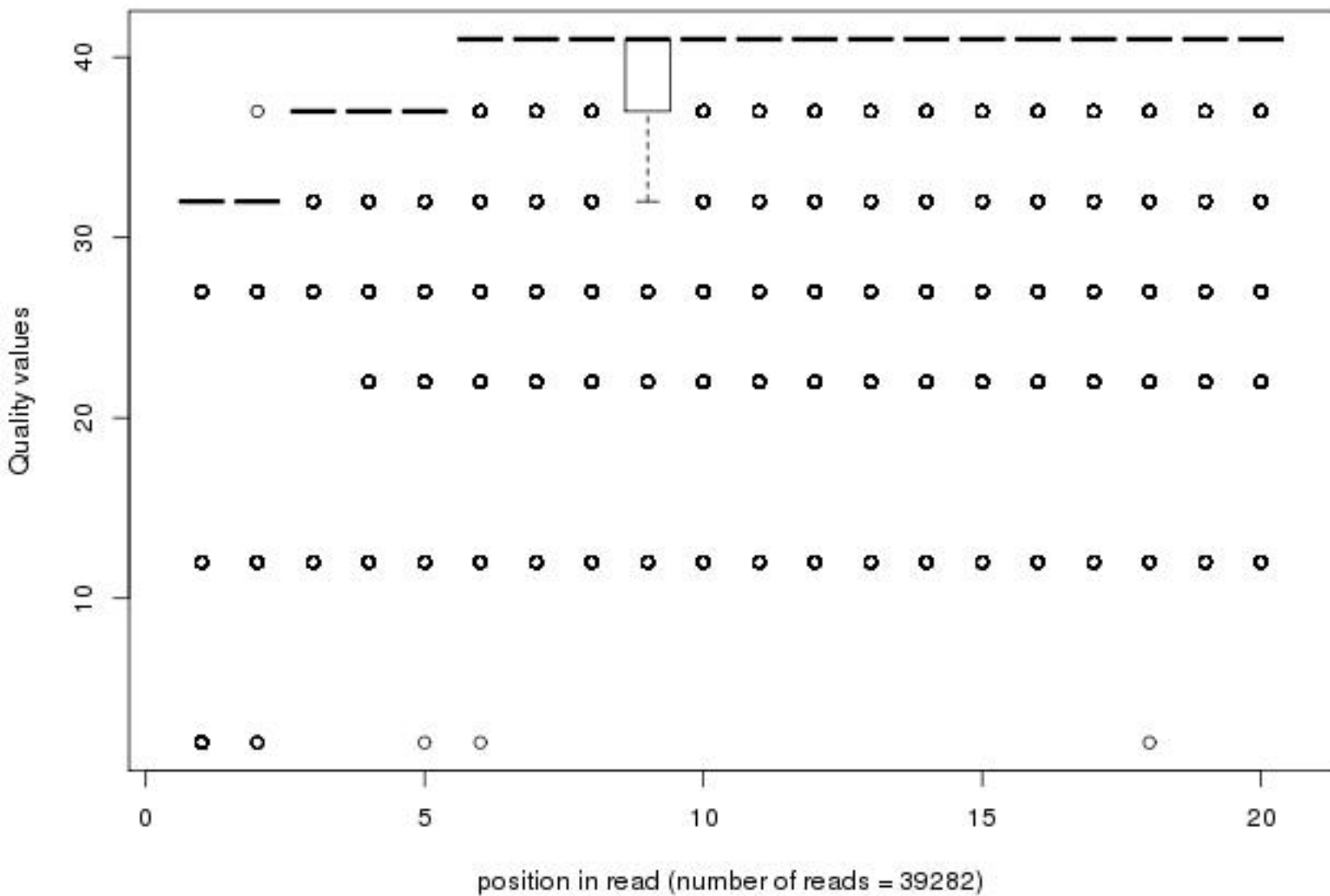
Quality distribution by position in read n2_unc73prp8fx_sy007_01of20_1_frac50_first20
