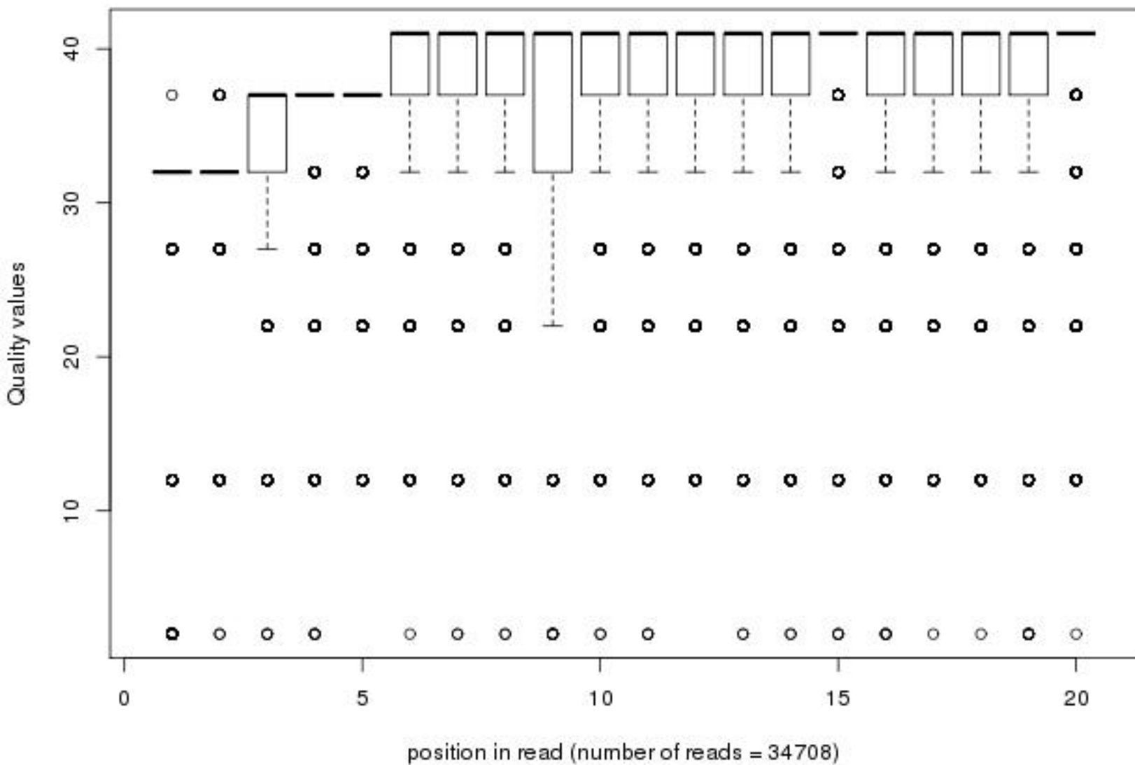
Quality distribution by position in read n2_unc73dxbp1x_sy012_01of20_2_frac50_first20
