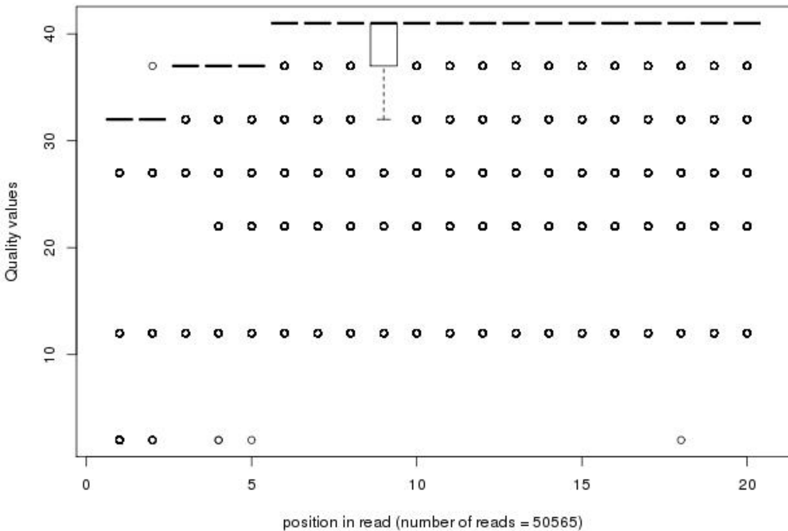
Quality distribution by position in read n2_unc73dxbp1x_sy011_01of20_1_frac50_first20
