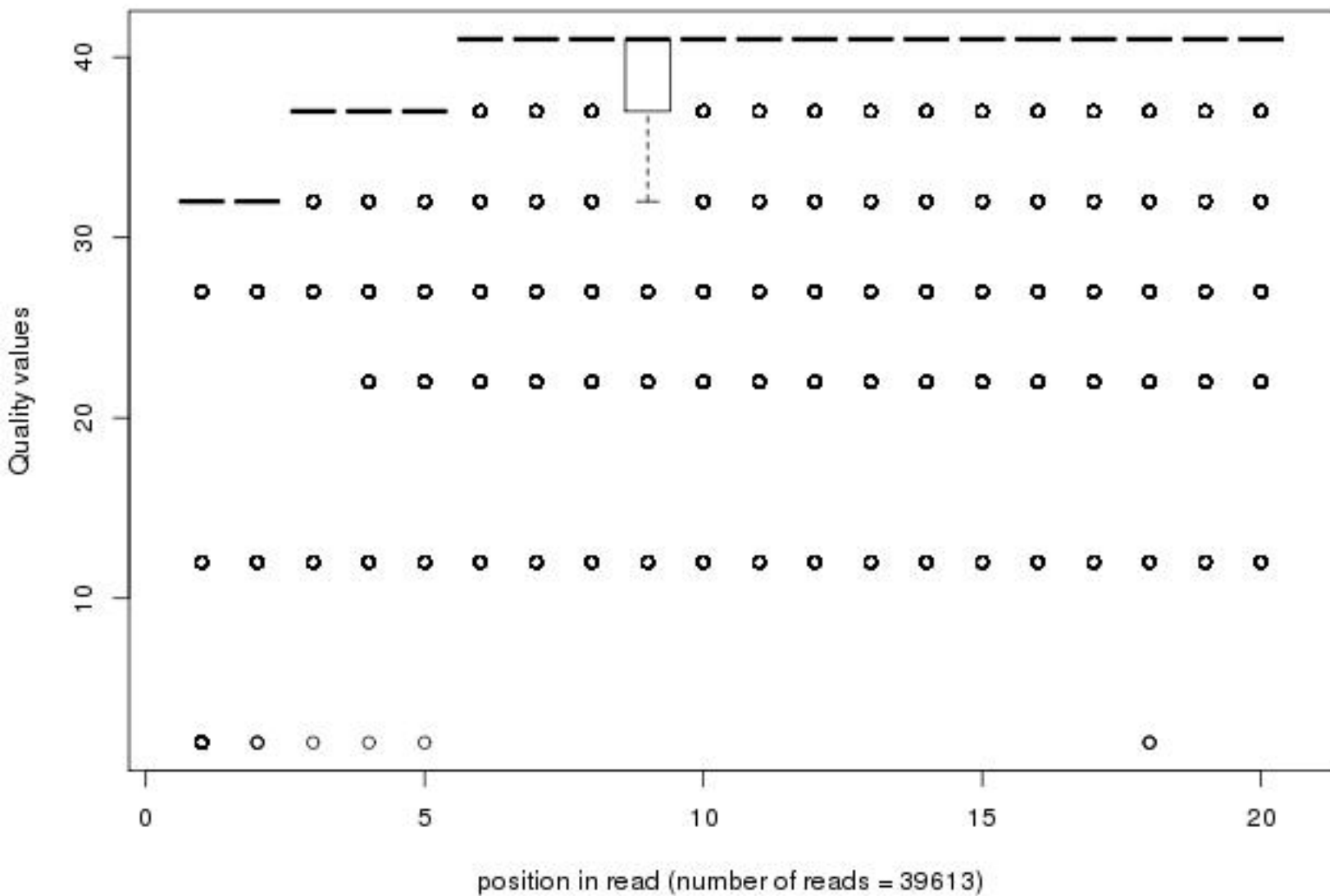
Quality distribution by position in read n2_unc73out2xx_sy015_01of20_1_frac50_first20
