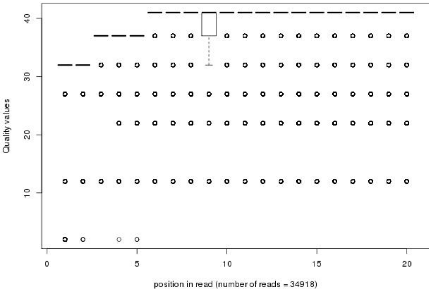
Quality distribution by position in read n2_dxbp1onlyxx_sy010_01of20_1_frac50_first20
