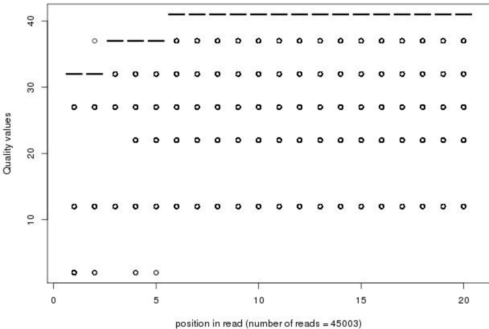
Quality distribution by position in read n2_unc73prp8eo_sy005_01of20_1_frac50_first20
