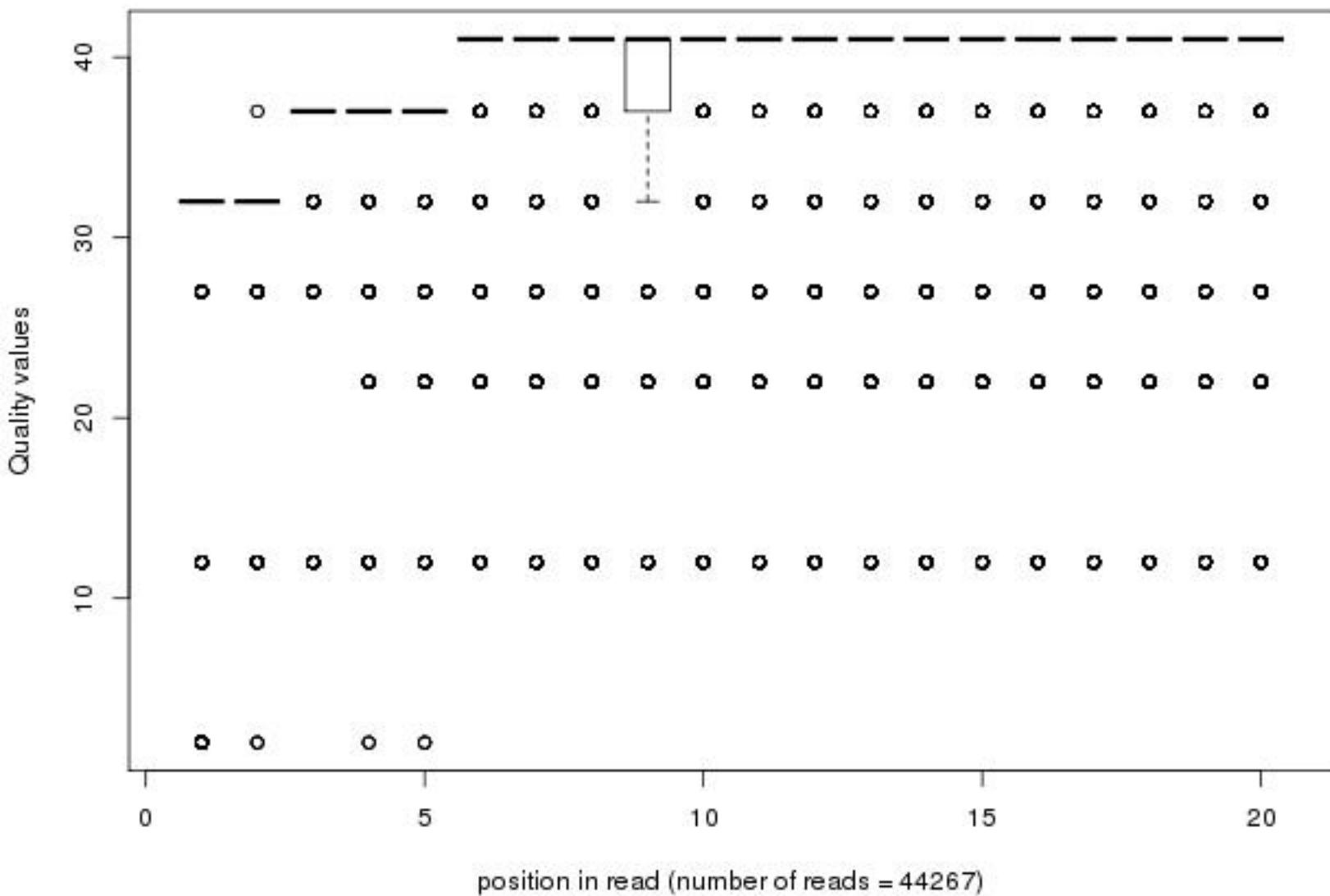
Quality distribution by position in read n2_wildtypexxx_sy002_01of20_1_frac50_first20
