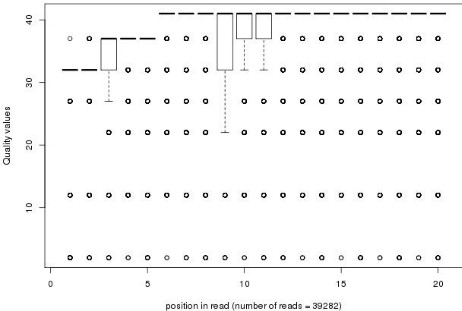
Quality distribution by position in read n2_unc73prp8fx_sy007_01of20_2_frac50_first20
