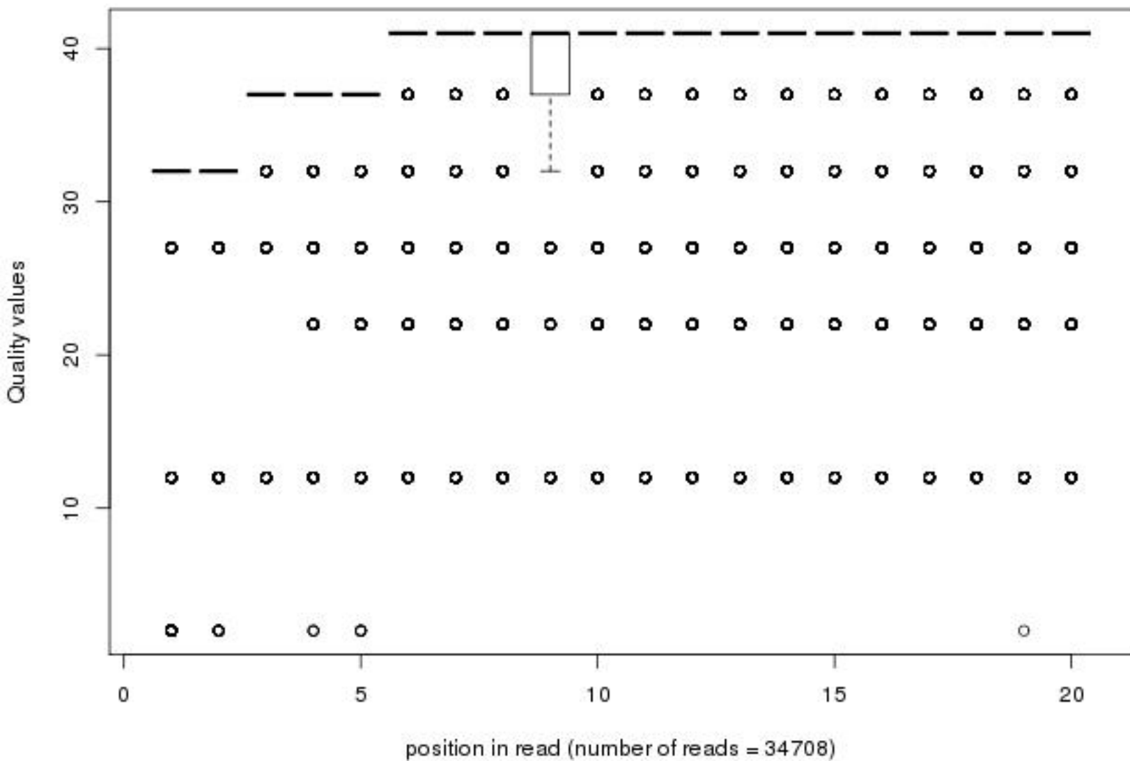
Quality distribution by position in read n2_unc73dxbp1x_sy012_01of20_1_frac50_first20
