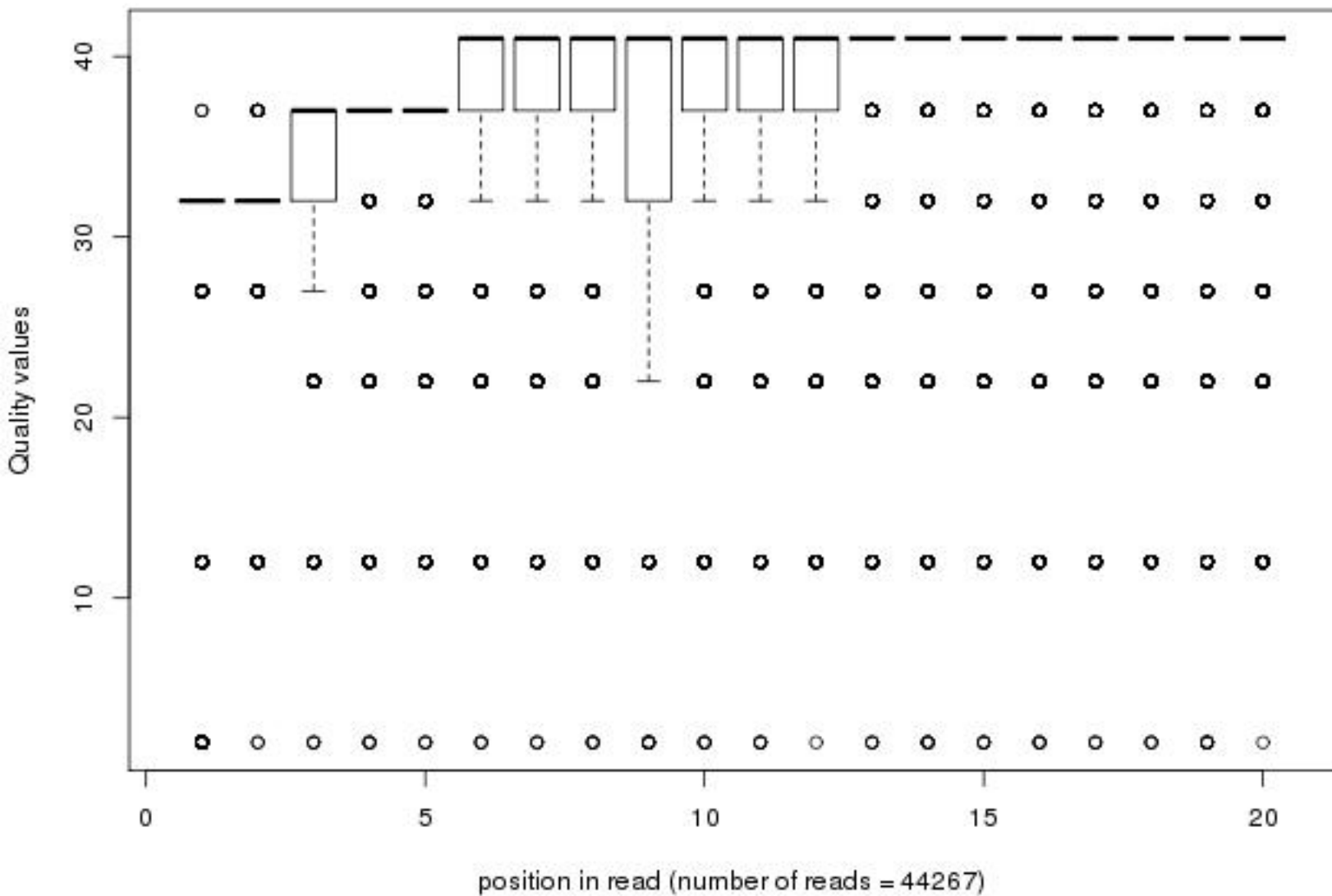
Quality distribution by position in read n2_wildtypexxx_sy002_01of20_2_frac50_first20
