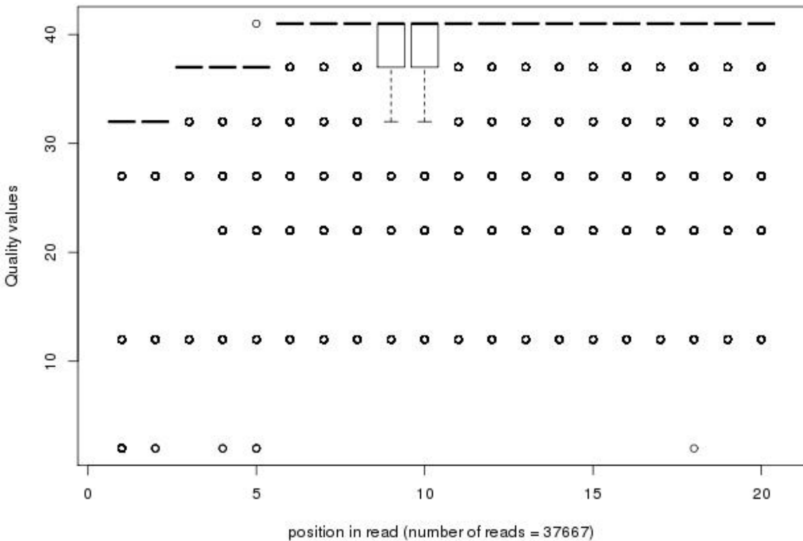
Quality distribution by position in read n2_unc73out2xx_sy016_01of20_1_frac50_first20
