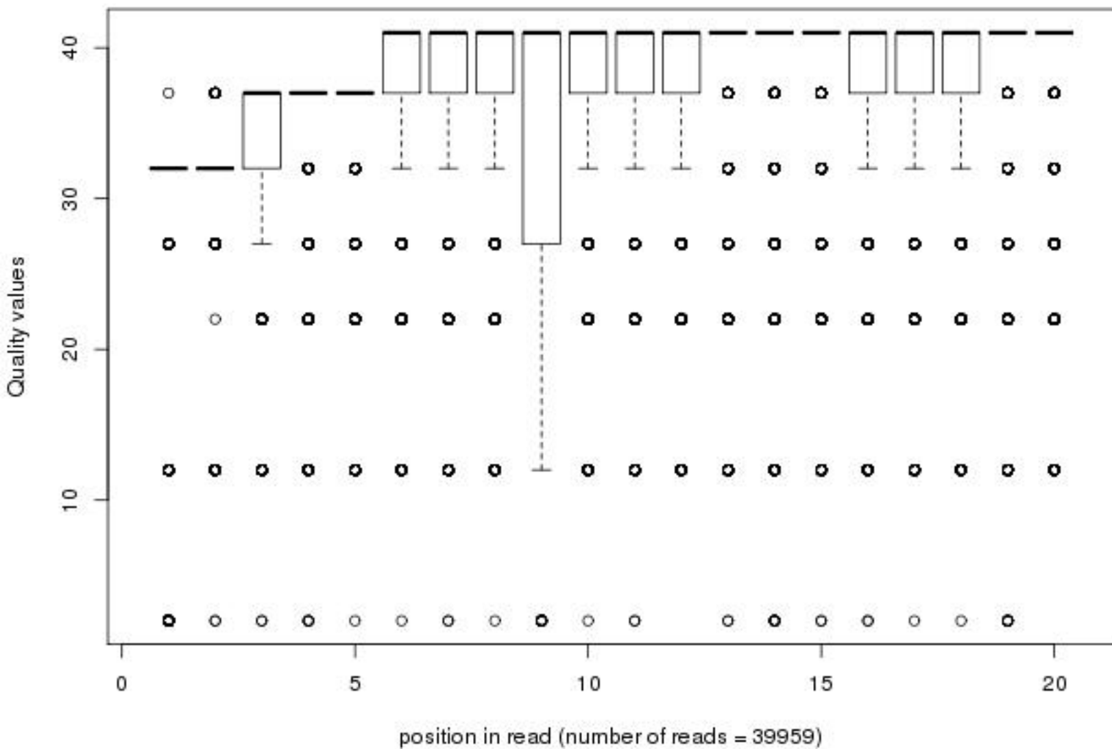
Quality distribution by position in read n2_unc73prp8eo_sy006_01of20_2_frac50_first20
