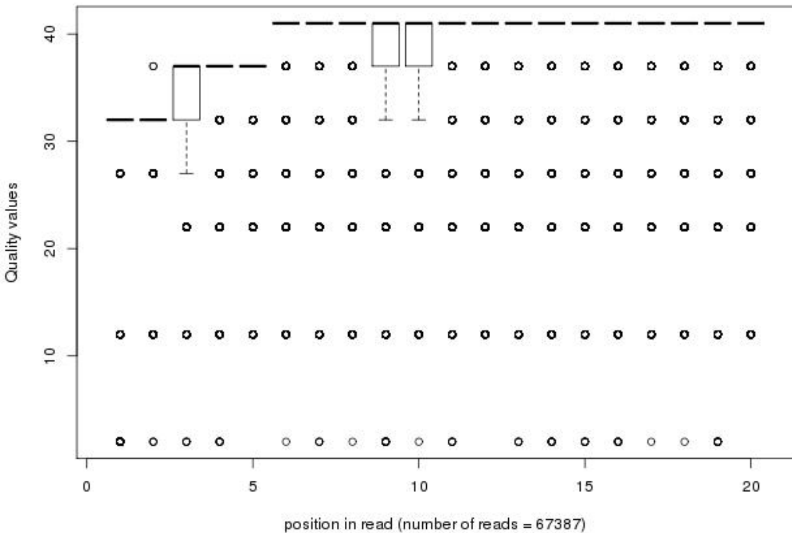
Quality distribution by position in read n2_unc73prp8ex_sy014_01of20_2_frac50_first20
