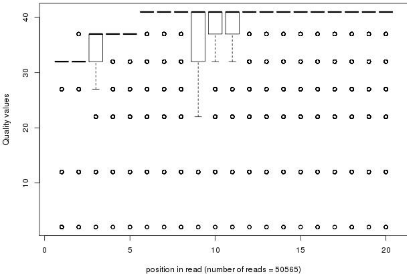
Quality distribution by position in read n2_unc73dxbp1x_sy011_01of20_2_frac50_first20
