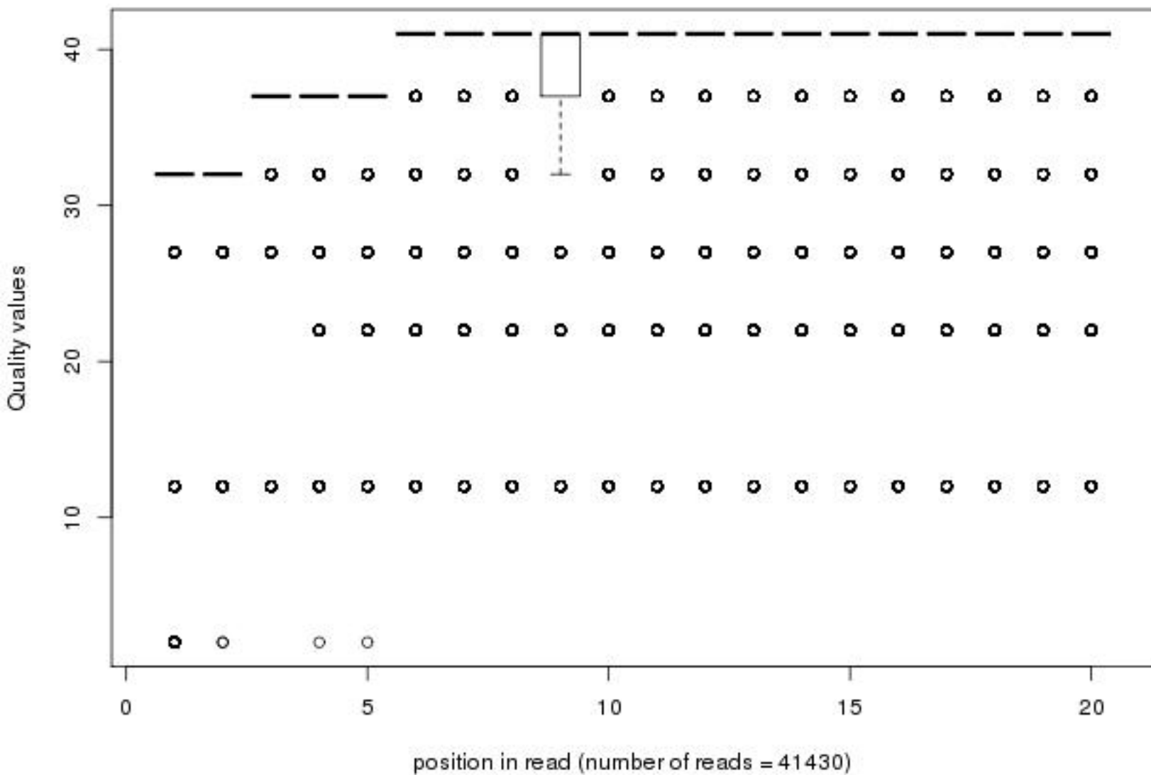
Quality distribution by position in read n2_dxbp1onlyxx_sy009_01of20_1_frac50_first20
