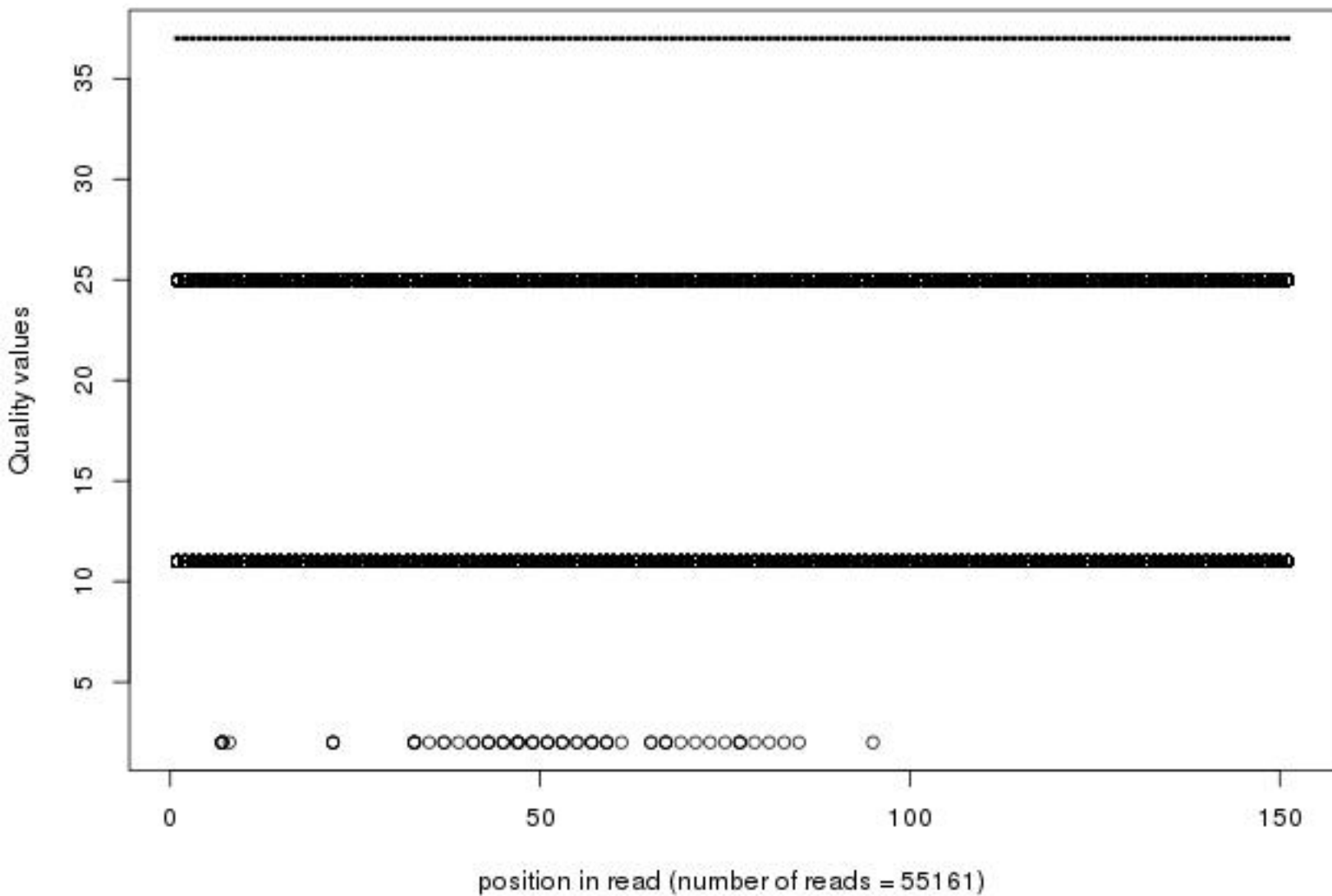
Quality distribution by position in read mmlin_wt_dr301_01of10_2_frac100_pad151
