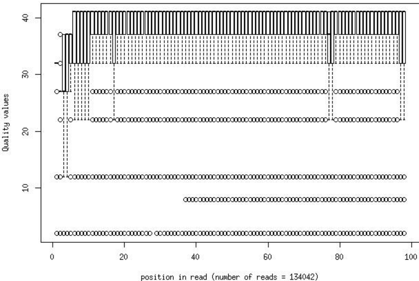
Quality distribution by position in read h9del158_wk02_gm113_bcode1of4_2_frac100
