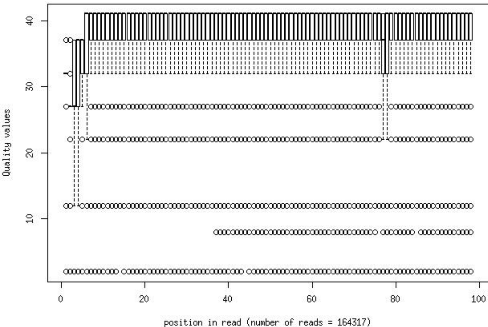
Quality distribution by position in read h9del137_wk04_gm120_bcode1of4_2_frac100
