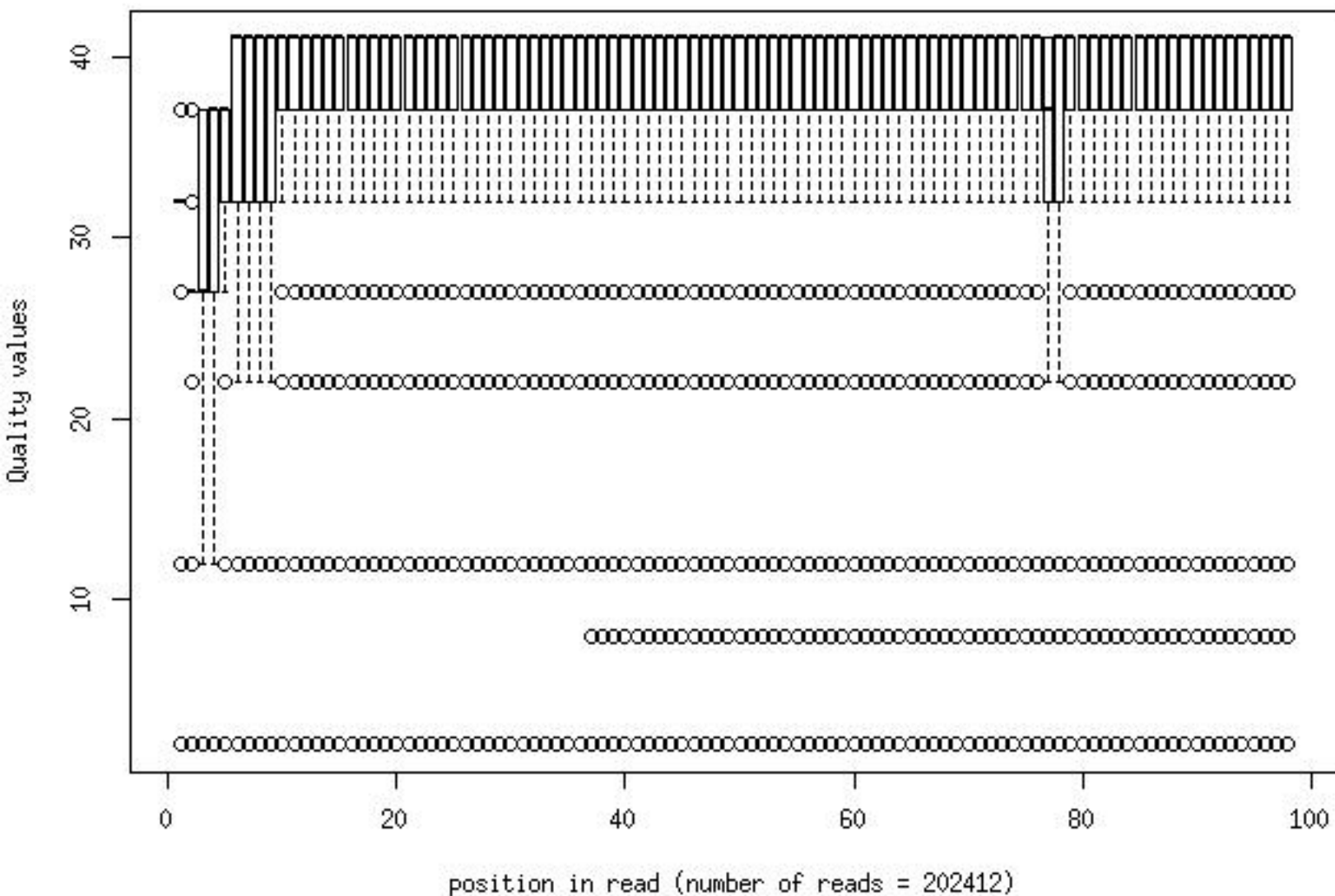
Quality distribution by position in read h9del137_wk02_gm111_bcode1of4_2_frac100
