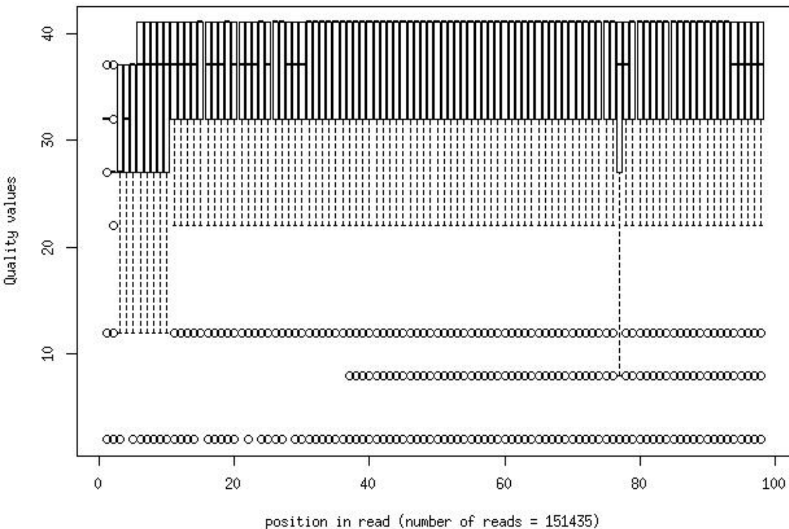
Quality distribution by position in read hesc2wt_wk02_gm117_bcode1of4_2_frac100
