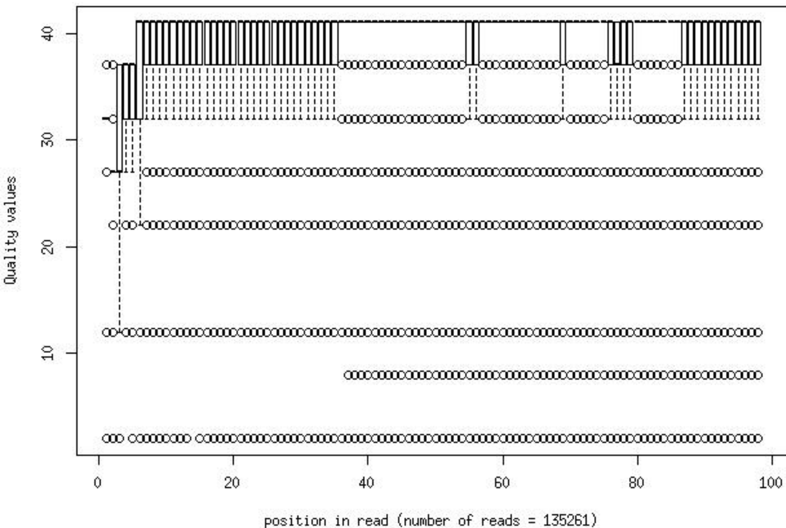
Quality distribution by position in read hesc2wt_wk02_gm118_bcode1of4_2_frac100
