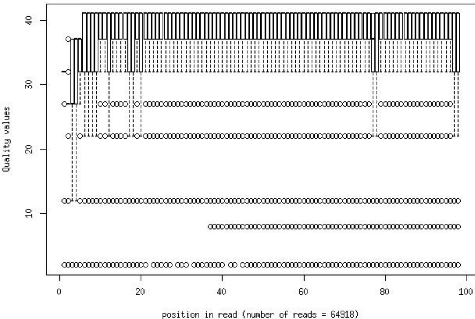
Quality distribution by position in read h9del158_wk04_gm121_bcode1of4_2_frac100
