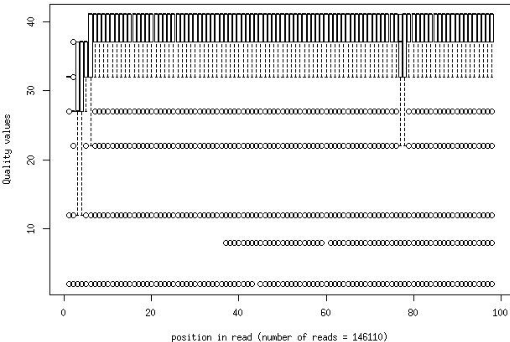
Quality distribution by position in read h9del170_wk04_gm124_bcode1of4_2_frac100
