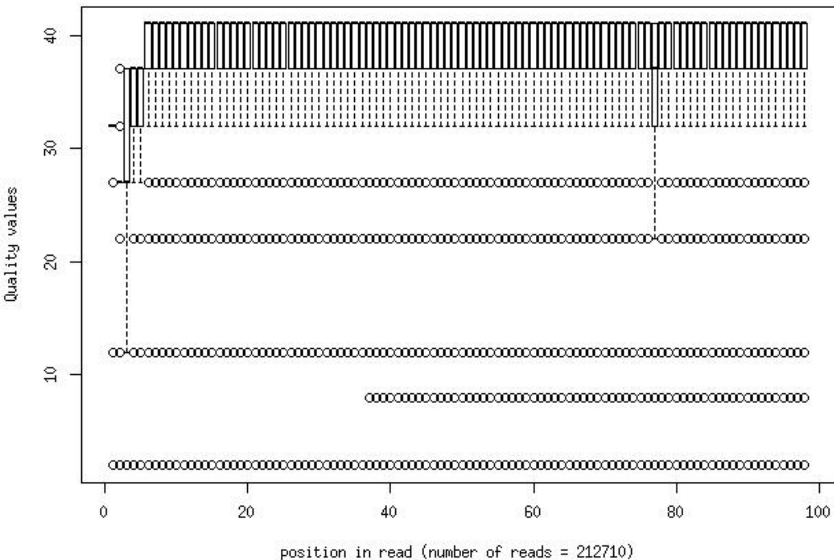
Quality distribution by position in read hesc2wt_wk04_gm126_bcode1of4_2_frac100
