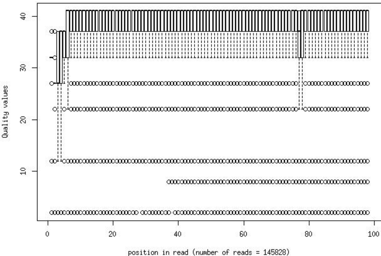
Quality distribution by position in read h9del170_wk04_gm123_bcode1of4_2_frac100
