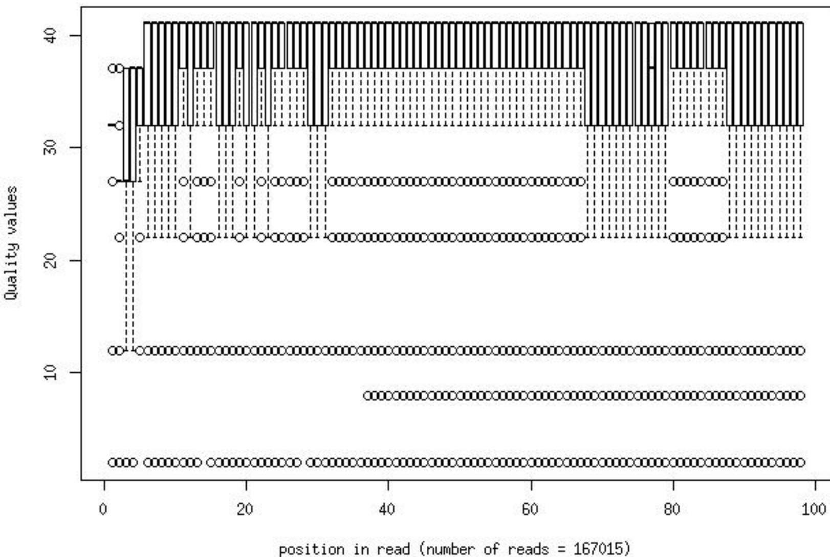
Quality distribution by position in read h9del170_wk02_gm116_bcode1of4_2_frac100
