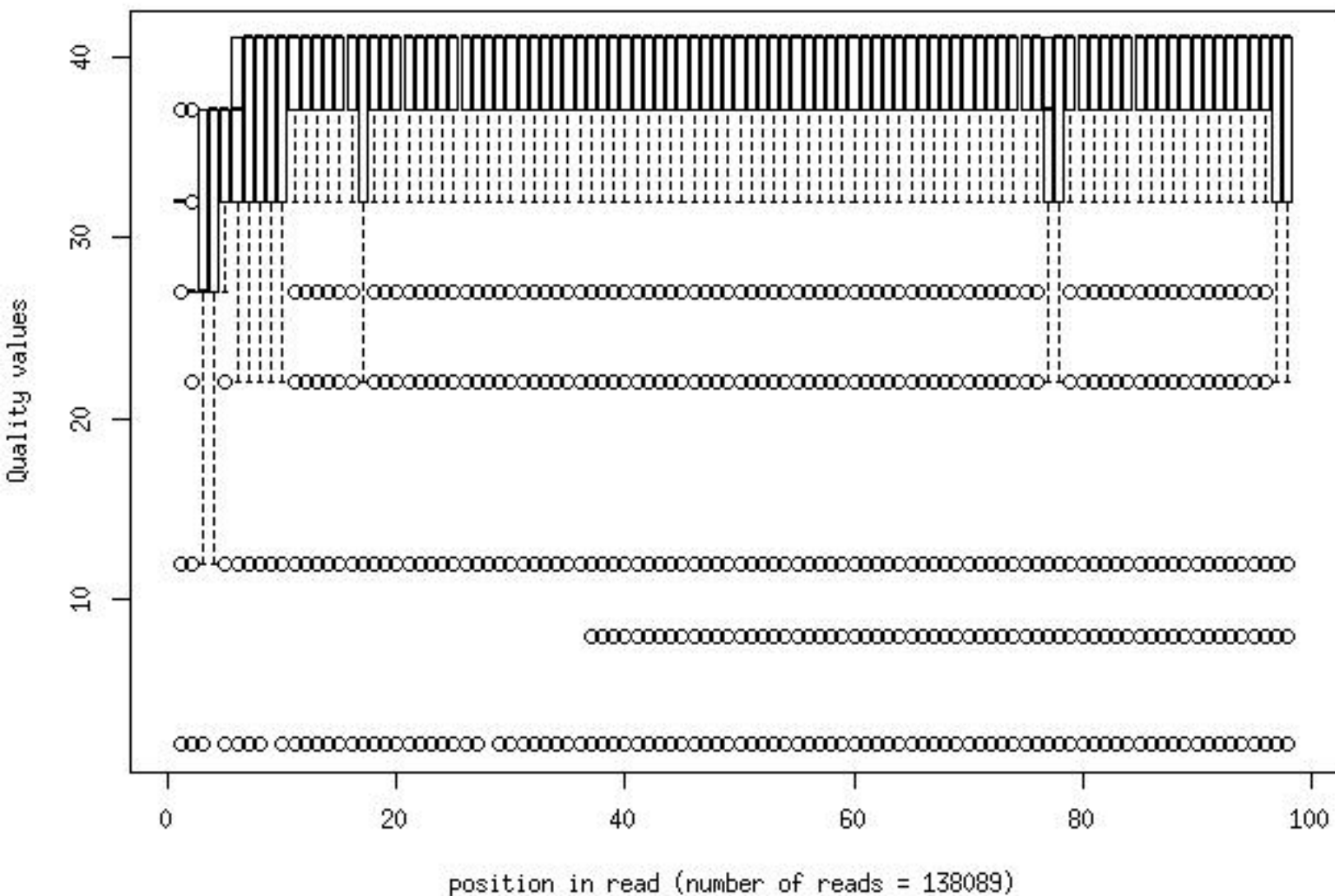
Quality distribution by position in read h9del137_wk02_gm112_bcode1of4_2_frac100
