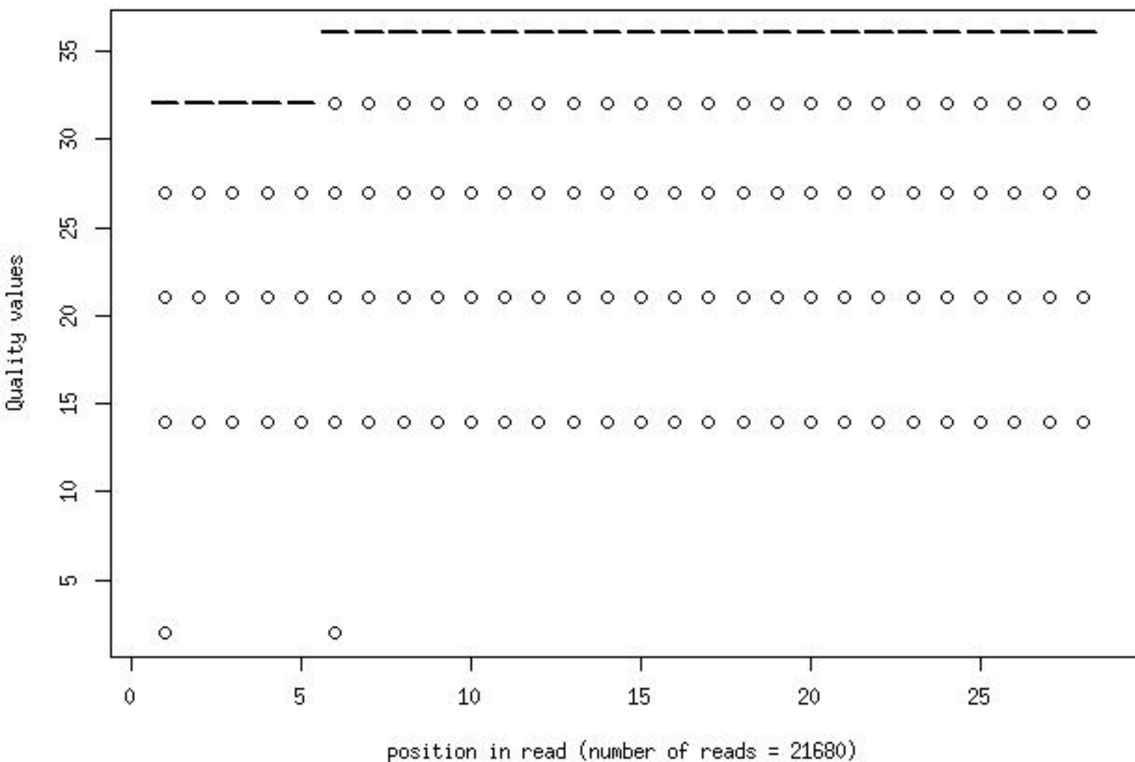
Quality distribution by position in read ms_msbc_gm171m3_1_frac100
