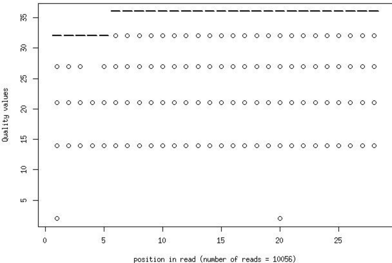
Quality distribution by position in read ms_msbc_gm173m3_1_frac100
