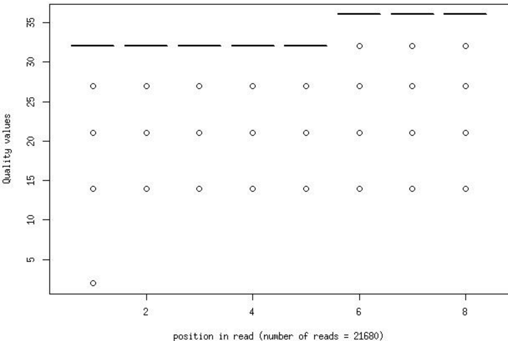
Quality distribution by position in read ms_msbc_gm171m3_2_frac100
