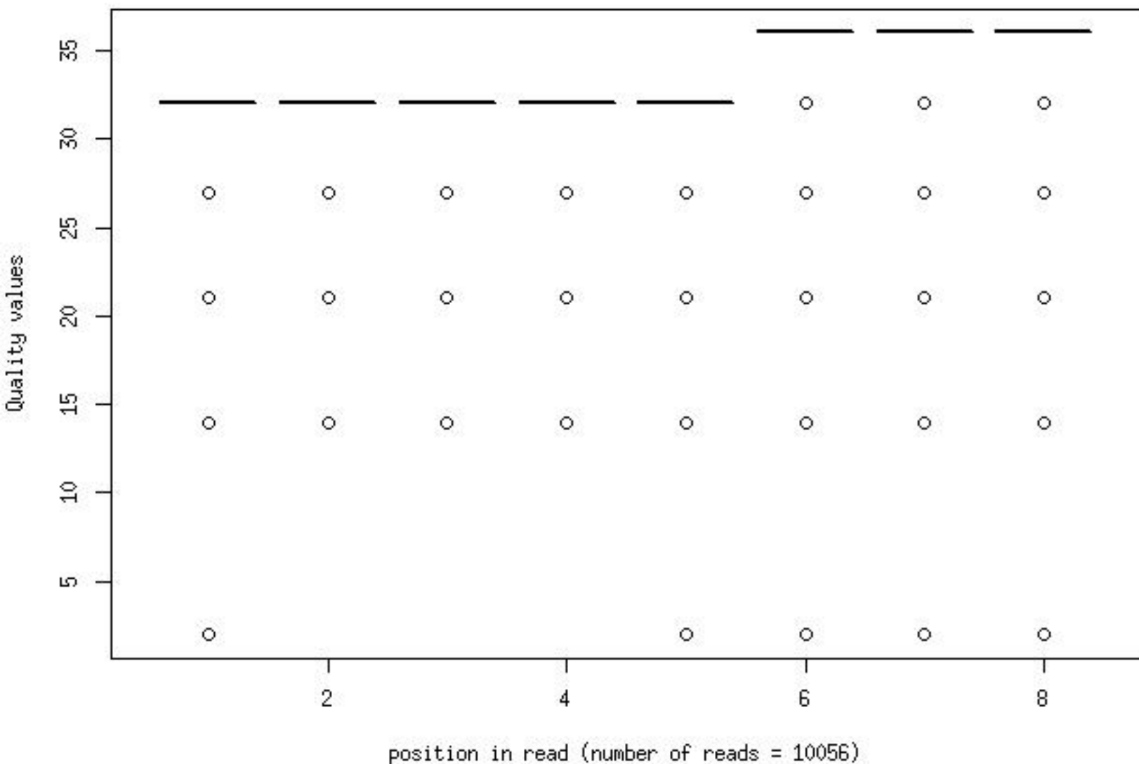
Quality distribution by position in read ms_msbc_gm173m3_2_frac100
