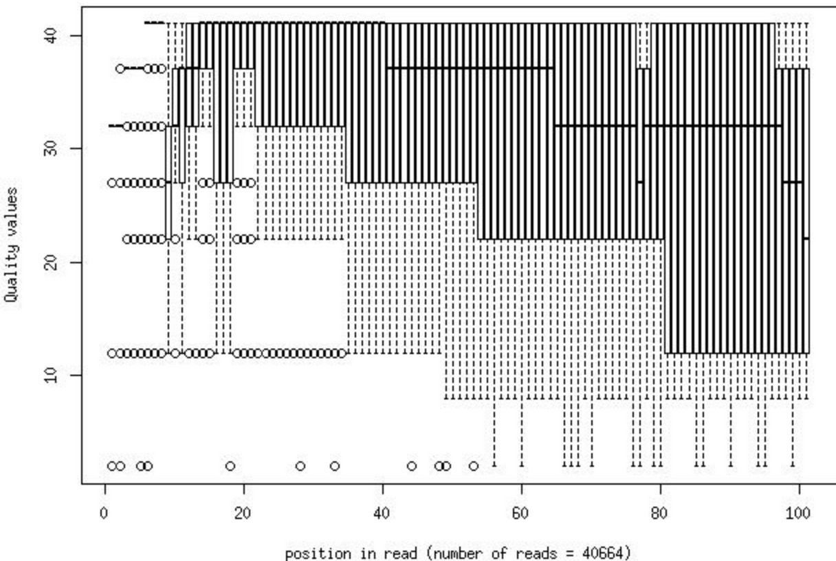
Quality distribution by position in read hips_765g2_ndx_pa006_1_frac1000
