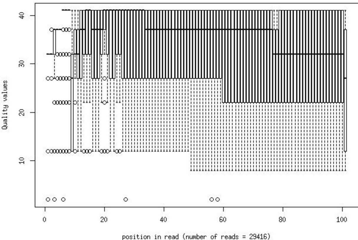
Quality distribution by position in read hips_ntcg7_dox_pa007_1_frac1000
