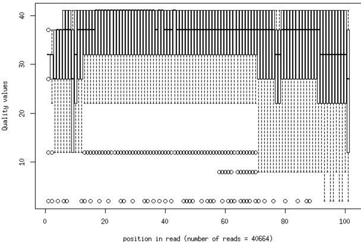
Quality distribution by position in read hips_765g2_ndx_pa006_2_frac1000
