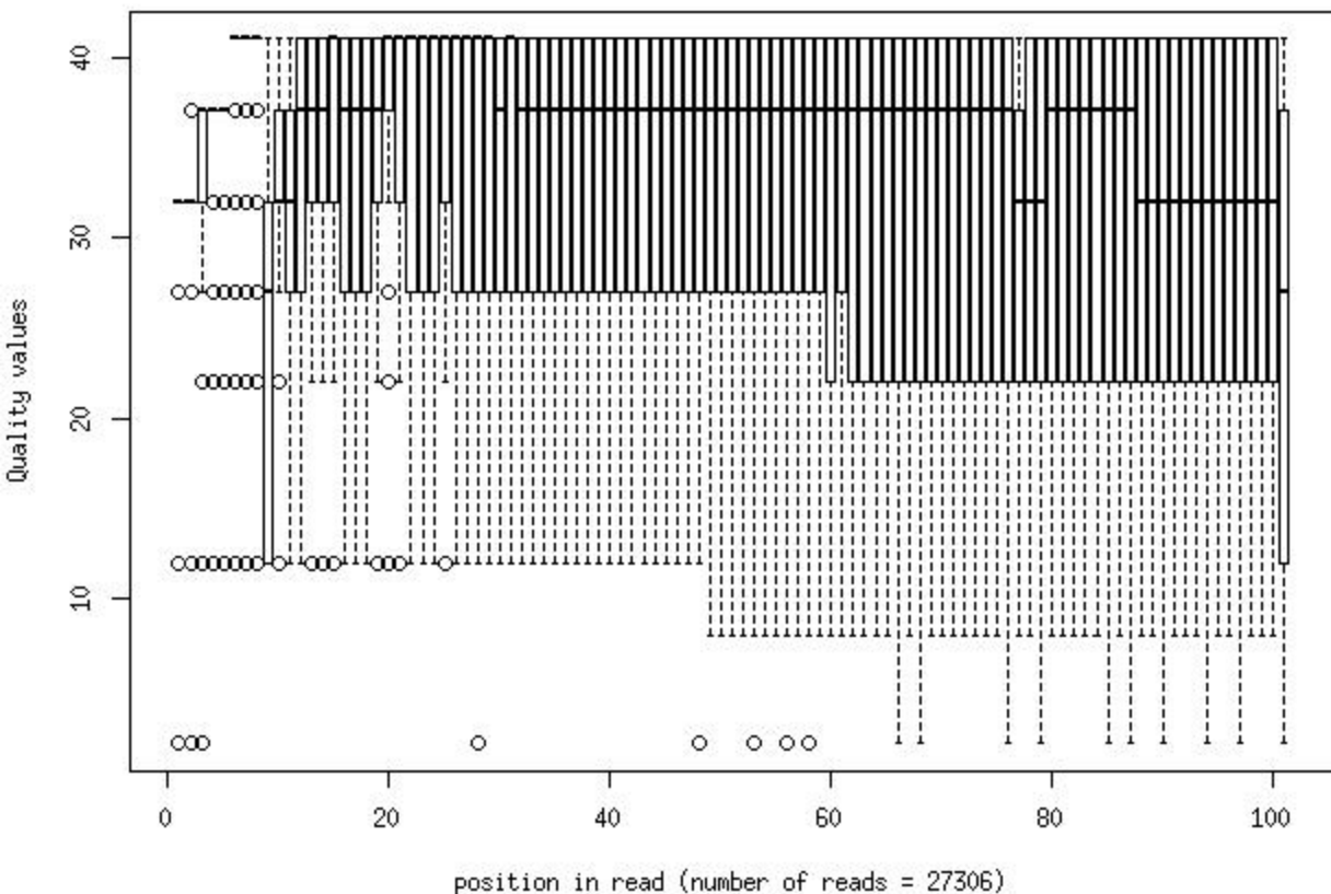
Quality distribution by position in read hips_ntcg7_dox_pa008_1_frac1000
