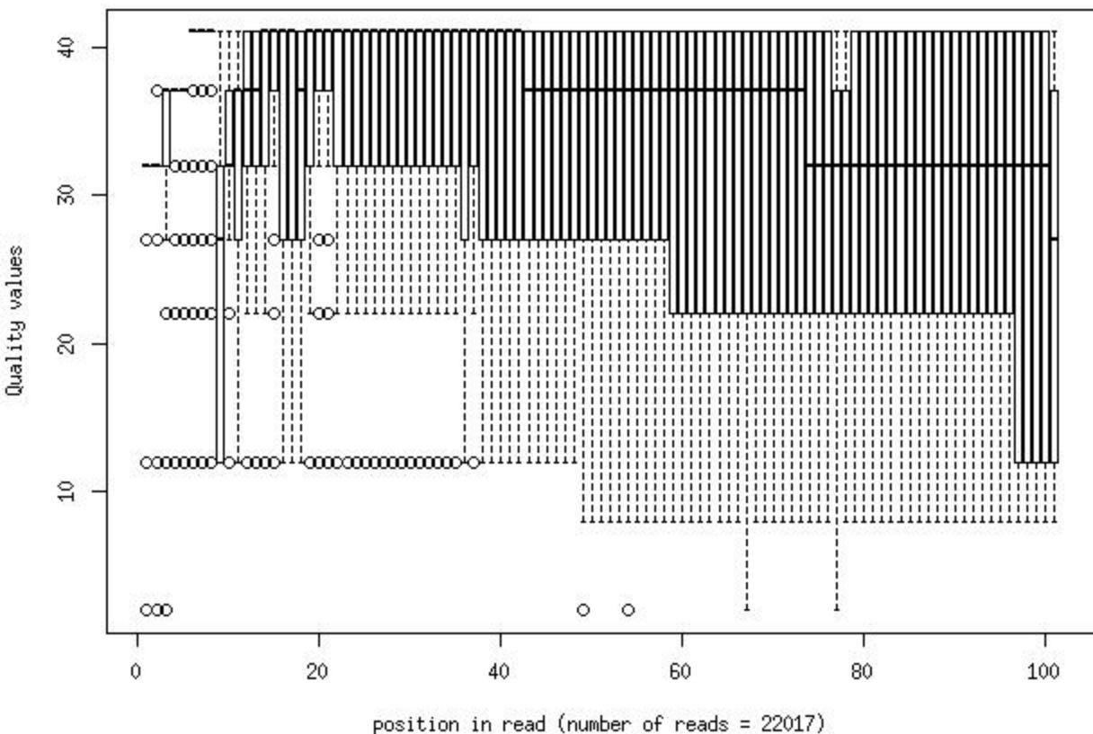
Quality distribution by position in read hips_765g2_ndx_pa005_1_frac1000
