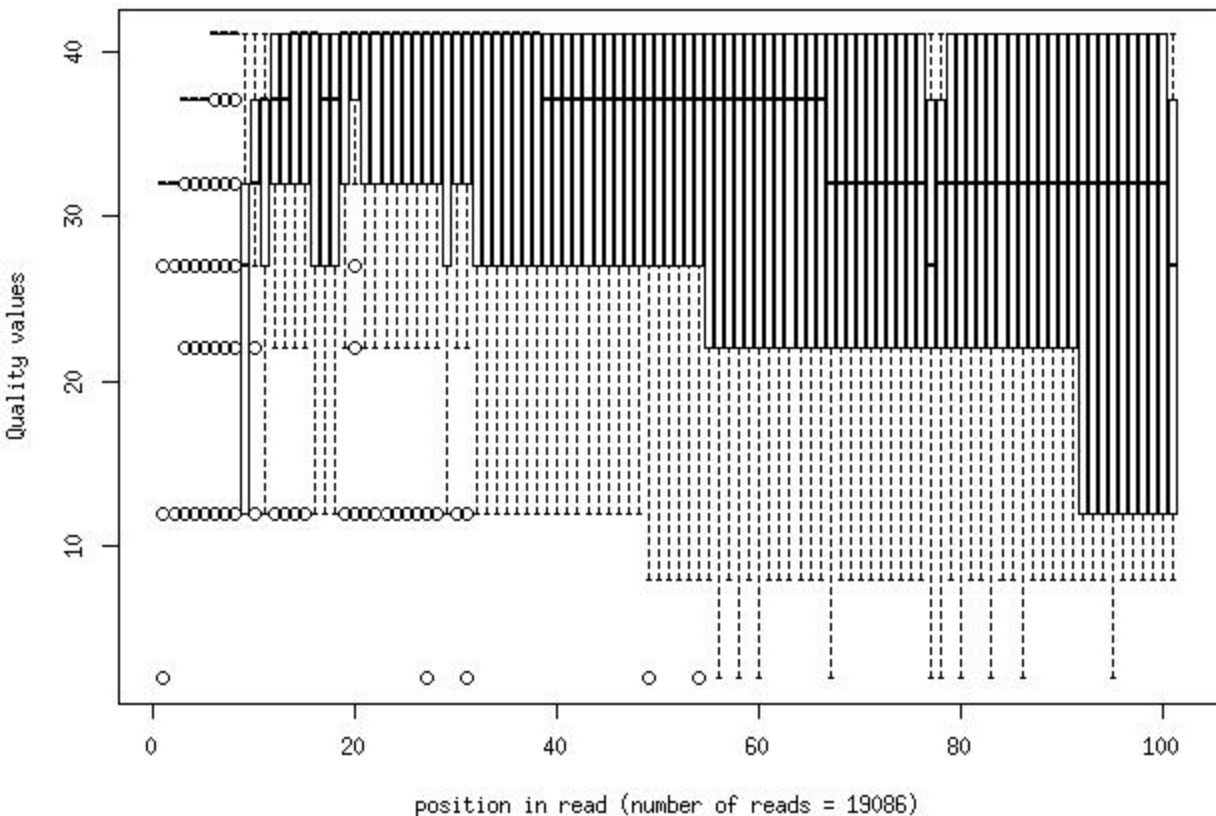
Quality distribution by position in read hips_ntcg7_ndx_pa004_1_frac1000
