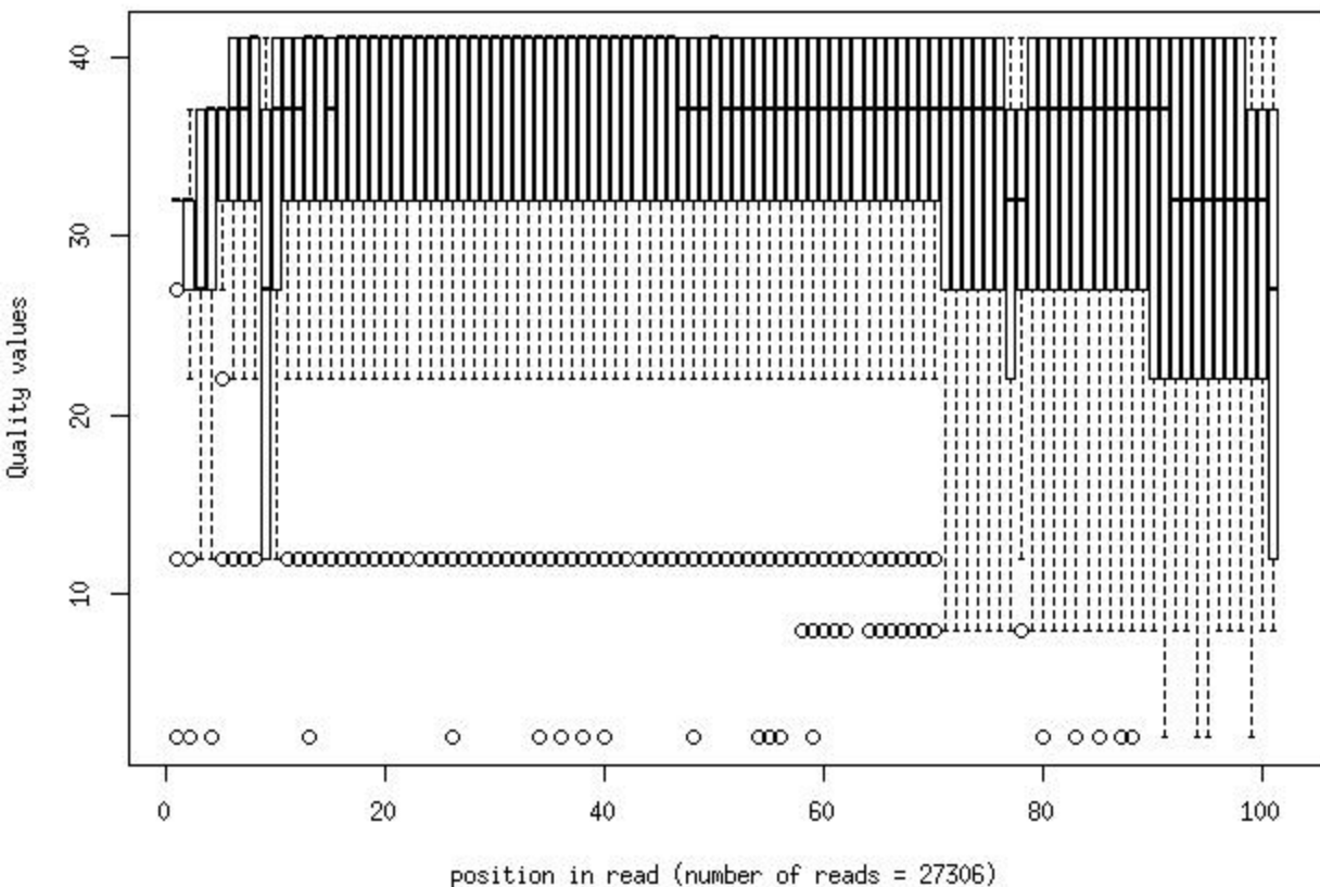
Quality distribution by position in read hips_ntcg7_dox_pa008_2_frac1000
