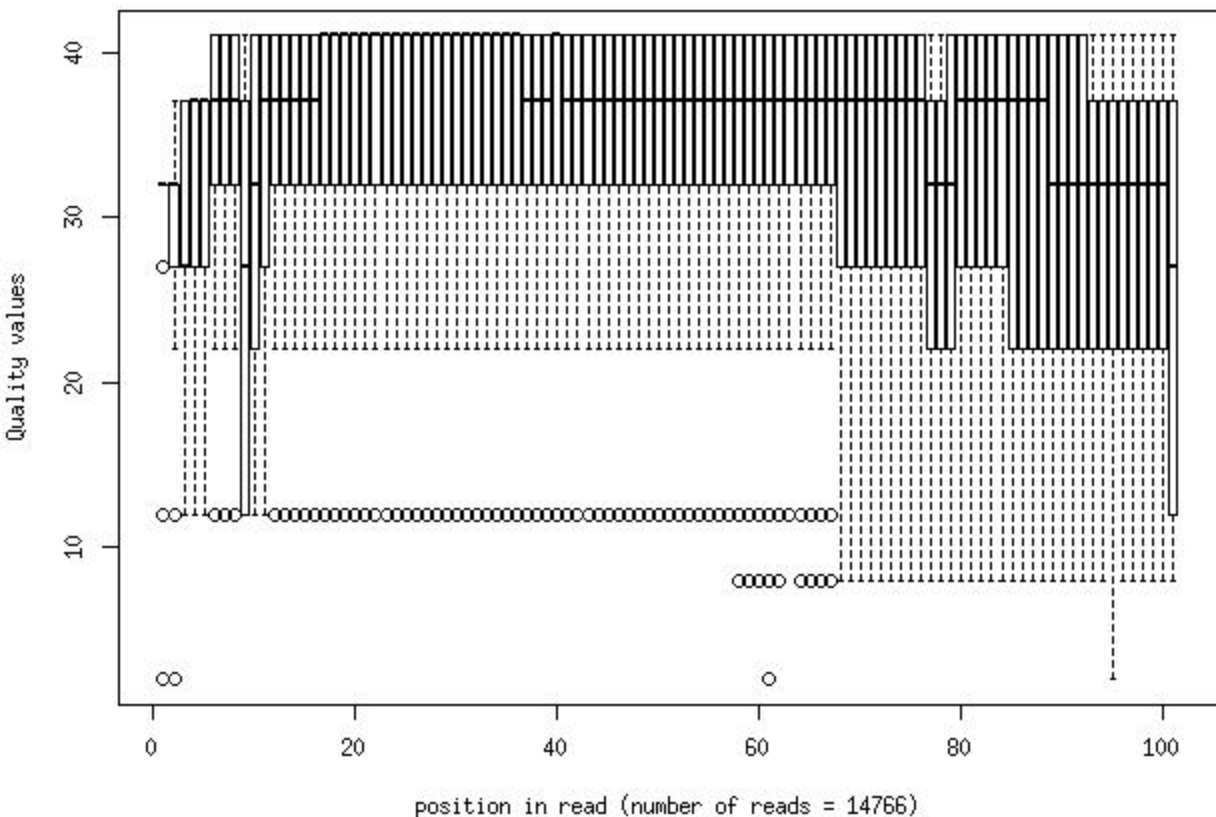
Quality distribution by position in read hips_765g2_dox_pa009_2_frac100
