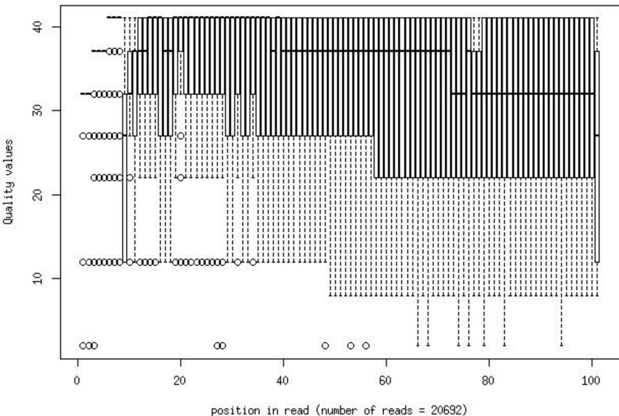
Quality distribution by position in read hips_765g2_dox_pa010_1_frac1000
