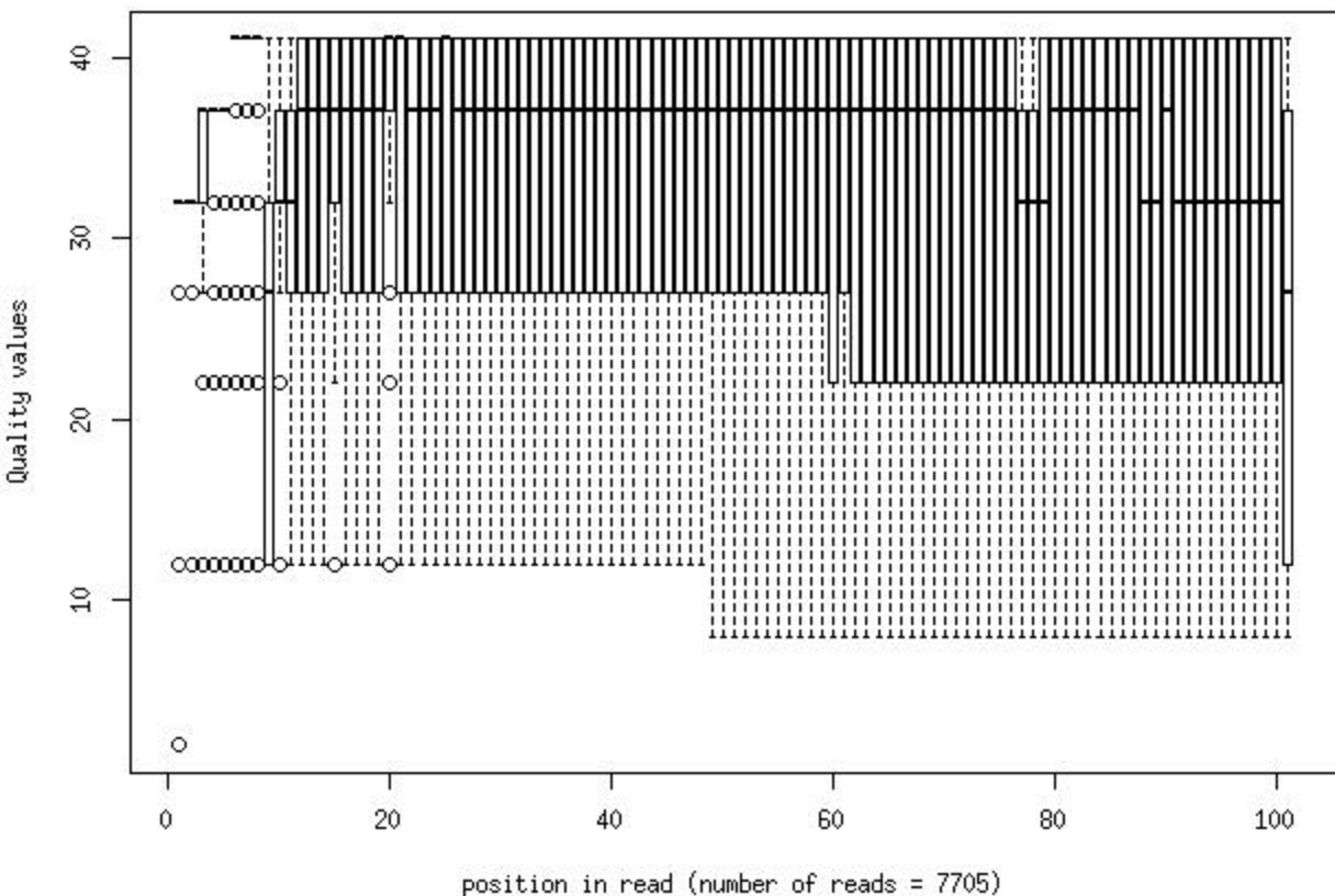
Quality distribution by position in read hips_ntcg7_ndx_pa003_1_frac1000
