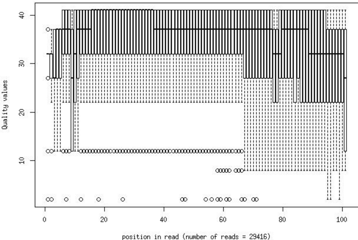
Quality distribution by position in read hips_ntcg7_dox_pa007_2_frac1000
