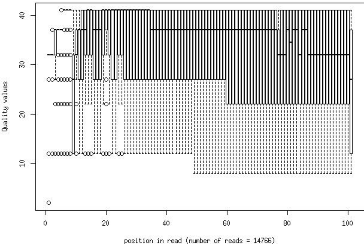
Quality distribution by position in read hips_765g2_dox_pa009_1_frac1000
