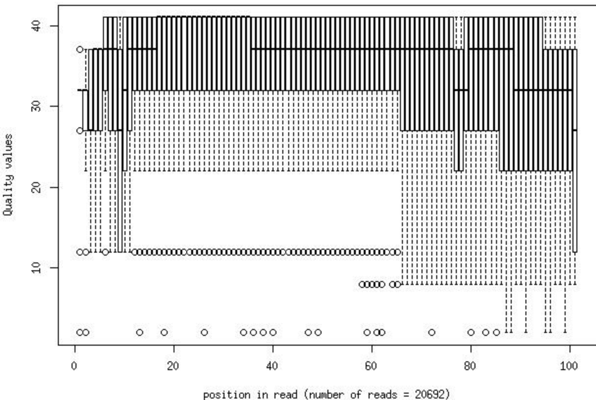
Quality distribution by position in read hips_765g2_dox_pa010_2_frac100
