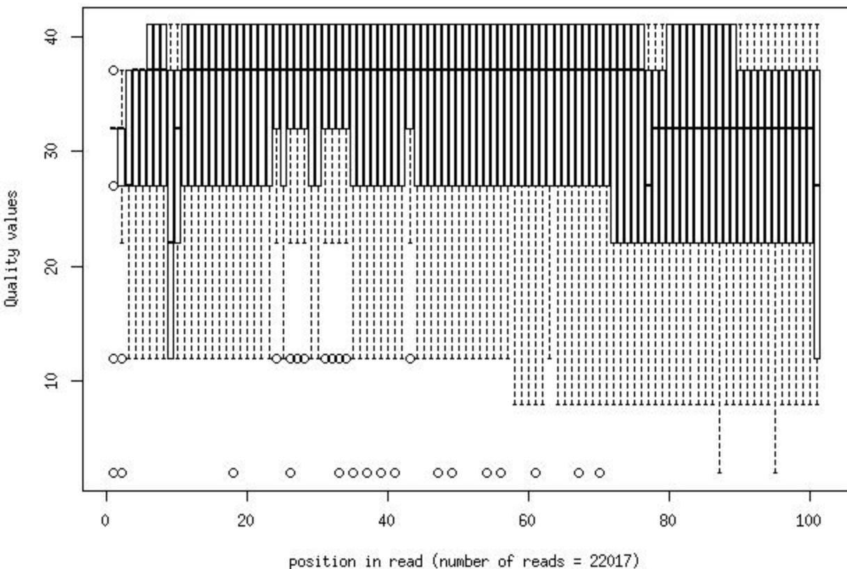
Quality distribution by position in read hips_765g2_ndx_pa005_2_frac1000
