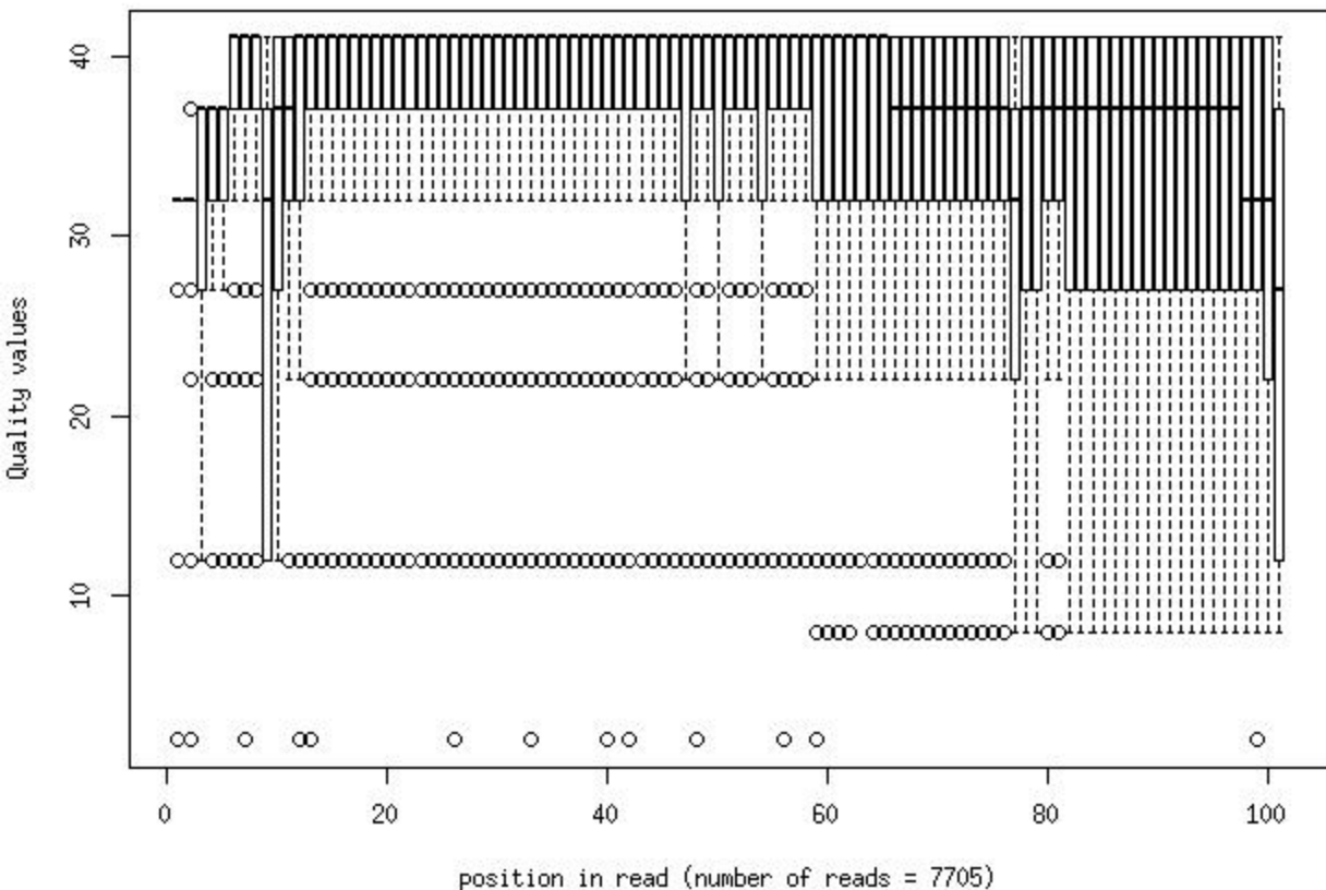
Quality distribution by position in read hips_ntcg7_ndx_pa003_2_frac1000
