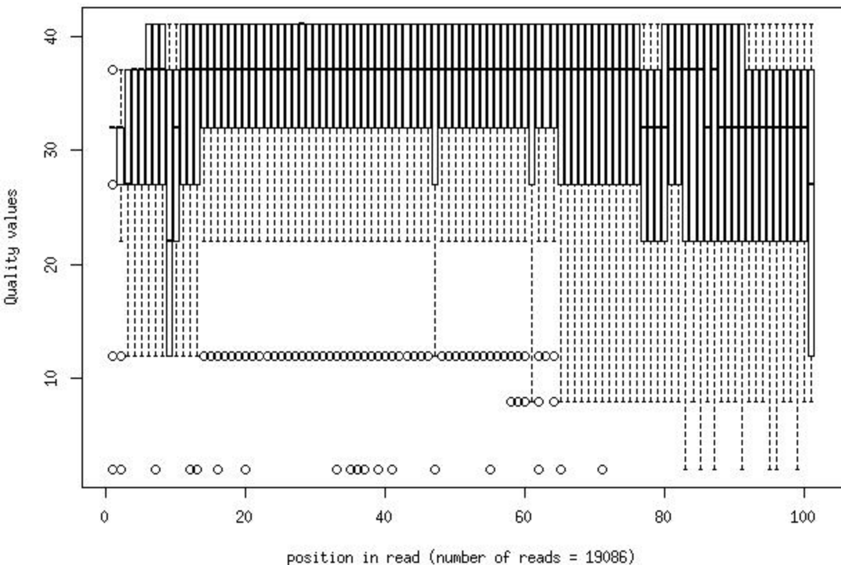
Quality distribution by position in read hips_ntcg7_ndx_pa004_2_frac1000
