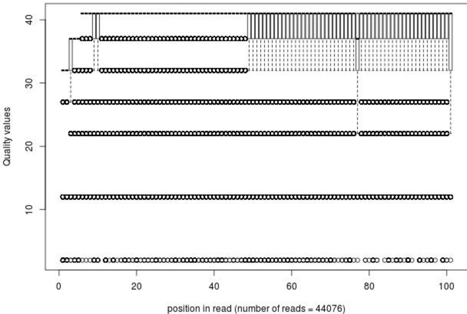
Quality distribution by position in read hips_prime_jf085_01of10_2_frac100
