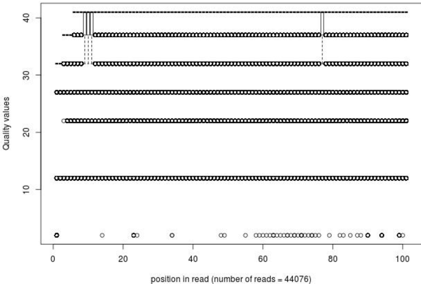
Quality distribution by position in read hips_prime_jf085_01of10_1_frac100
