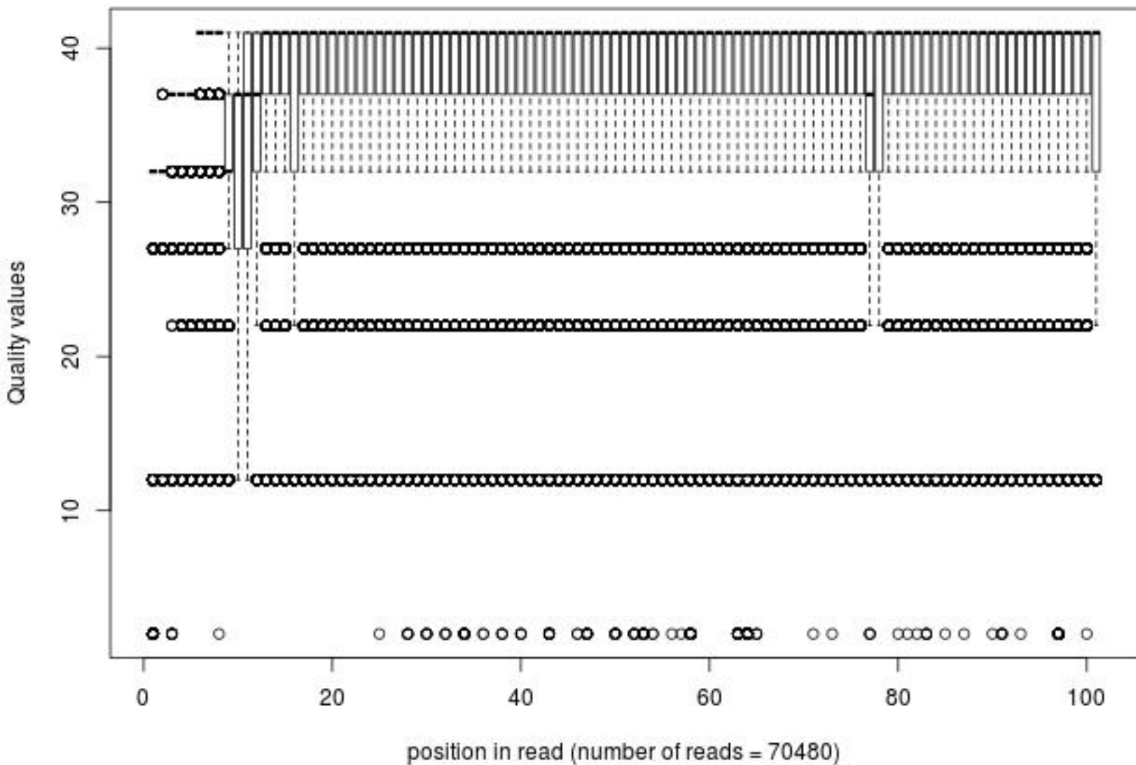
Quality distribution by position in read hips_naive_jf089_01of10_1_frac100
