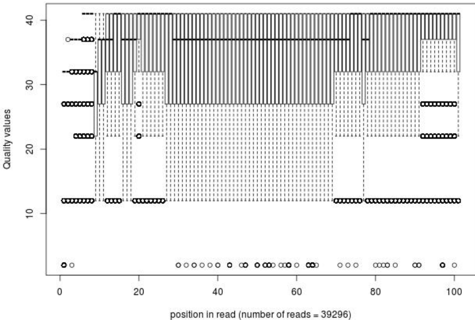
Quality distribution by position in read hips_naive_jf088_01of10_1_frac100
