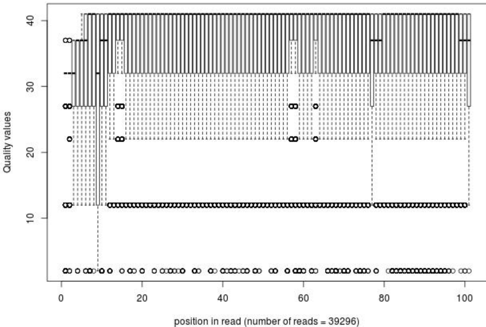
Quality distribution by position in read hips_naive_jf088_01of10_2_frac100
