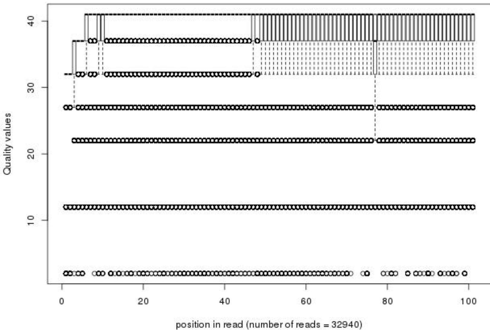
Quality distribution by position in read hips_prime_jf084_01of10_2_frac100
