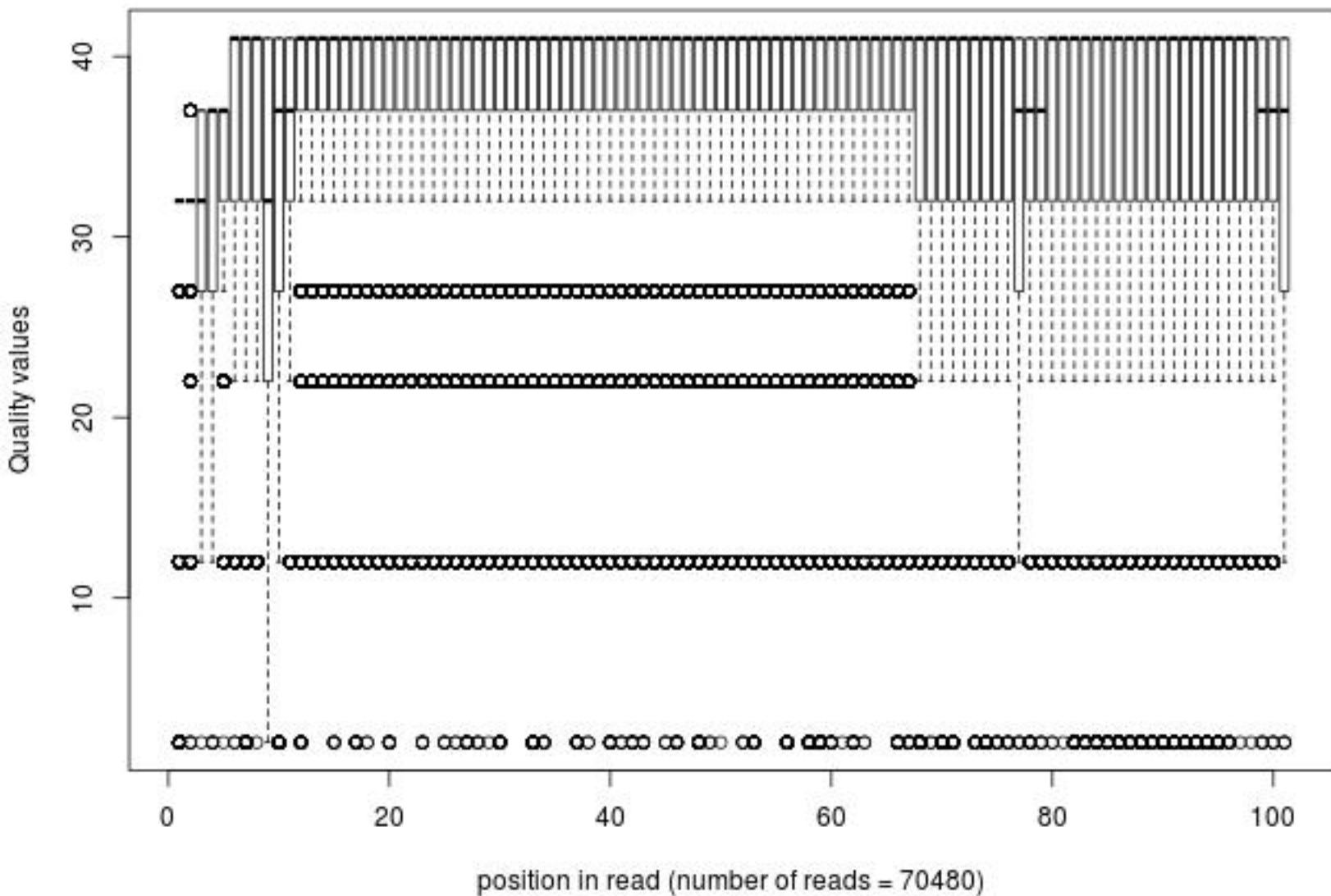
Quality distribution by position in read hips_naive_jf089_01of10_2_frac100
