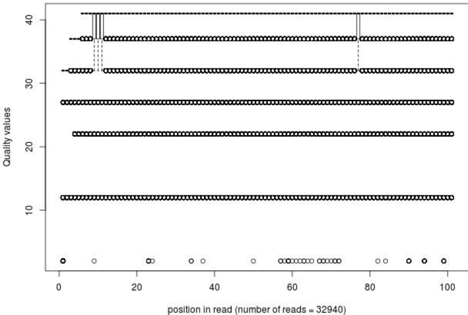
Quality distribution by position in read hips_prime_jf084_01of10_1_frac100
