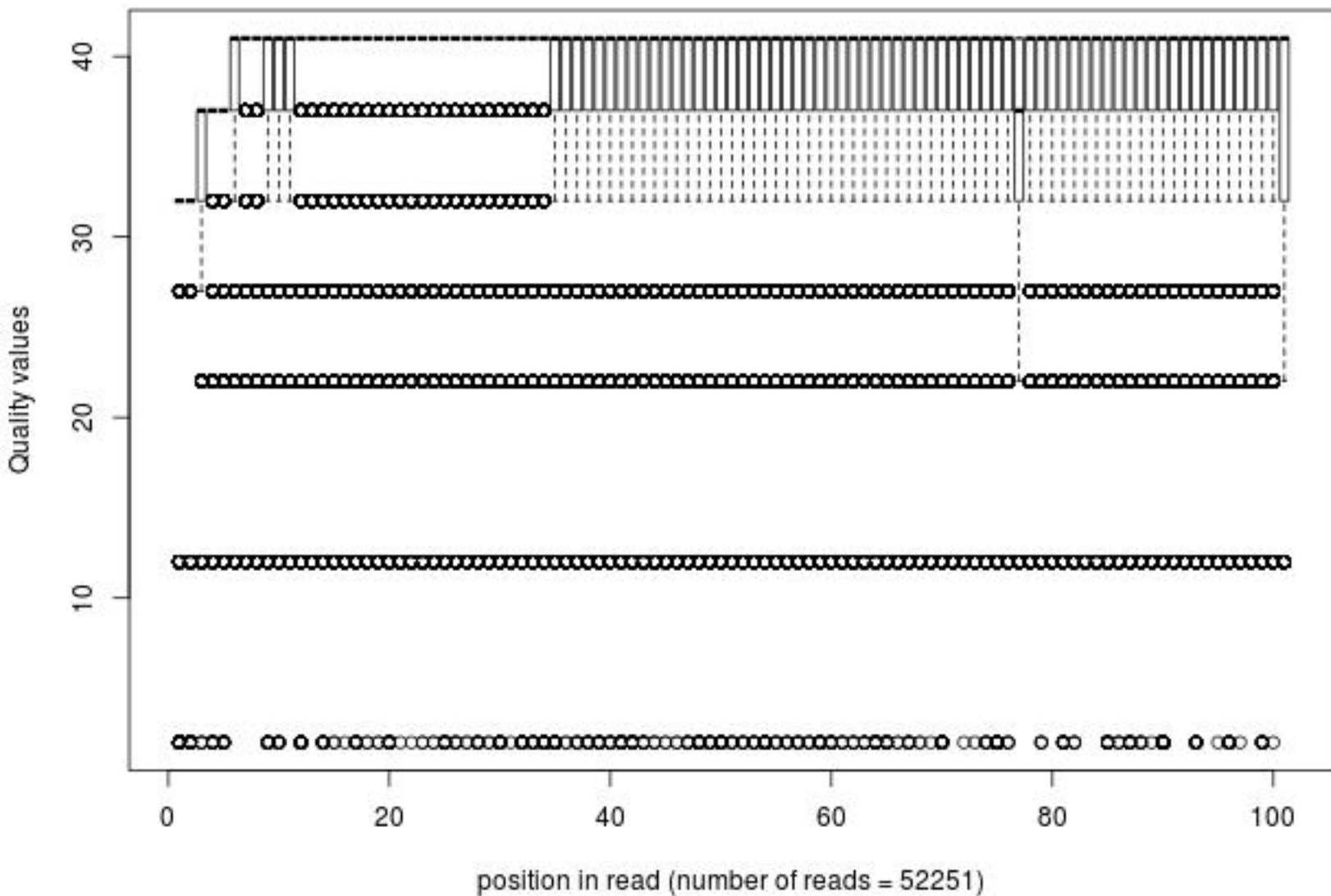
Quality distribution by position in read oips_prime_jf081_01of10_2_frac100
