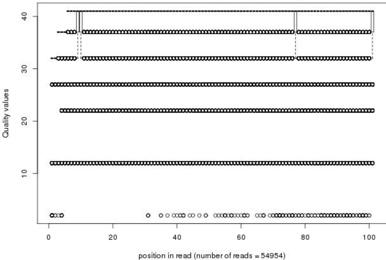
Quality distribution by position in read hek_trex4039_mo115_01of20_1_frac50
