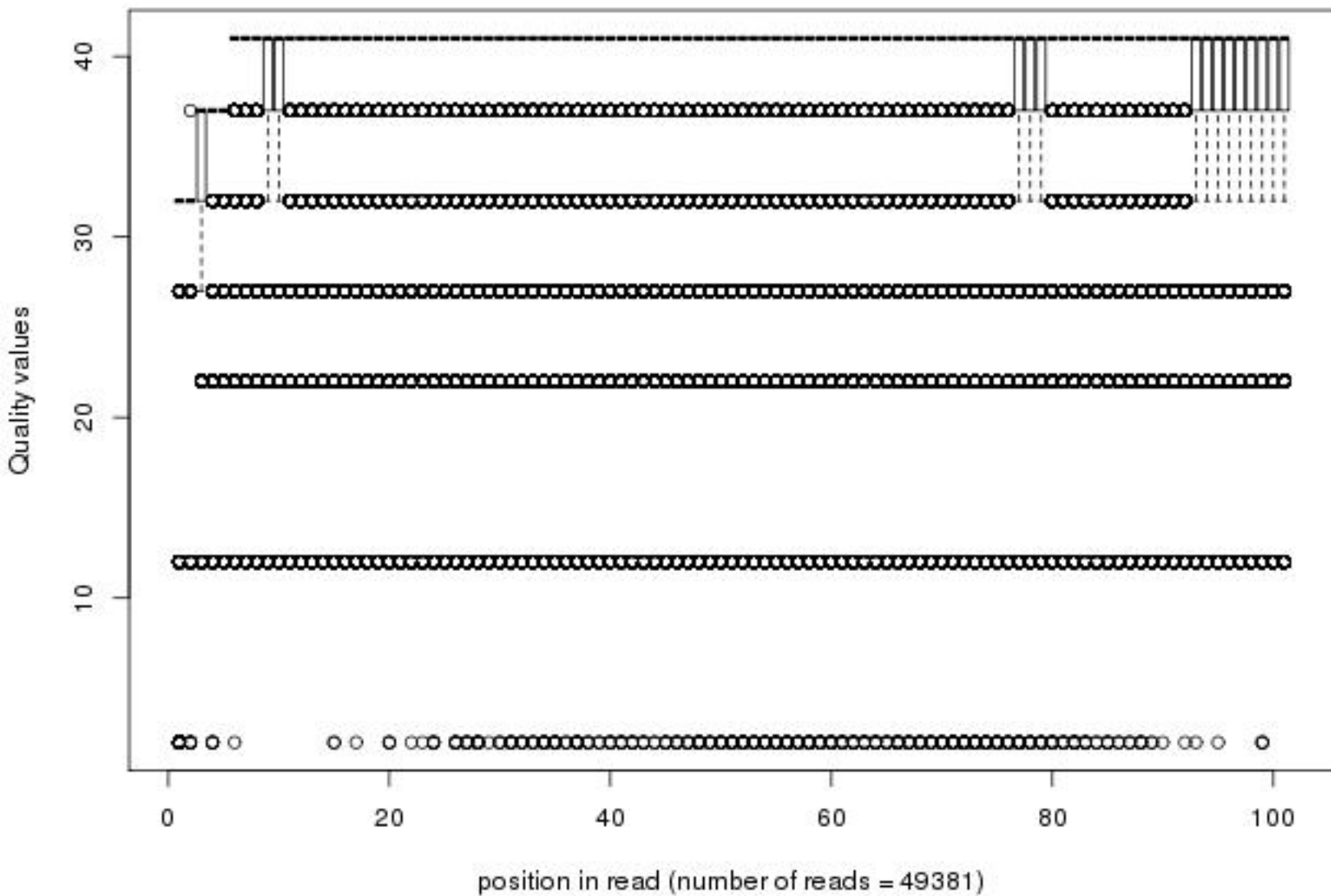
Quality distribution by position in read hek_trex5008_mo111_01of20_2_frac50
