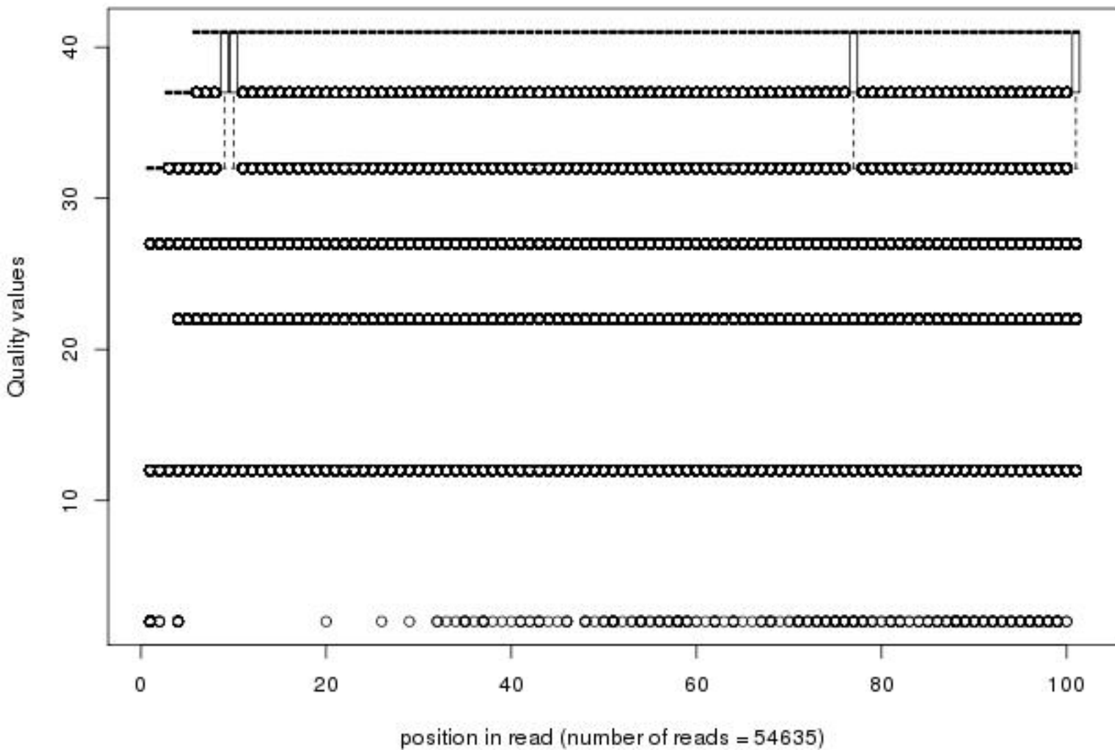
Quality distribution by position in read hek_trex0108_mo108_01of20_1_frac50
