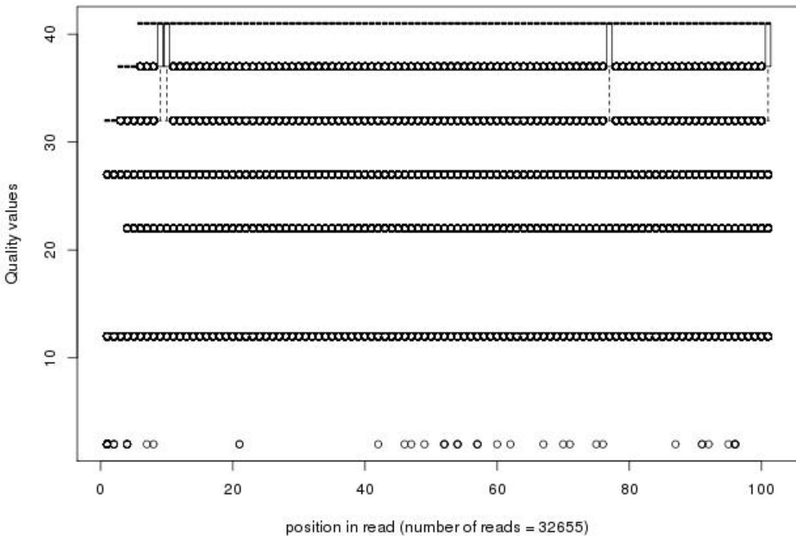
Quality distribution by position in read h9_prime_jf014_01of40_1_frac50
