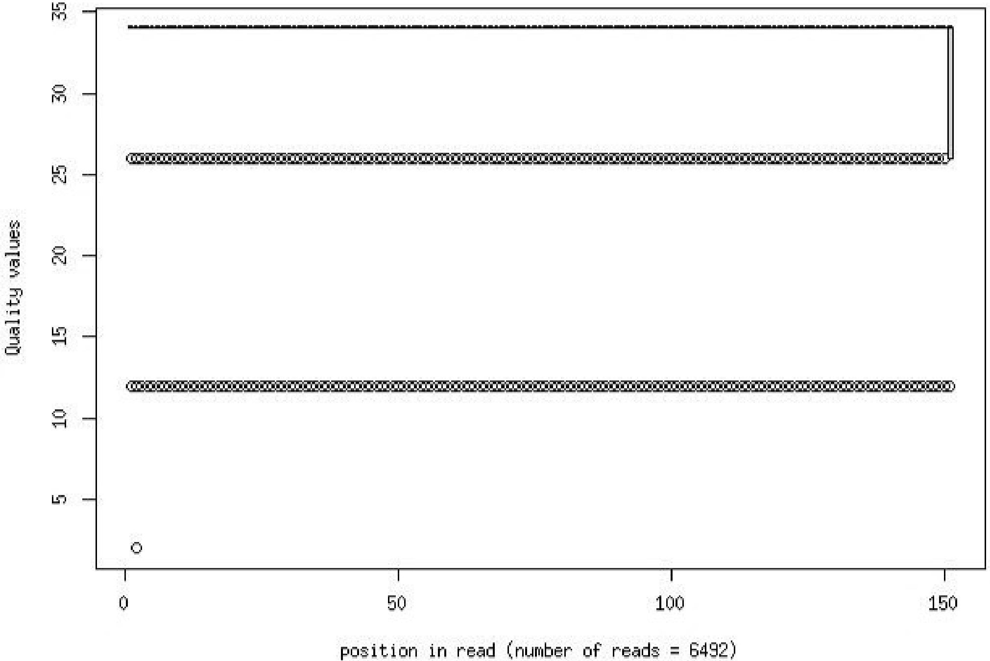
Quality distribution by position in read h9corg_ccult_qb002_1_frac1000
