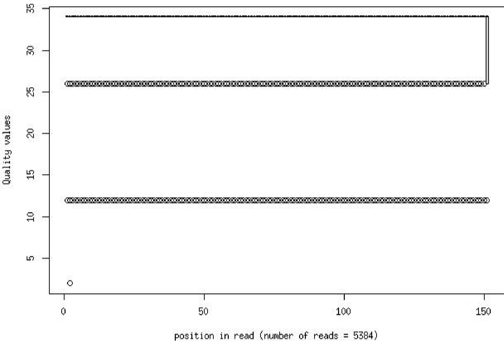
Quality distribution by position in read h9scorg_alone_qb004_1_frac1000
