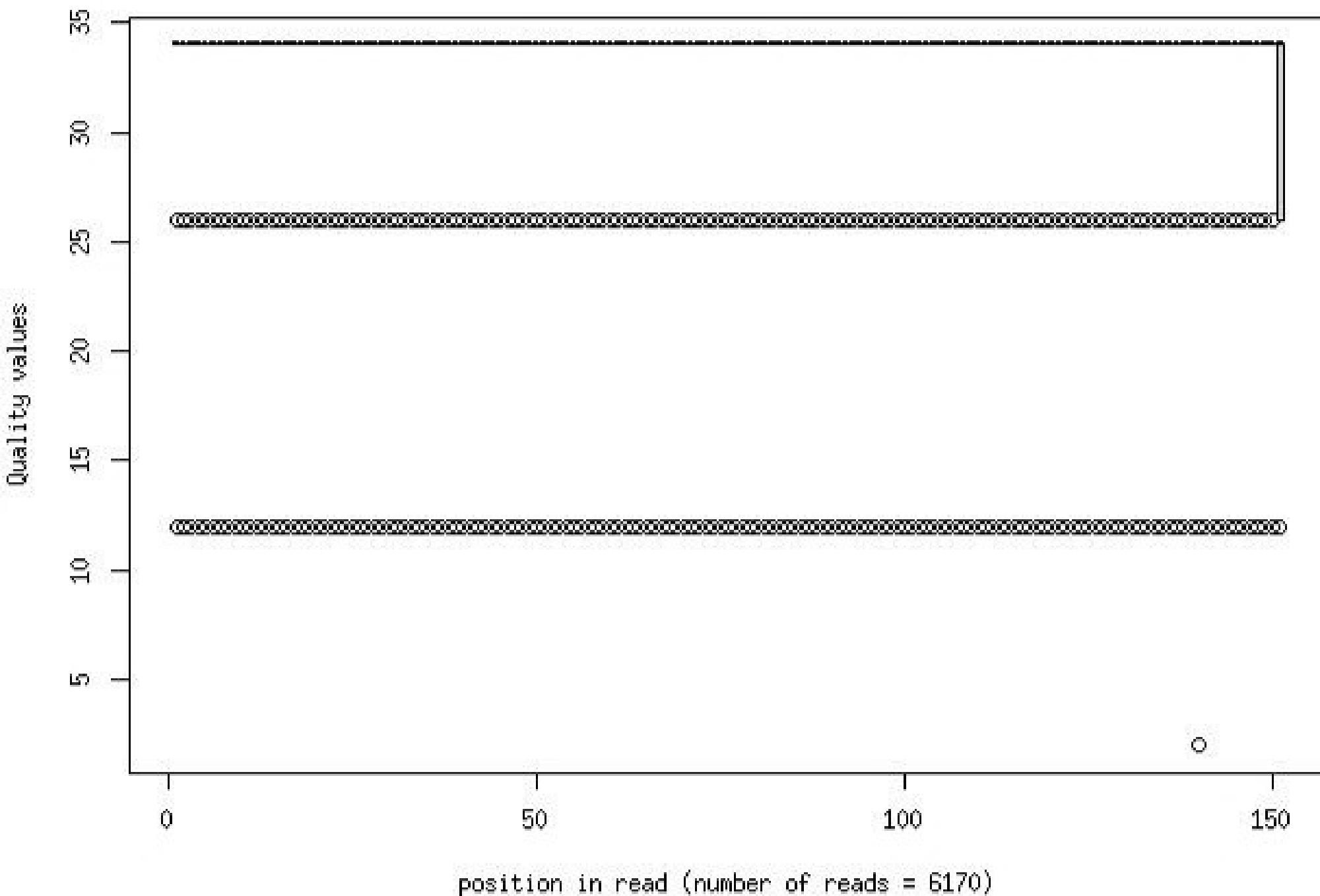
Quality distribution by position in read stn149_alone_qb003_2_frac1000
