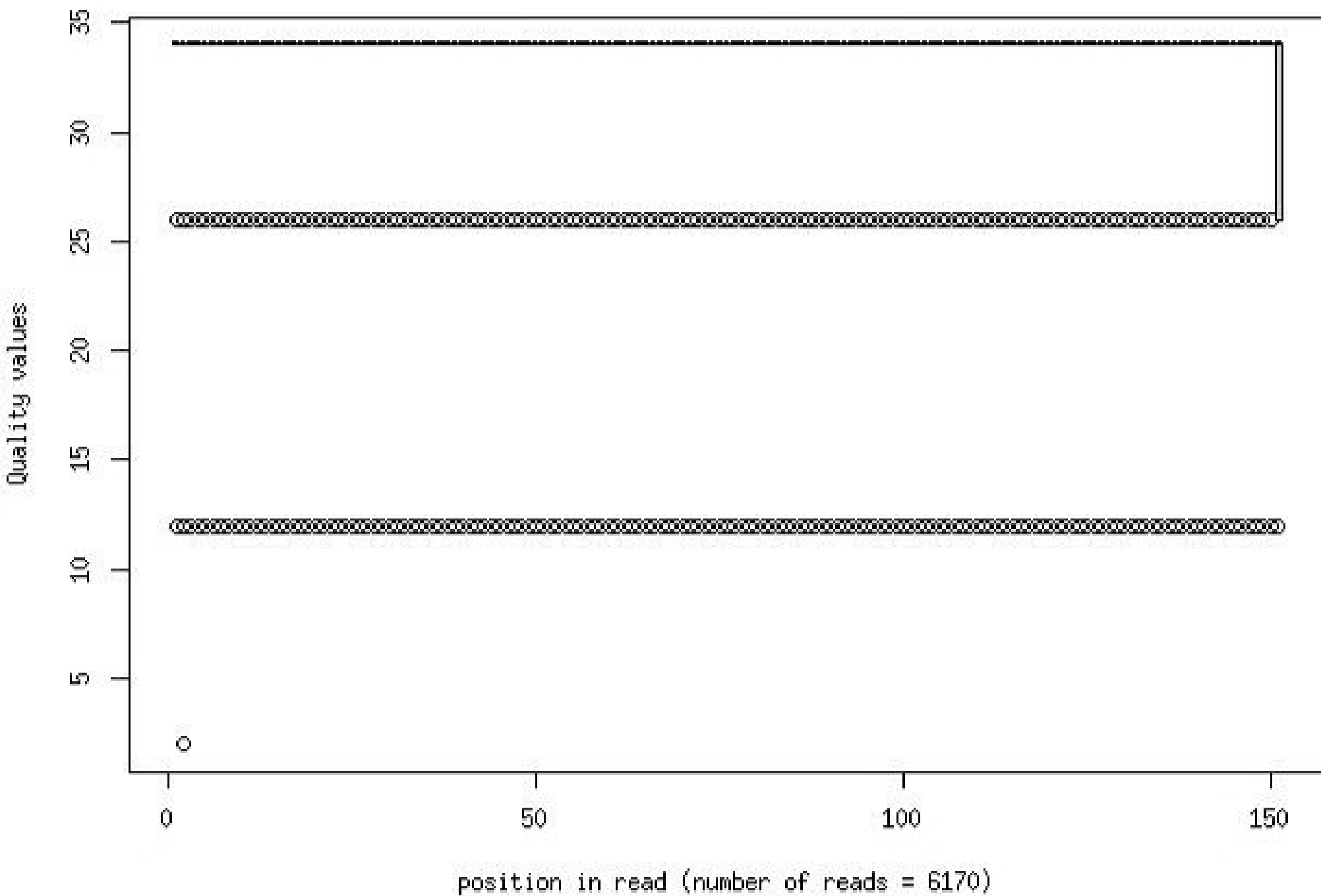
Quality distribution by position in read stn149_alone_qb003_1_frac1000
