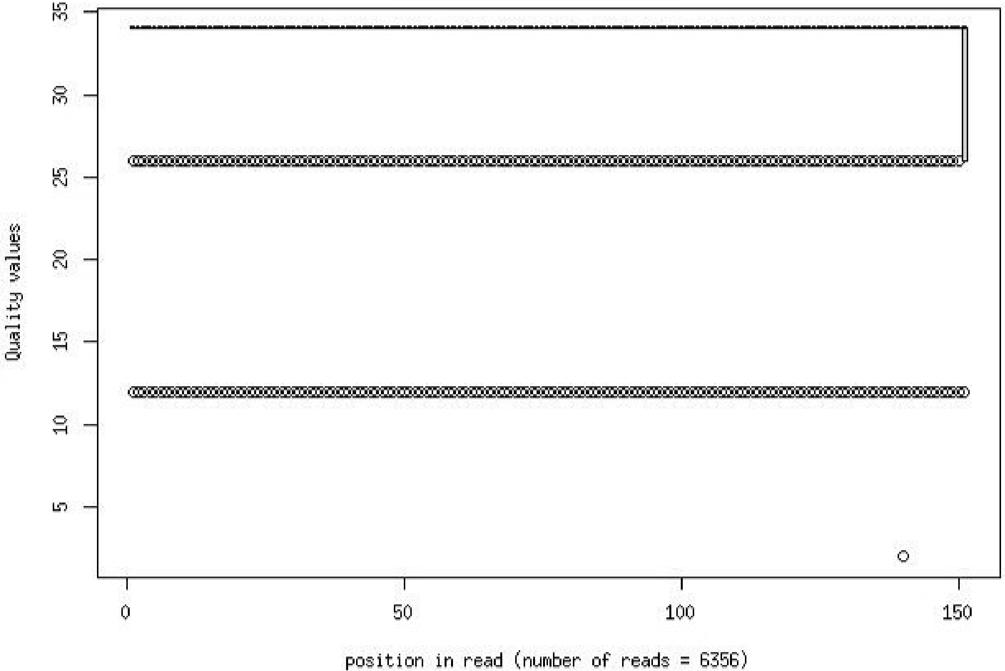
Quality distribution by position in read stn149_ccult_qb001_2_frac1000
