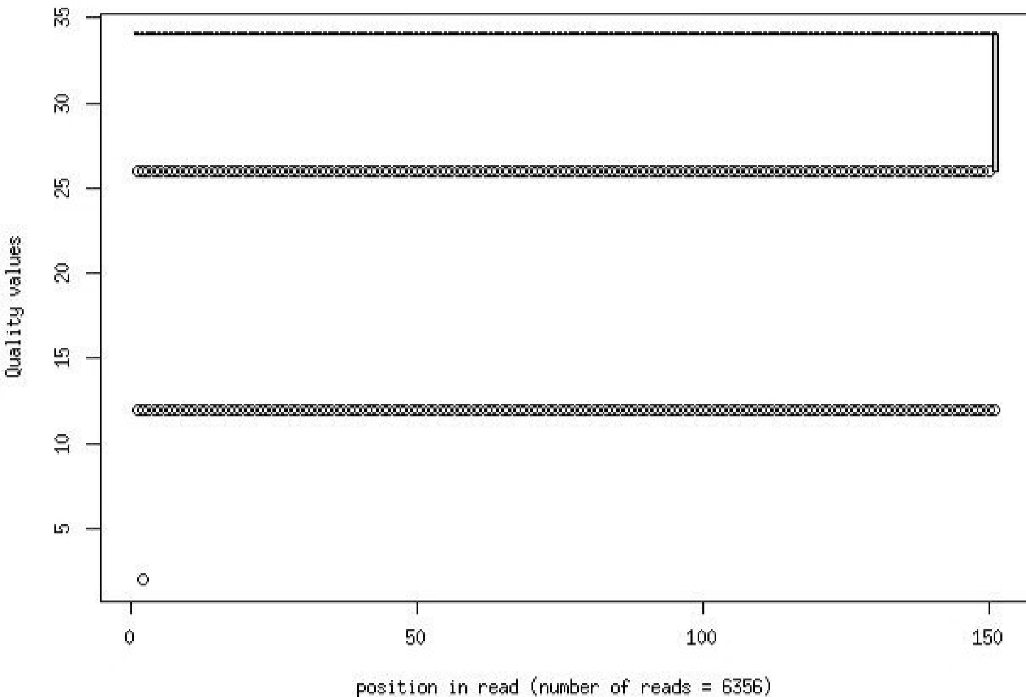
Quality distribution by position in read stn149_ccult_qb001_1_frac1000
