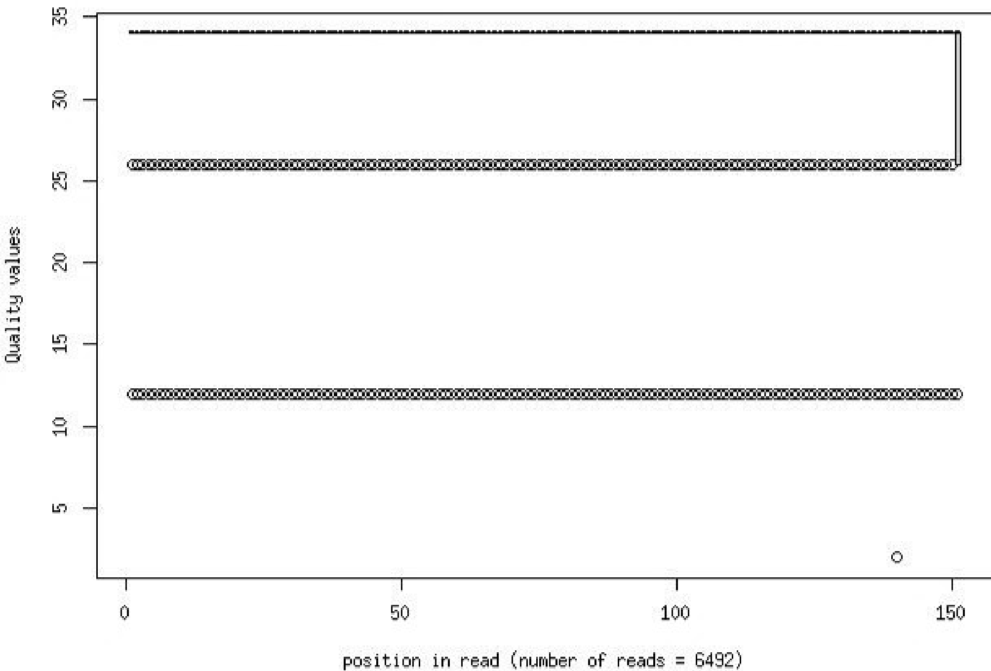
Quality distribution by position in read h9corg_ccult_qb002_2_frac1000
