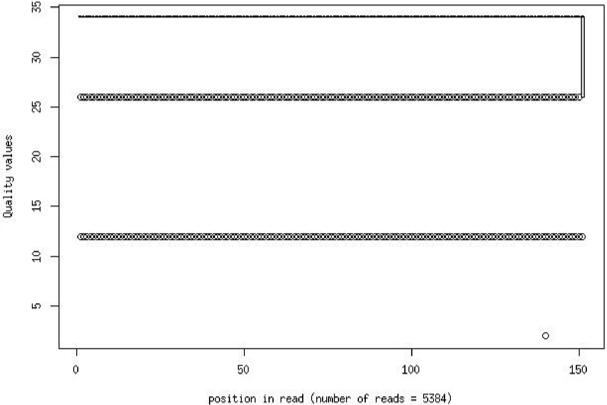
Quality distribution by position in read h9corg_alone_qb004_2_frac1000
