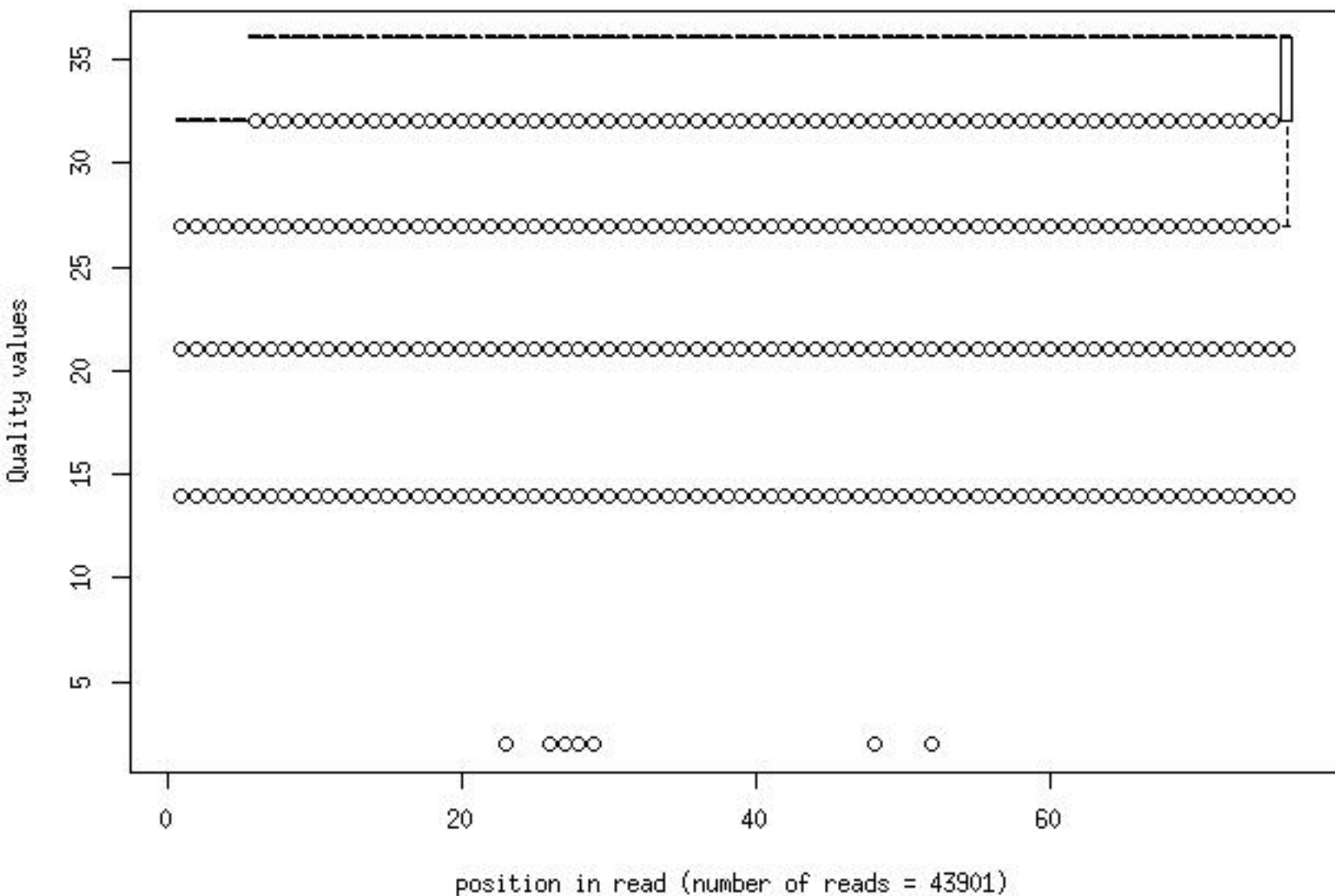
Quality distribution by position in read hips_649g2_dox_pa021_1_frac10
