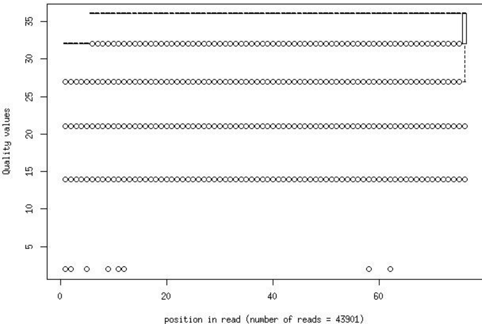
Quality distribution by position in read hips_649g2_dox_pa021_2_frac10
