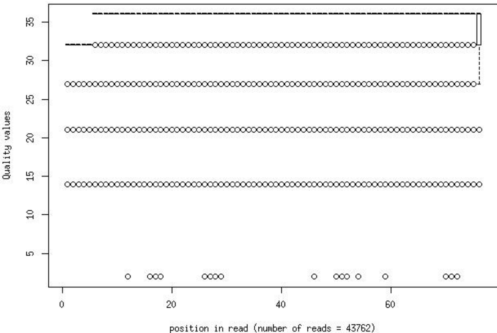
Quality distribution by position in read hips_649g2_ndx_pa019_1_frac10
