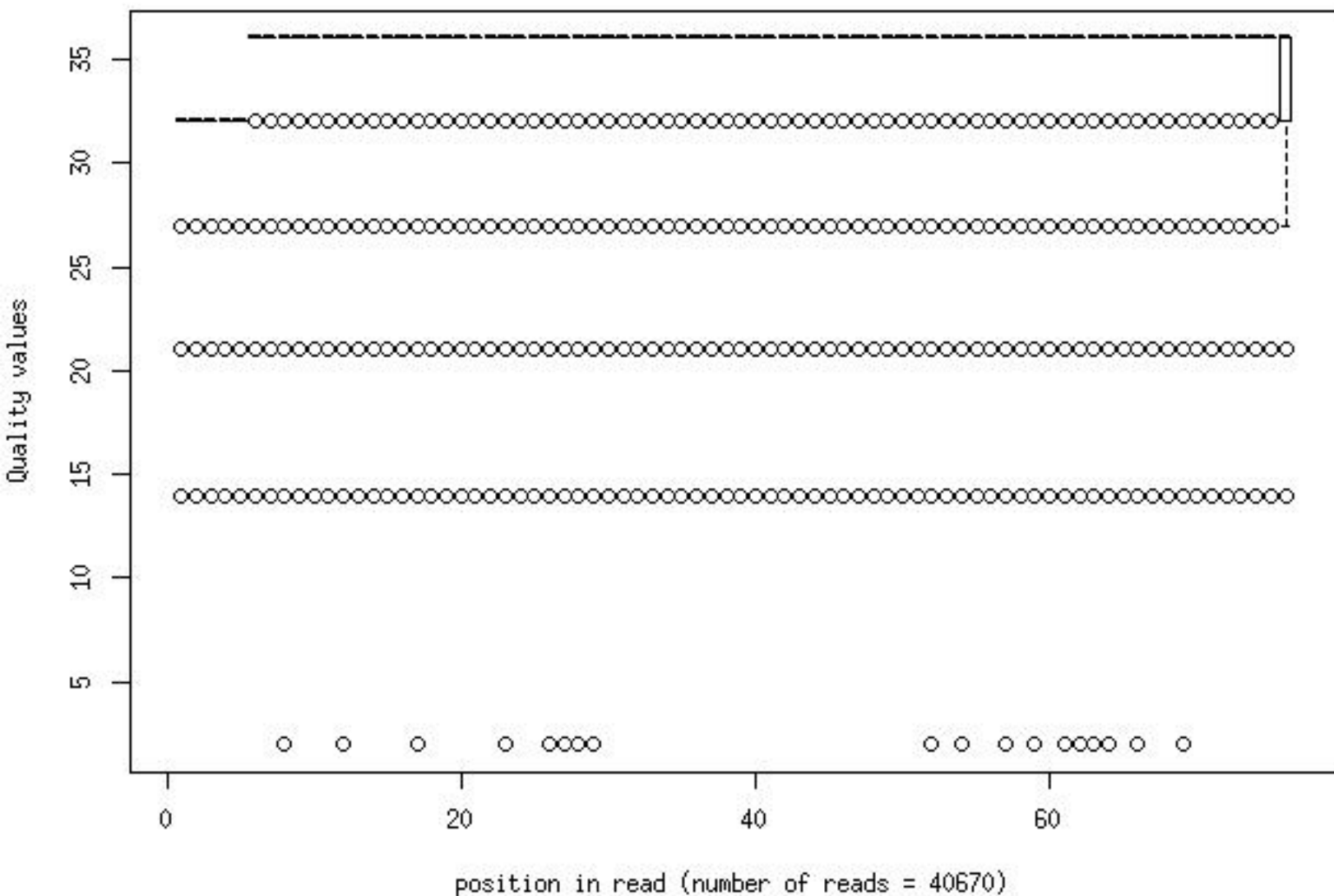
Quality distribution by position in read hips_649g2_ndx_pa020_1_frac10
