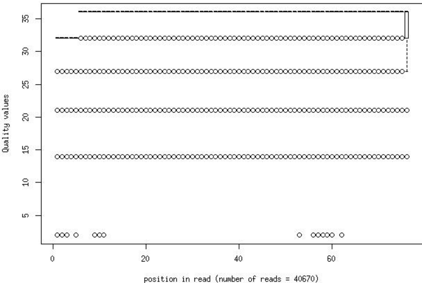
Quality distribution by position in read hips_649g2_ndx_pa020_2_frac10
