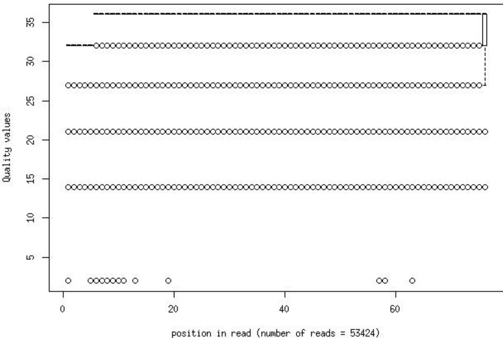
Quality distribution by position in read hips_649g2_dox_pa022_2_frac10
