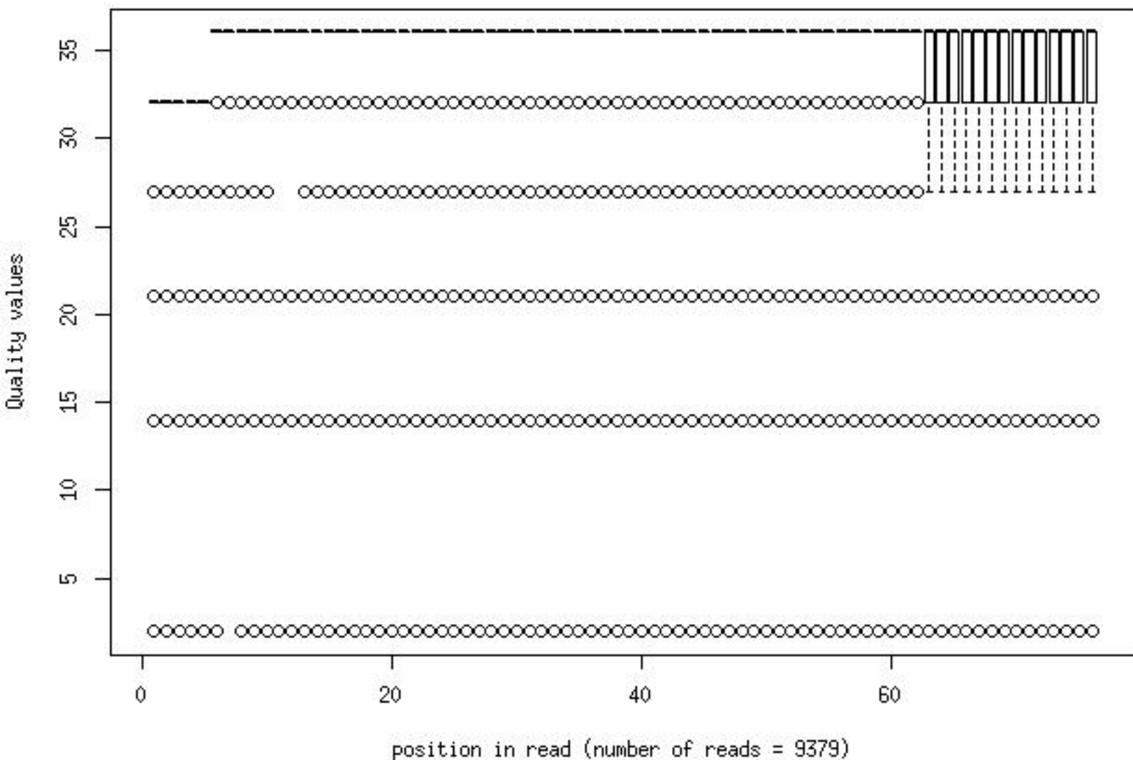
Quality distribution by position in read dipg_exos_xxx_ss006_01of10_2_frac100
