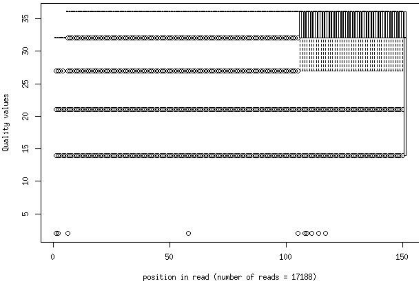
Quality distribution by position in read epi_naive_jf099_1_frac100
