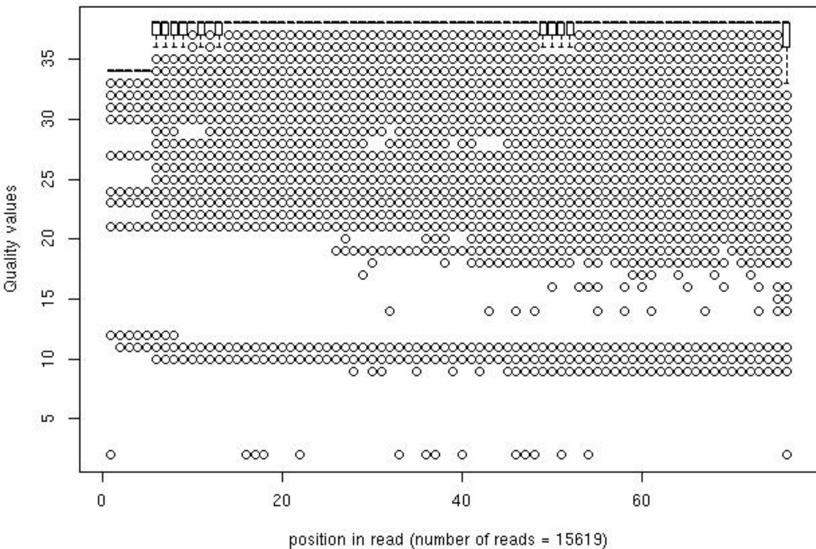
Quality distribution by position in read cips_naive_jf087_2_frac100
