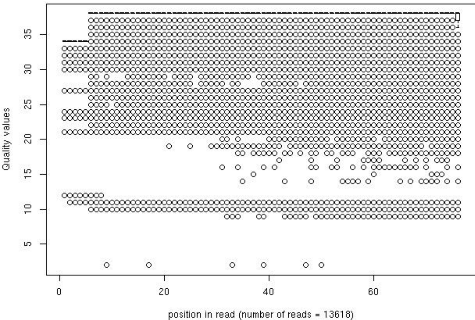
Quality distribution by position in read cips_naive_jf086_2_frac100
