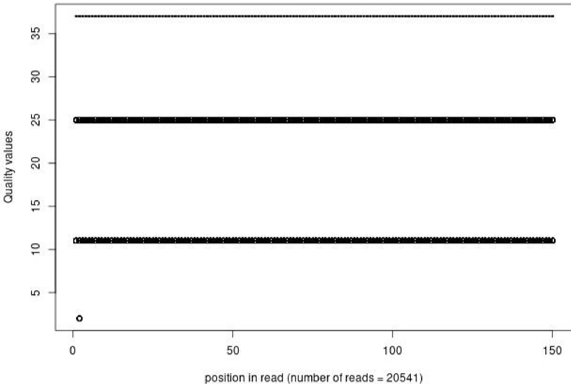
Quality distribution by position in read bmdm_kotg_az316_01of10_1_frac100
