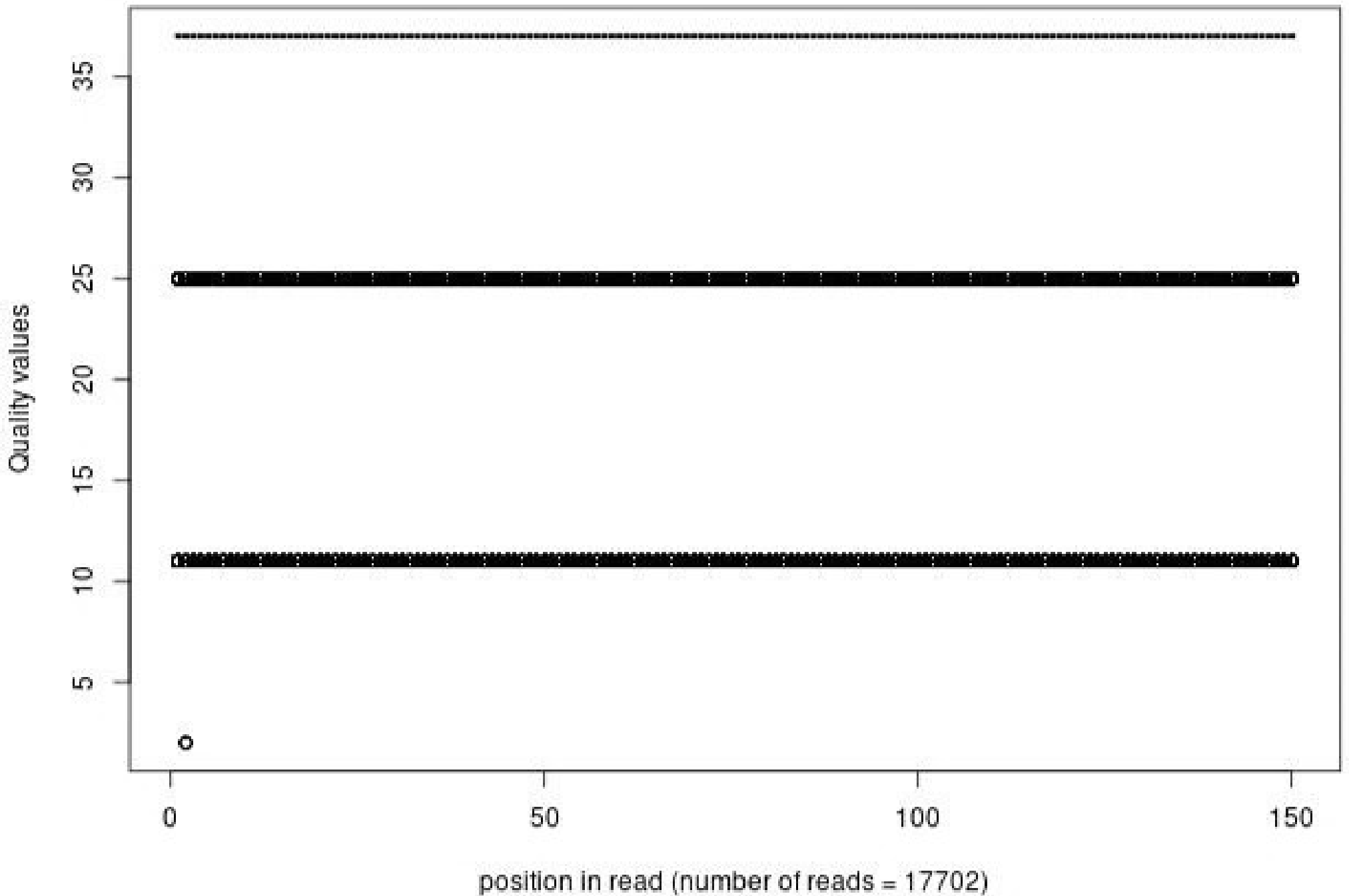
Quality distribution by position in read bmdm_kotg_az313_01of10_1_frac100
