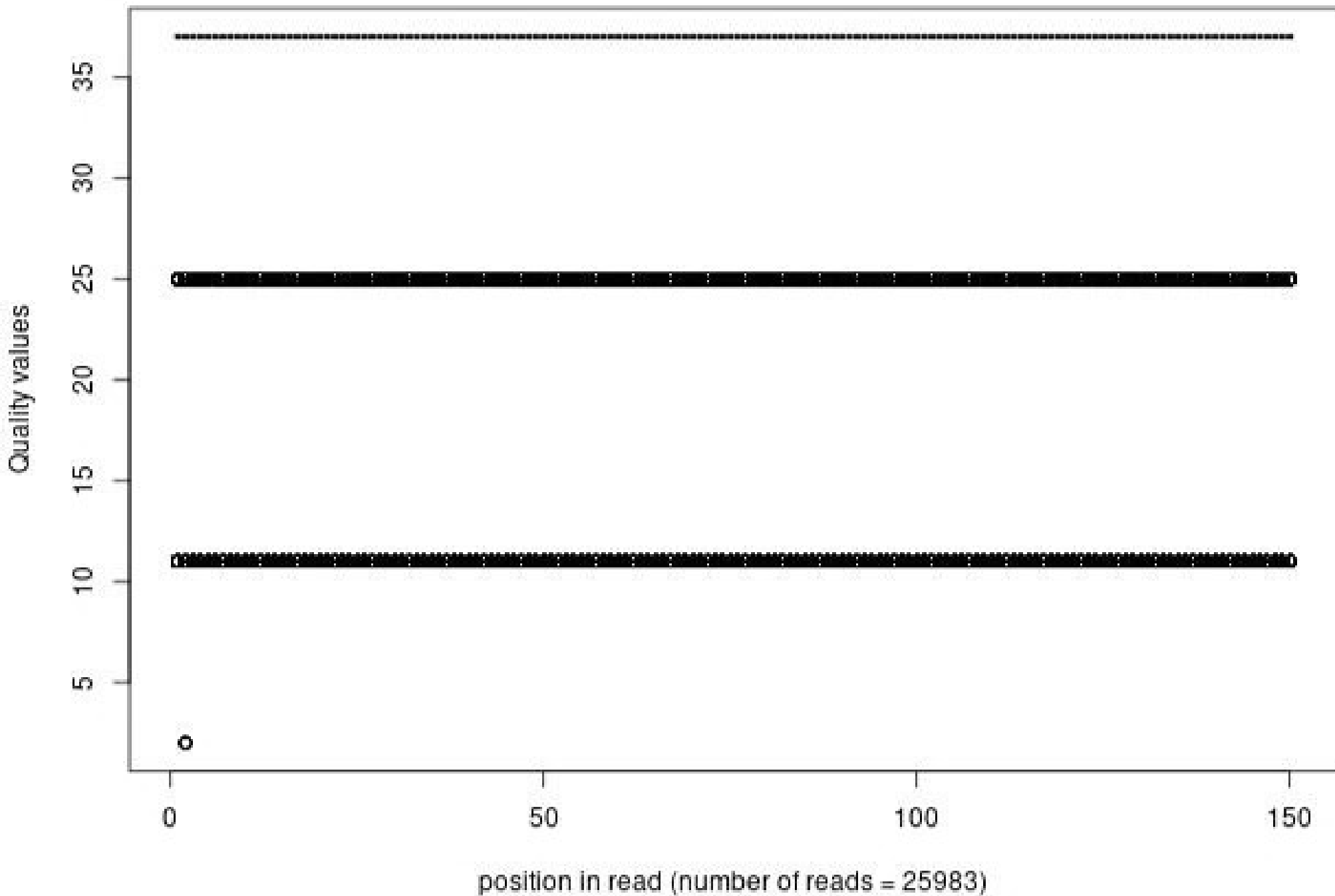
Quality distribution by position in read bmdm_koxx_az309_01of10_1_frac100
