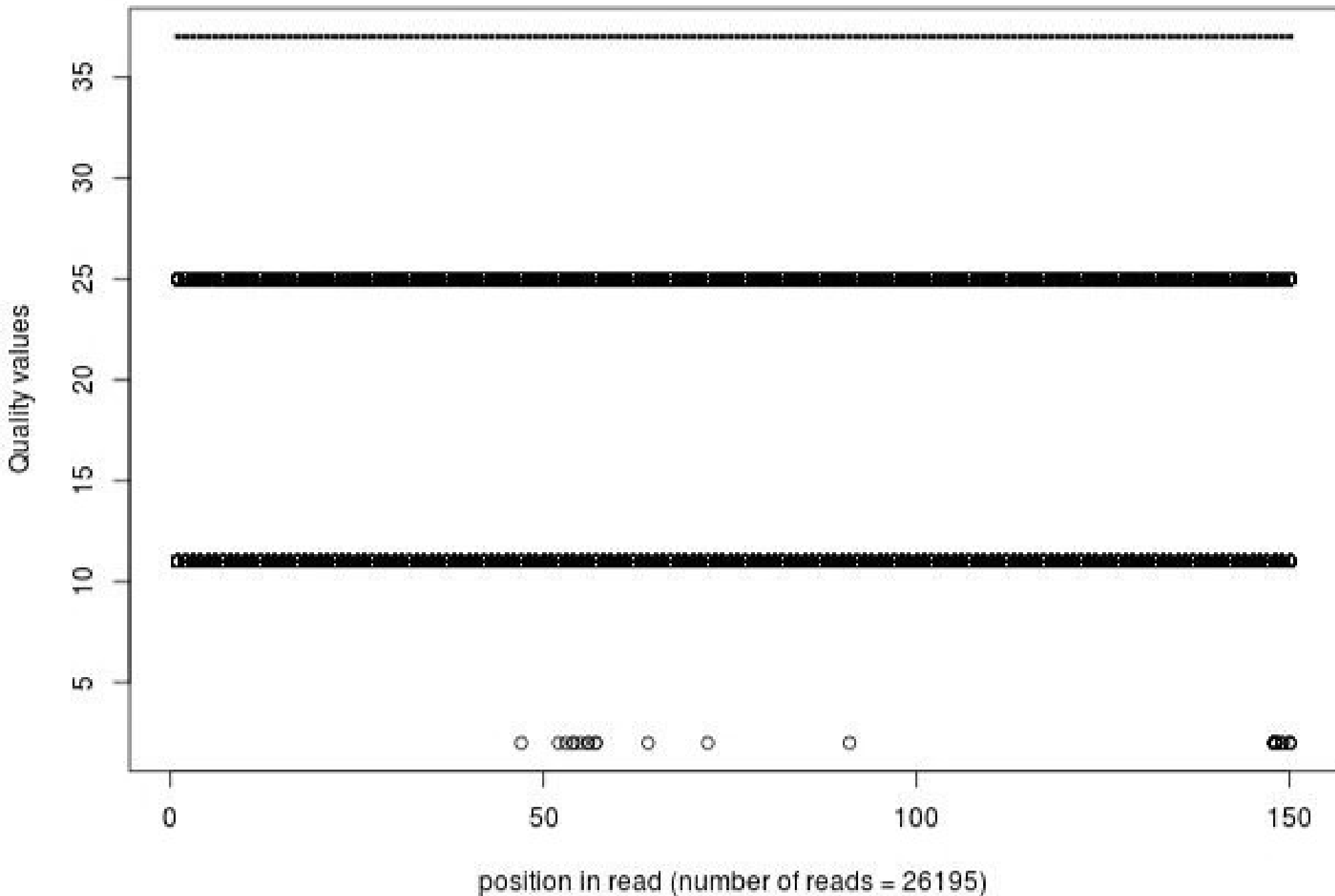
Quality distribution by position in read bmdm_koxx_az308_01of10_2_frac100
