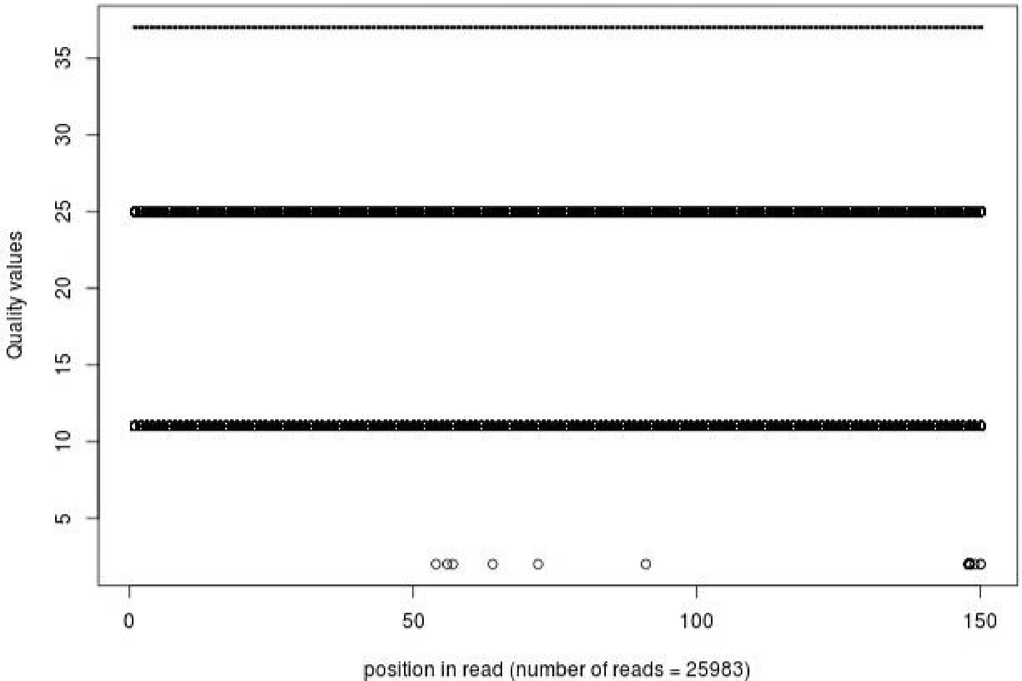
Quality distribution by position in read bmdm_koxx_az309_01of10_2_frac100
