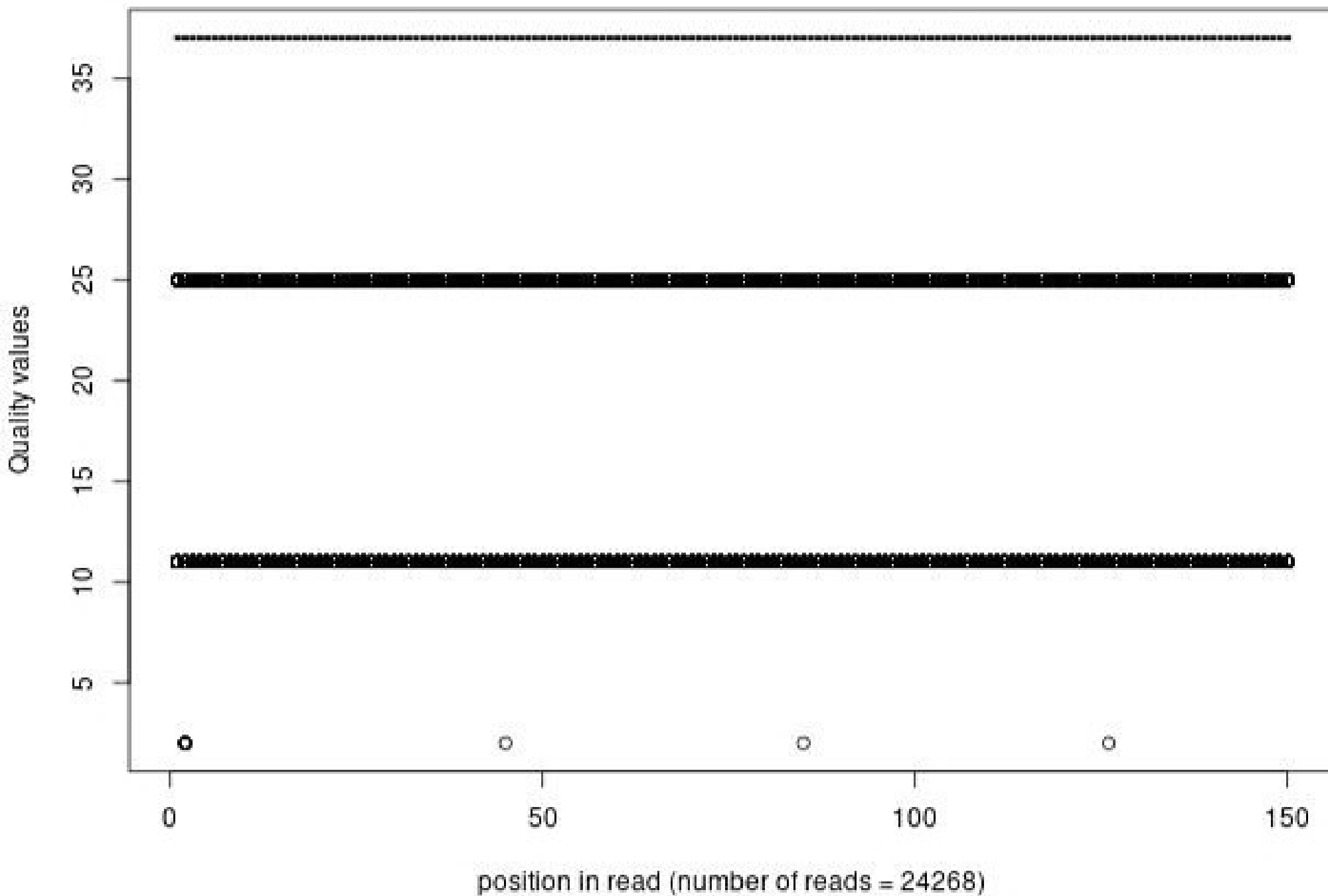
Quality distribution by position in read bmdm_wild_az302_01of10_1_frac100
