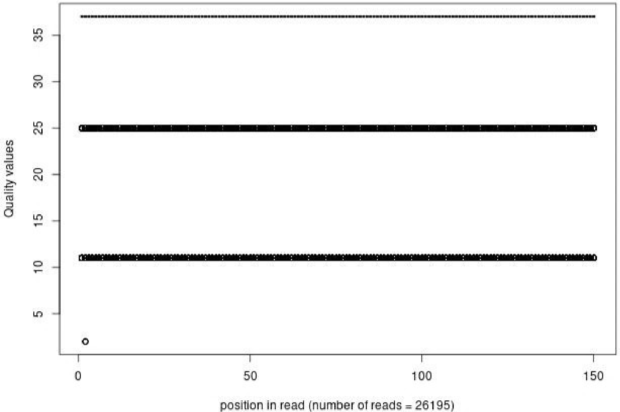
Quality distribution by position in read bmdm_koxx_az308_01of10_1_frac100
