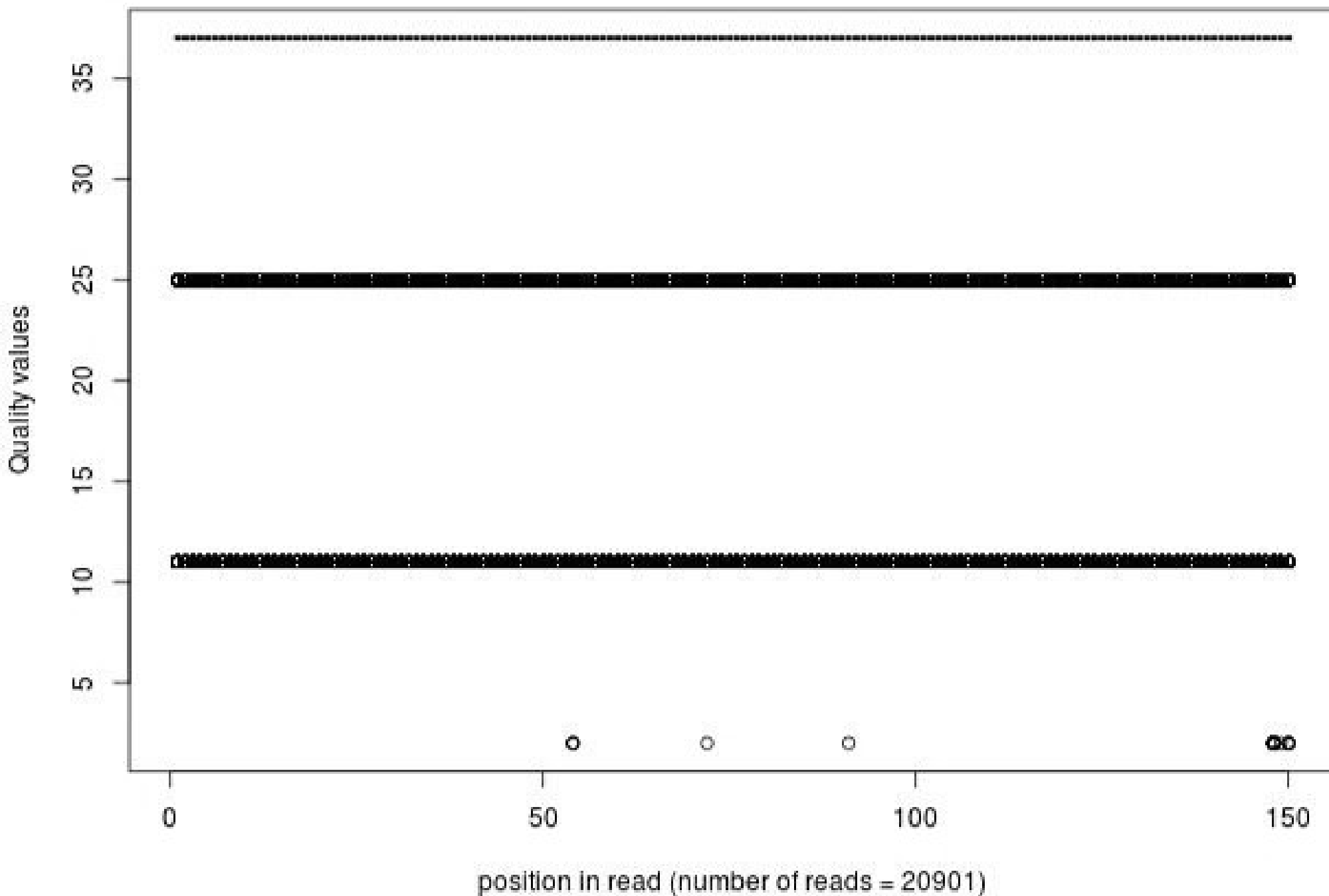
Quality distribution by position in read bmdm_koxx_az310_01of10_2_frac100
