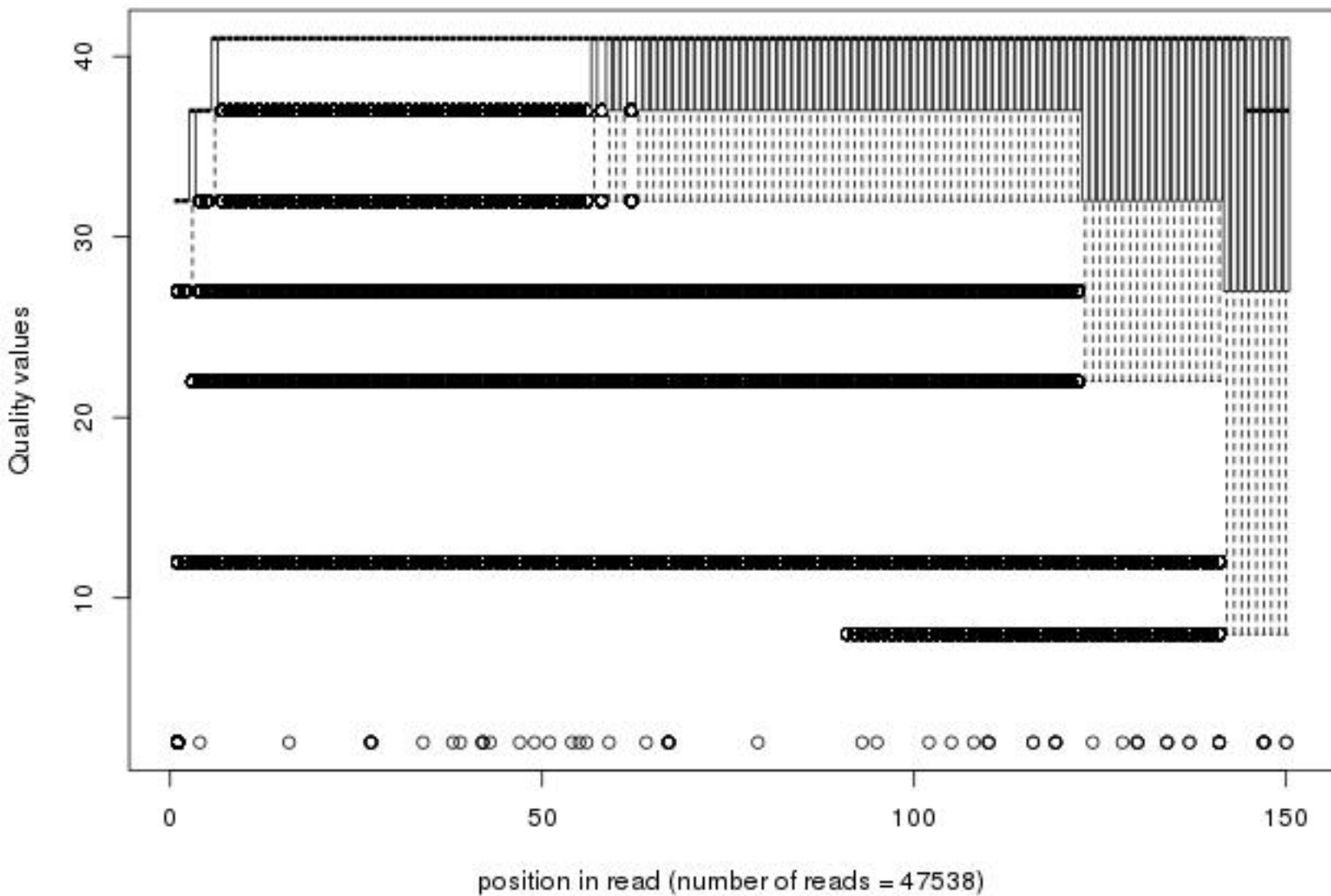
Quality distribution by position in read bal_rmair_er041_01of40_2_frac25
