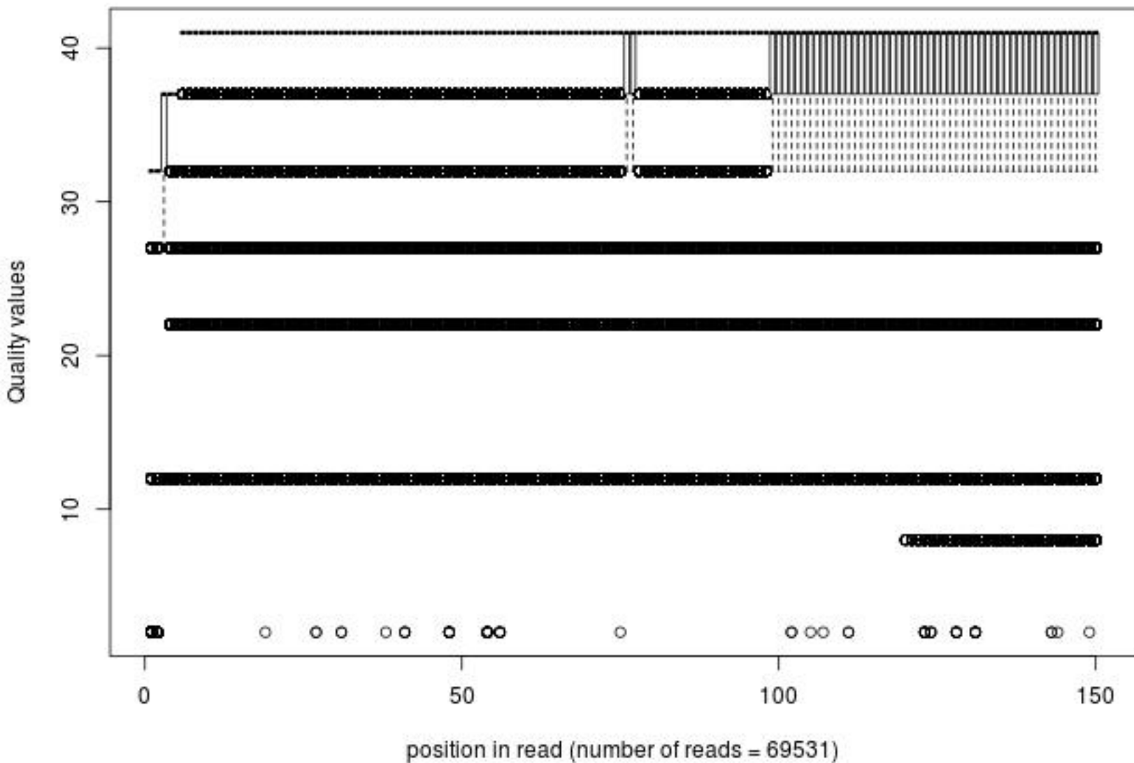
Quality distribution by position in read bal_cgsmk_er045_01of40_1_frac25
