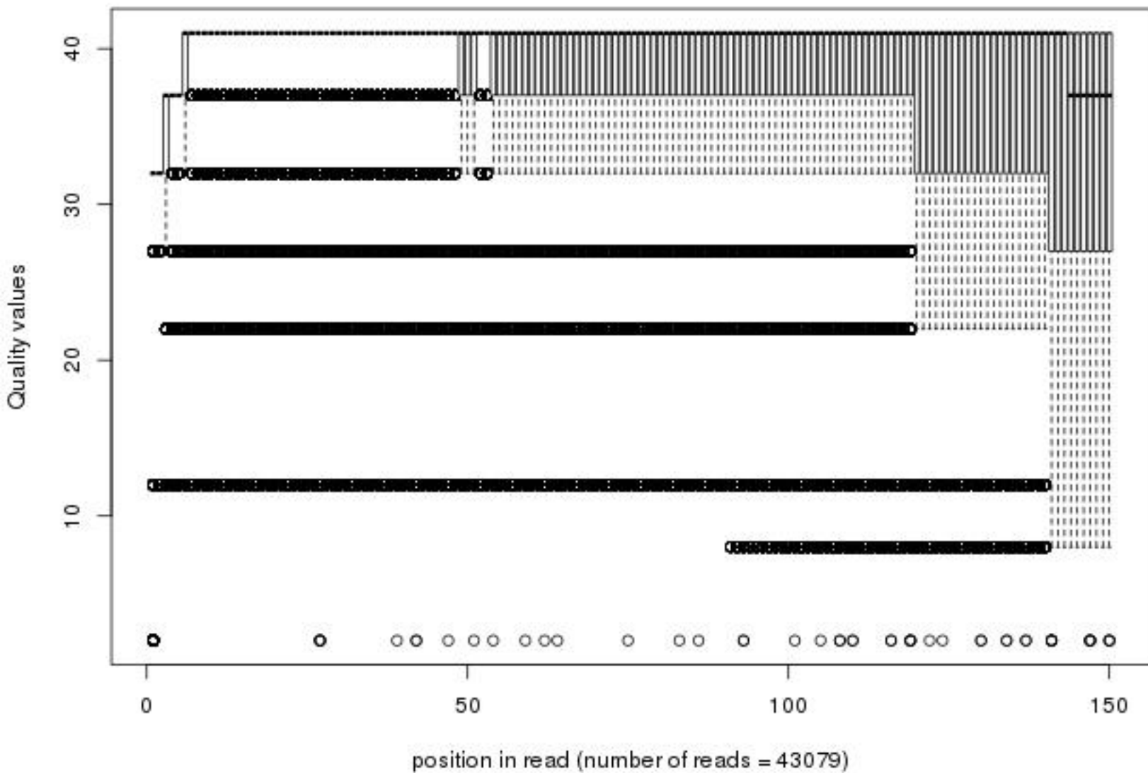
Quality distribution by position in read bal_cgsmk_er048_01of40_2_frac25
