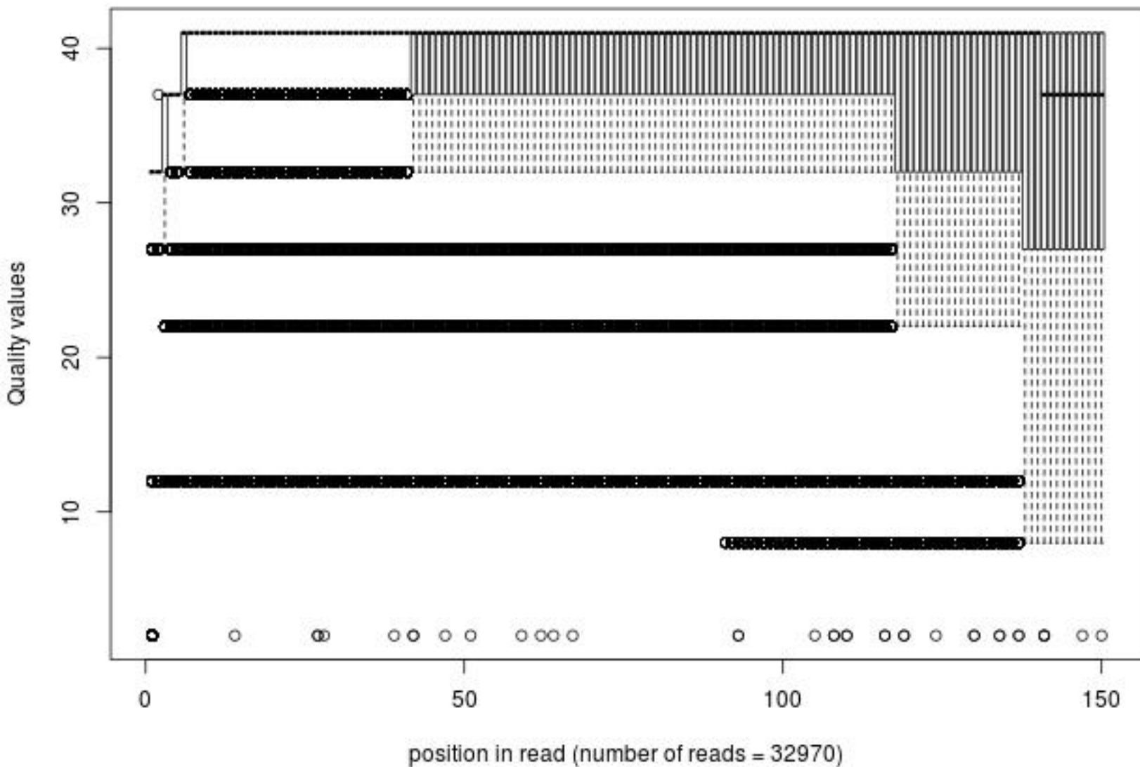
Quality distribution by position in read bal_rmair_er043_01of40_2_frac25
