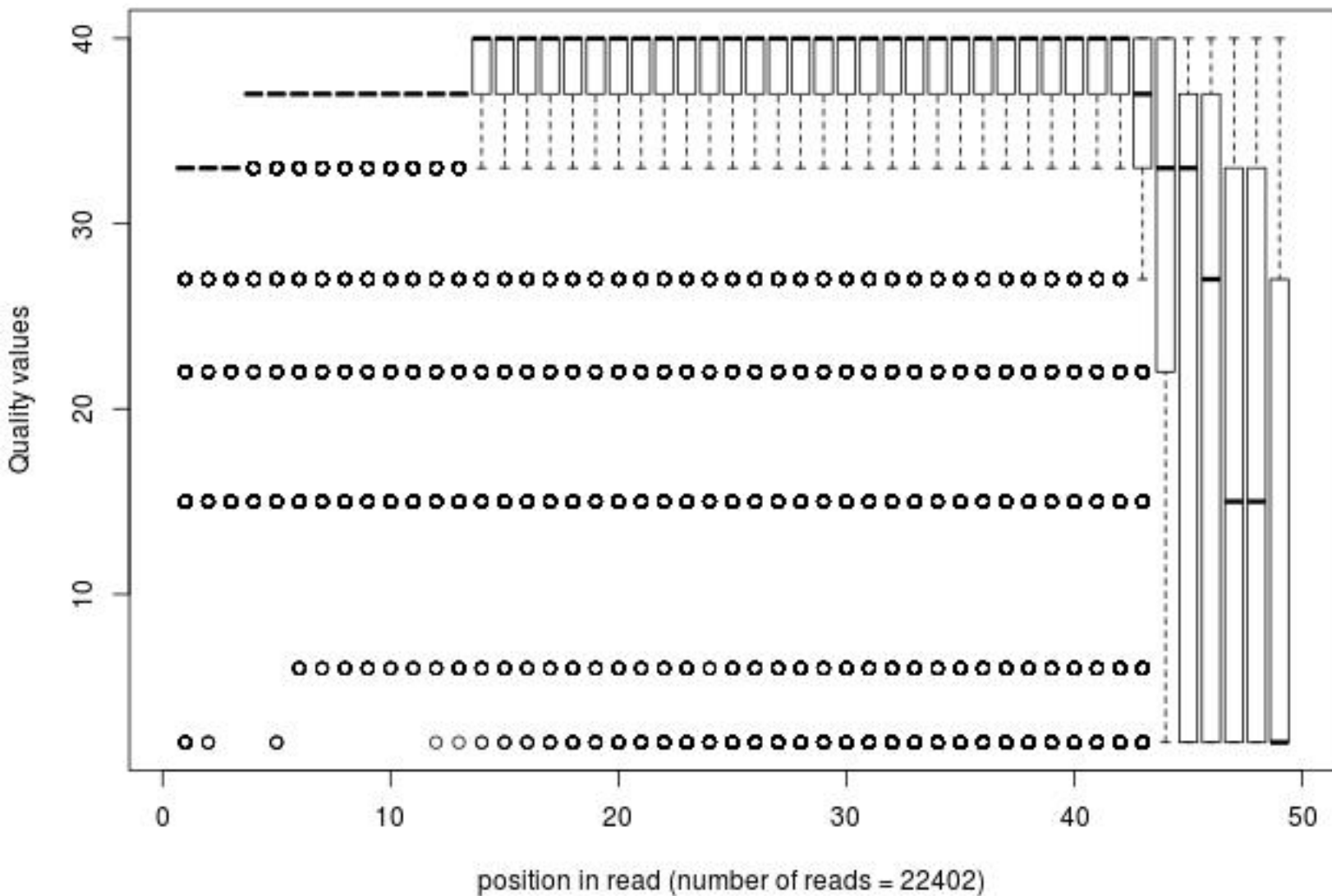
Quality distribution by position in read bcell_wz412_frac100
