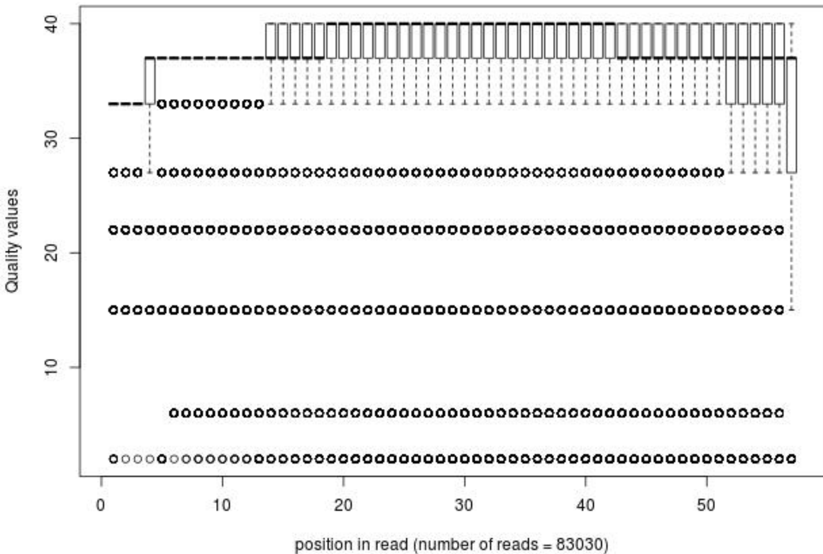
Quality distribution by position in read mppxx_wz383_frac100
