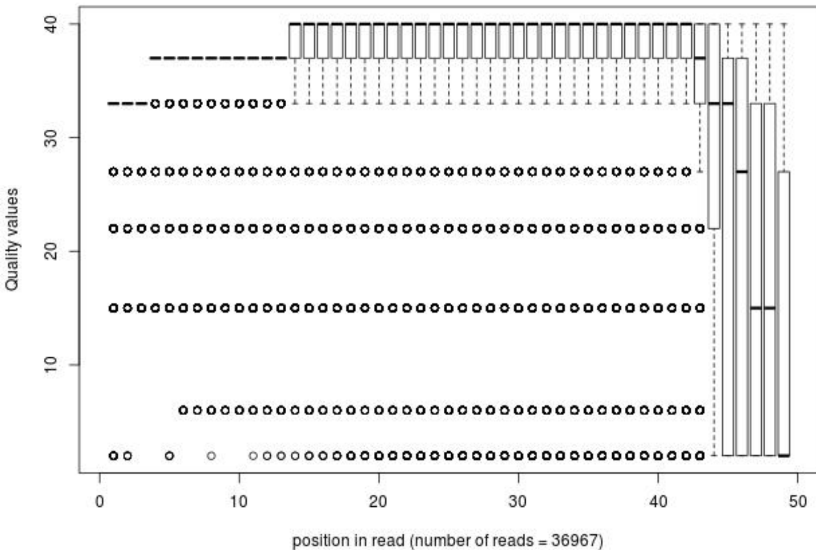
Quality distribution by position in read clpxx_wz387_frac100
