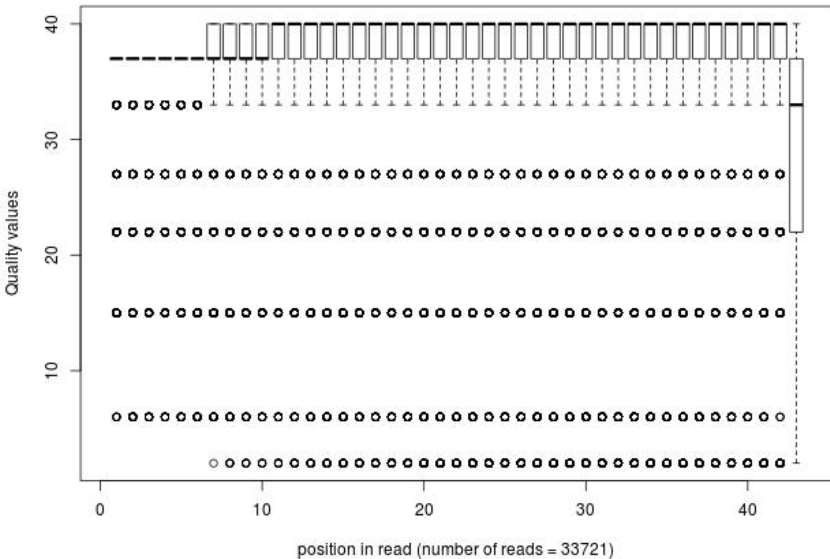
Quality distribution by position in read macro_wz398_frac100
