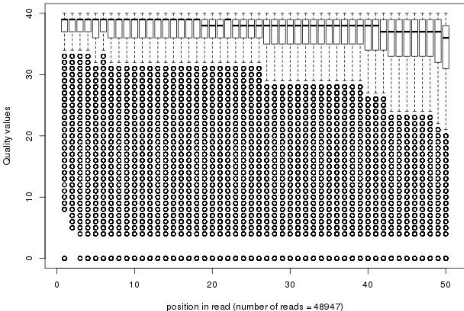
Quality distribution by position in read bmdm_chro_060m_sm004_01of20_frac100
