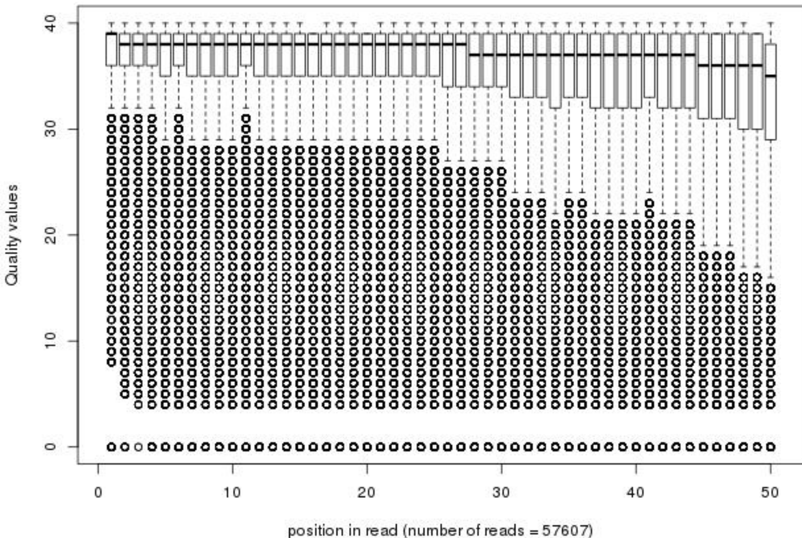
Quality distribution by position in read bmdm_nucl_030m_sm013_01of20_frac100
