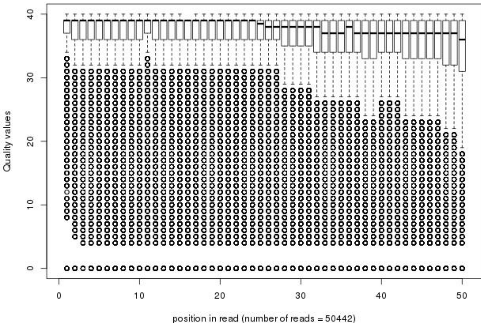
Quality distribution by position in read bmdm_nucl_000m_sm011_01of20_frac100
