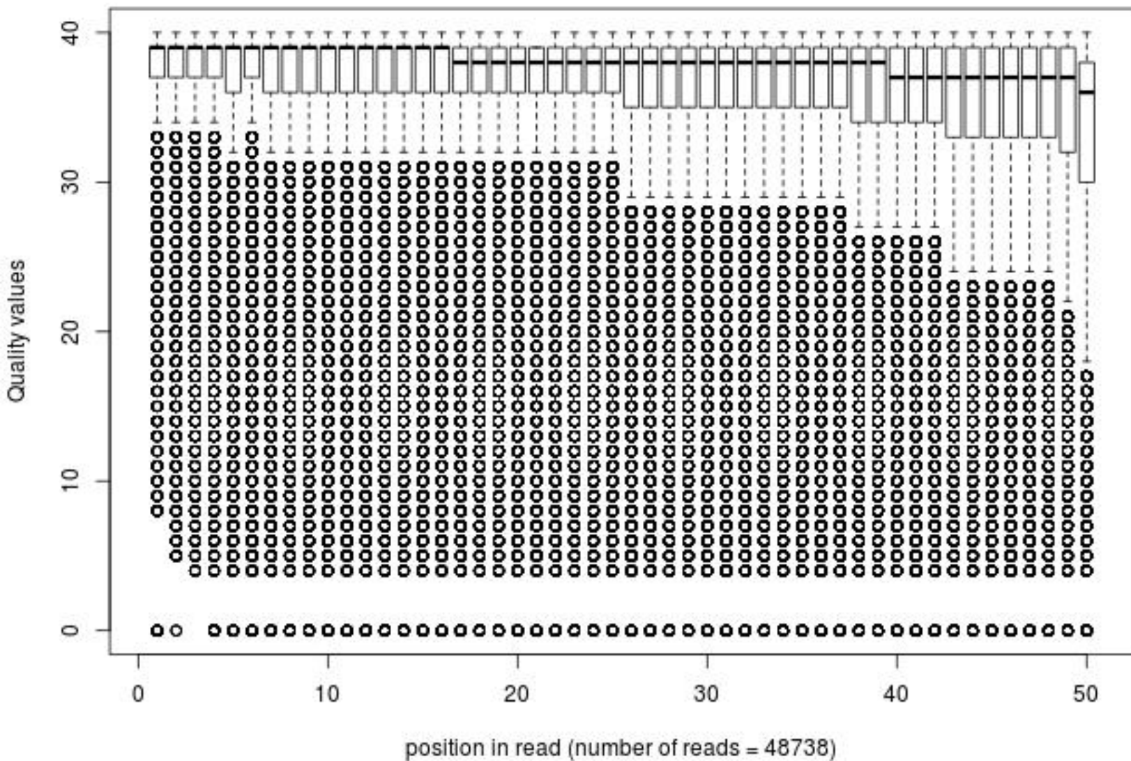
Quality distribution by position in read bmdm_chro_120m_sm005_01of20_frac100
