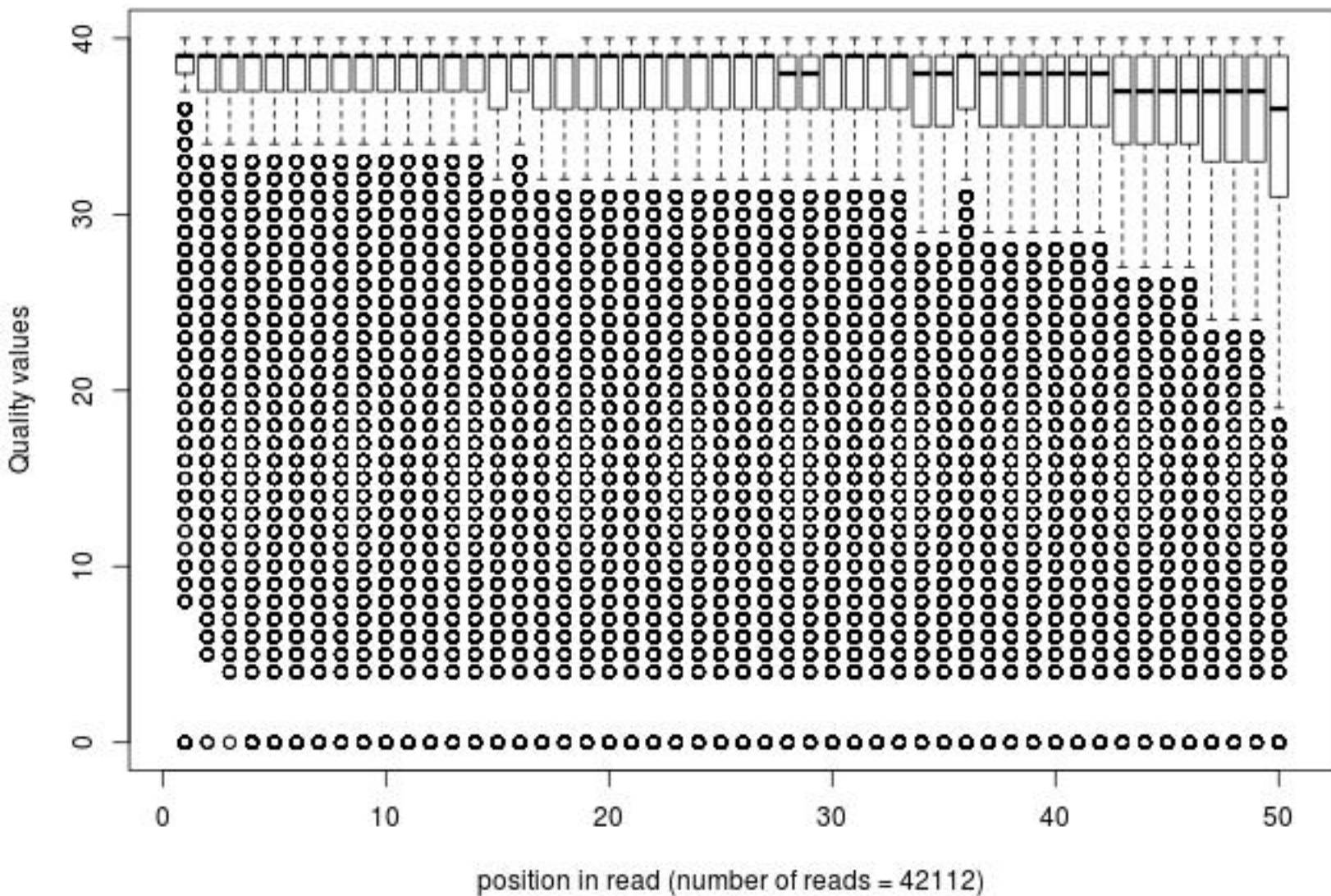
Quality distribution by position in read bmdm_chro_030m_sm003_01of20_frac100
