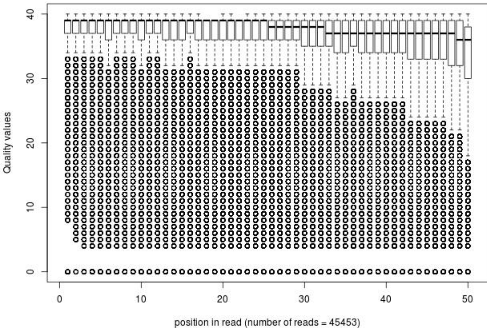
Quality distribution by position in read bmdm_cyto_060m_sm009_01of20_frac100
