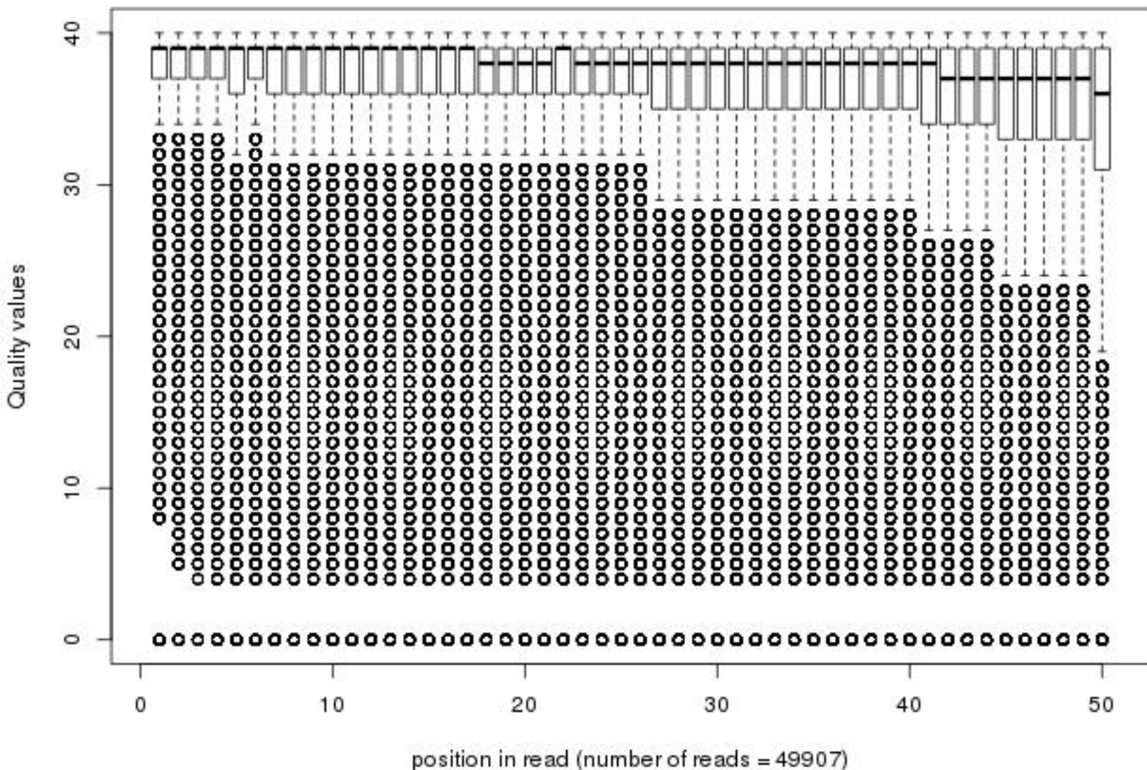
Quality distribution by position in read bmdm_chro_015m_sm002_01of20_frac100
