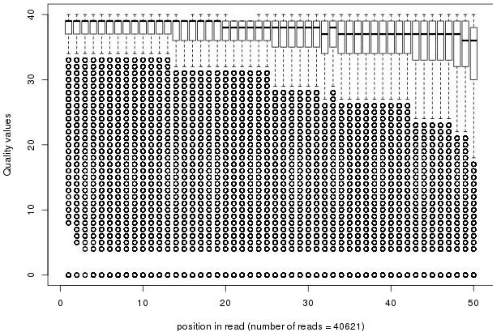
Quality distribution by position in read bmdm_cyto_000m_sm006_01of20_frac100
