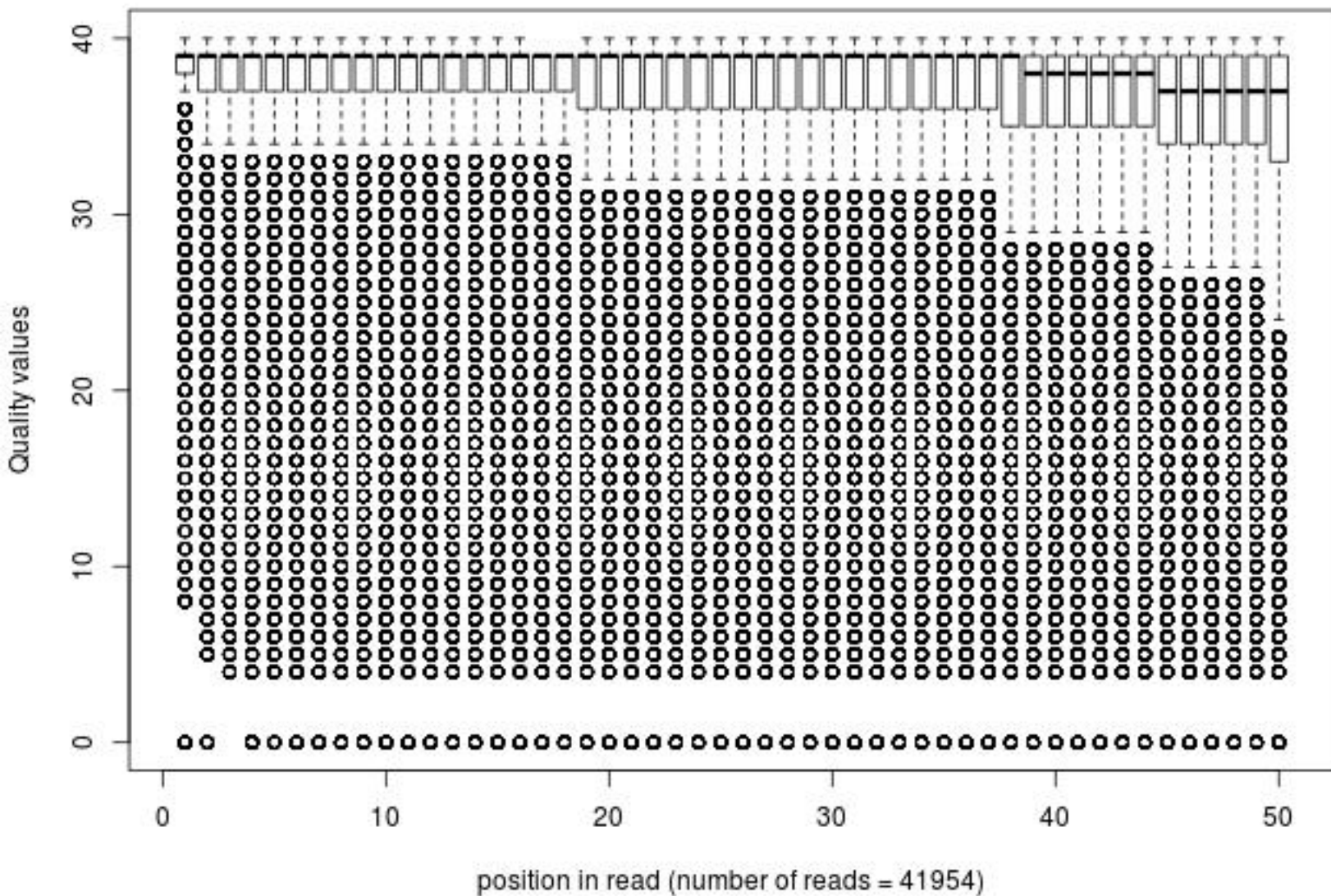
Quality distribution by position in read bmdm_chro_000m_sm001_01of20_frac100
