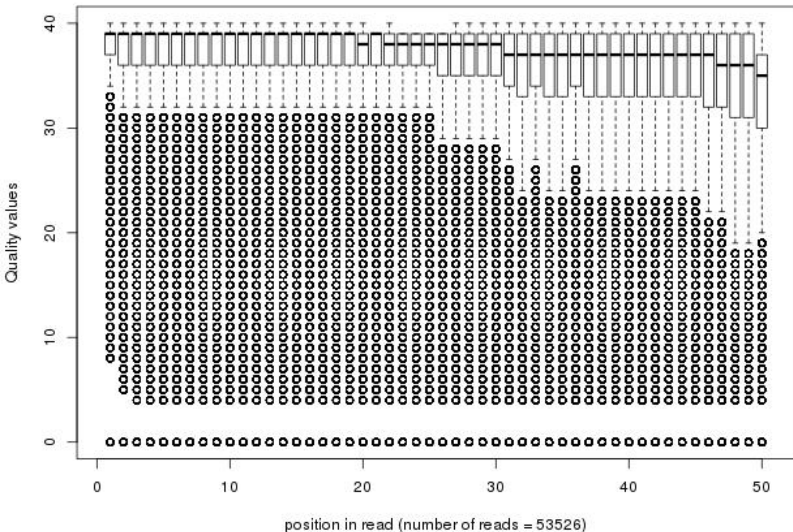
Quality distribution by position in read bmdm_cyto_120m_sm010_01of20_frac100
