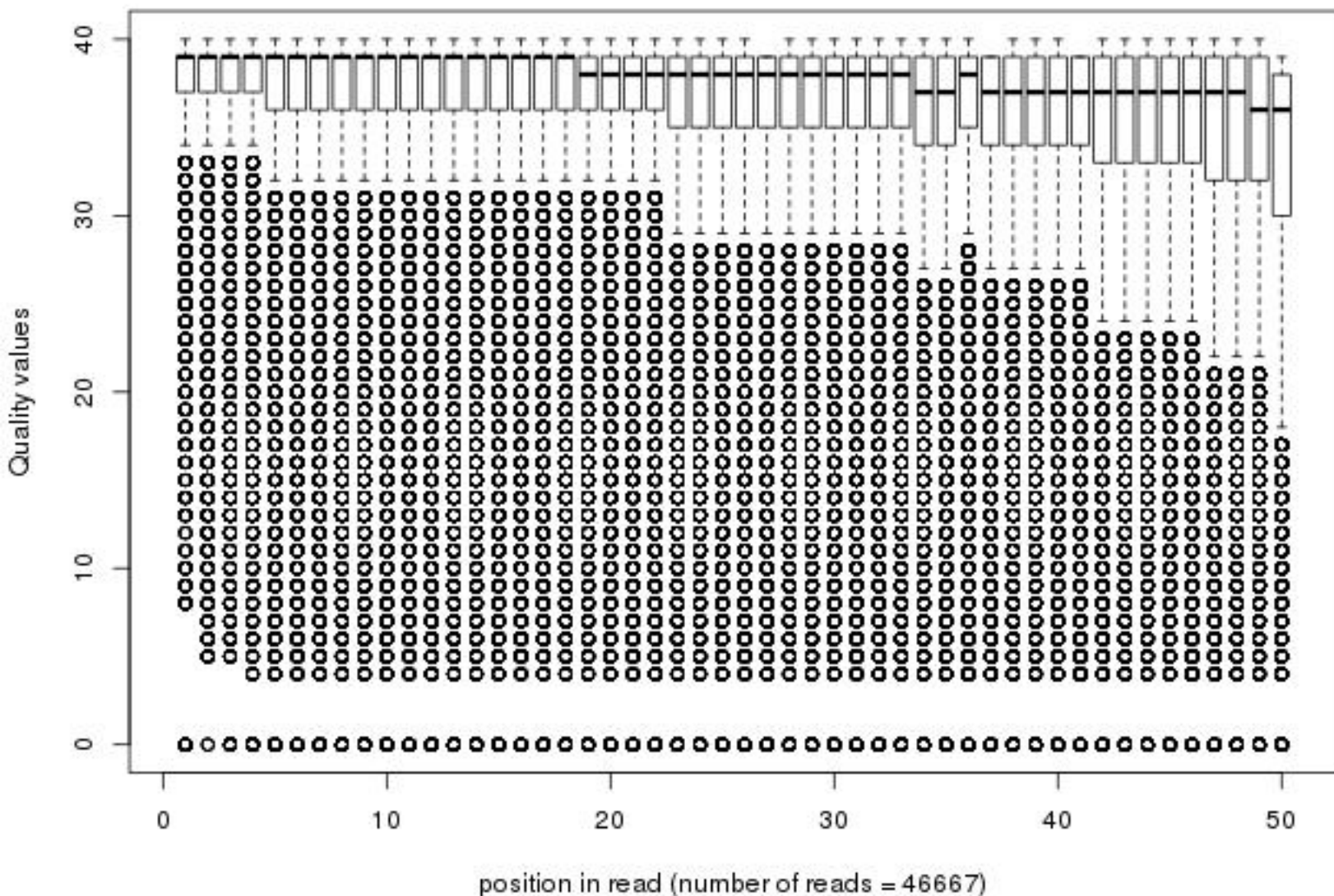
Quality distribution by position in read bmdm_cyto_030m_sm008_01of20_frac100
