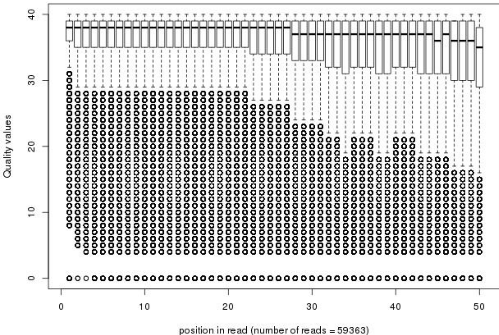
Quality distribution by position in read bmdm_nucl_120m_sm015_01of20_frac100
