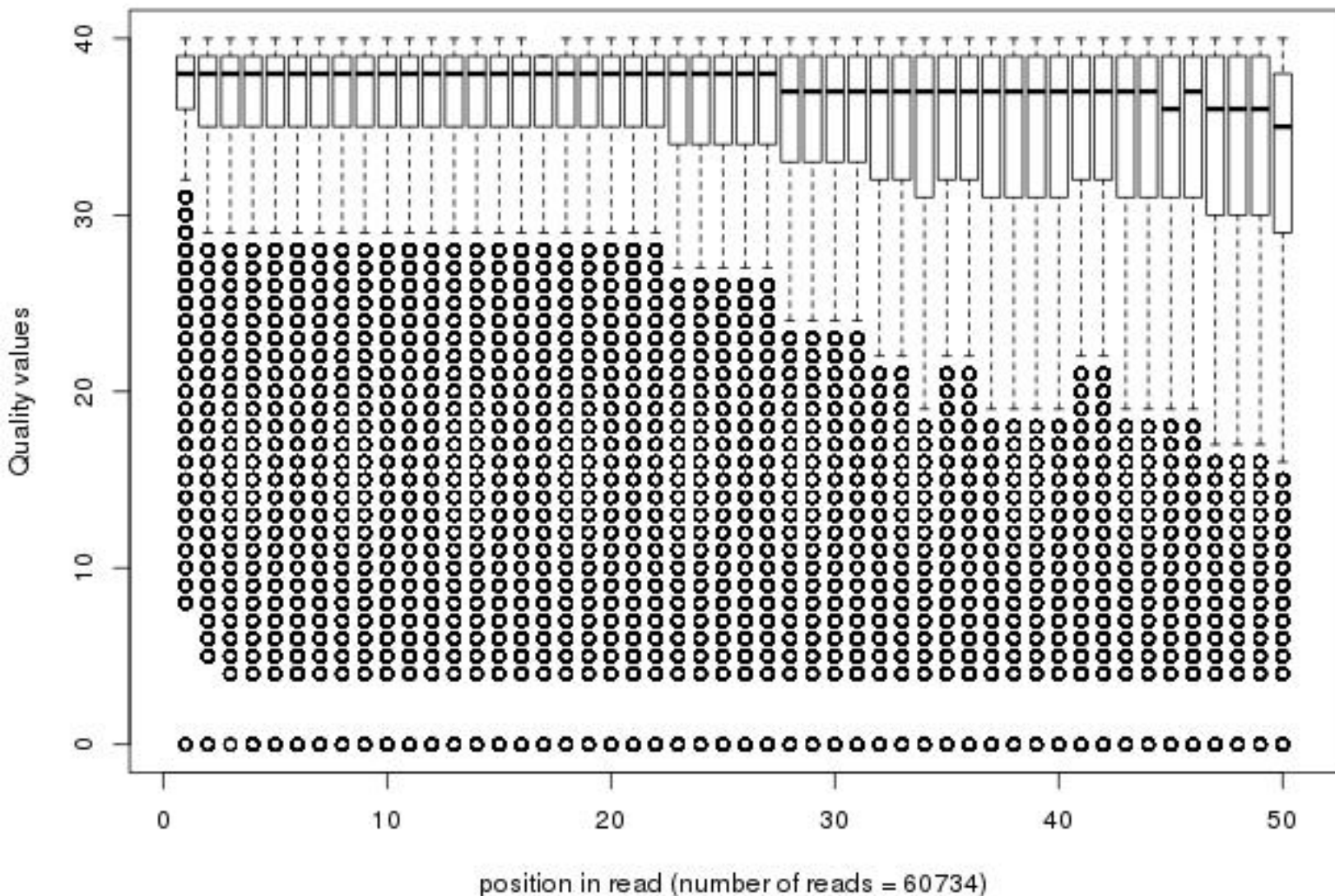
Quality distribution by position in read bmdm_nucl_015m_sm012_01of20_frac100
