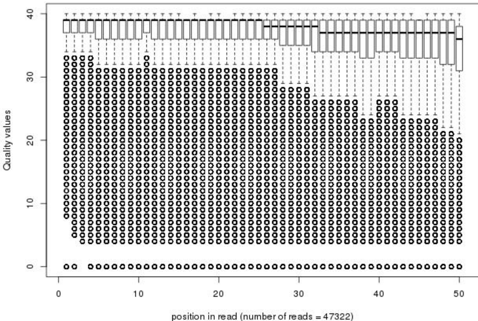
Quality distribution by position in read bmdm_nucl_060m_sm014_01of20_frac100
