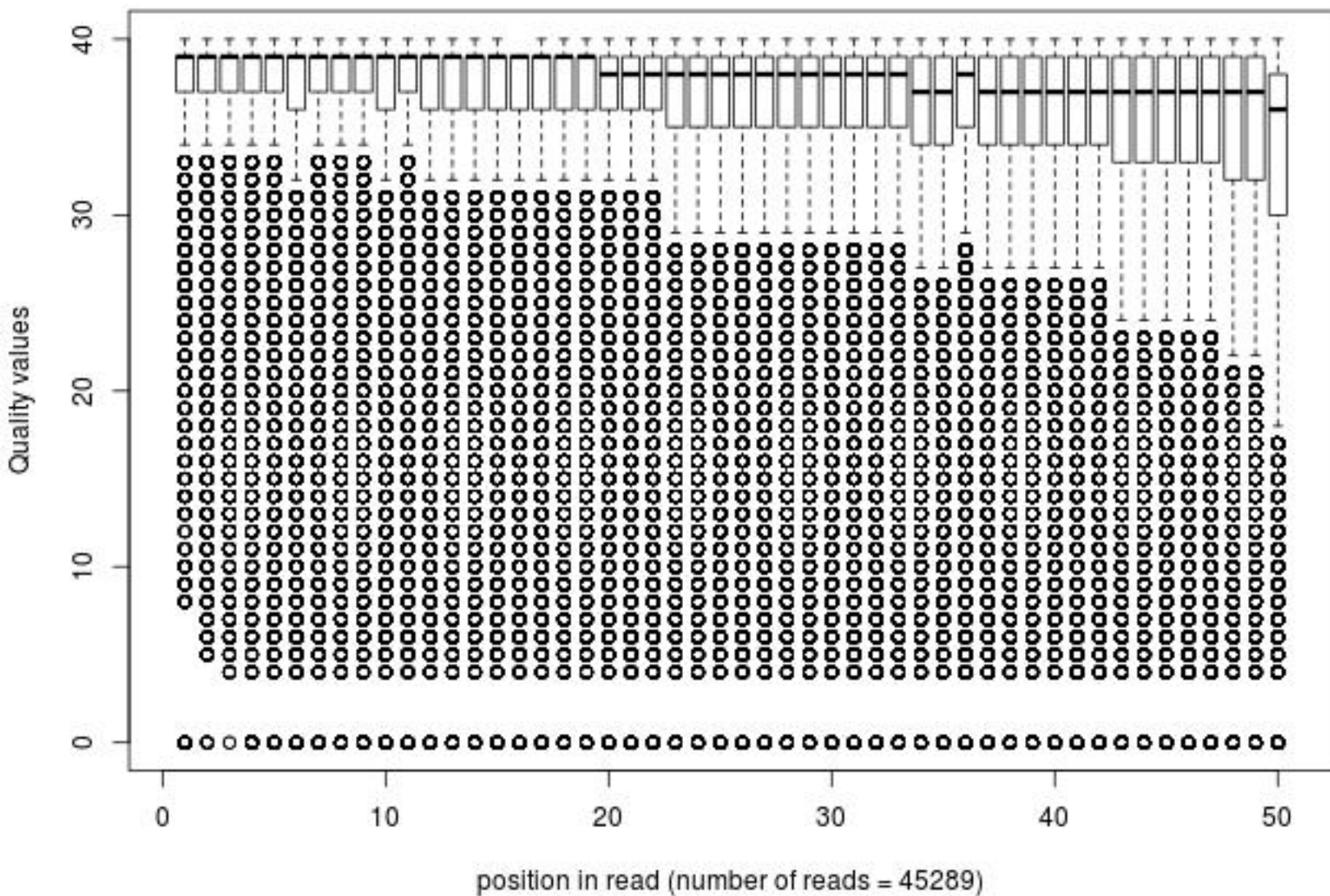
Quality distribution by position in read bmdm_cyto_015m_sm007_01of20_frac100
