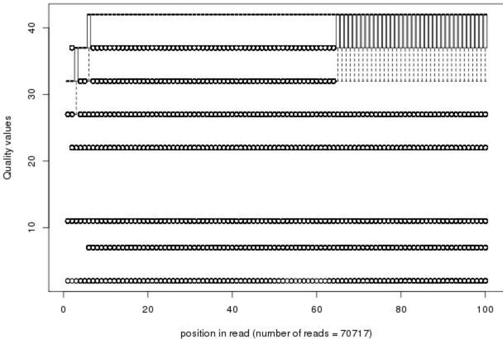
Quality distribution by position in read thp1_ctrl_p3csk4_sc003_01of40_2_frac25
