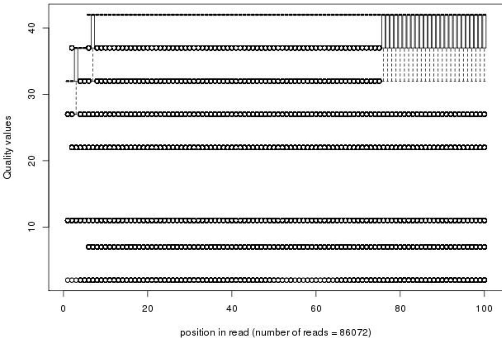
Quality distribution by position in read thp1_cox2_p3csk4_sc001_01of40_2_frac25
