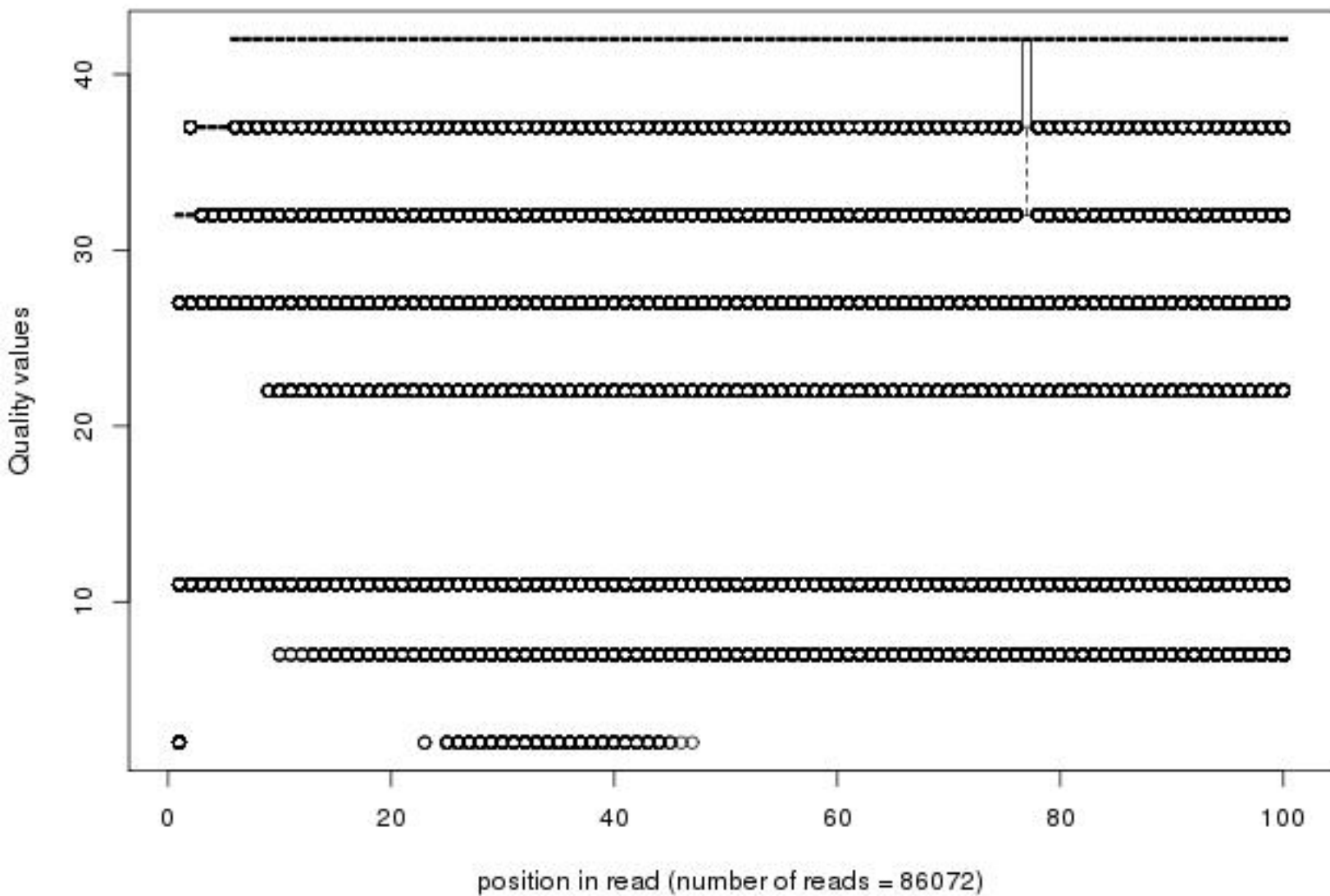
Quality distribution by position in read thp1_cox2_p3csk4_sc001_01of40_1_frac25
