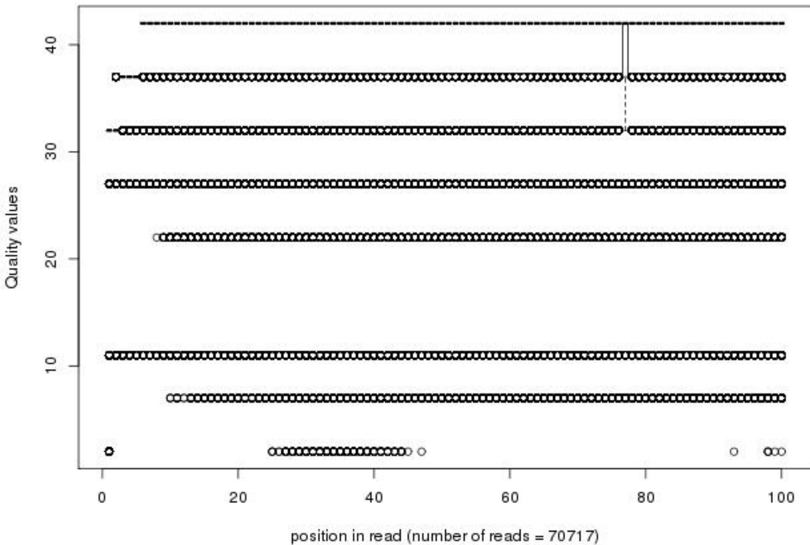
Quality distribution by position in read thp1_ctrl_p3csk4_sc003_01of40_1_frac25
