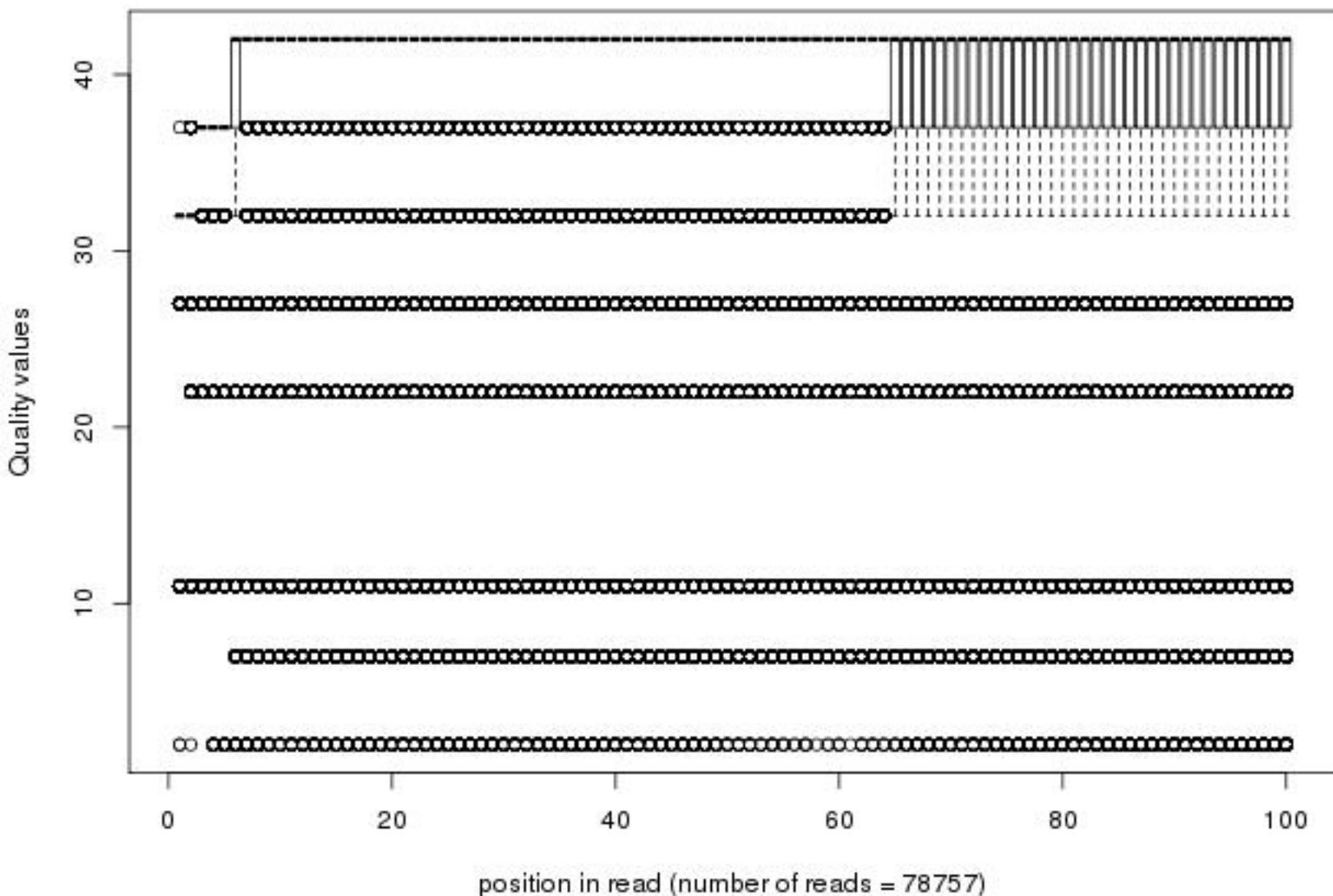
Quality distribution by position in read thp1_cox2_unstim_sc002_01of40_2_frac25
