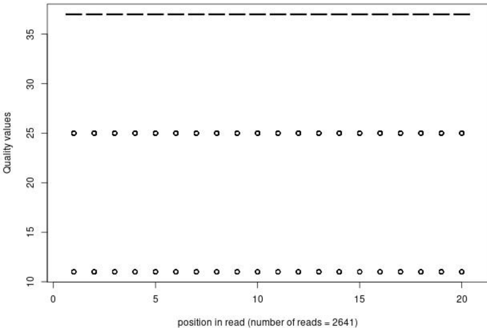
Quality distribution by position in read krab_xx_bmdm_lpsx_av025_L1_1_frac10000
