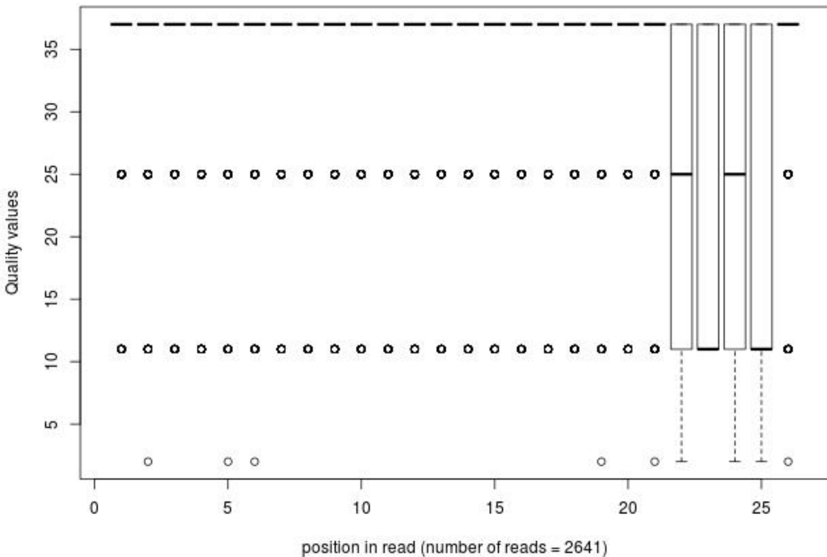
Quality distribution by position in read krab_xx_bmdm_lpsx_av025_L1_2_frac10000
