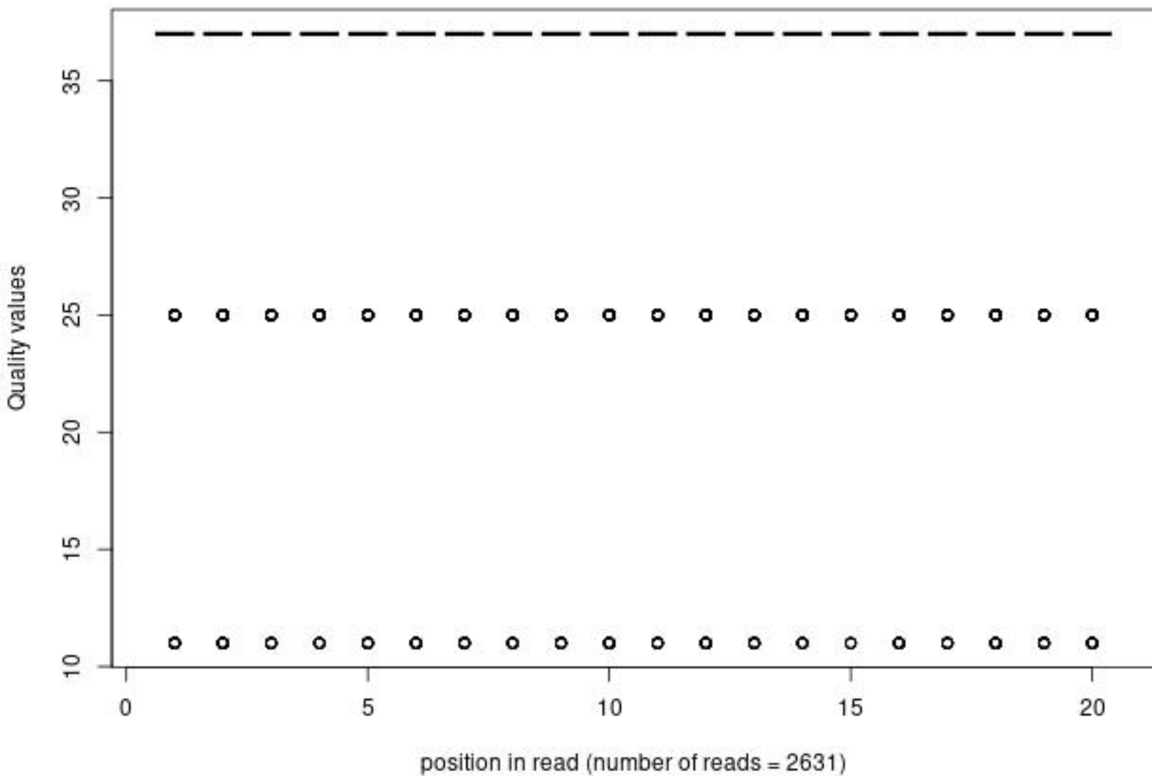
Quality distribution by position in read krab_xx_bmdm_lpsx_av025_L2_1_frac10000
