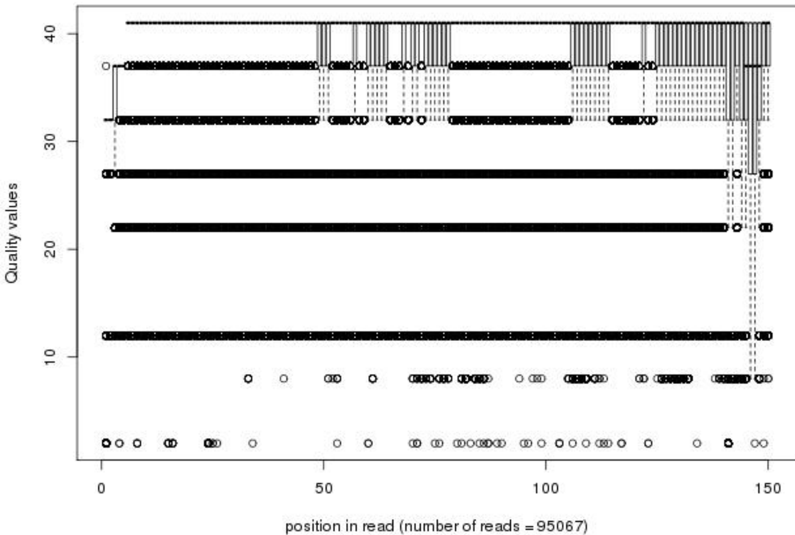
Quality distribution by position in read krab_wt_bmdm_lowx_av024_01of20_2_frac50
