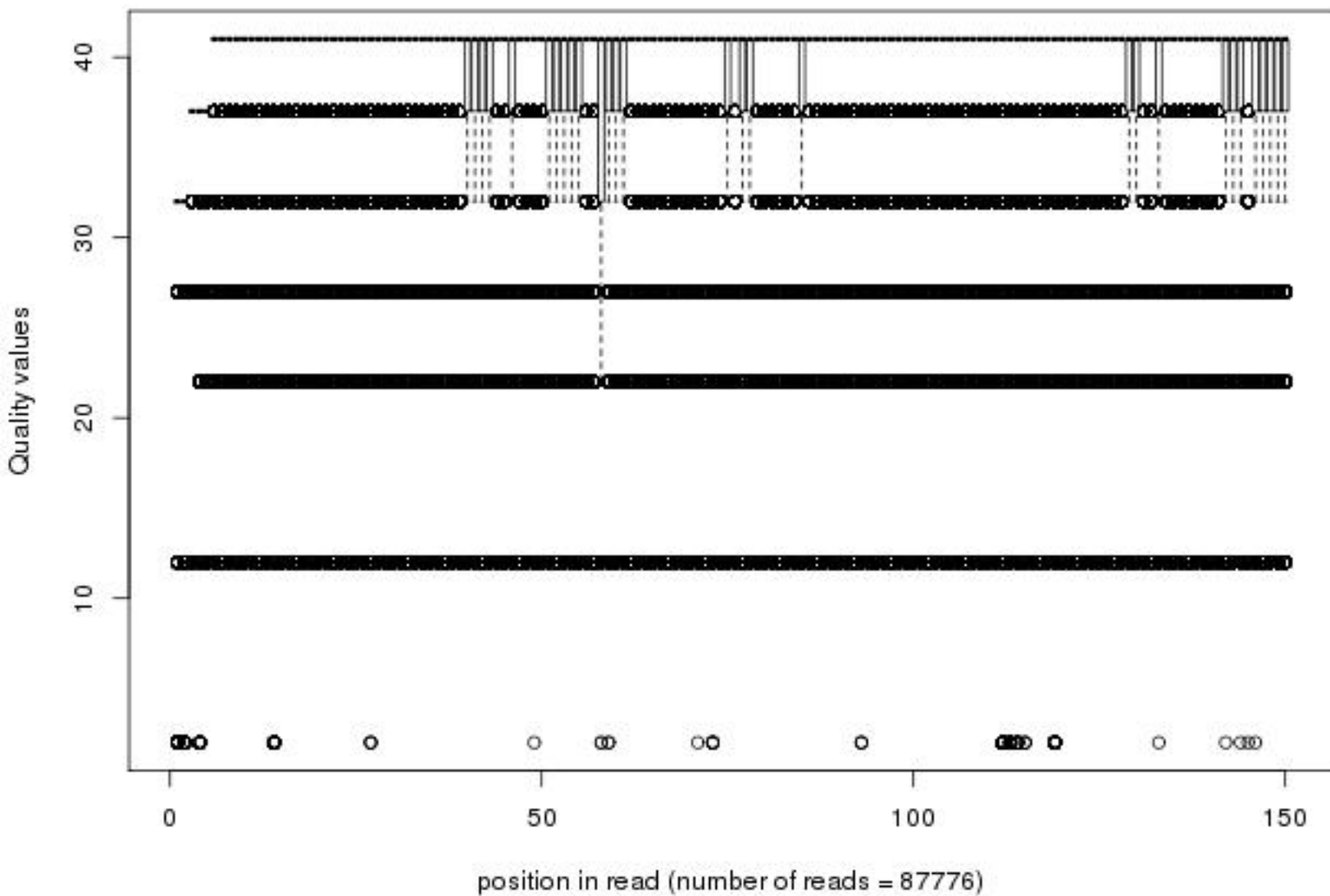
Quality distribution by position in read krab_wt_bmdm_high_av023_01of20_1_frac50
