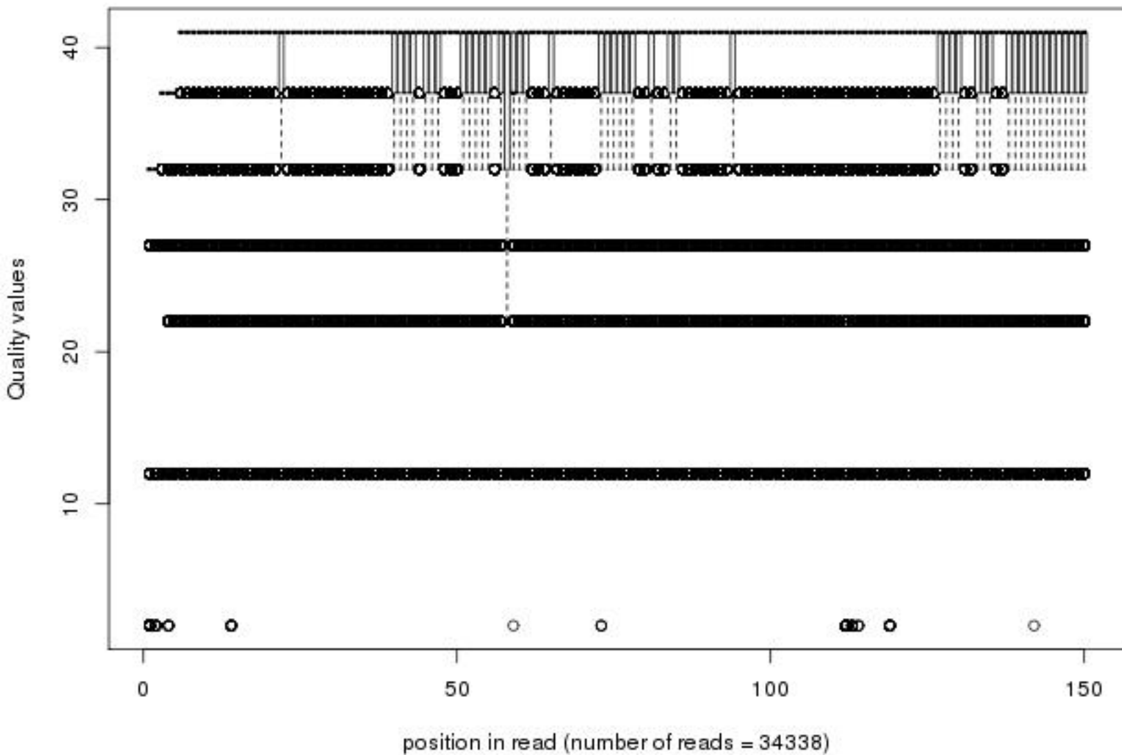
Quality distribution by position in read krab_xx_bmdm_lpsx_av025_01of20_1_frac50
