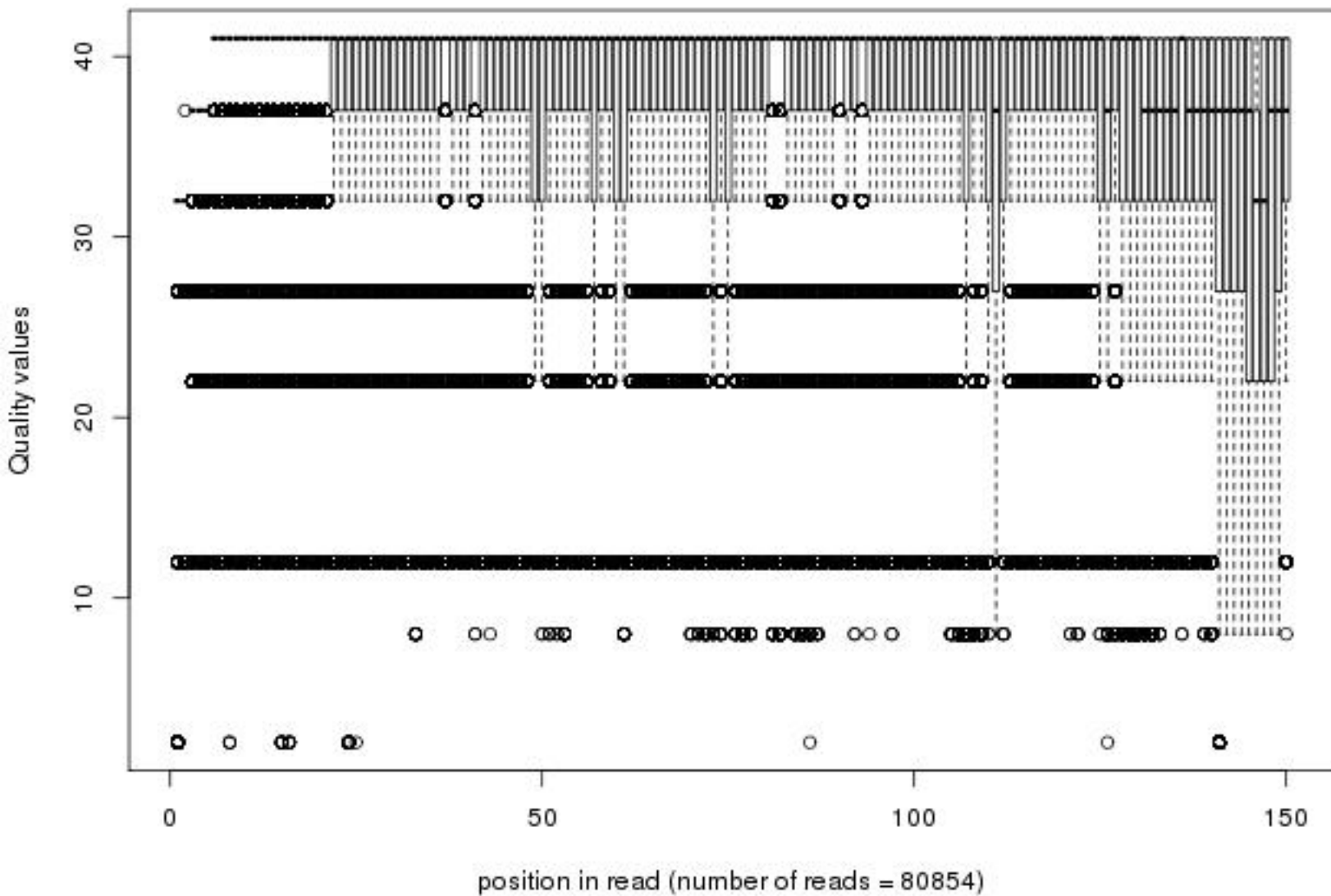
Quality distribution by position in read krab_wt_pmid_base_av021_01of20_2_frac50
