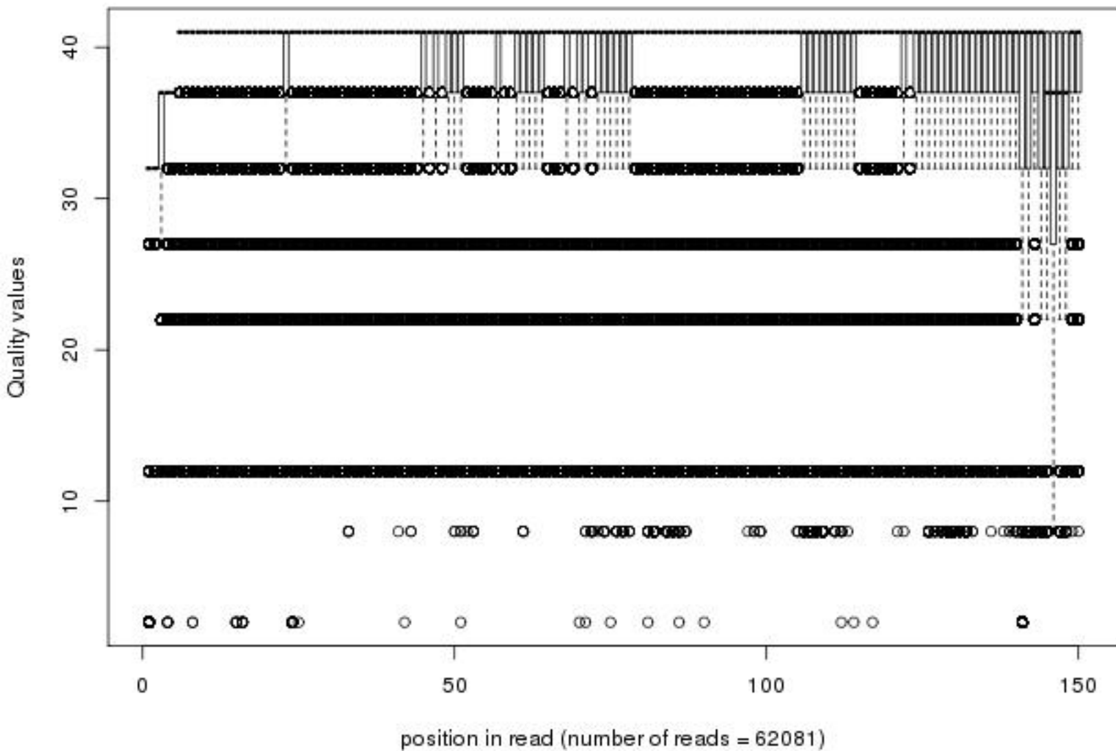
Quality distribution by position in read krab_wt_bmdm_base_av022_01of20_2_frac50
