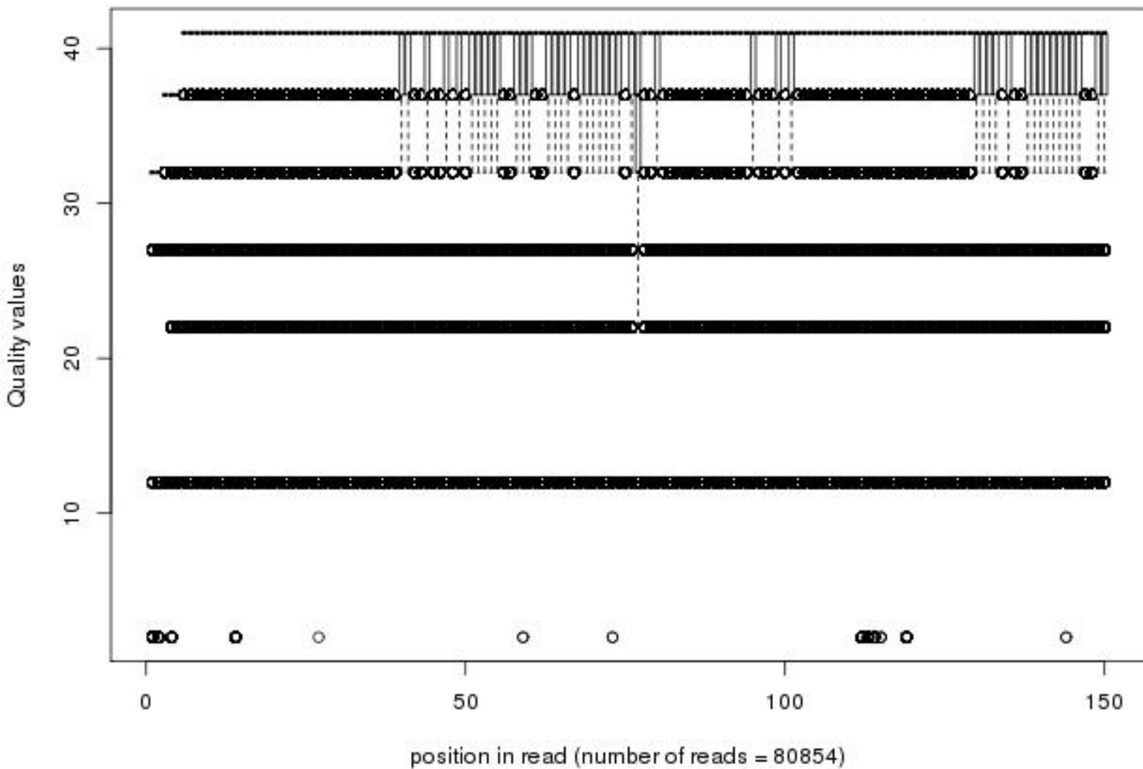
Quality distribution by position in read krab_wt_pmid_base_av021_01of20_1_frac50
