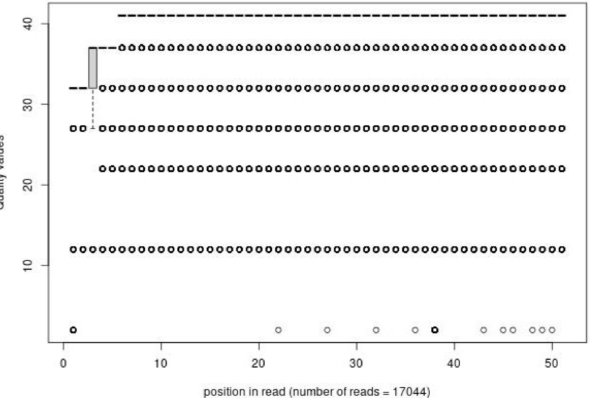
Quality distribution by position in read thp1_gfphi_av063_01of10_1_frac100
