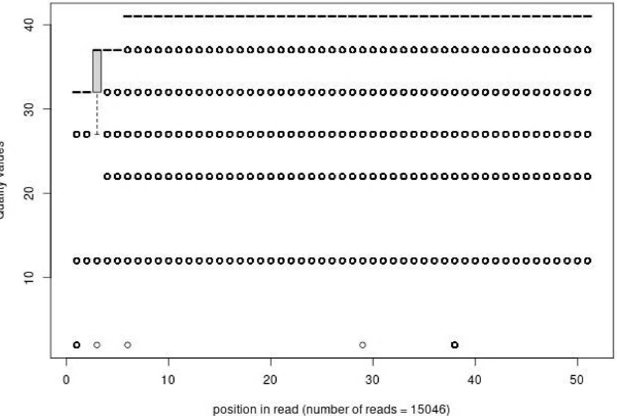
Quality distribution by position in read thp1_gfphi_av061_01of10_1_frac100
