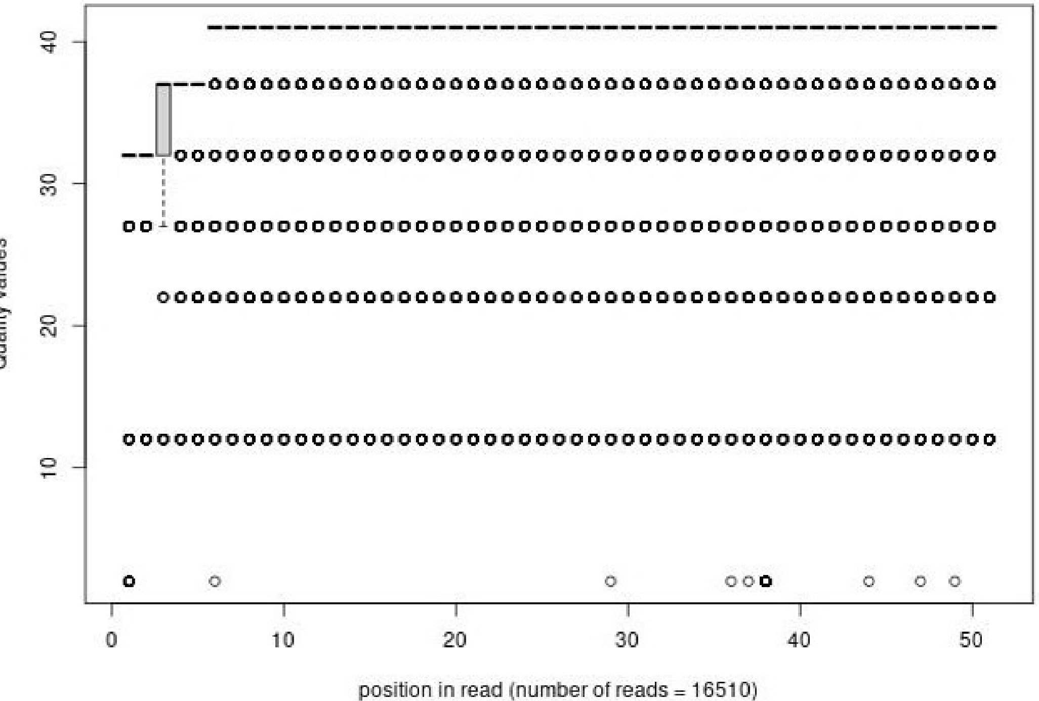
Quality distribution by position in read thp1_gfphi_av059_01of10_1_frac100
