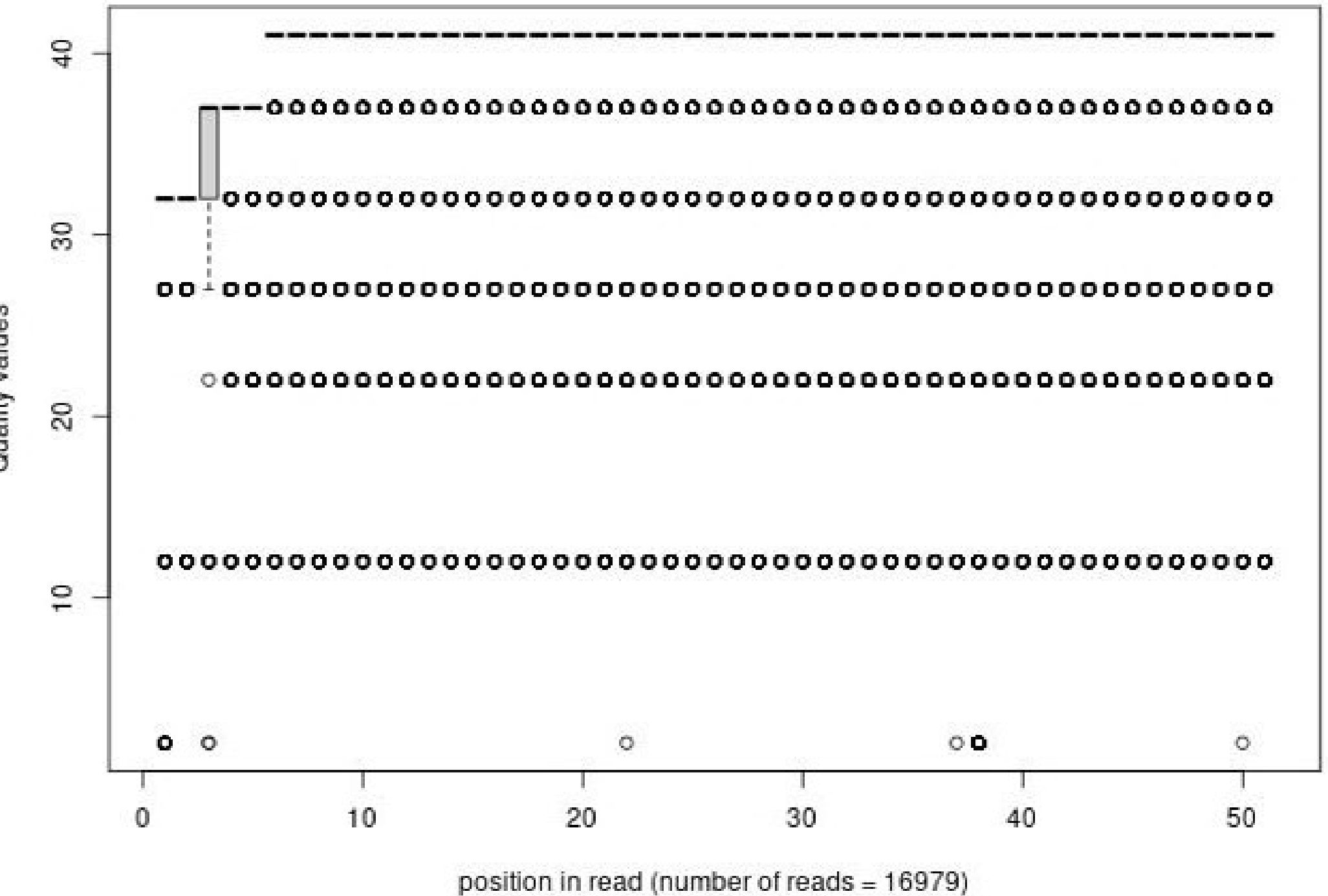
Quality distribution by position in read thp1_gfplo_av058_01of10_1_frac100
