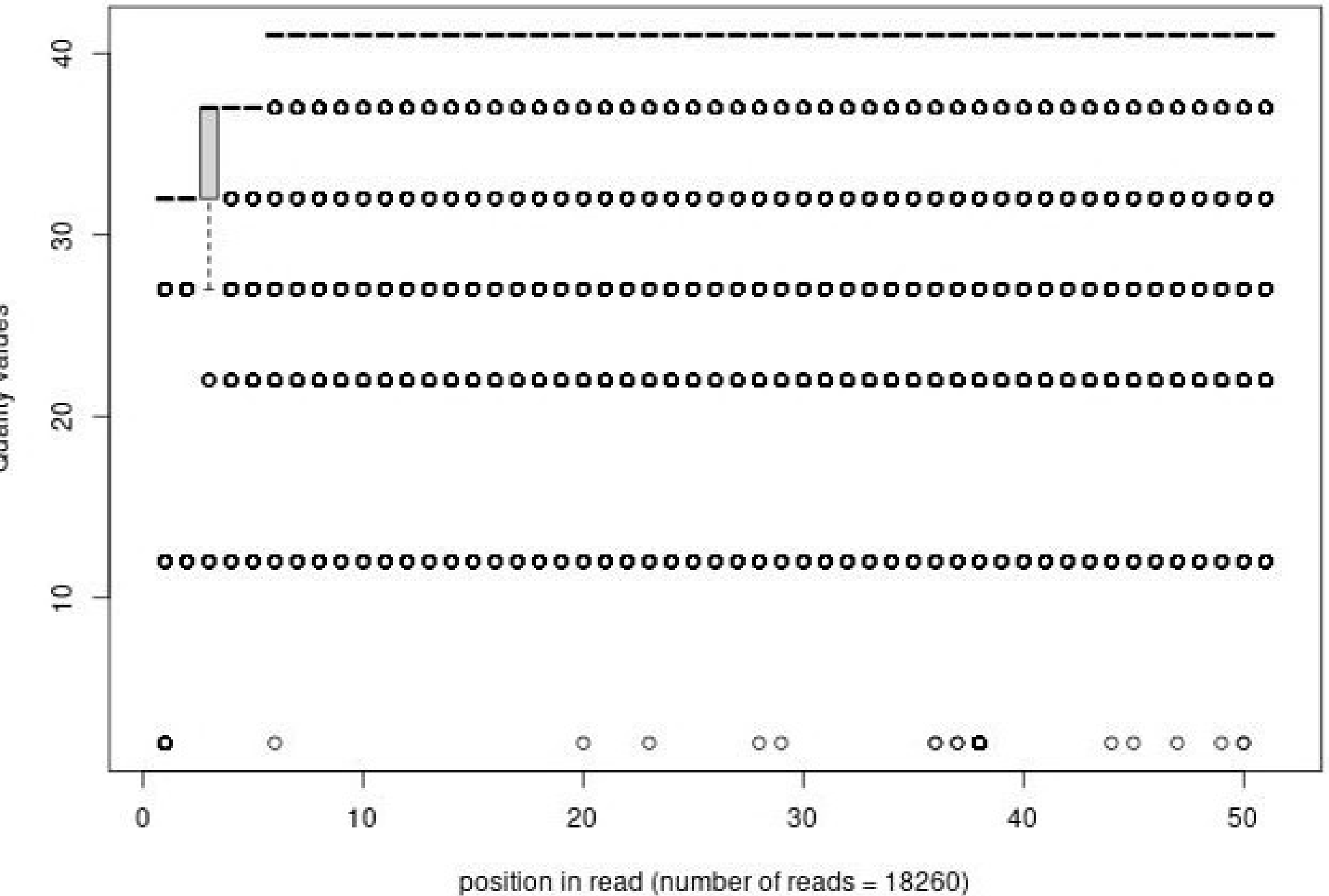
Quality distribution by position in read thp1_gfplo_av060_01of10_1_frac100
