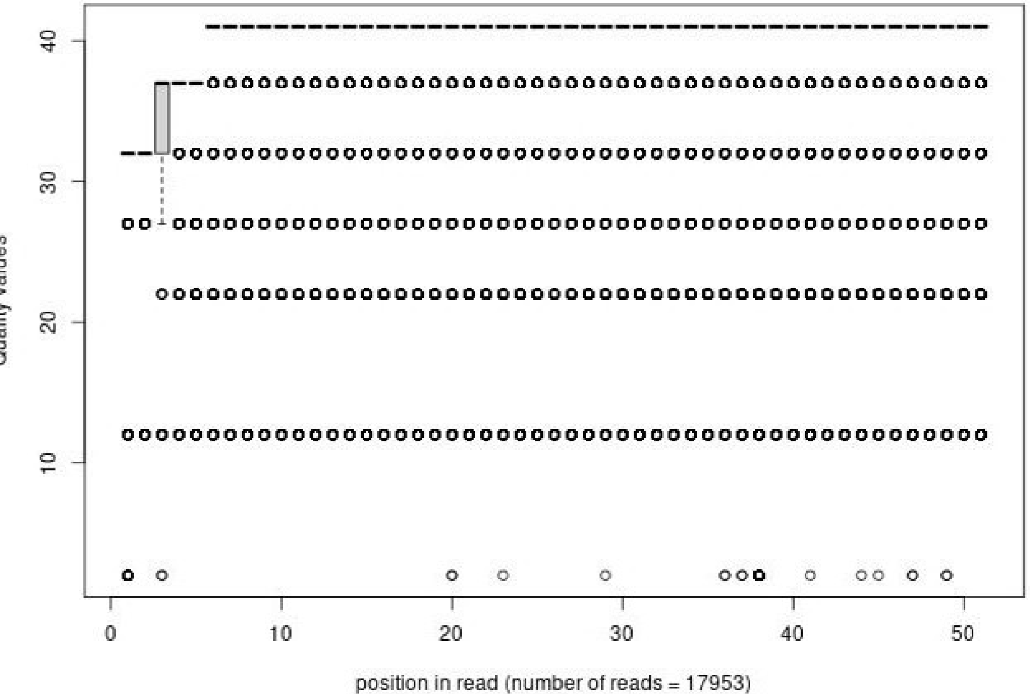
Quality distribution by position in read thp1_gfplo_av062_01of10_1_frac100
