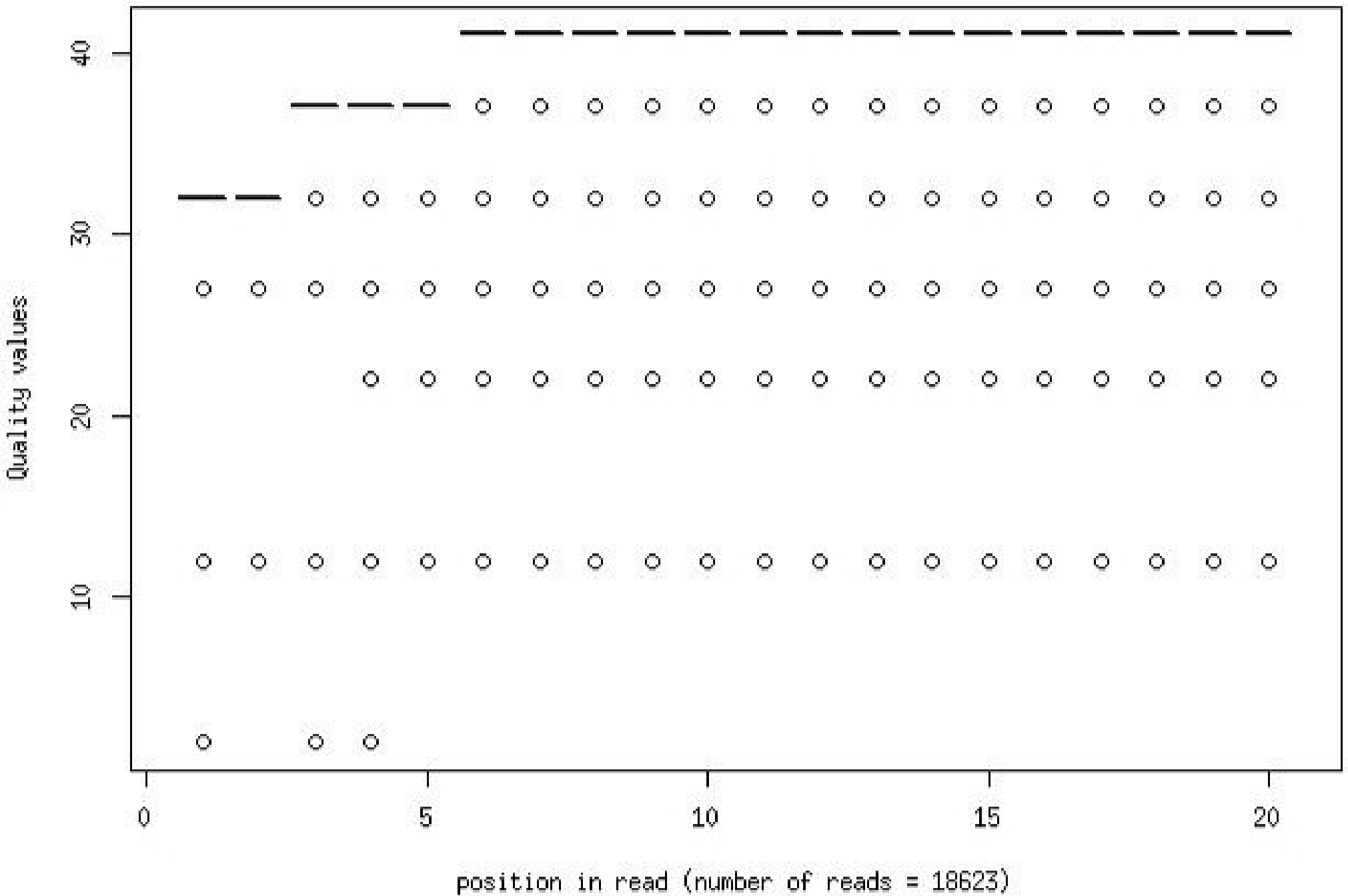
Quality distribution by position in read bmdm_ifn_tbi_chrh_sc10_qrn0L4_1_frac1000
