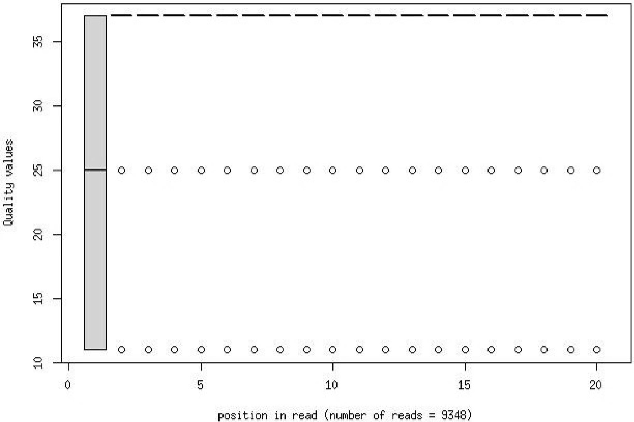
Quality distribution by position in read bmdm_plasmid_ntrt_ms01_drn1L1_1_frac1000
