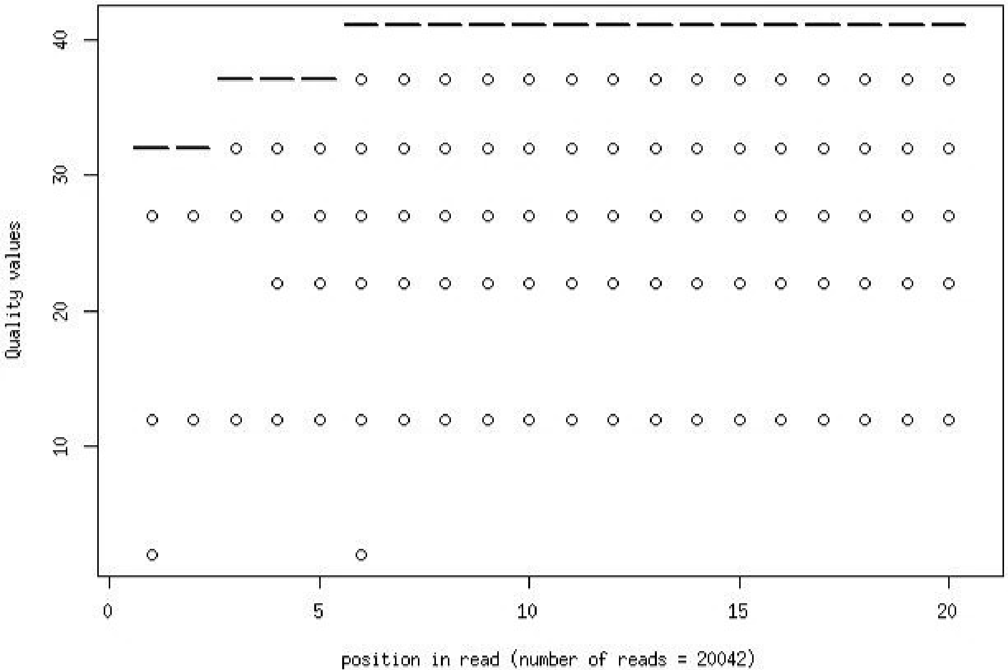
Quality distribution by position in read bmdm_day21xx_ntrt_sc04_qrn0L4_1_frac1000
