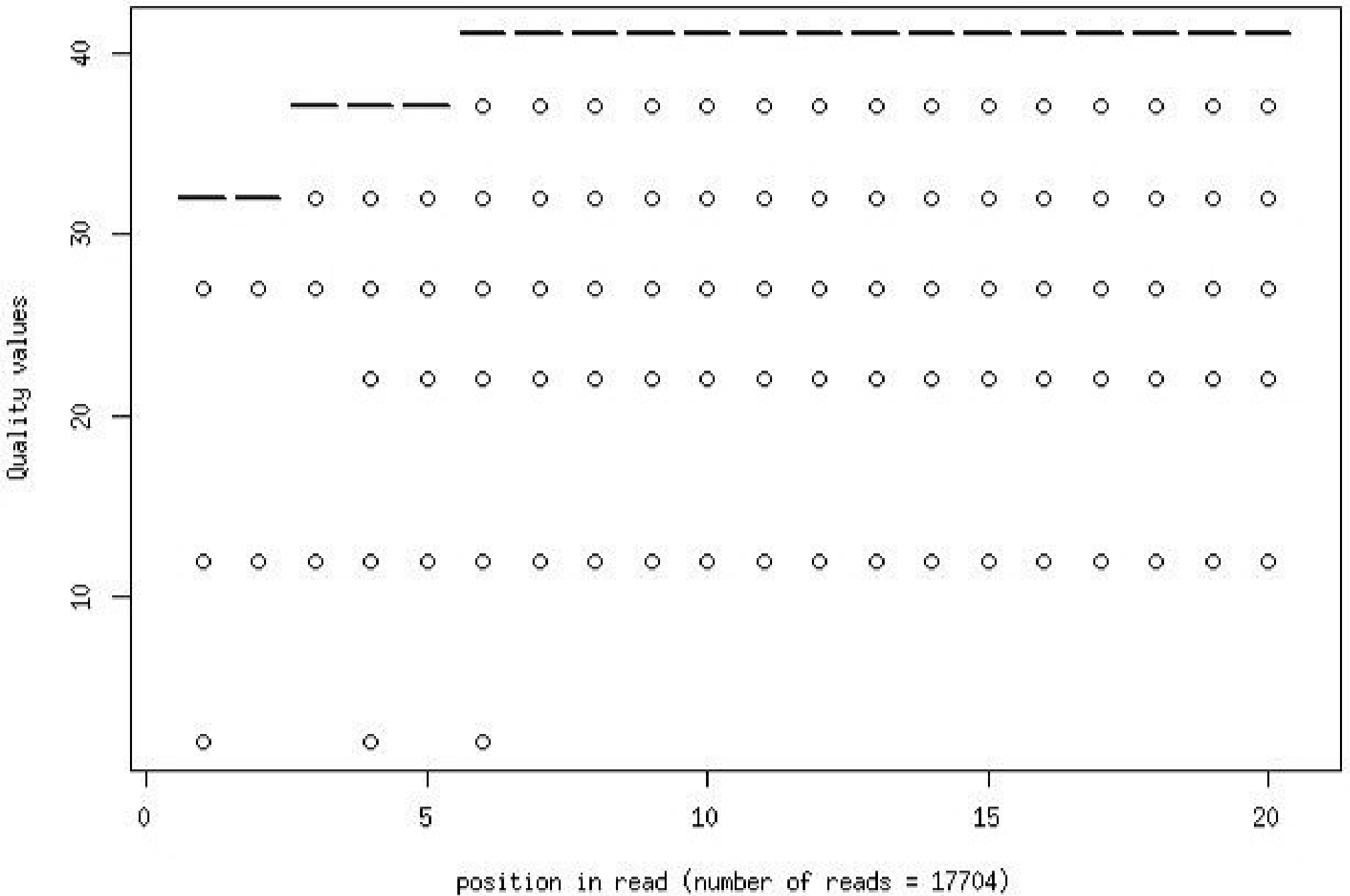
Quality distribution by position in read bmdm_necropt_xxxx_sc06_qrn0L4_1_frac1000
