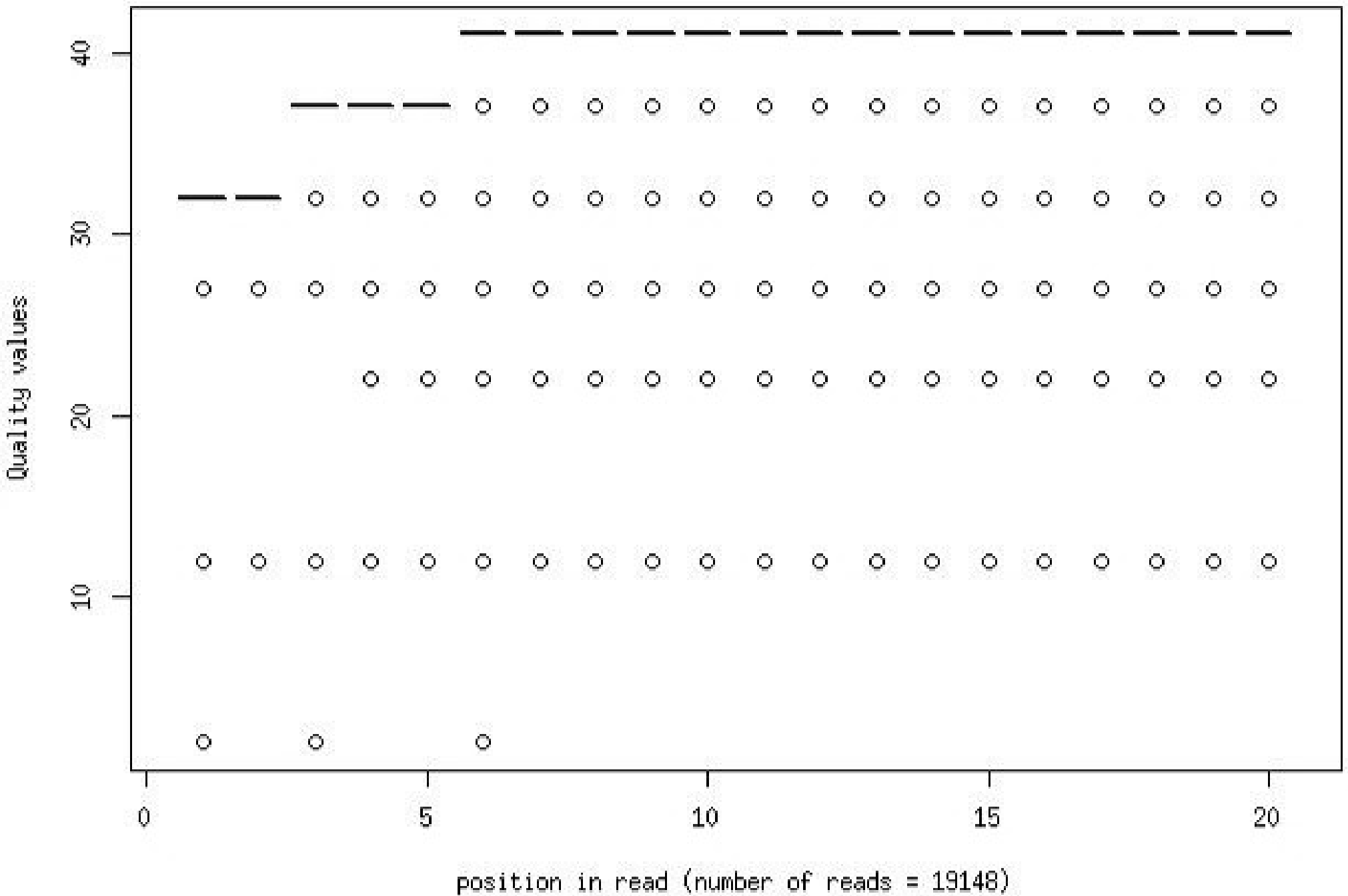
Quality distribution by position in read bmdm_necropt_xxxx_sc07_qrn0L4_1_frac1000
