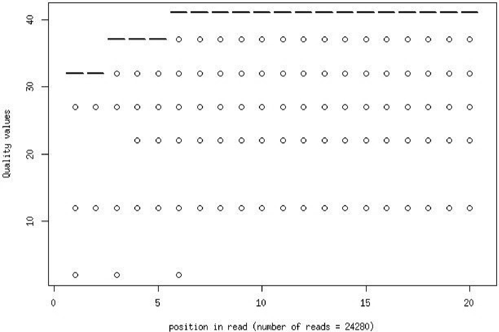
Quality distribution by position in read bmdm_day03xx_ntrt_sc02_qrn0L4_1_frac1000
