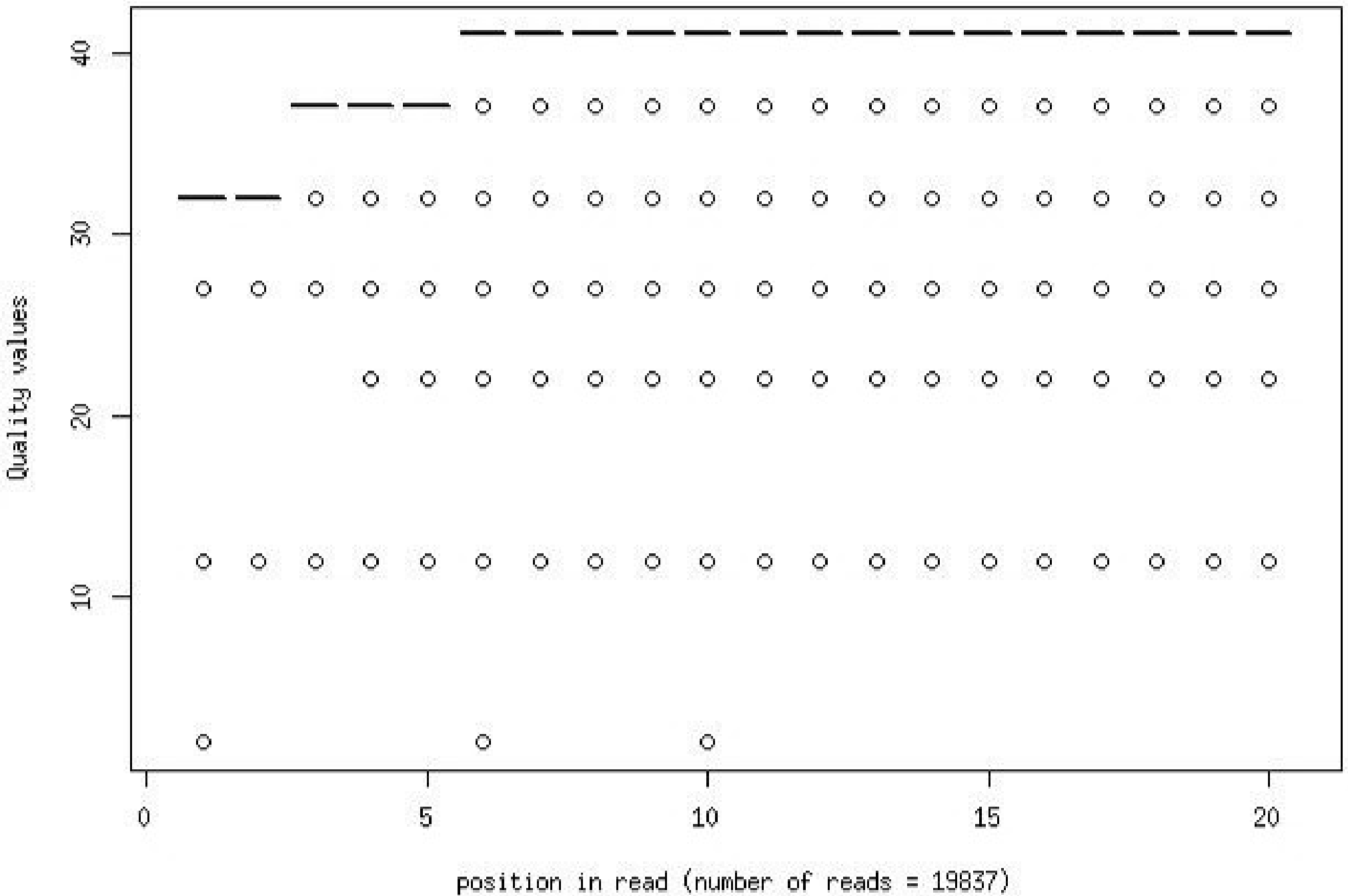
Quality distribution by position in read bmdm_ifn_tbi_chrh_sc11_qrn0L4_1_frac1000
