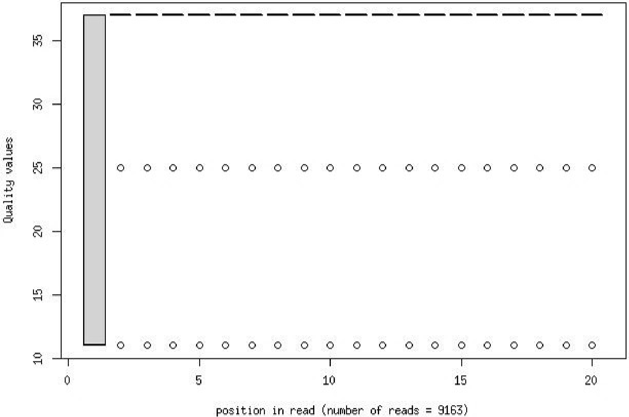
Quality distribution by position in read bmdm_plasmid_ntrt_ms01_drn1L2_1_frac1000
