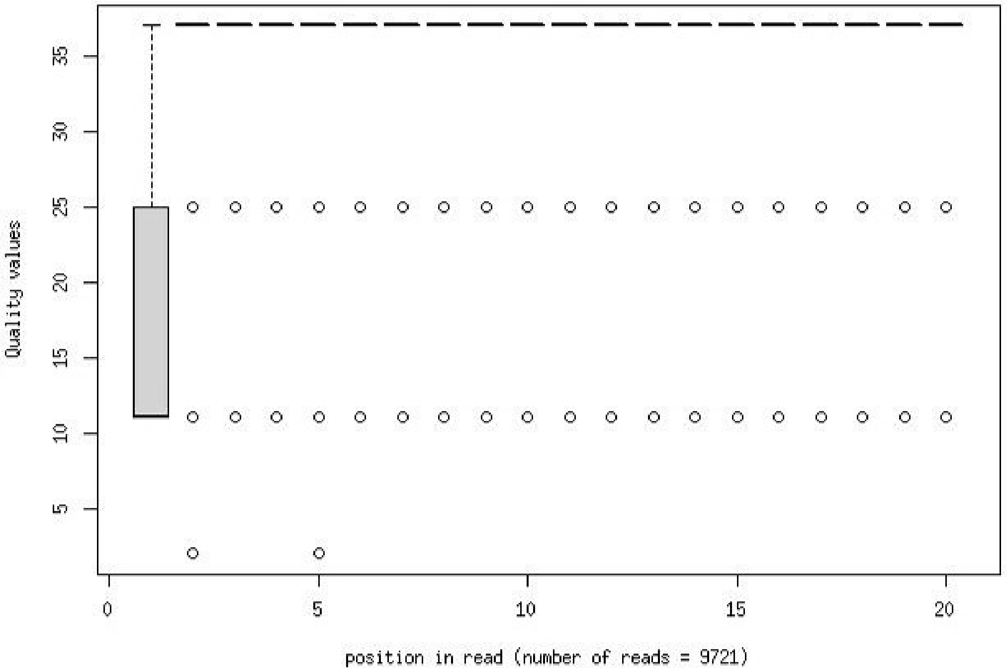
Quality distribution by position in read bmdm_plasmid_ntrt_ms01_drn2L2_1_frac1000
