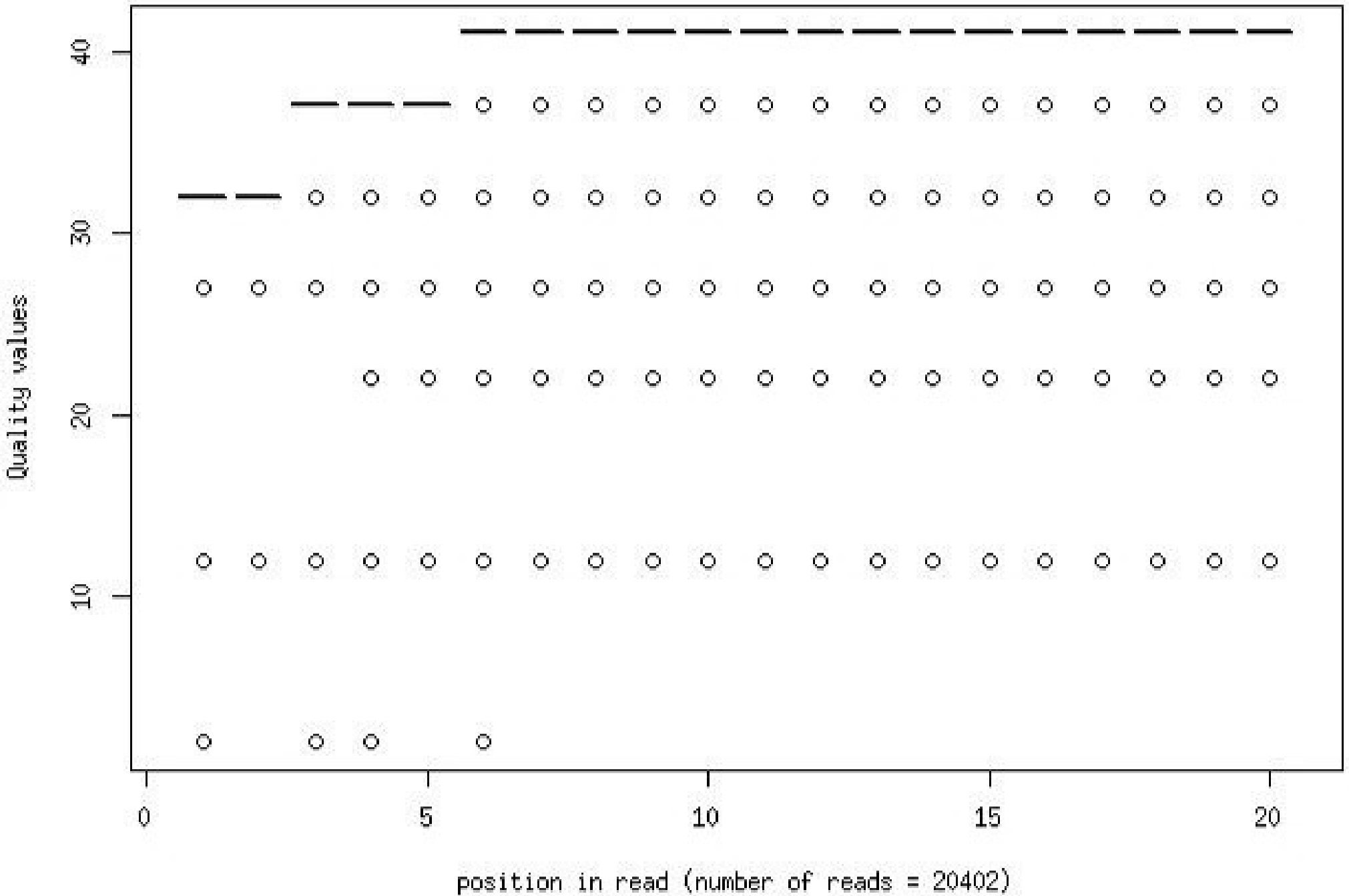
Quality distribution by position in read bmdm_ifn_ntb_xxxx_sc08_qrn0L4_1_frac1000
