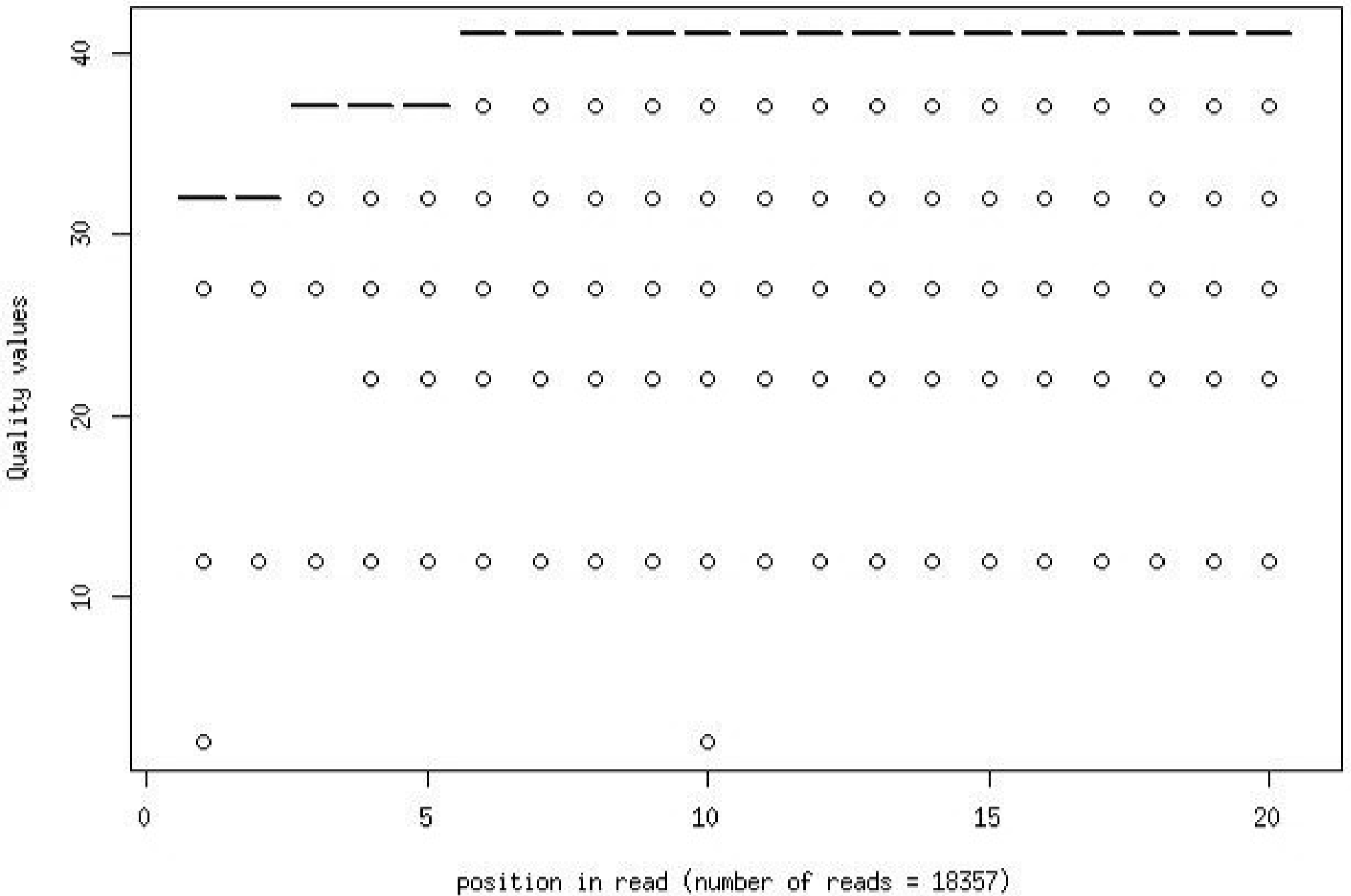
Quality distribution by position in read bmdm_plasmid_ntrt_sc01_qrn0L4_1_frac1000
