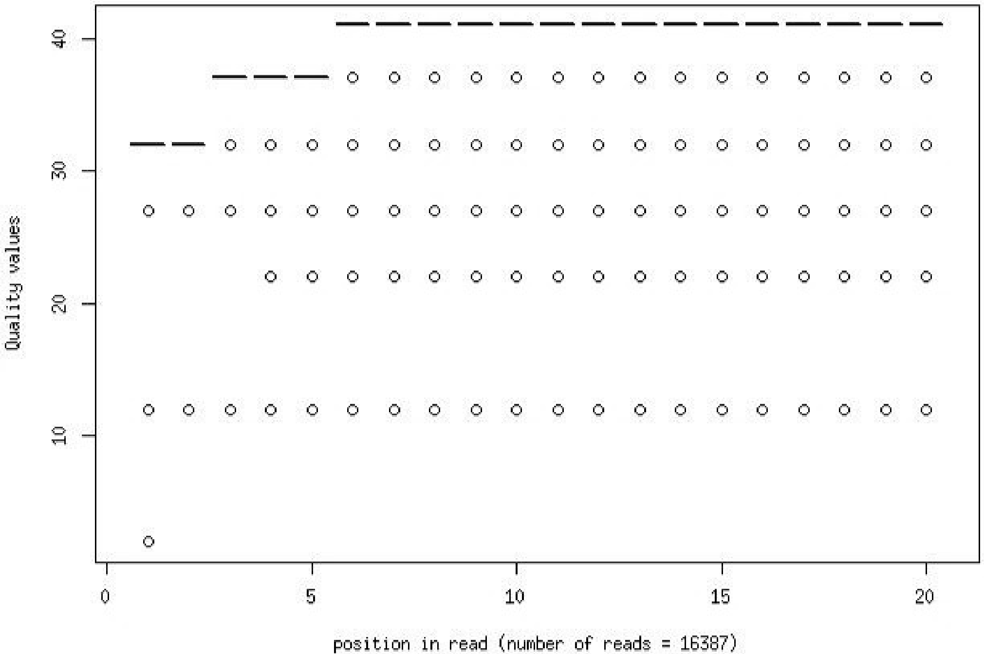
Quality distribution by position in read bmdm_day21xx_ntrt_sc05_qrn0L4_1_frac1000
