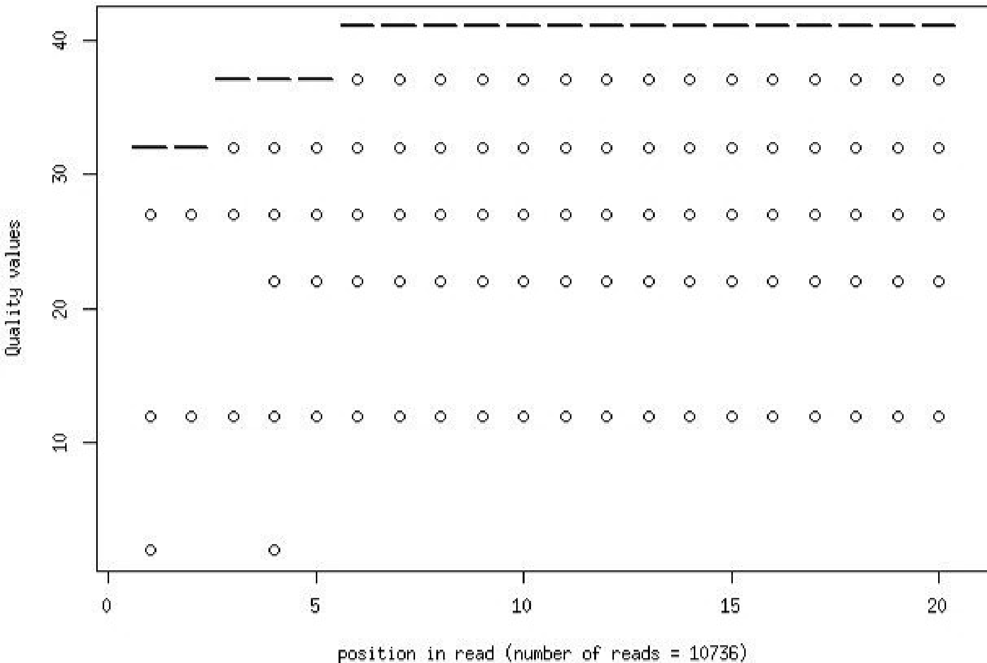
Quality distribution by position in read bmdm_plasmid_ntrt_ms01_qrn0L3_1_frac1000
