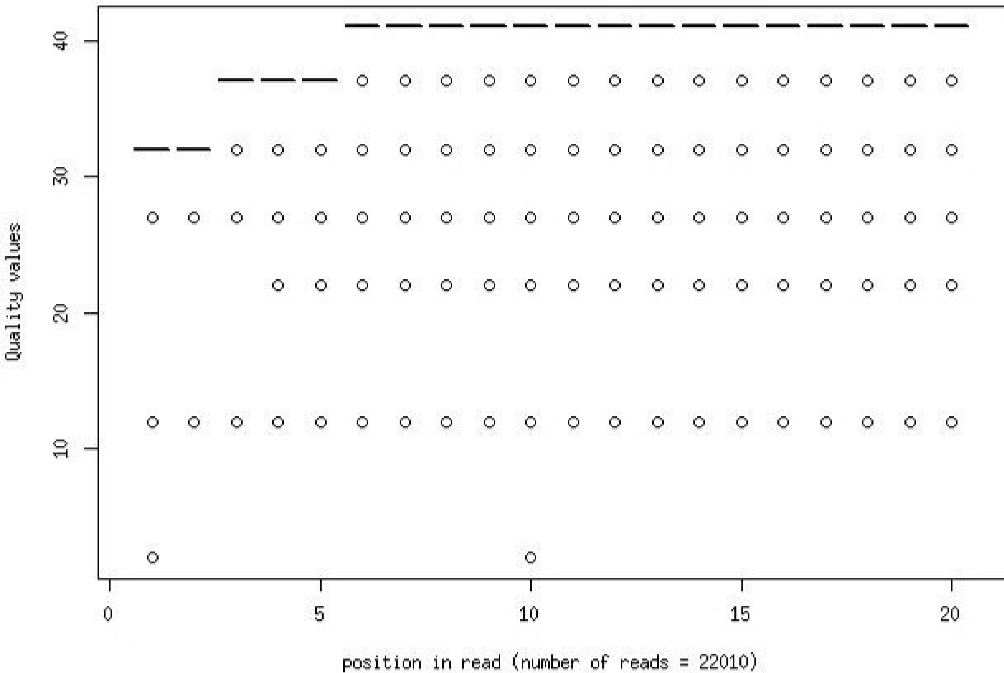
Quality distribution by position in read bmdm_ifn_ntb_xxxx_sc09_qrn0L4_1_frac1000
