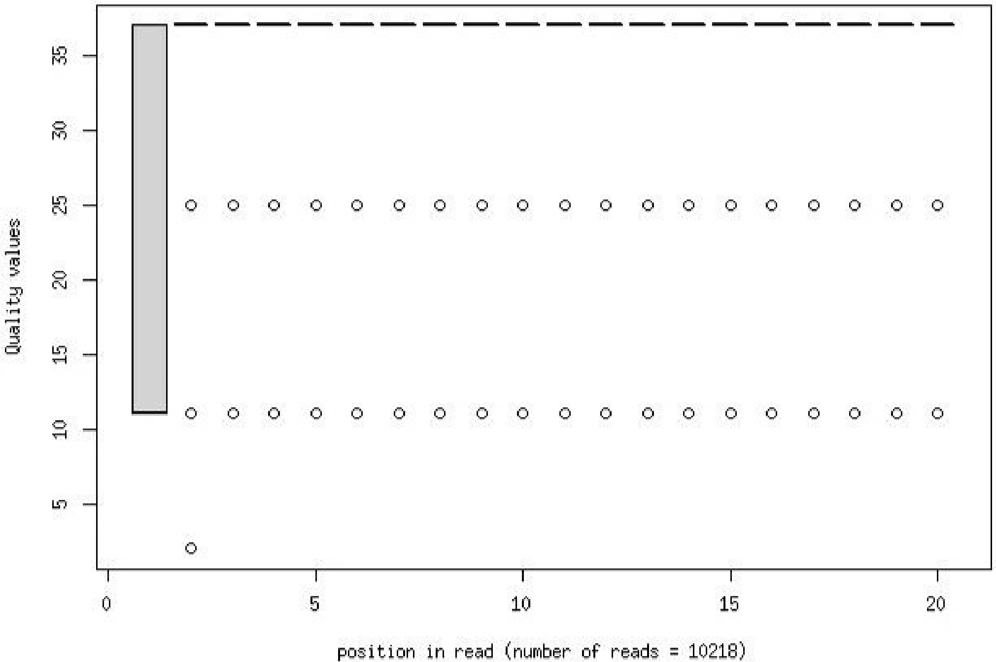
Quality distribution by position in read bmdm_plasmid_ntrt_ms01_drn2L1_1_frac1000
