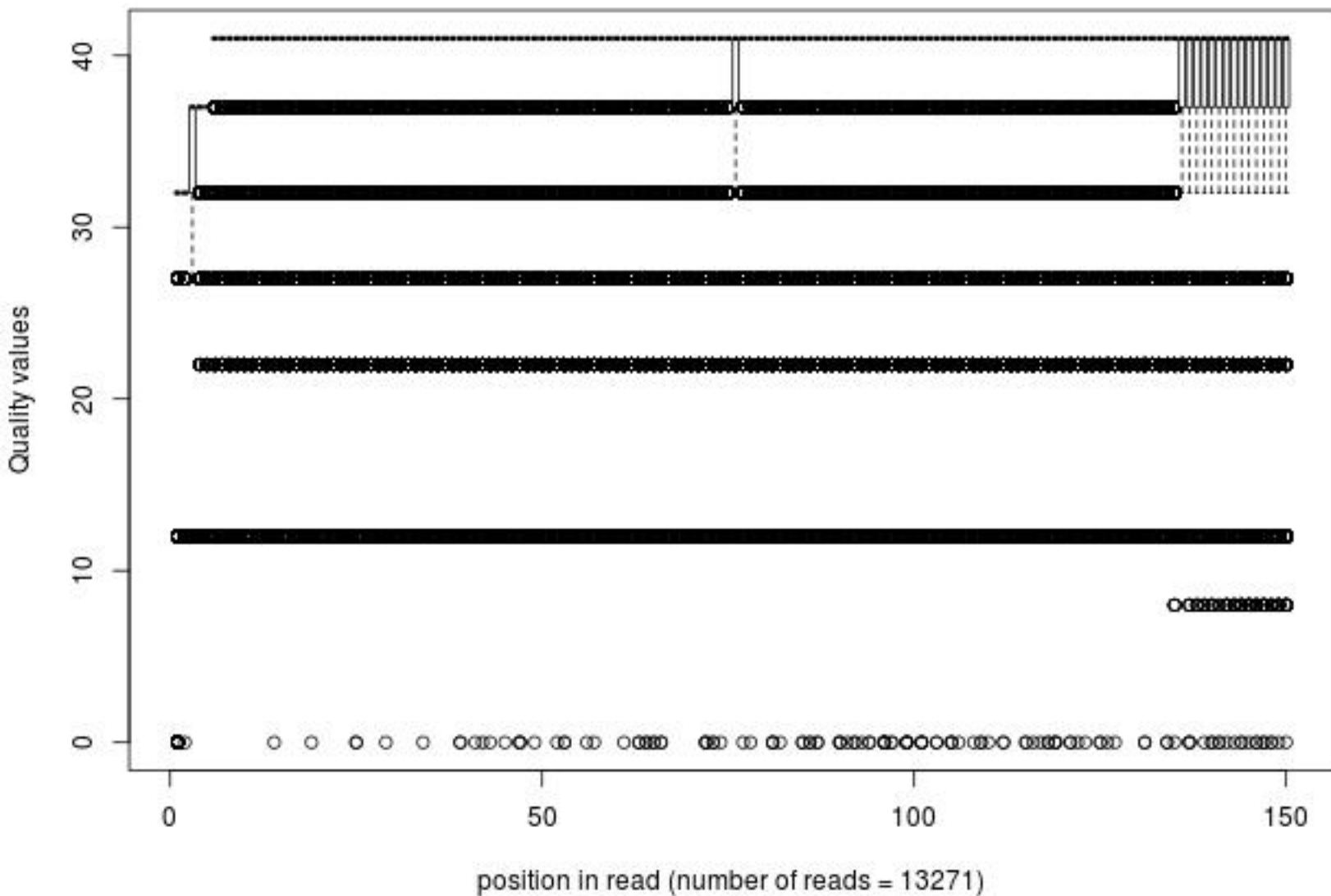
Quality distribution by position in read hek_bens_em_fg029_01of10_1_frac1000_pad150
