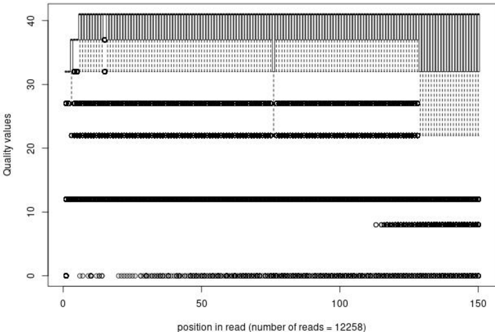
Quality distribution by position in read hek_untr_em_fg028_01of10_2_frac1000_pad150
