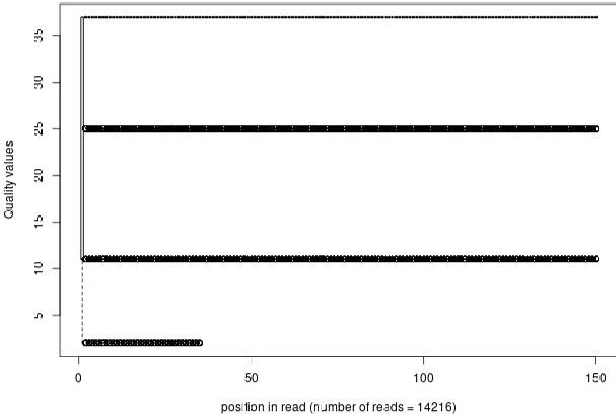
Quality distribution by position in read scer_hu_thailahi_oh028_01of10_1_frac1000_pad150
