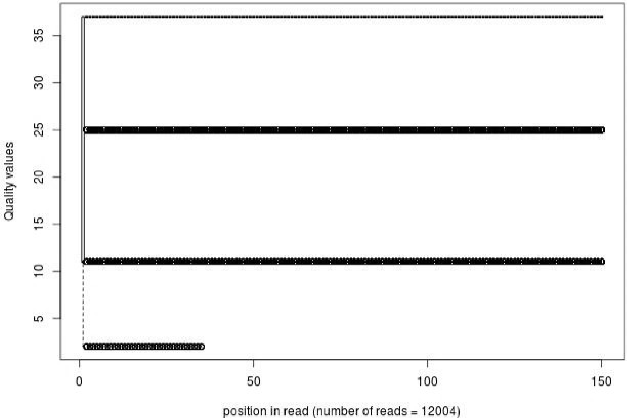
Quality distribution by position in read scer_hu_drugnone_oh025_01of10_1_frac1000_pad150
