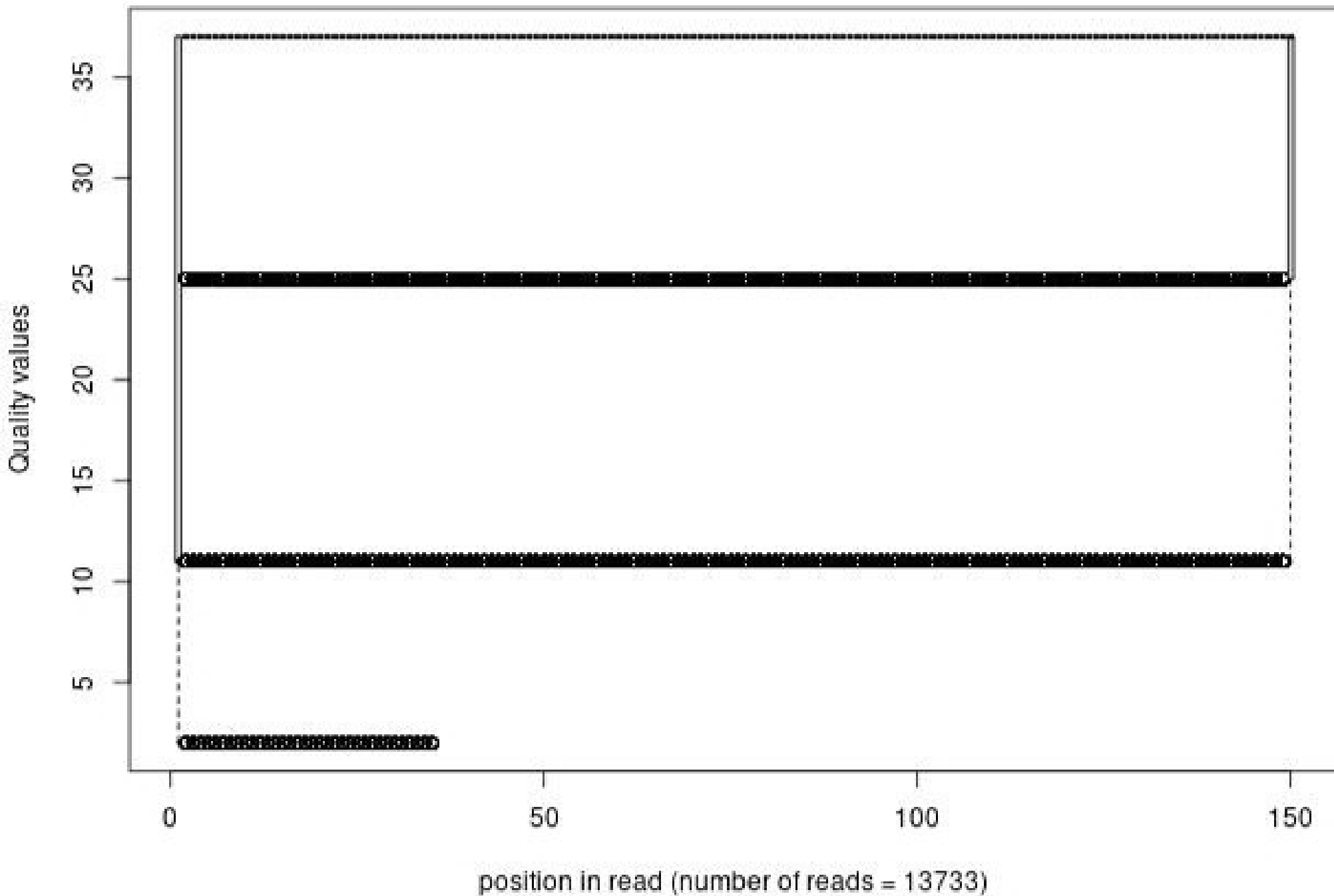
Quality distribution by position in read scer_hu_pladbxlo_oh033_01of10_1_frac1000_pad150
