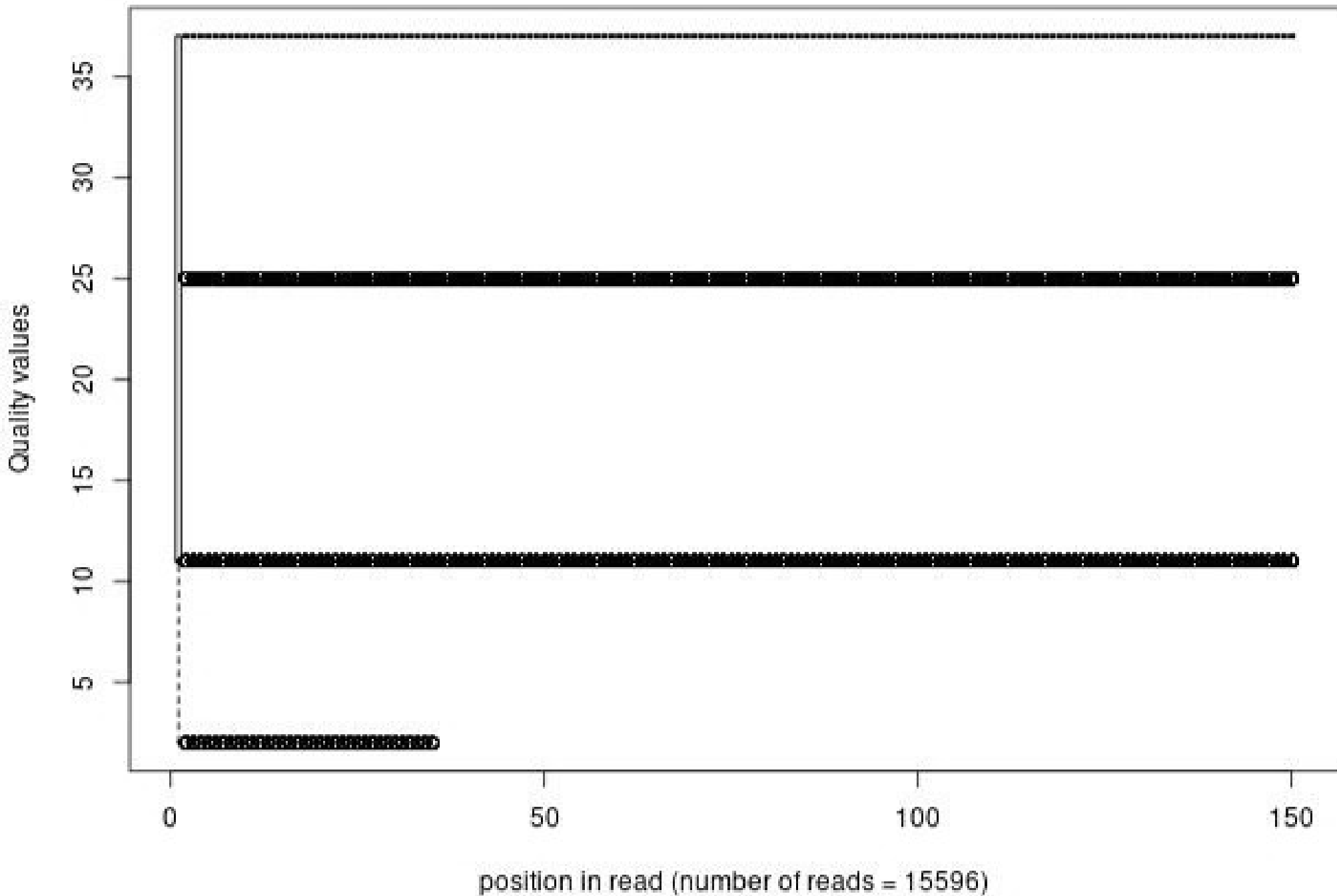
Quality distribution by position in read scer_wt_pladbxhi_oh030_01of10_1_frac1000_pad150
