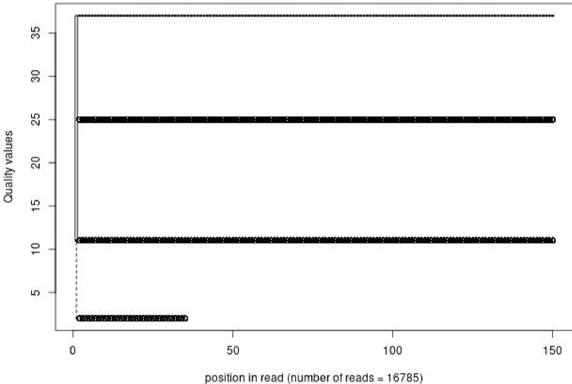
Quality distribution by position in read scer_hu_pladbxhi_oh026_01of10_1_frac1000_pad150
