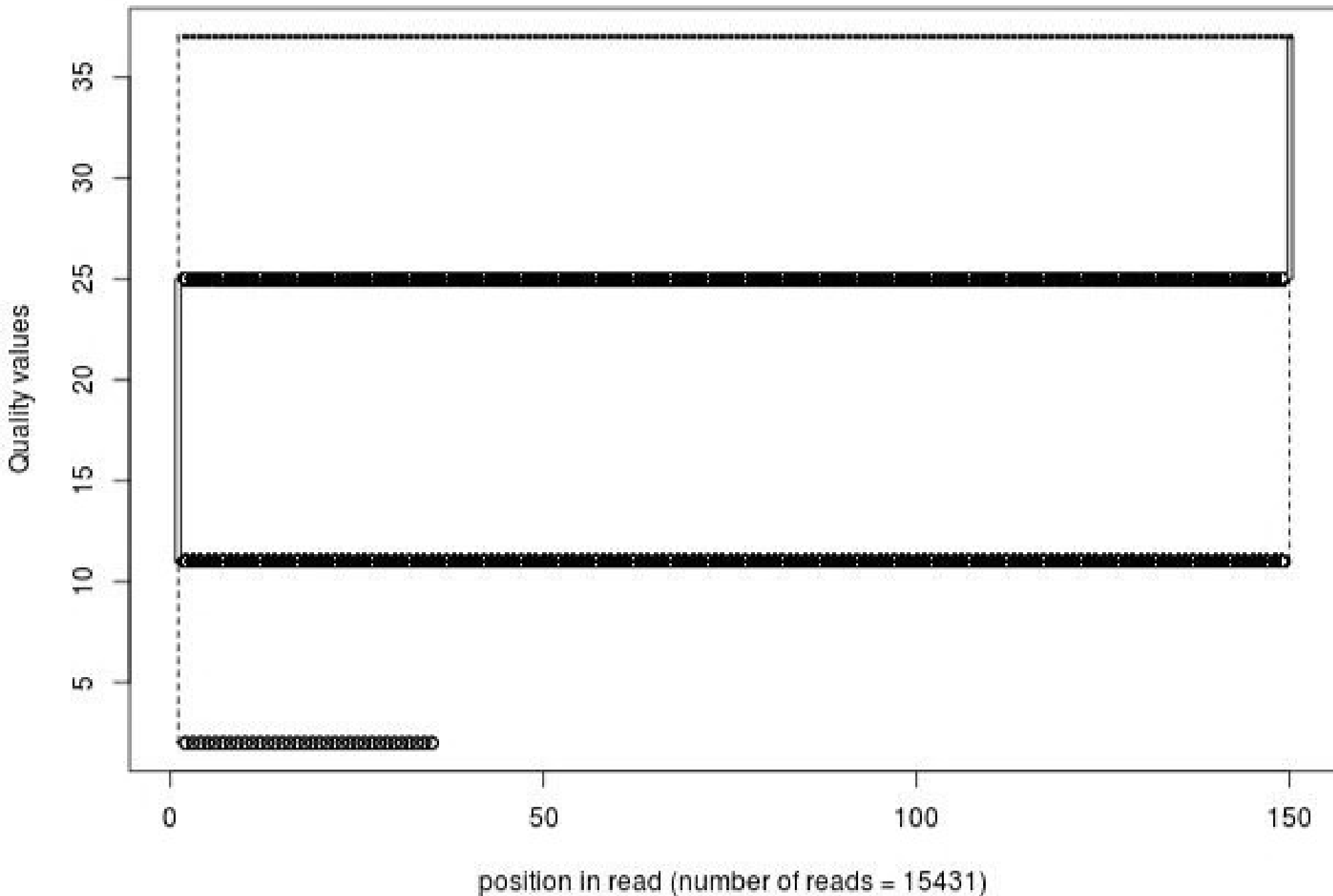
Quality distribution by position in read scer_hu_drugnone_oh031_01of10_2_frac1000_pad150
