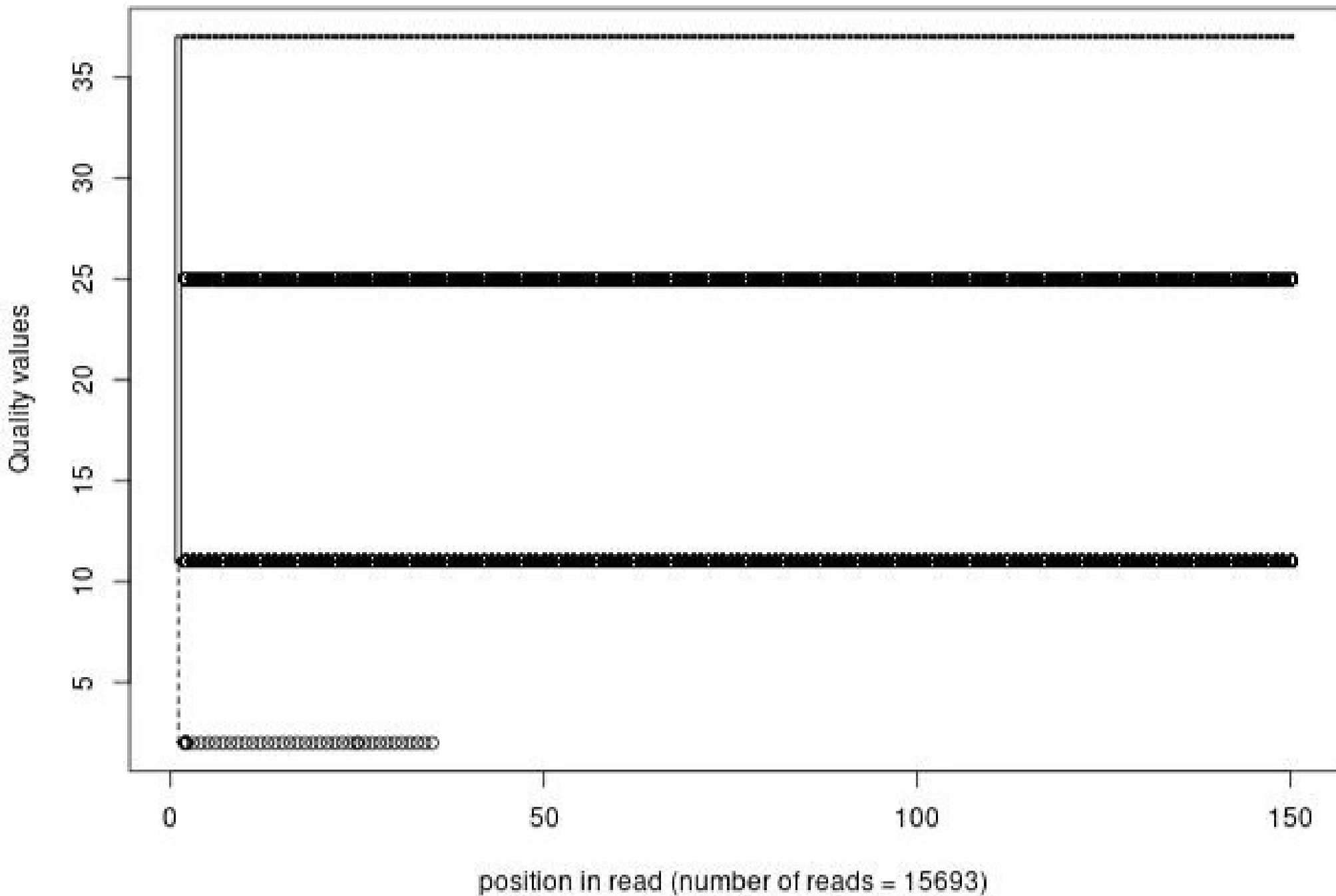
Quality distribution by position in read scer_hu_pladbxlo_oh027_01of10_1_frac1000_pad150
