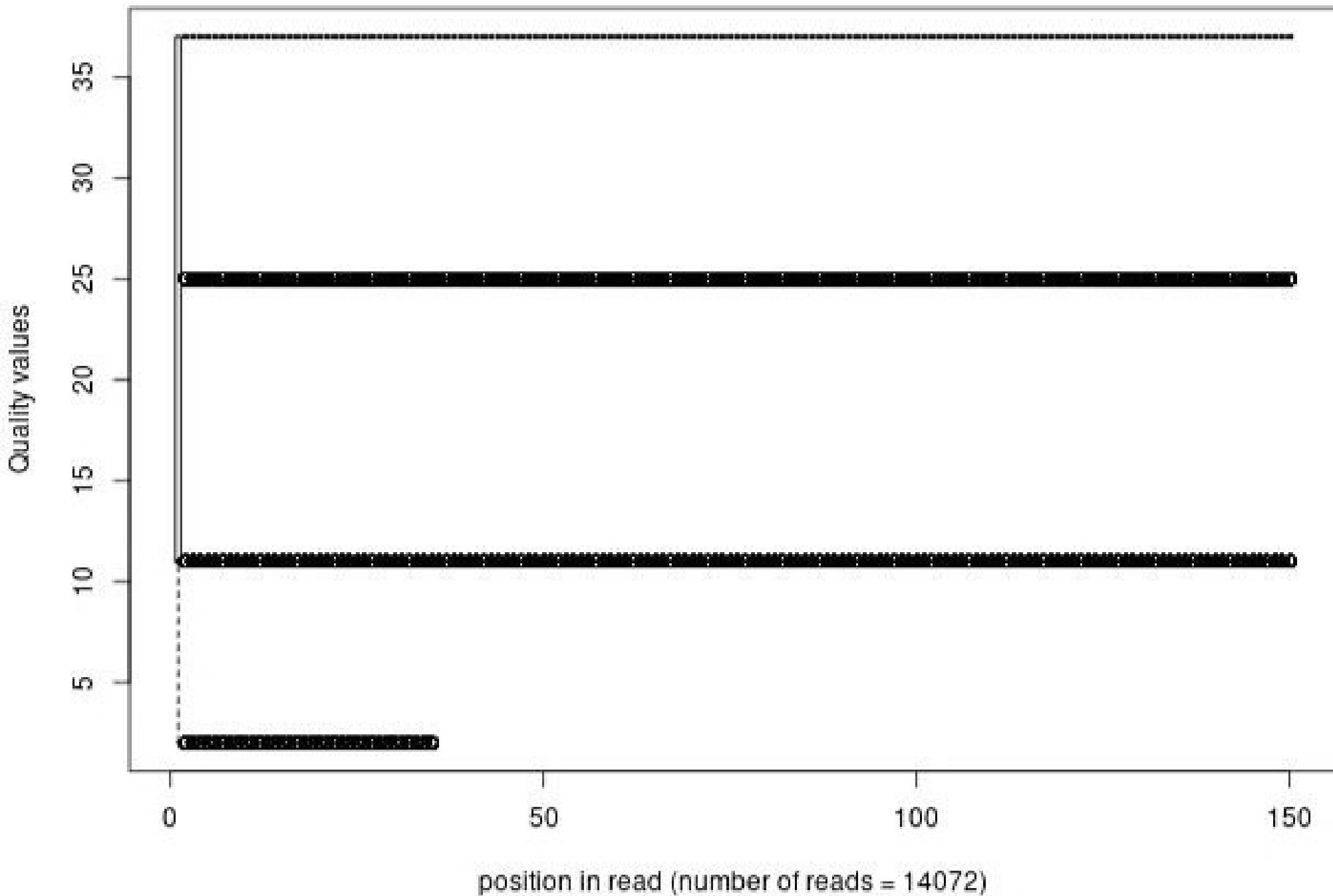
Quality distribution by position in read scer_hu_thailahi_oh034_01of10_1_frac1000_pad150
