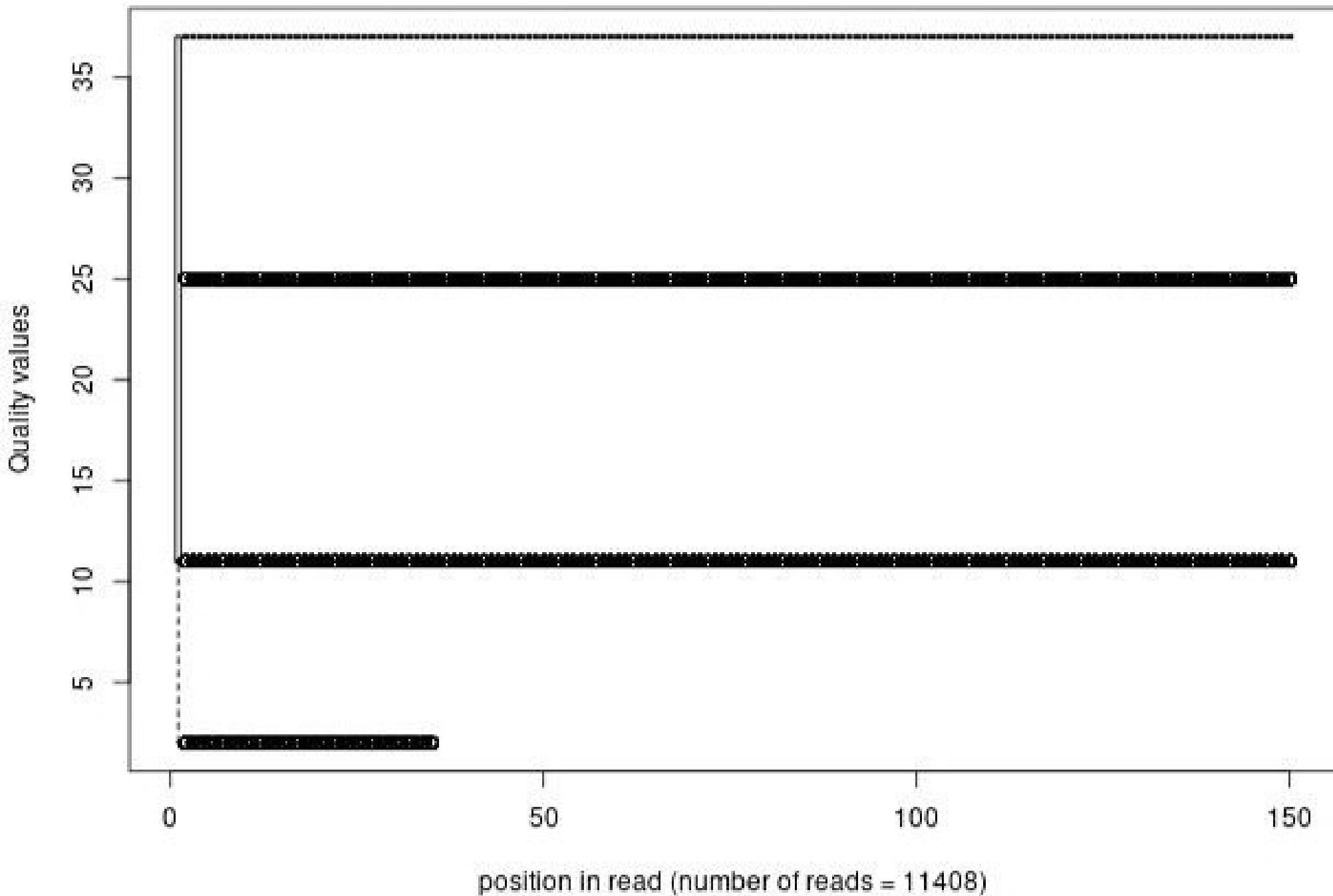
Quality distribution by position in read scer_wt_drugnone_oh035_01of10_1_frac1000_pad150
