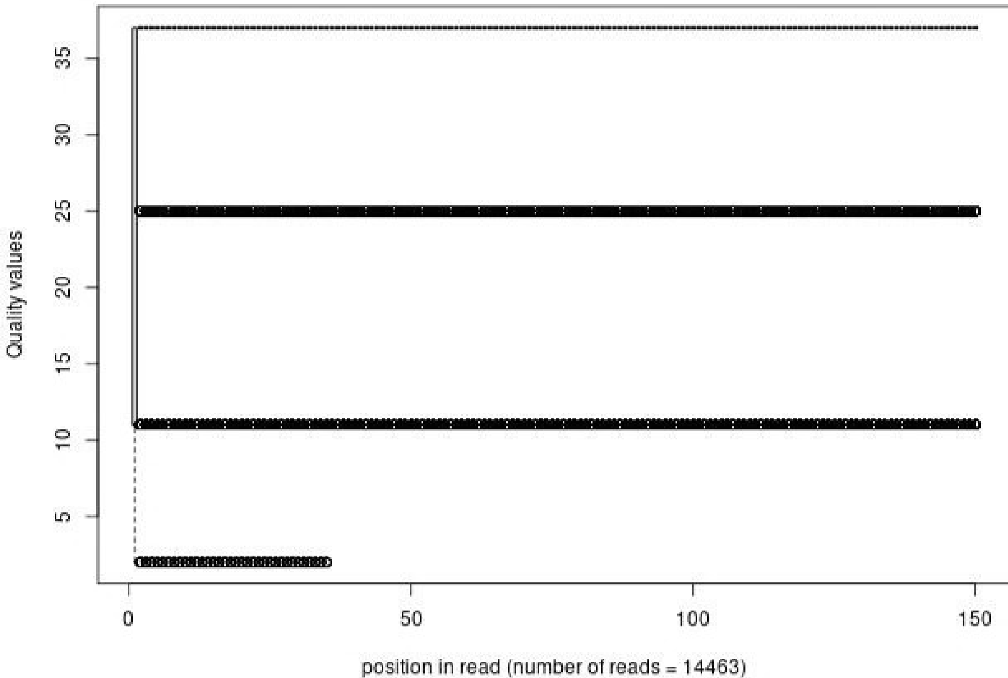
Quality distribution by position in read scer_hu_pladbxhi_oh032_01of10_1_frac1000_pad150
