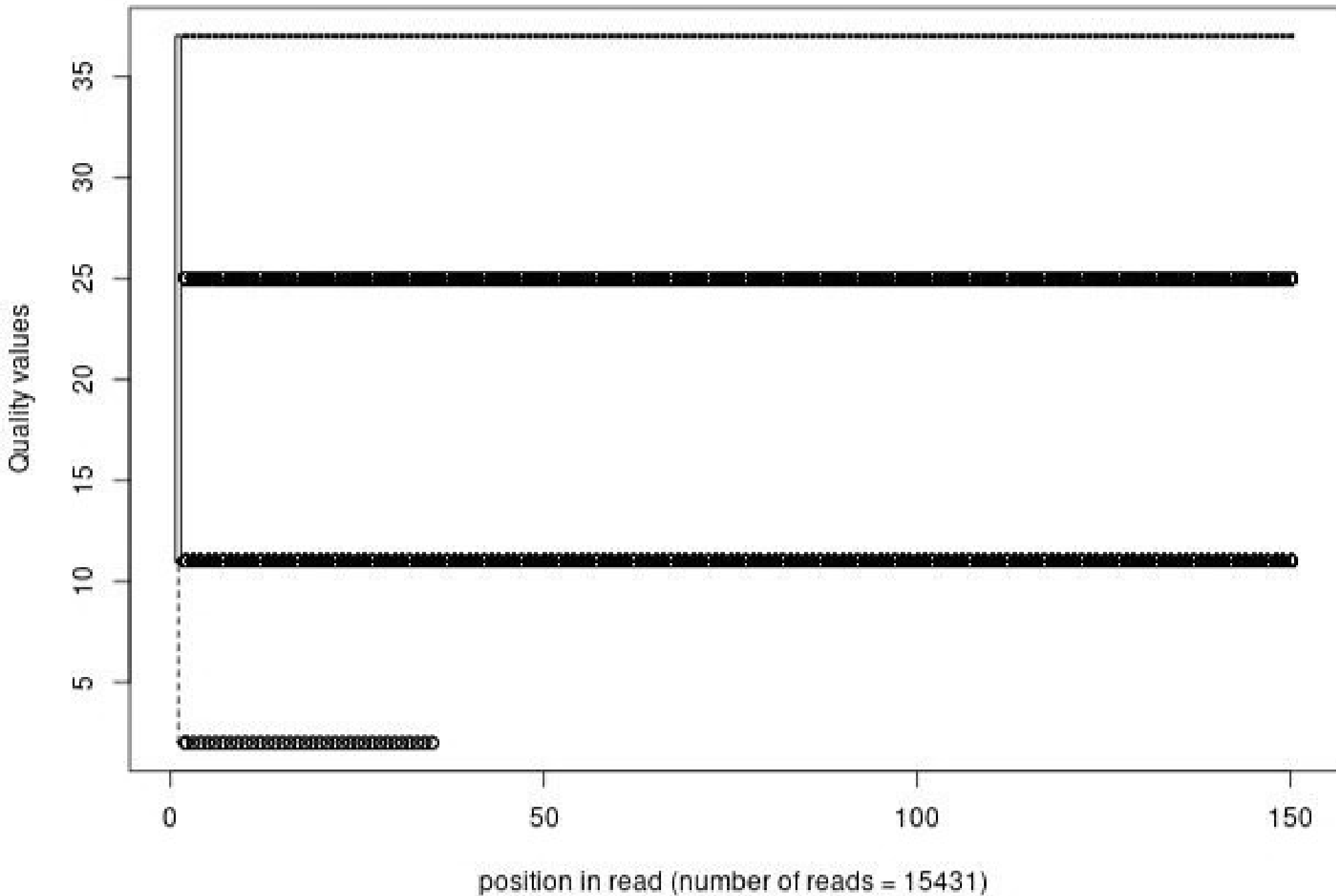
Quality distribution by position in read scer_hu_drugnone_oh031_01of10_1_frac1000_pad150
