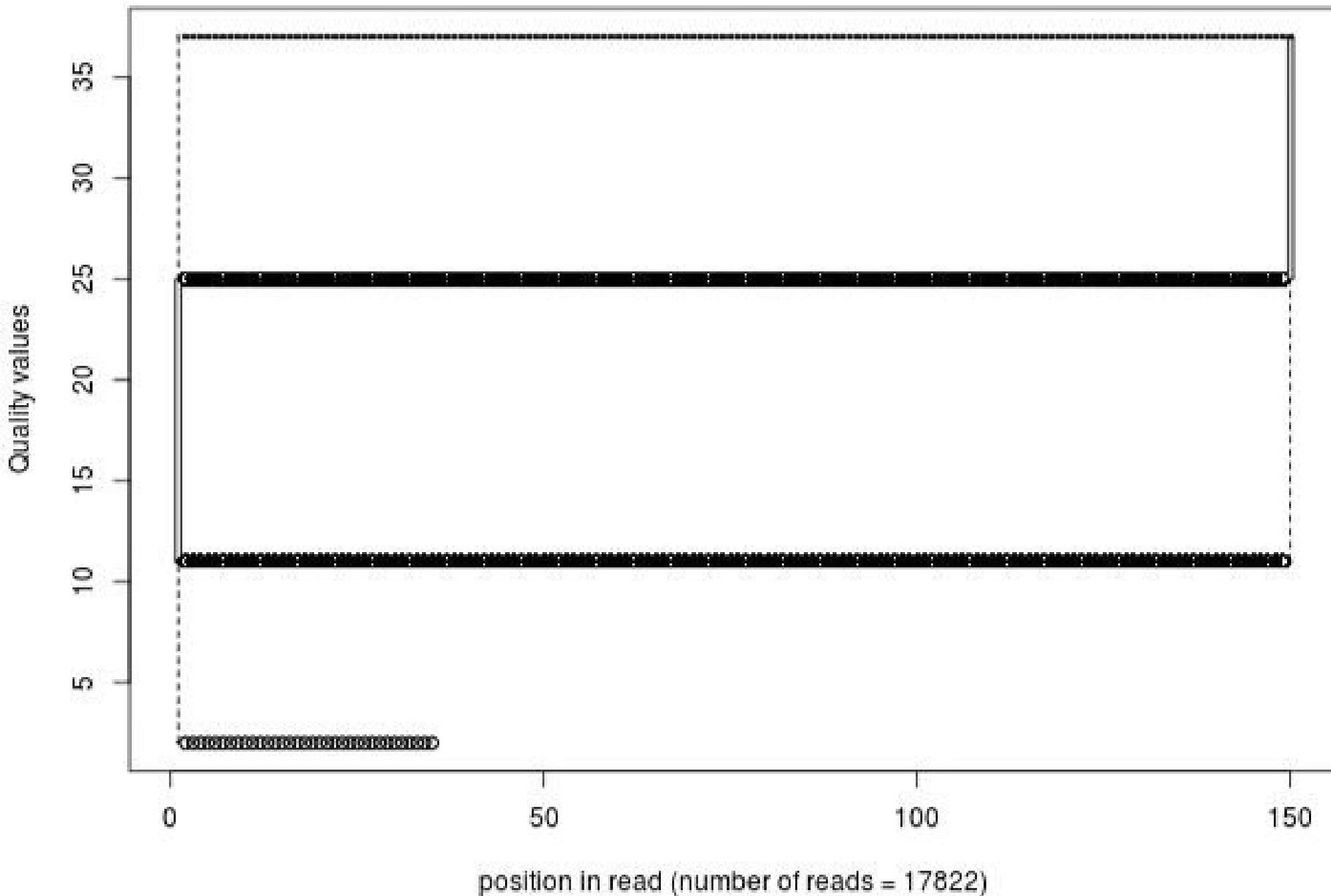
Quality distribution by position in read scer_wt_drugnone_oh029_01of10_2_frac1000_pad150
