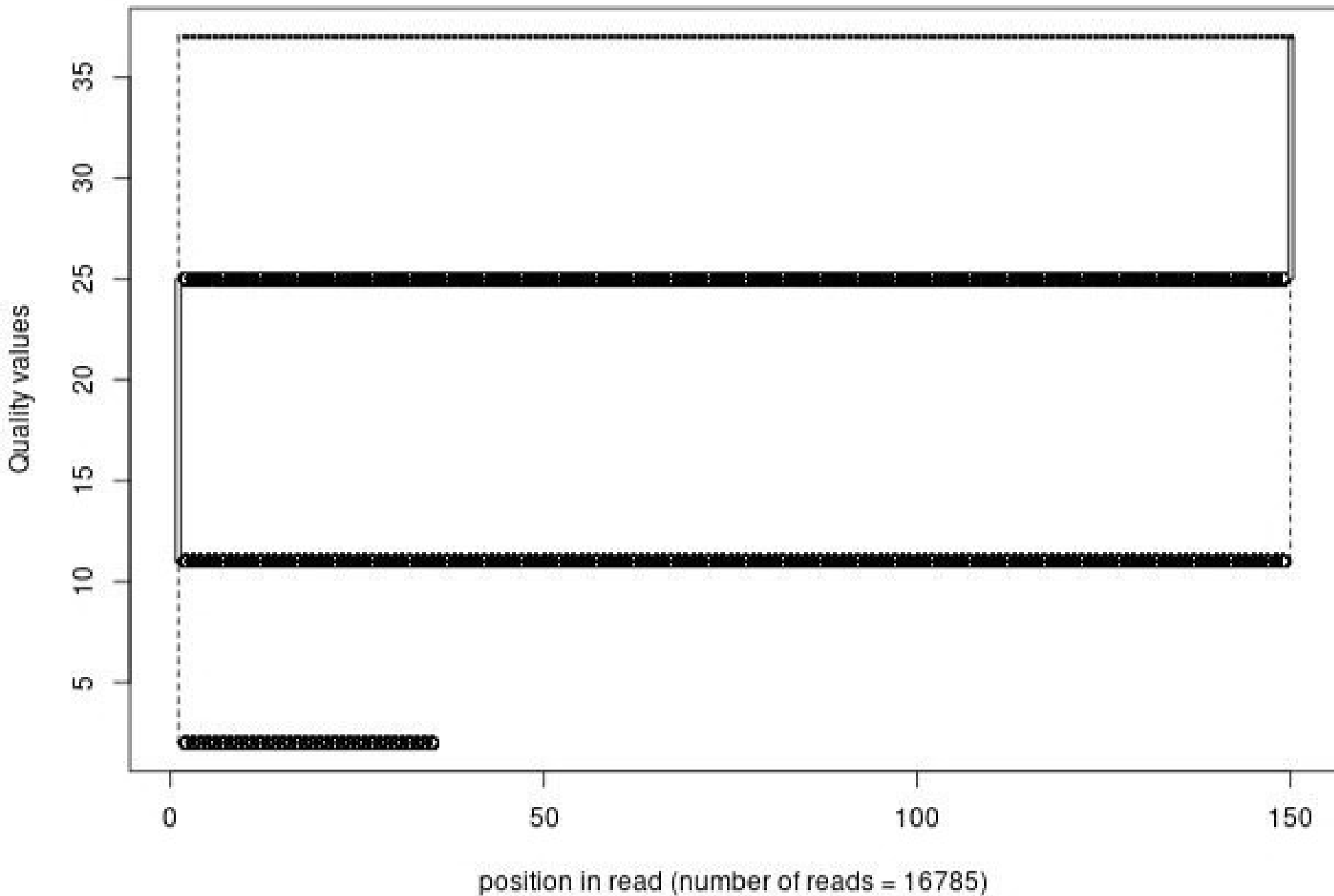
Quality distribution by position in read scer_hu_pladbxi_oh026_01of10_2_frac1000_pad150
