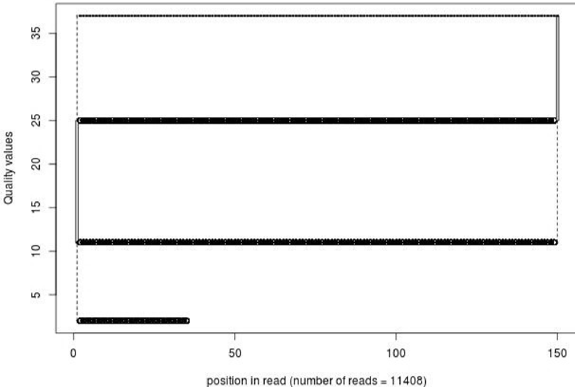
Quality distribution by position in read scer_wt_drugnone_oh035_01of10_2_frac1000_pad150
