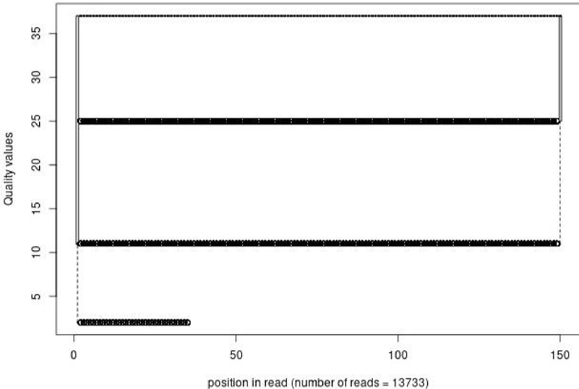
Quality distribution by position in read scer_hu_pladbxlo_oh033_01of10_2_frac1000_pad150
