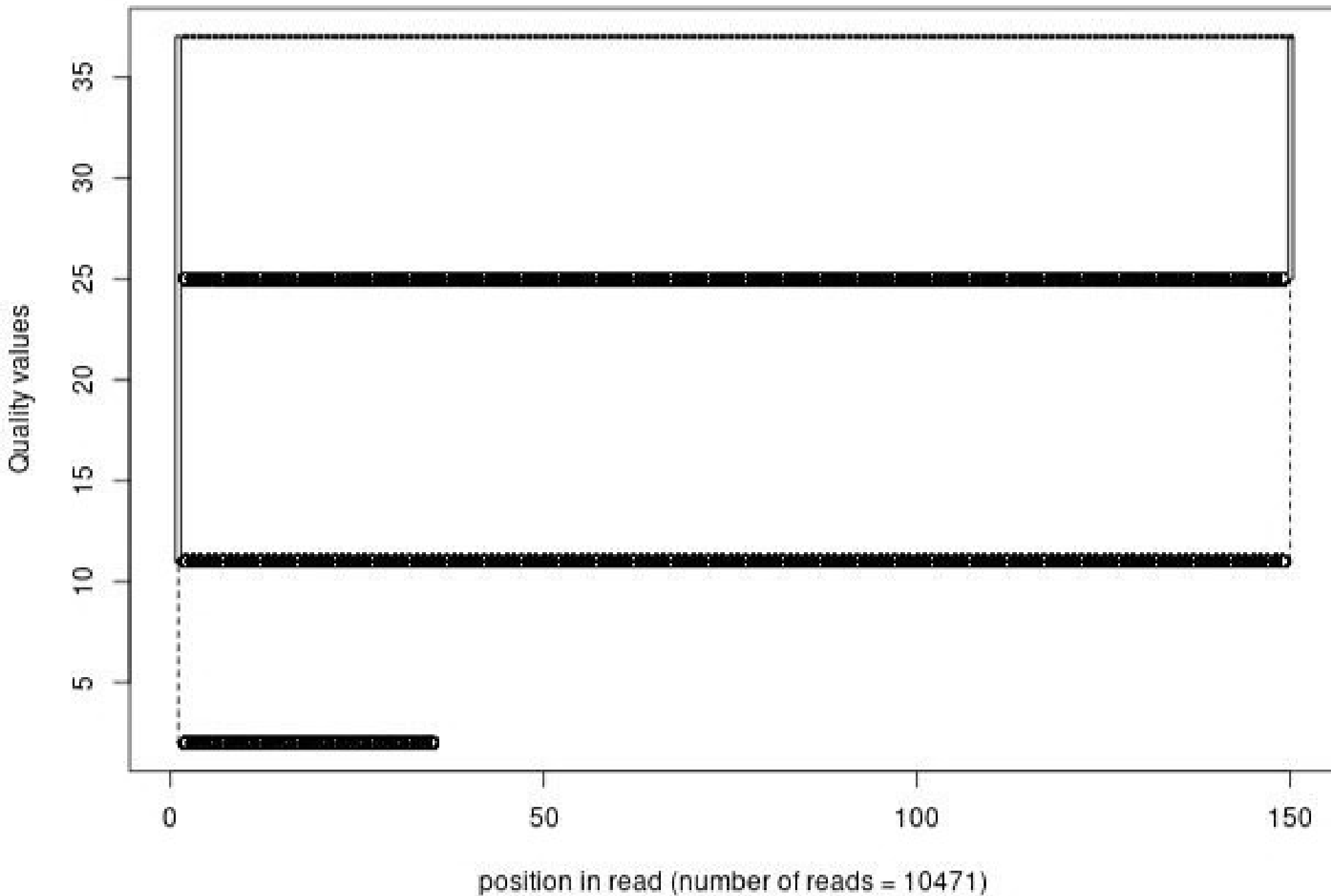
Quality distribution by position in read scer_wt_pladbxhi_oh036_01of10_2_frac1000_pad150
