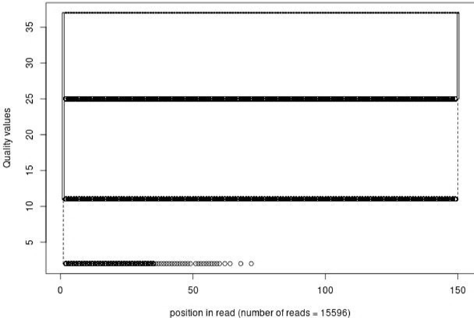
Quality distribution by position in read scer_wt_pladbxhi_oh030_01of10_2_frac1000_pad150
