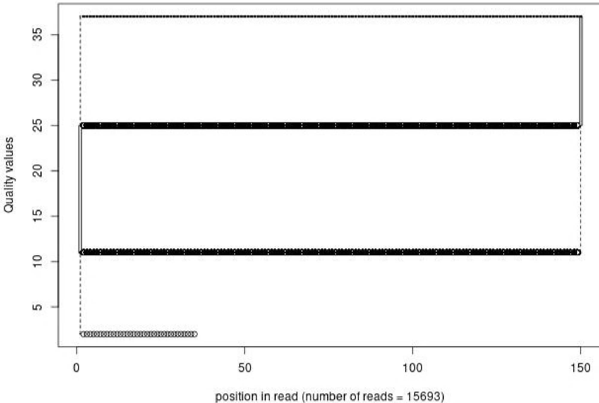
Quality distribution by position in read scer_hu_pladbxlo_oh027_01of10_2_frac1000_pad150
