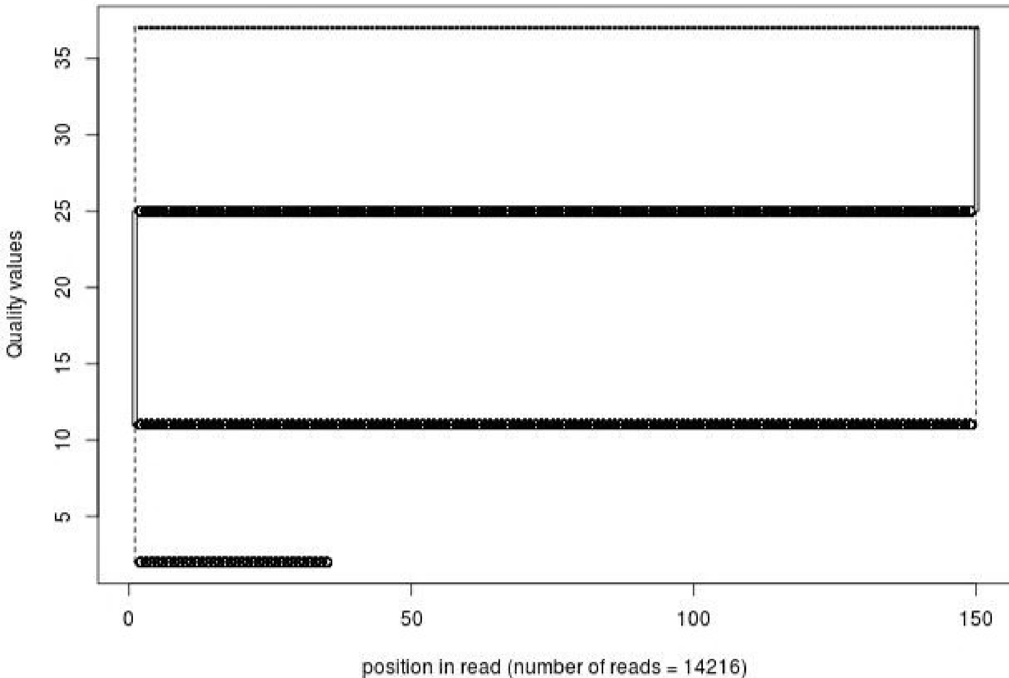
Quality distribution by position in read scer_hu_thailahi_oh028_01of10_2_frac1000_pad150
