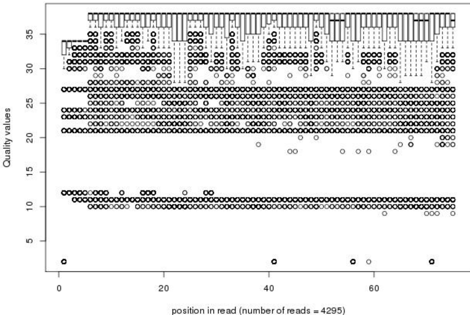
Quality distribution by position in read scer_12_ssp382_i7_ma002_00of1_2_frac100
