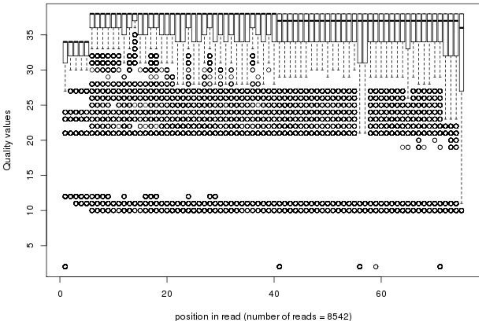
Quality distribution by position in read scer_21_wildxx_i2_ma007_00of10_2_frac100
