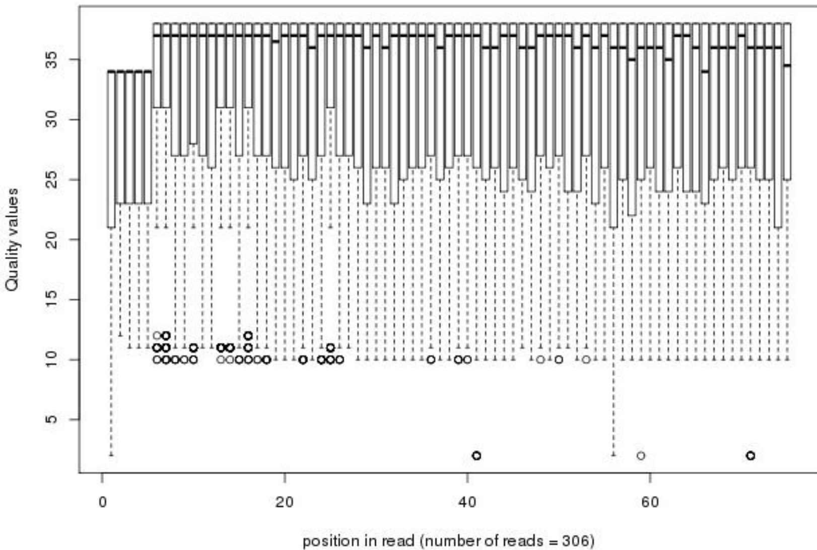
Quality distribution by position in read scer_15_trf6dx_i7_ma005_00of1_2_frac100
