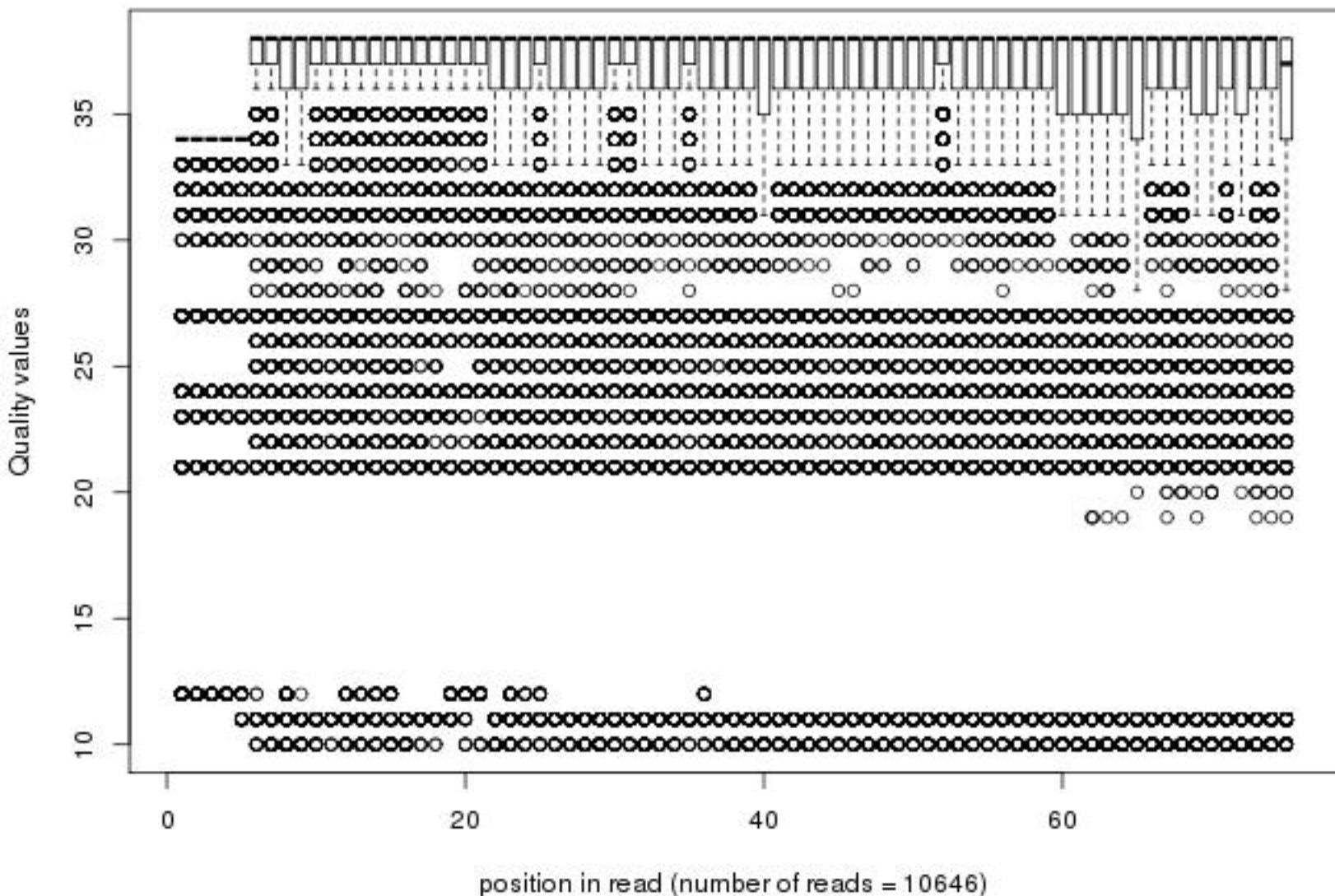
Quality distribution by position in read scer_11_wildxx_i7_ma001_00of1_1_frac100
