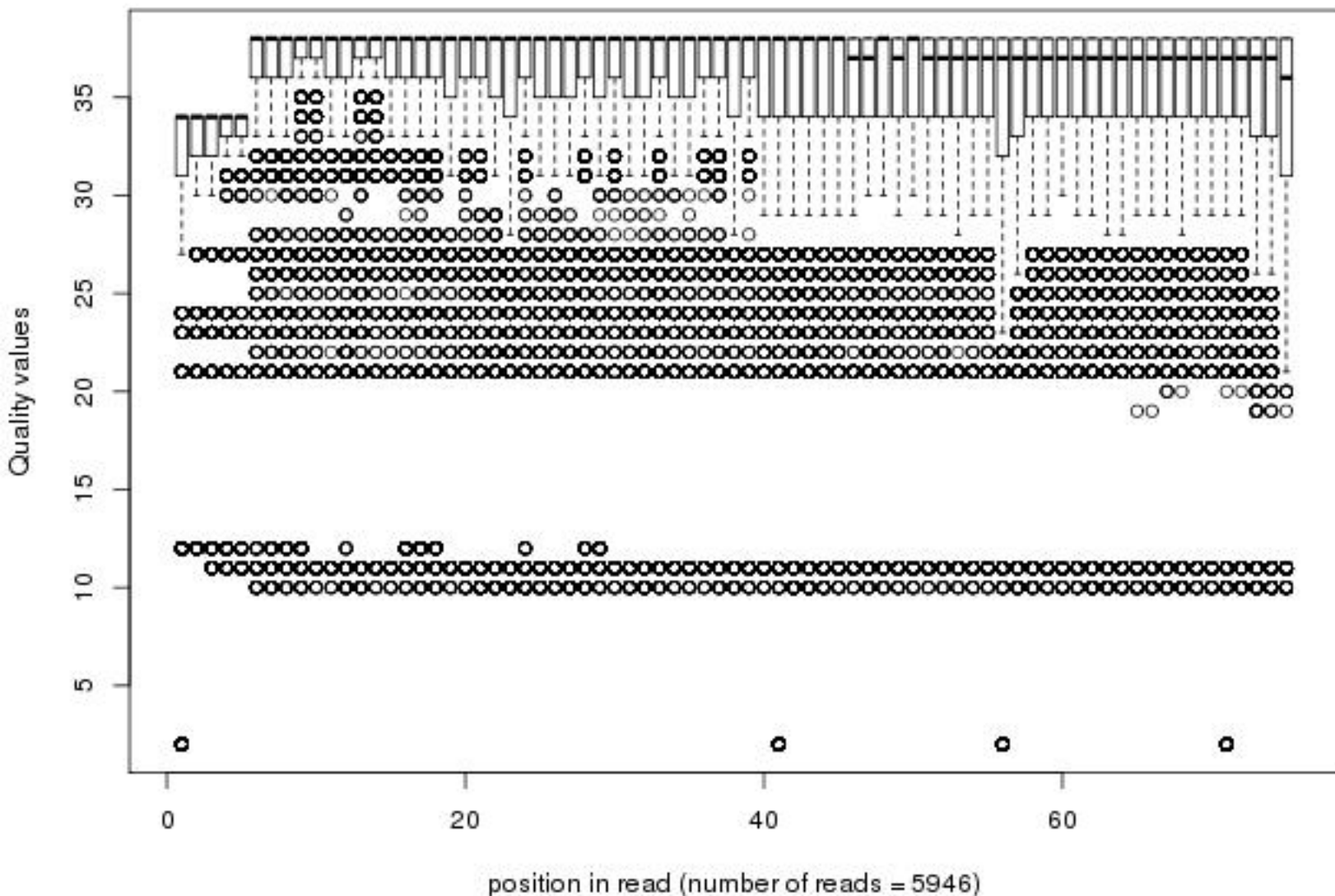
Quality distribution by position in read scer_22_ssp382_i2_ma008_00of1_2_frac100
