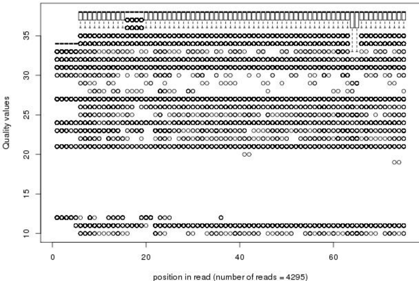
Quality distribution by position in read scer_12_ssp382_i7_ma002_00of1_1_frac100
