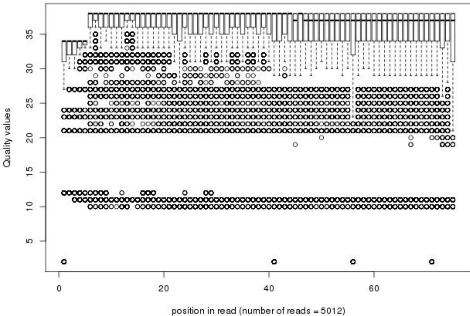
Quality distribution by position in read scer_23_trf4dx_i2_ma009_00of1_2_frac100
