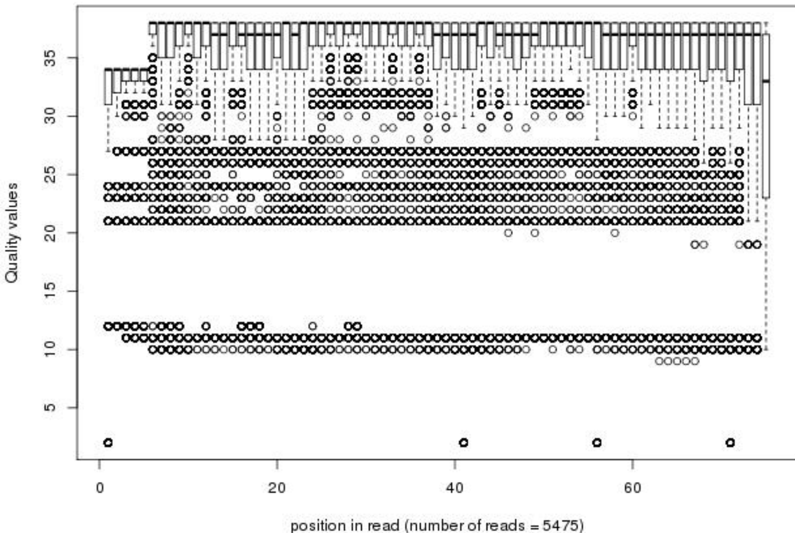
Quality distribution by position in read scer_14_trf5dx_i7_ma004_00of1_2_frac100
