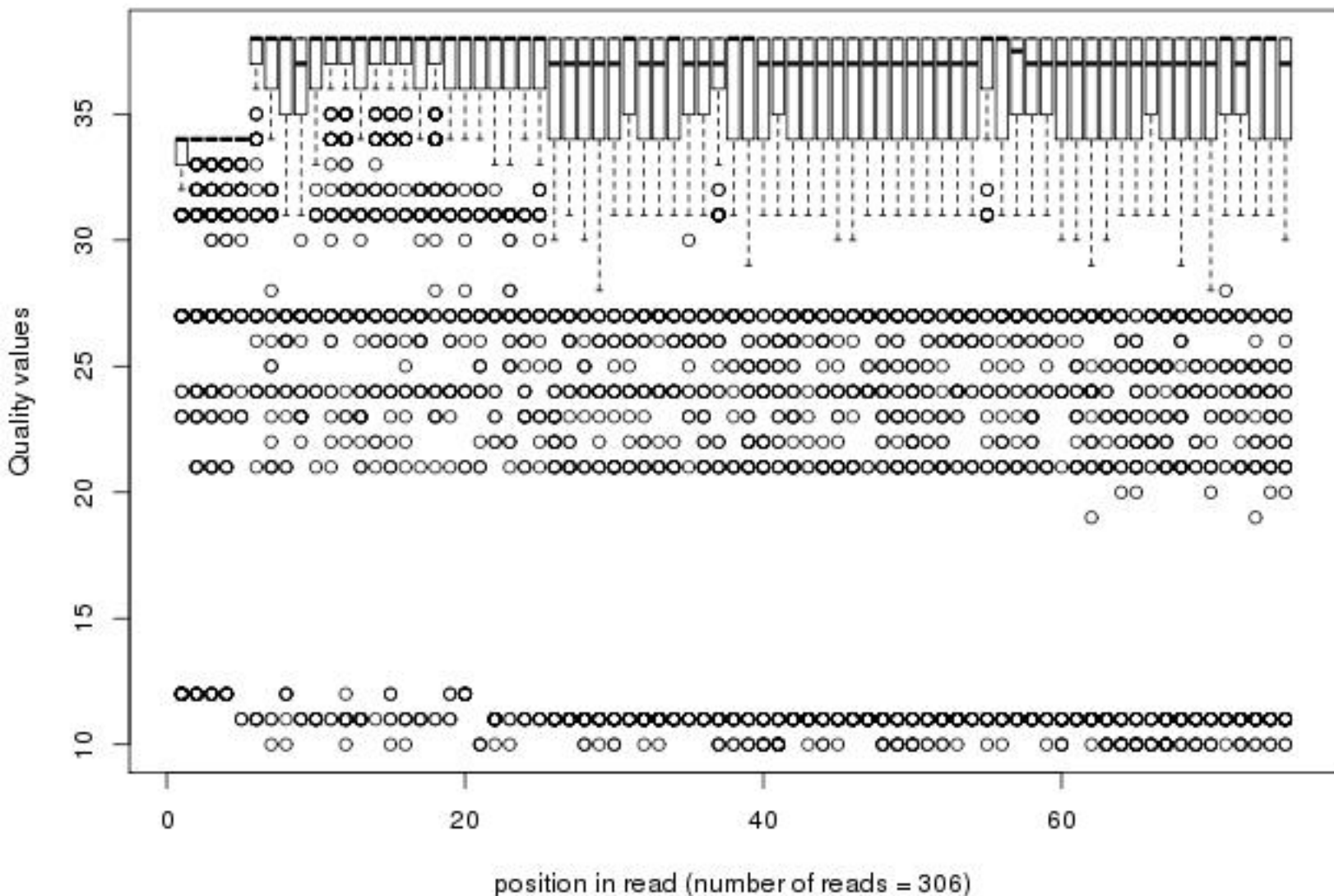
Quality distribution by position in read scer_15_trf6dx_i7_ma005_00of1_1_frac100
