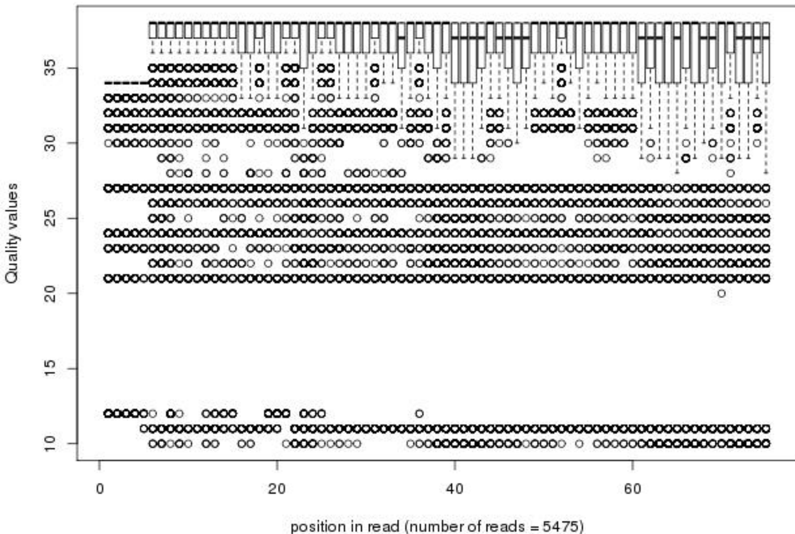
Quality distribution by position in read scer_14_trf5dx_i7_ma004_00of1_1_frac100
