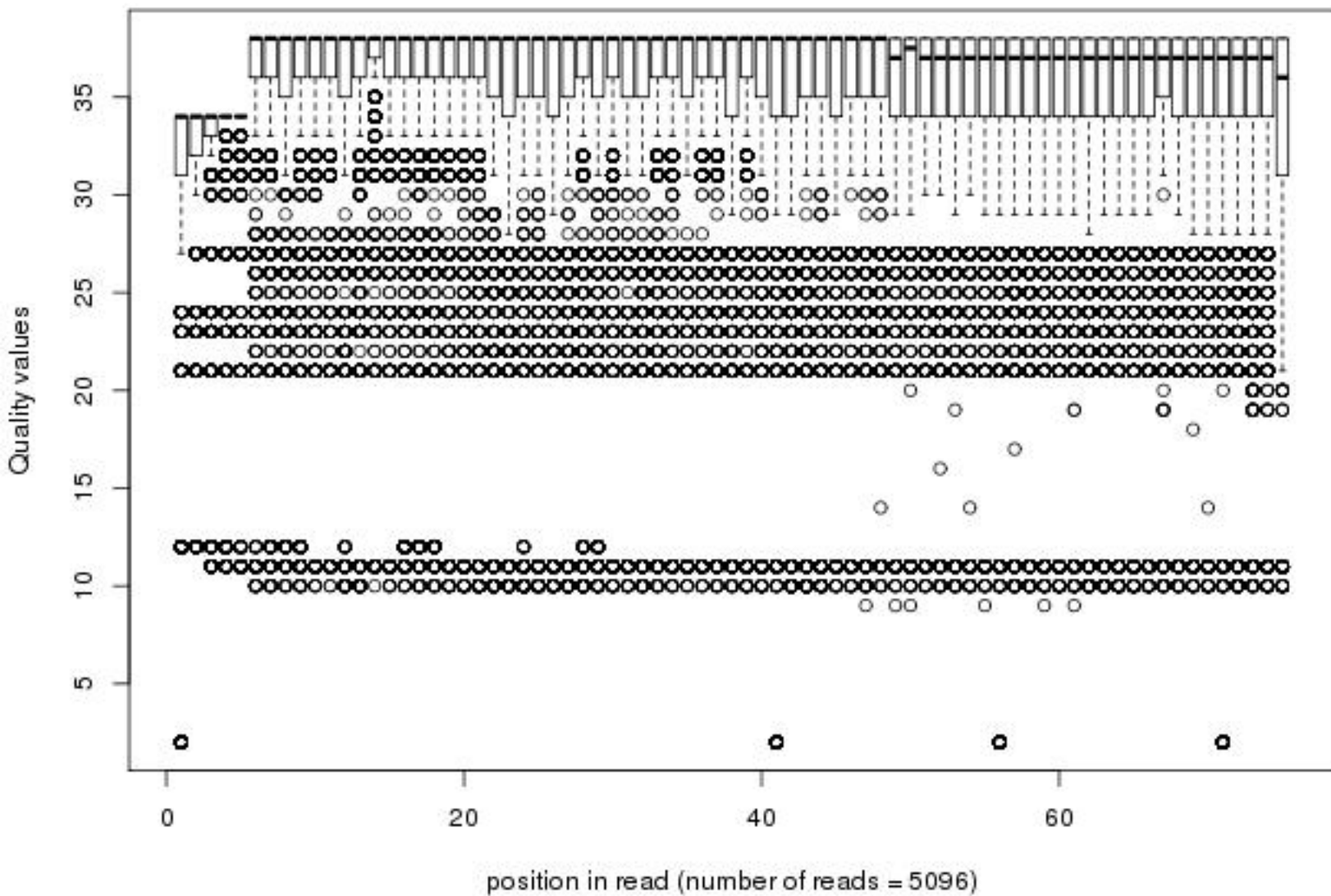
Quality distribution by position in read scer_24_trf5dx_i2_ma010_00of1_2_frac100
