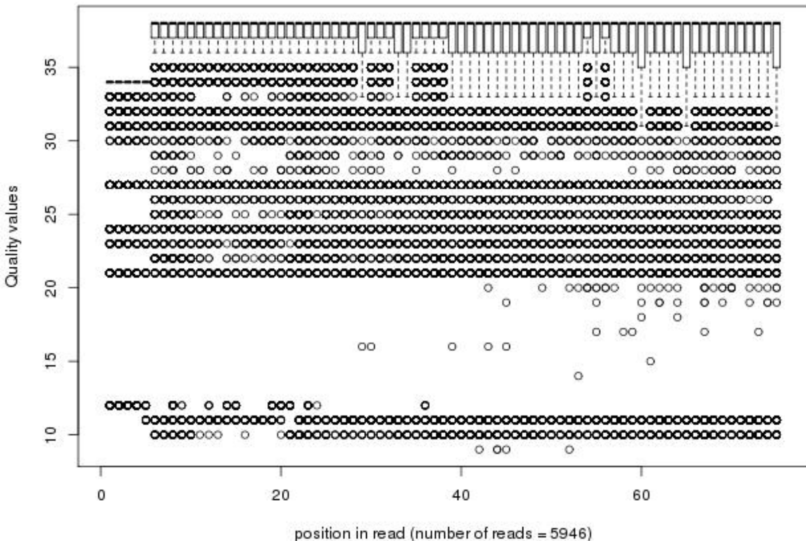
Quality distribution by position in read scer_22_ssp382_i2_ma008_00of1_1_frac100
