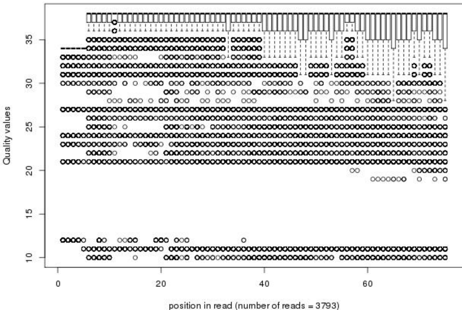
Quality distribution by position in read scer_26_drn1dx_i2_ma012_00of1_1_frac100
