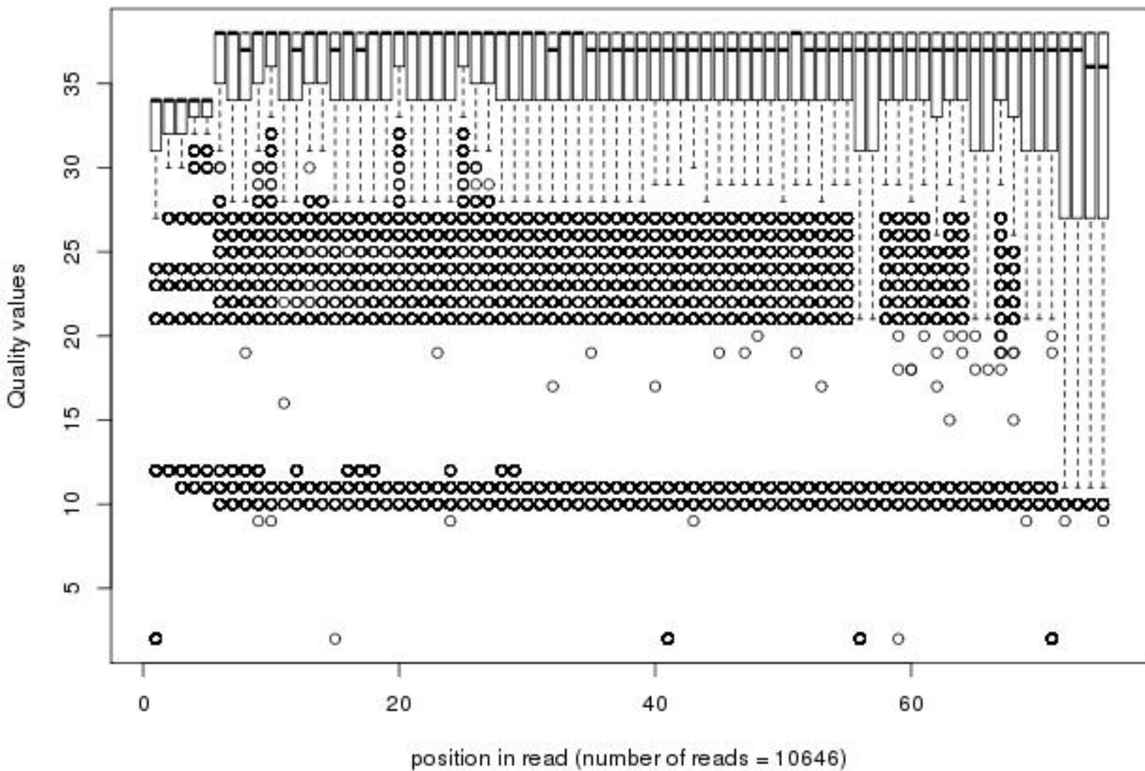
Quality distribution by position in read scer_11_wildxx_i7_ma001_00of1_2_frac100
