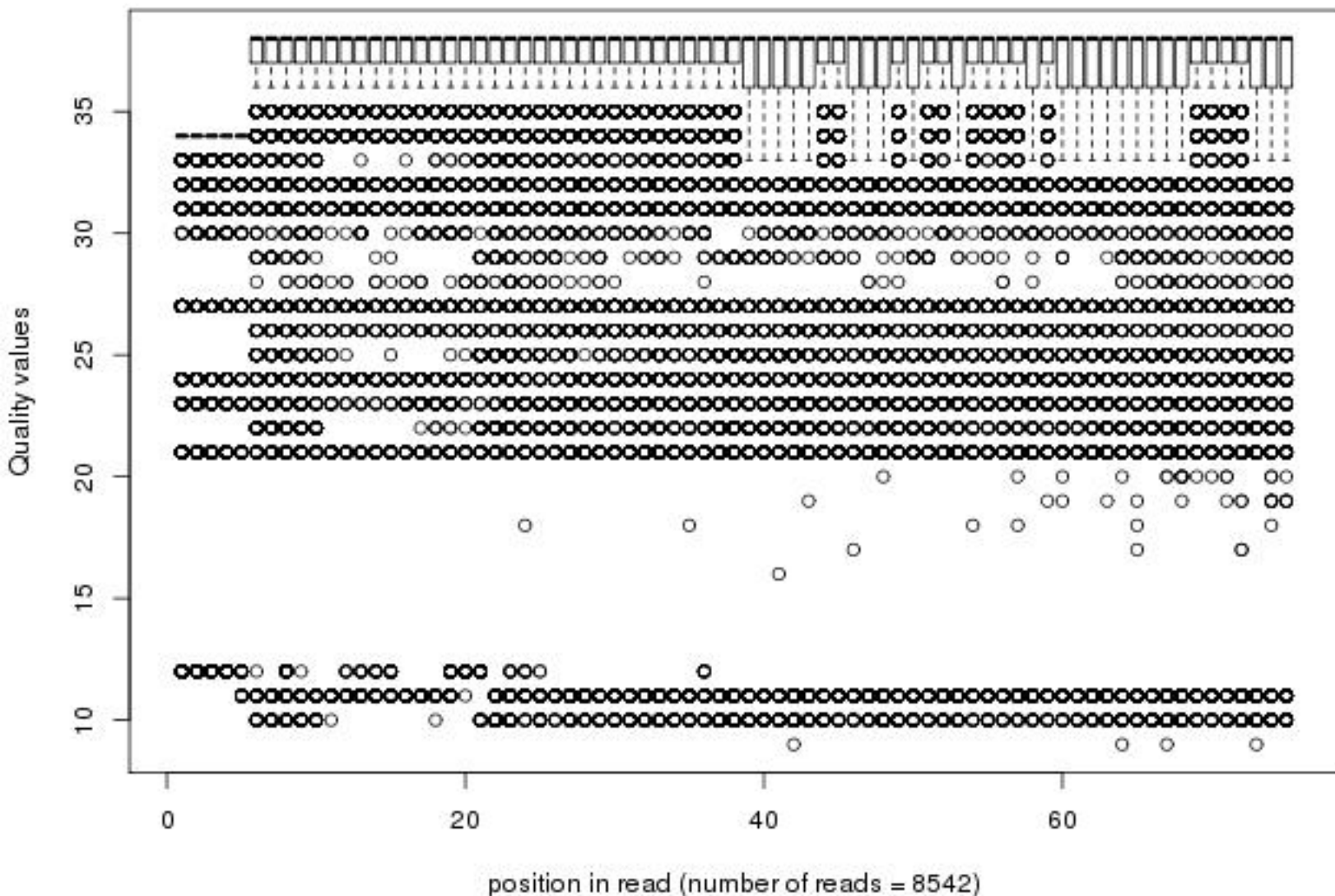
Quality distribution by position in read scer_21_wildxx_i2_ma007_00of10_1_frac100
