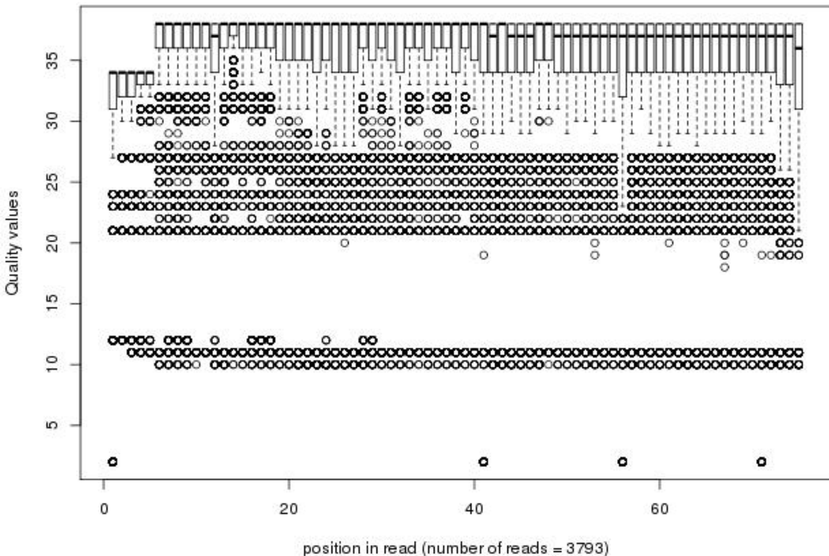
Quality distribution by position in read scer_26_drn1dx_i2_ma012_00of1_2_frac100
