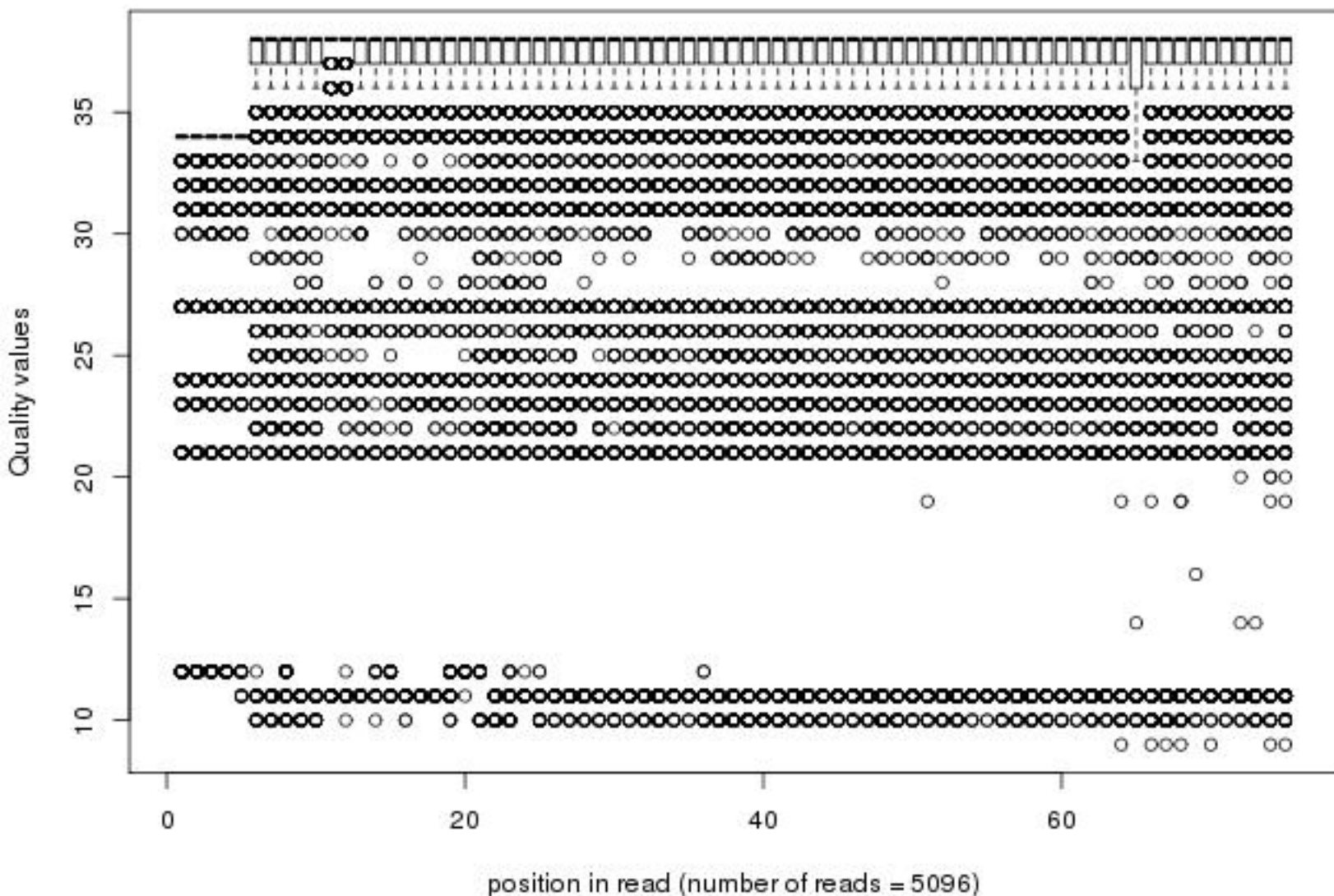
Quality distribution by position in read scer_24_trf5dx_i2_ma010_00of1_1_frac100
