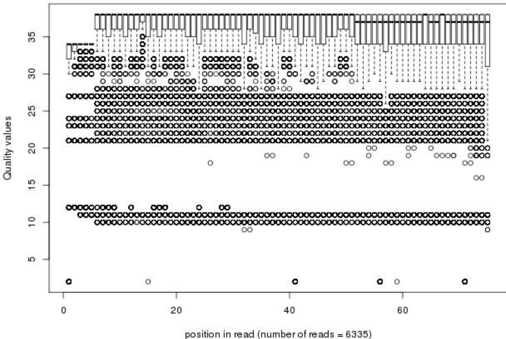
Quality distribution by position in read scer_16_drn1dx_i7_ma006_00of1_2_frac100
