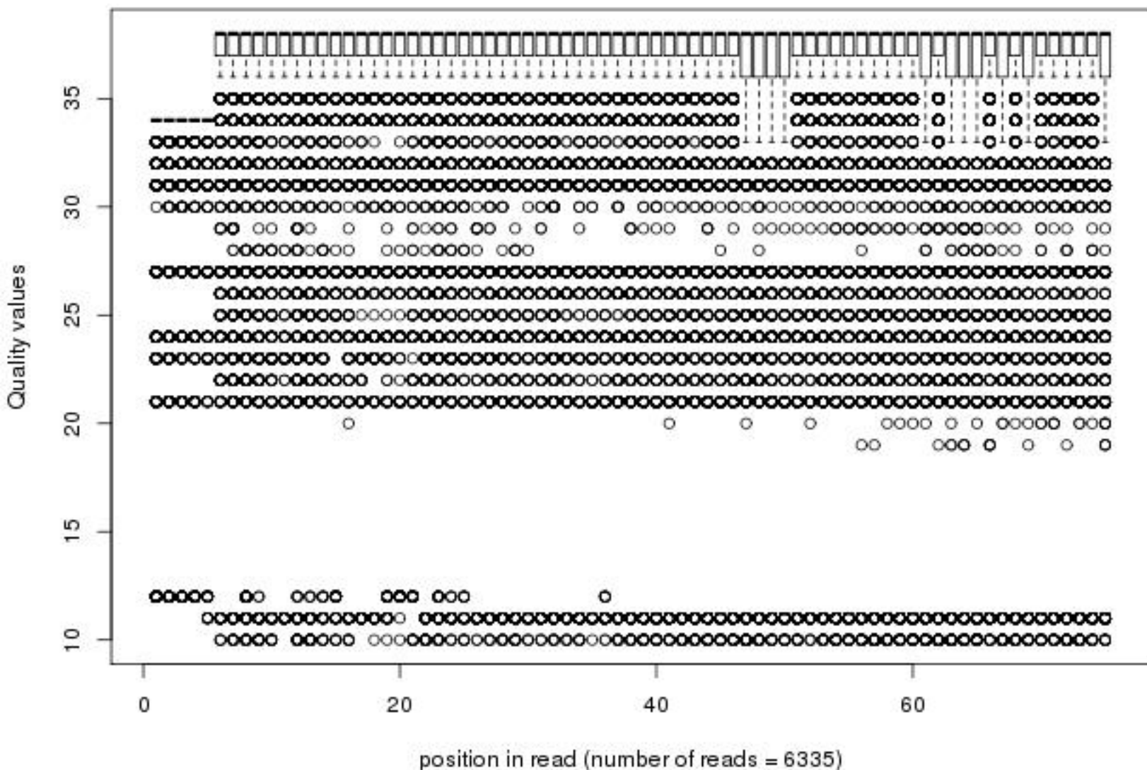
Quality distribution by position in read scer_16_drn1dx_i7_ma006_00of1_1_frac100
