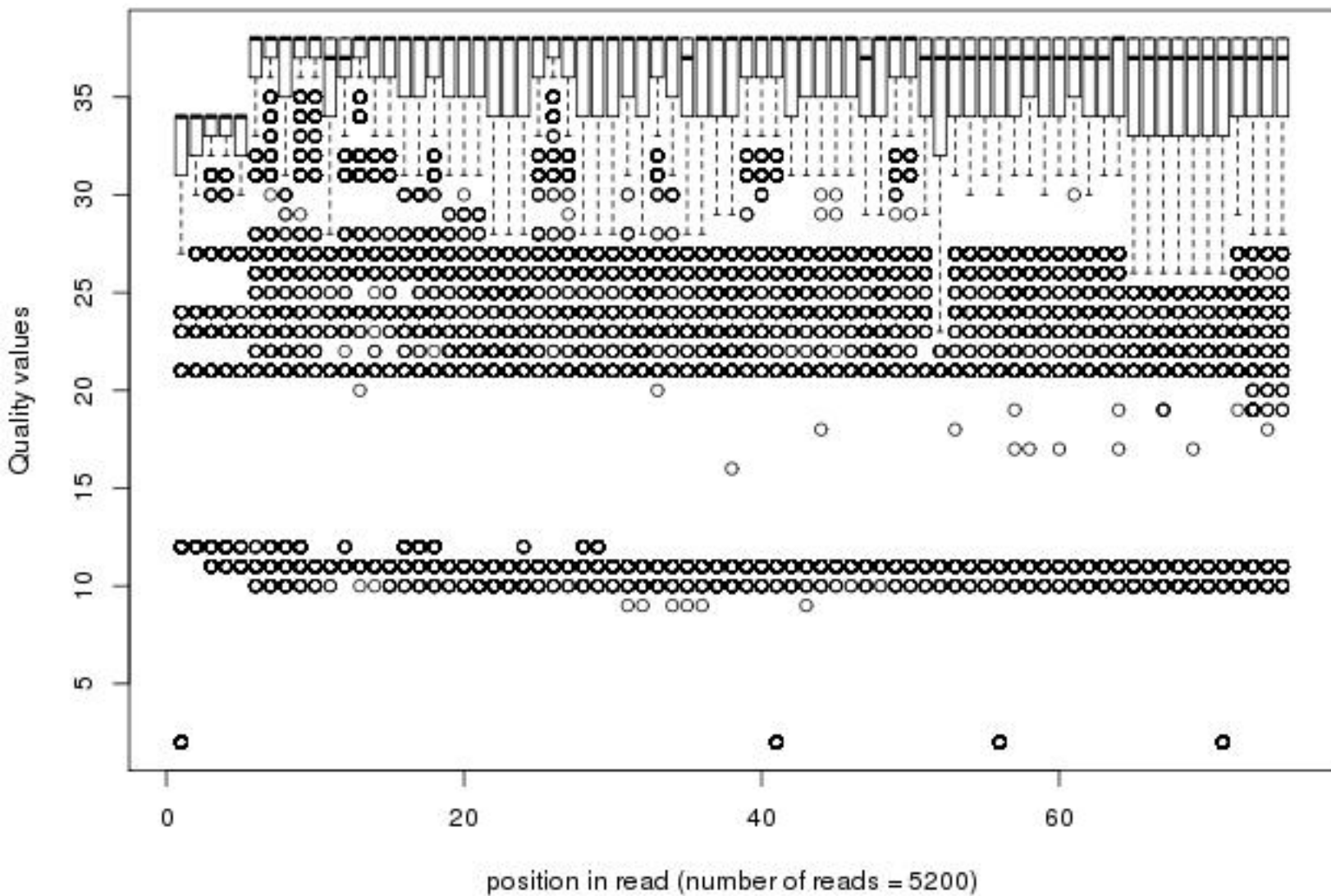
Quality distribution by position in read scer_13_trf4dx_i7_ma003_00of1_2_frac100
