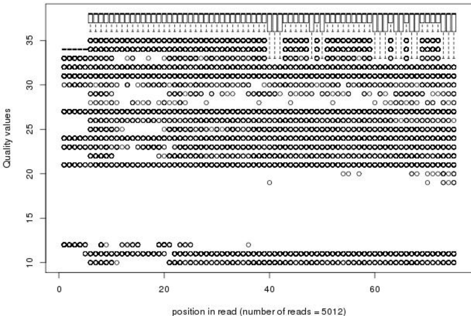
Quality distribution by position in read scer_23_trf4dx_i2_ma009_00of1_1_frac100
