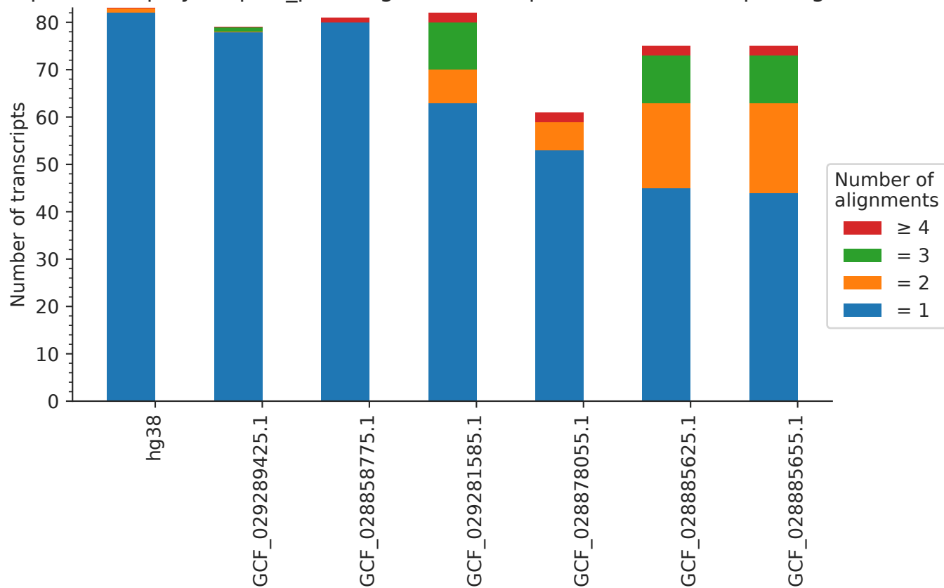
Proportion of polymorphic_pseudogene transcripts that have multiple alignments
