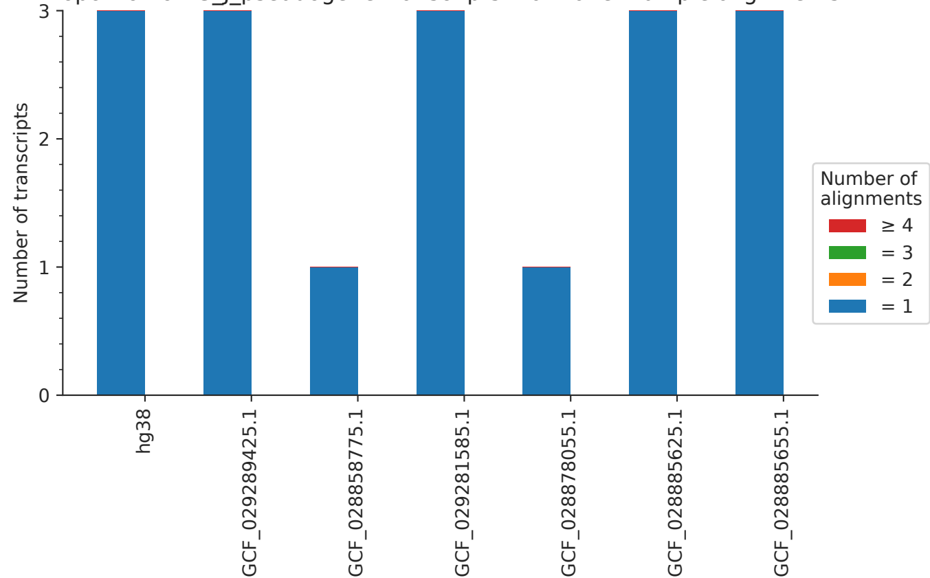
Proportion of IG_J_pseudogene transcripts that have multiple alignments
