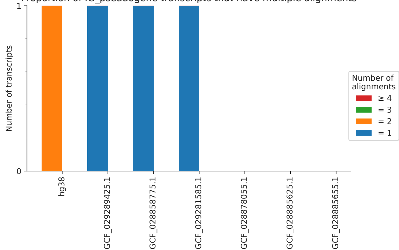
Proportion of IG_pseudogene transcripts that have multiple alignments
