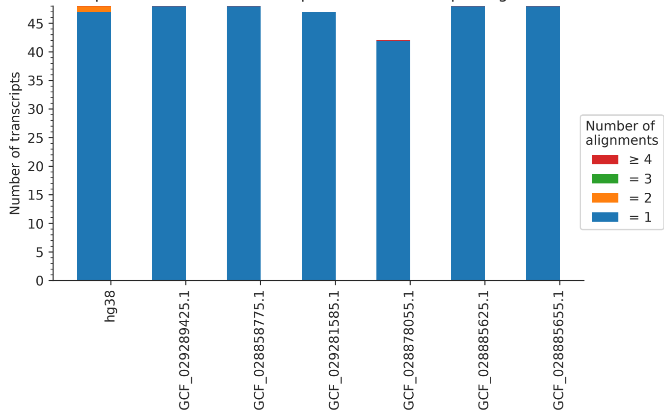
Proportion of scaRNA transcripts that have multiple alignments
