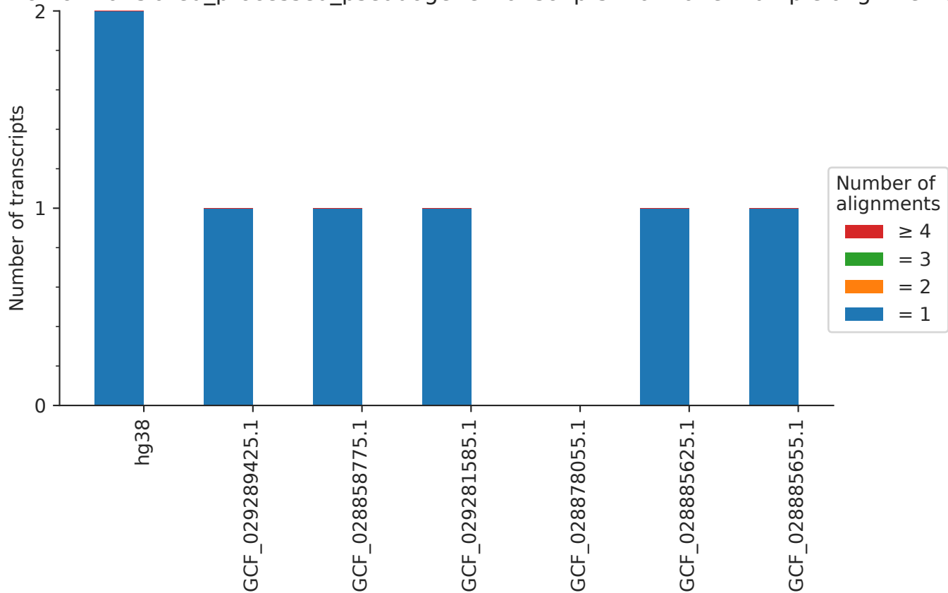
Proportion of translated_processed_pseudogene transcripts that have multiple alignments
