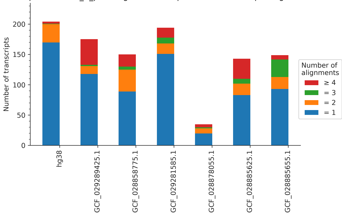
Proportion of IG_V_pseudogene transcripts that have multiple alignments
