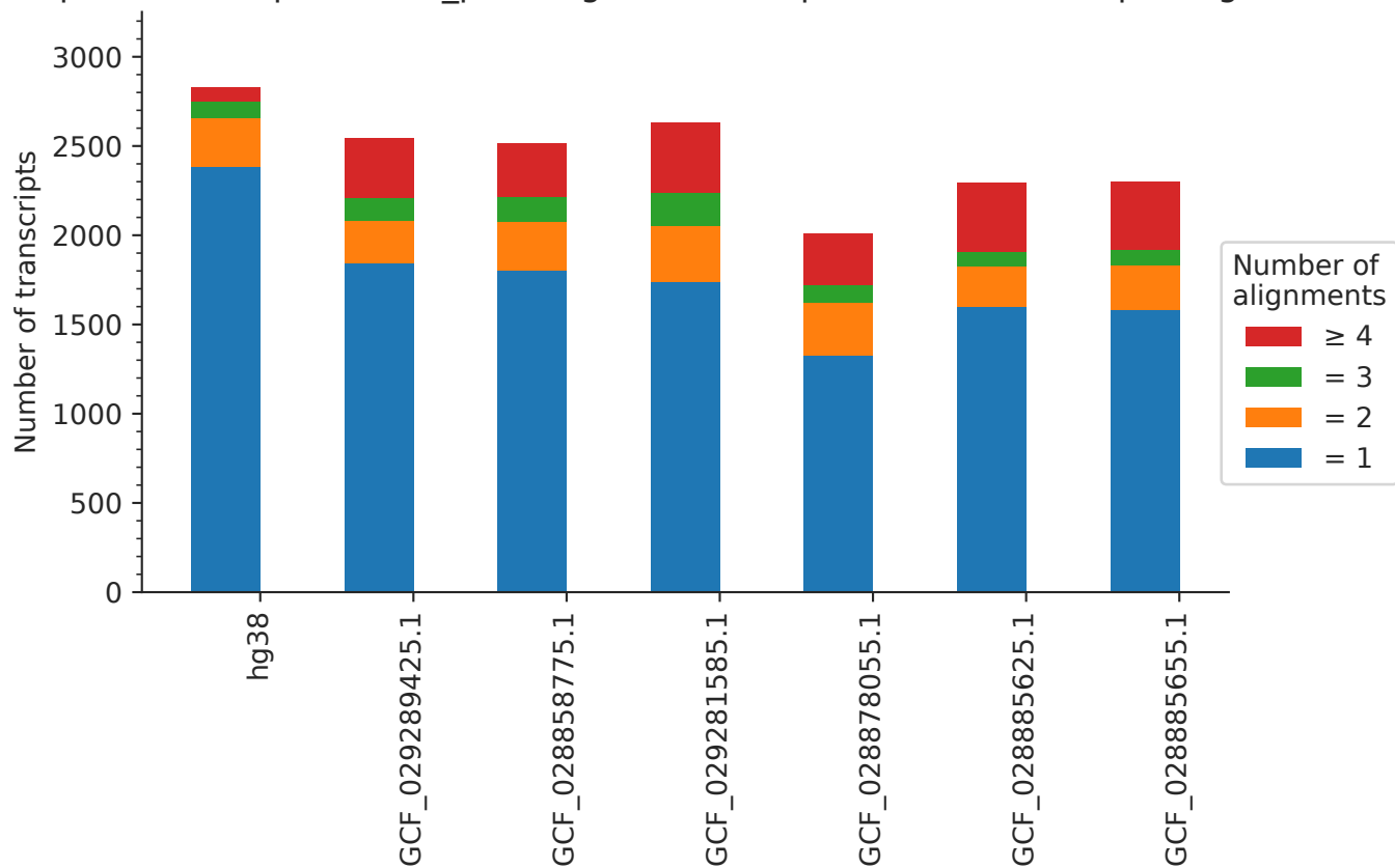
Proportion of unprocessed_pseudogene transcripts that have multiple alignments
