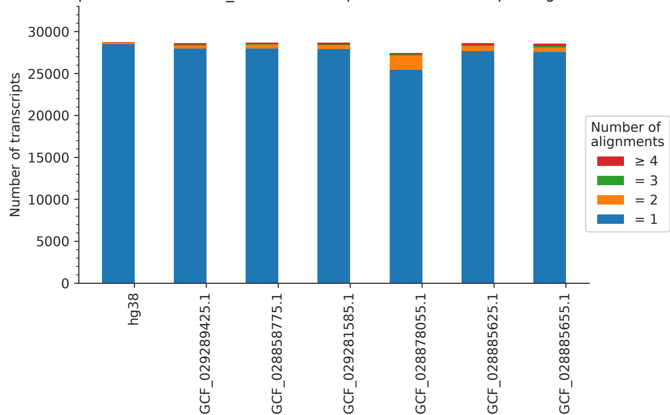
Proportion of retained_intron transcripts that have multiple alignments
