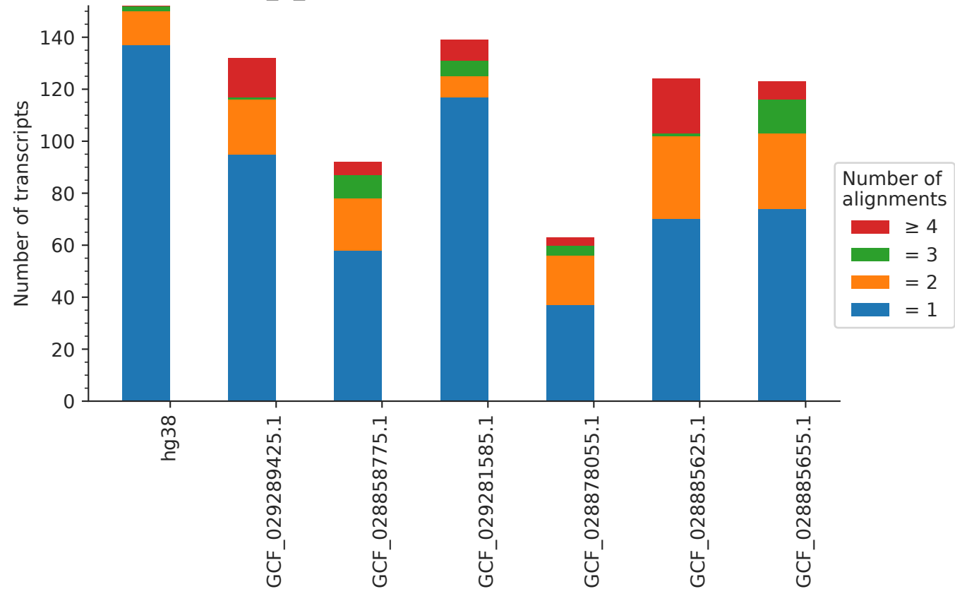
Proportion of IG_V_gene transcripts that have multiple alignments
