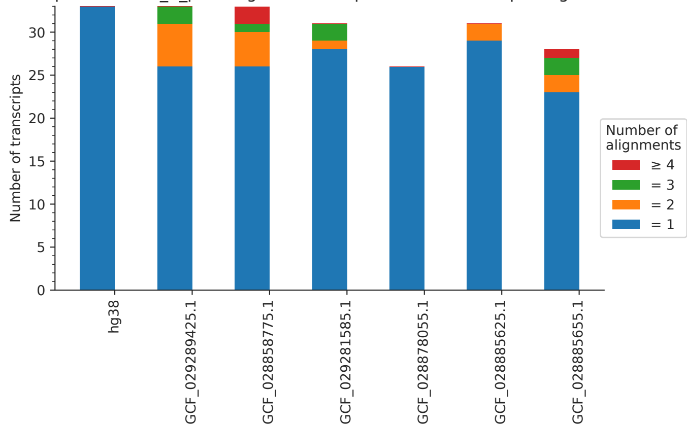
Proportion of TR_V_pseudogene transcripts that have multiple alignments
