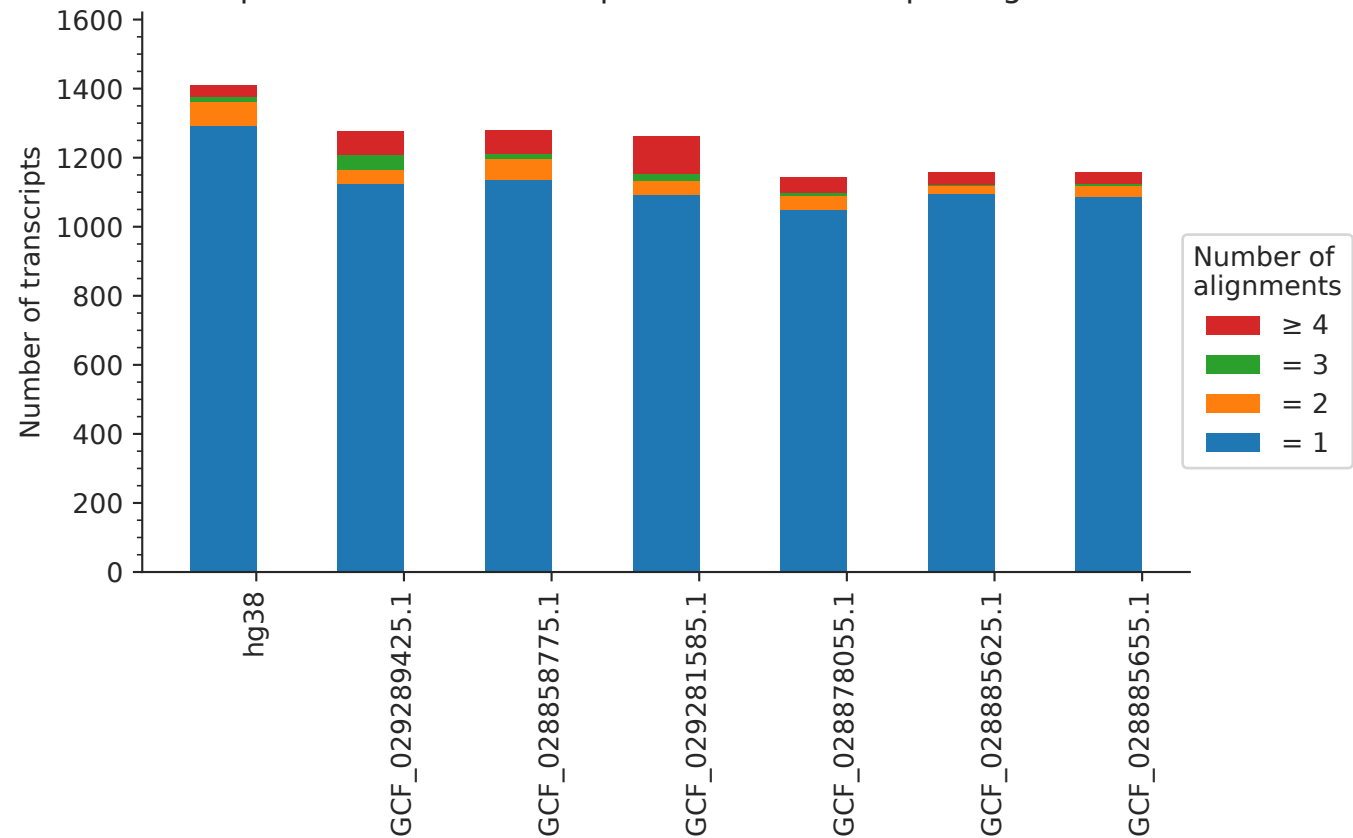
Proportion of TEC transcripts that have multiple alignments
