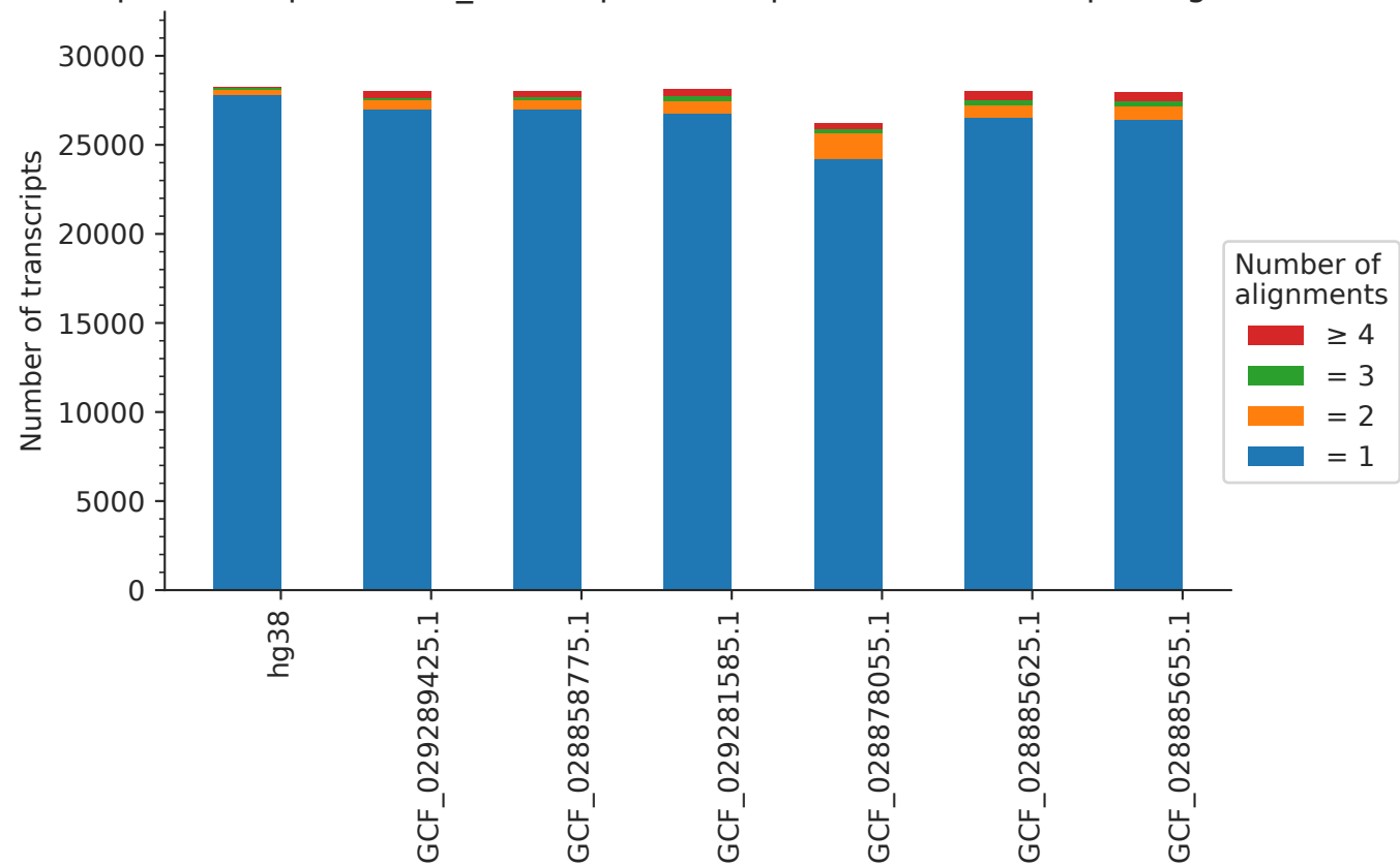
Proportion of processed_transcript transcripts that have multiple alignments
