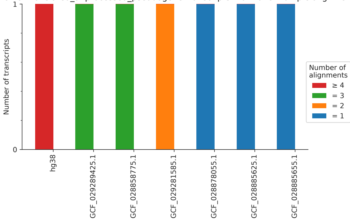
Proportion of translated_unprocessed_pseudogene transcripts that have multiple alignments
