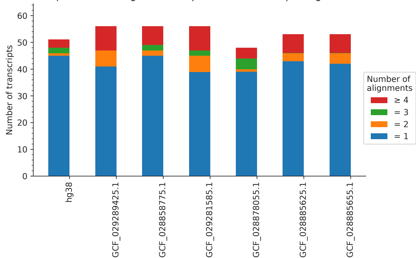
Proportion of StringTie transcripts that have multiple alignments
