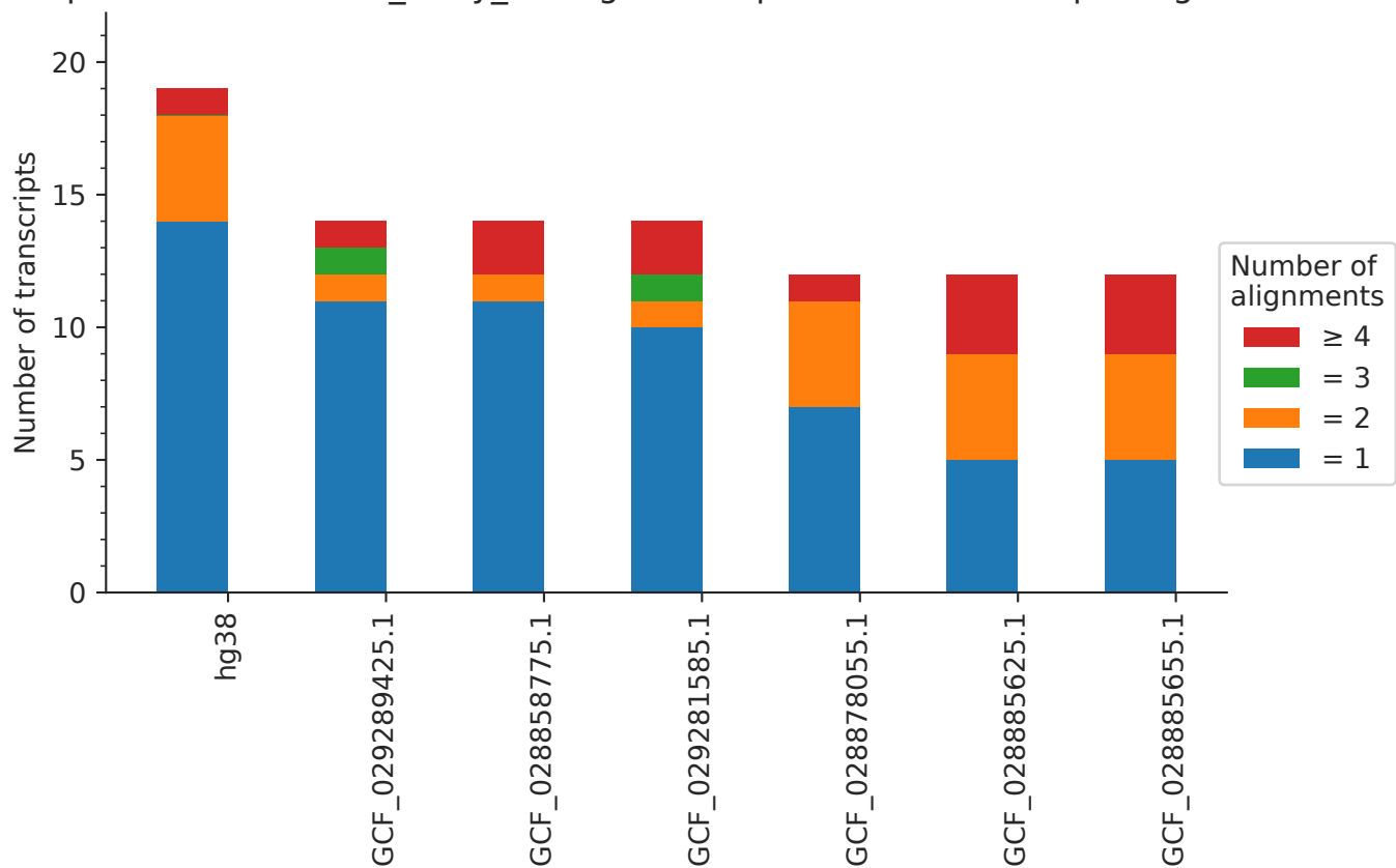
Proportion of unknown_likely_coding transcripts that have multiple alignments
