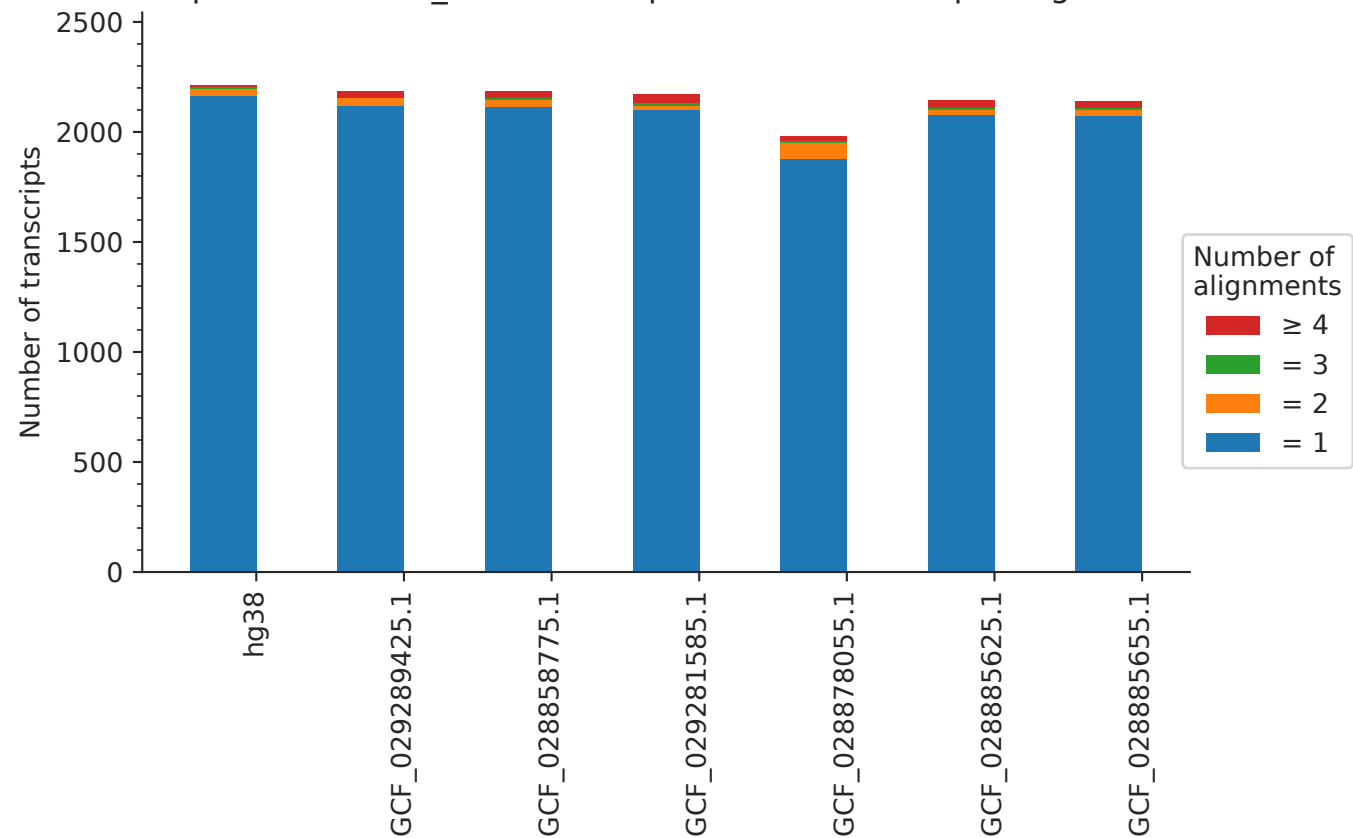
Proportion of misc_RNA transcripts that have multiple alignments
