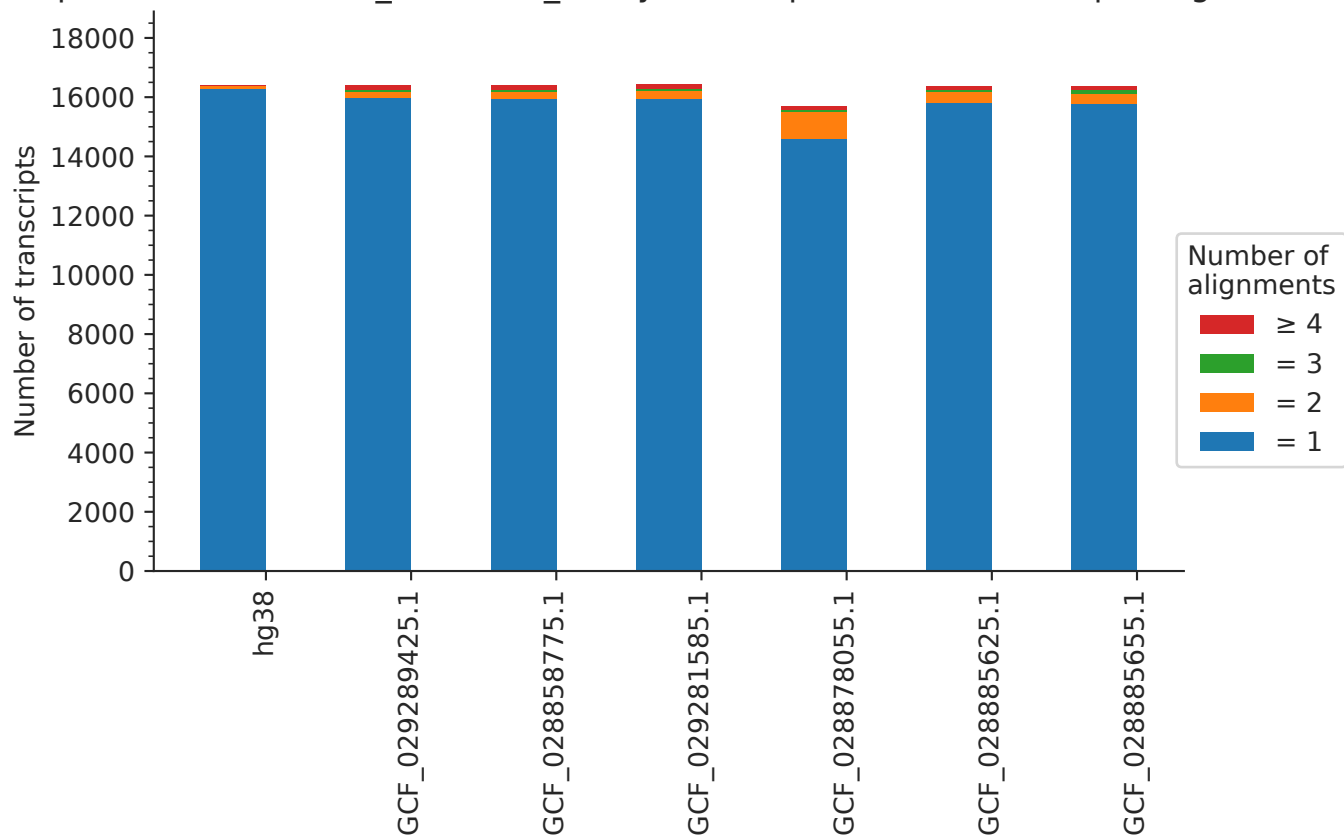
Proportion of nonsense_mediated_decay transcripts that have multiple alignments
