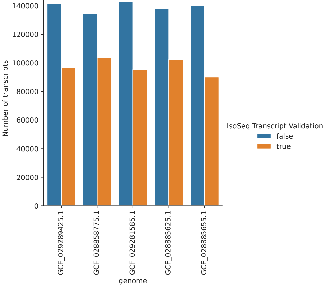
Isoforms validated by at least one IsoSeq read
